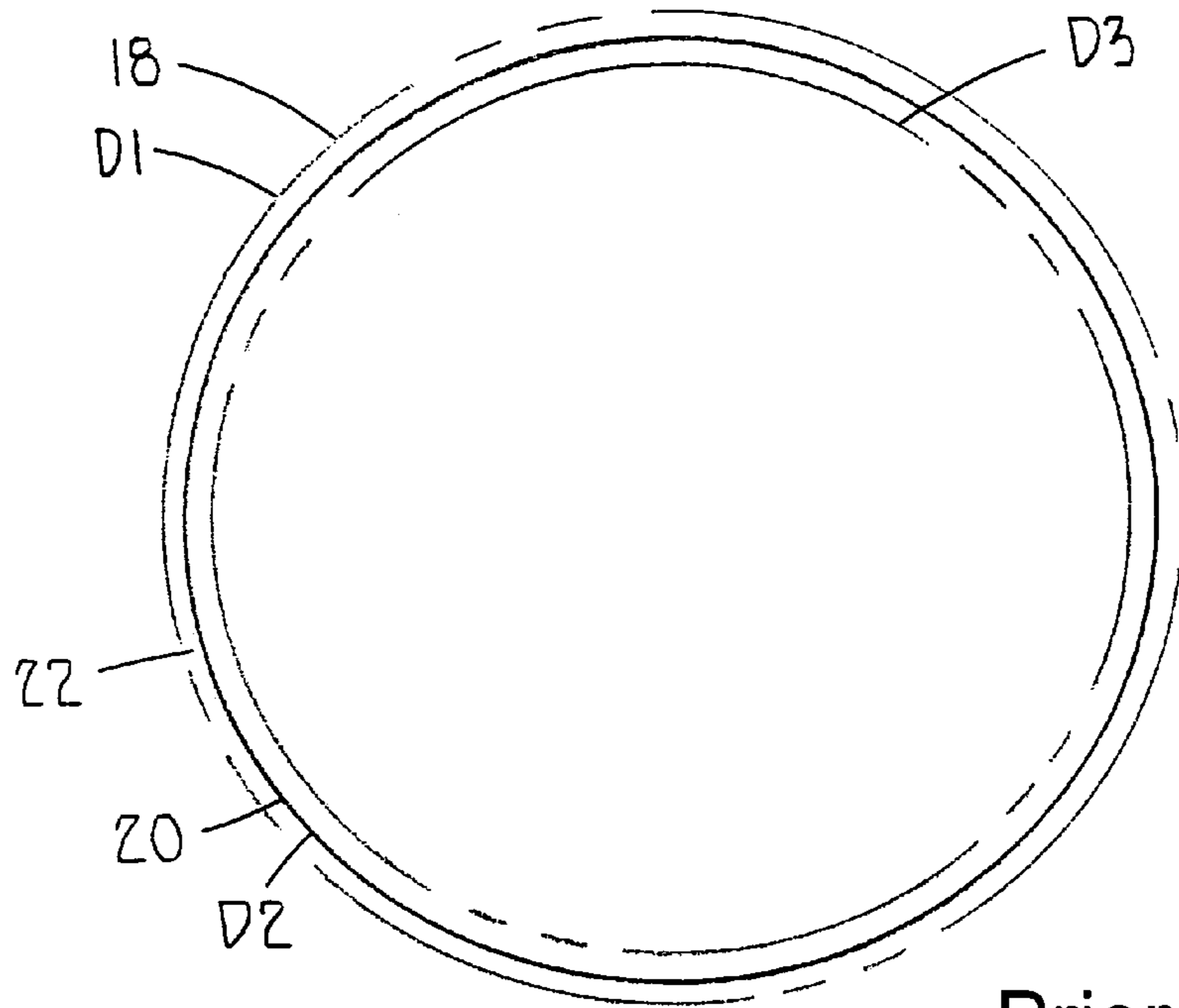
Prior Art
