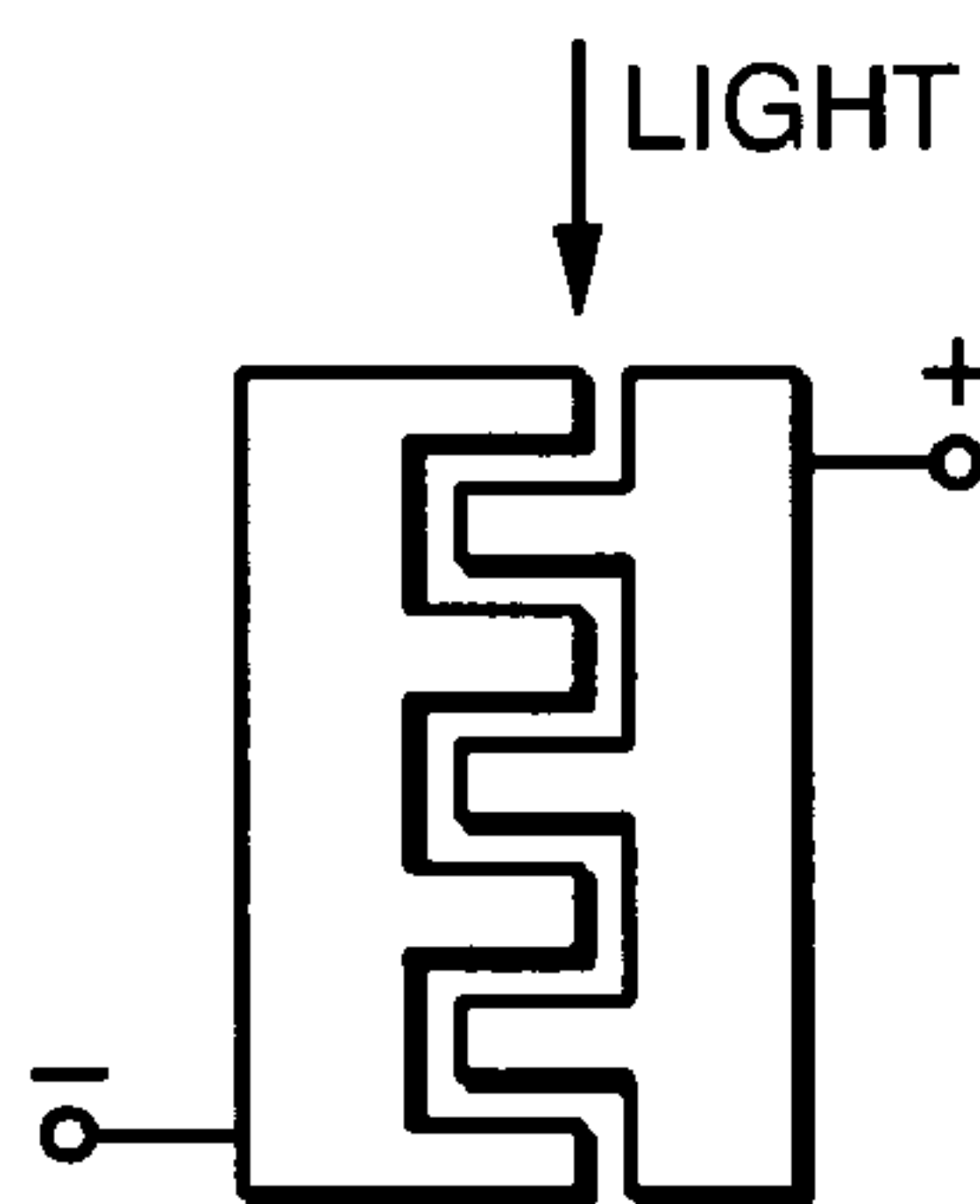
FIG. 27 (PRIOR ART)
