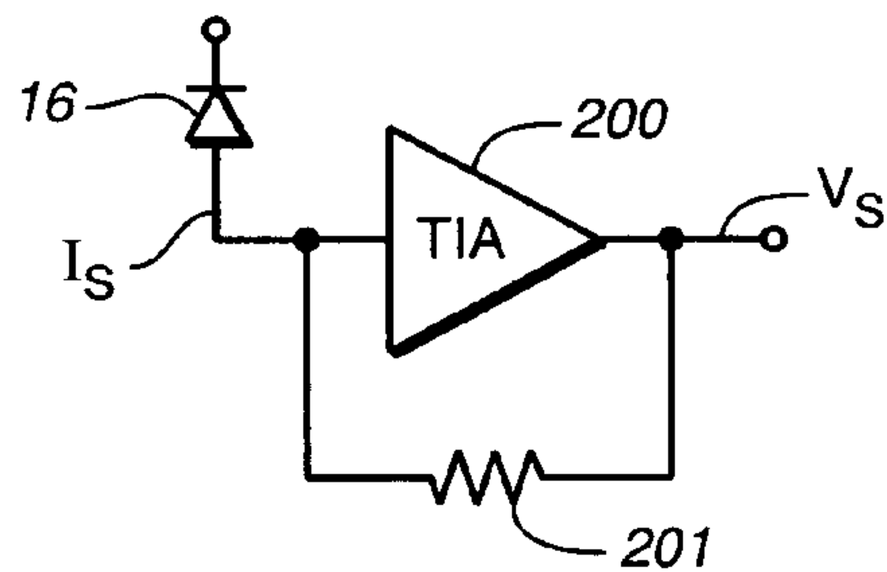
FIG. 48 (PRIOR ART)
