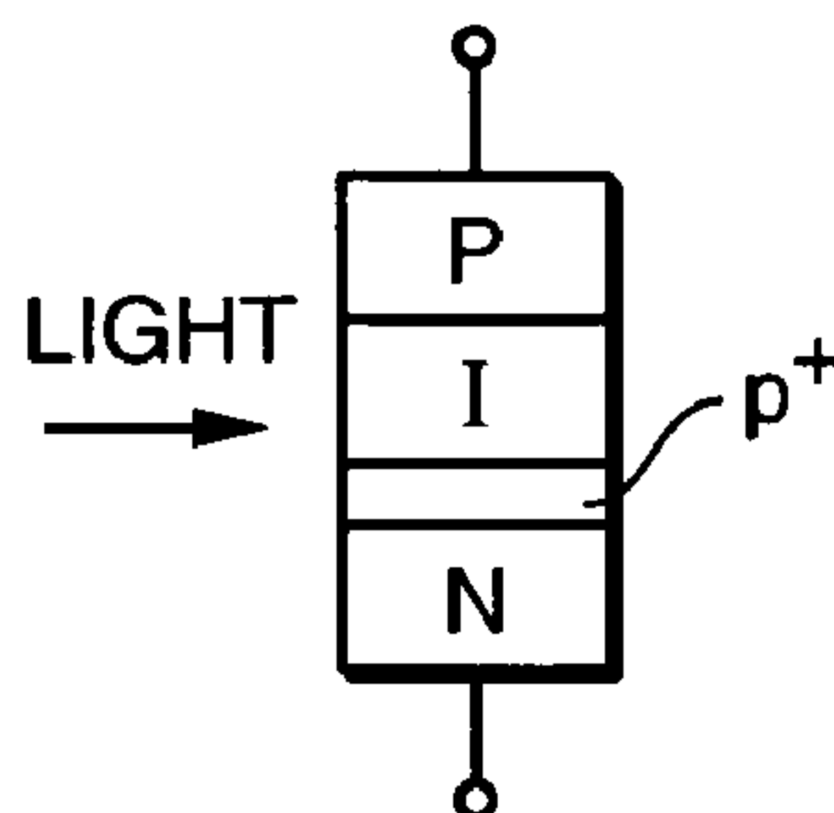
FIG. 26 (PRIOR ART)
