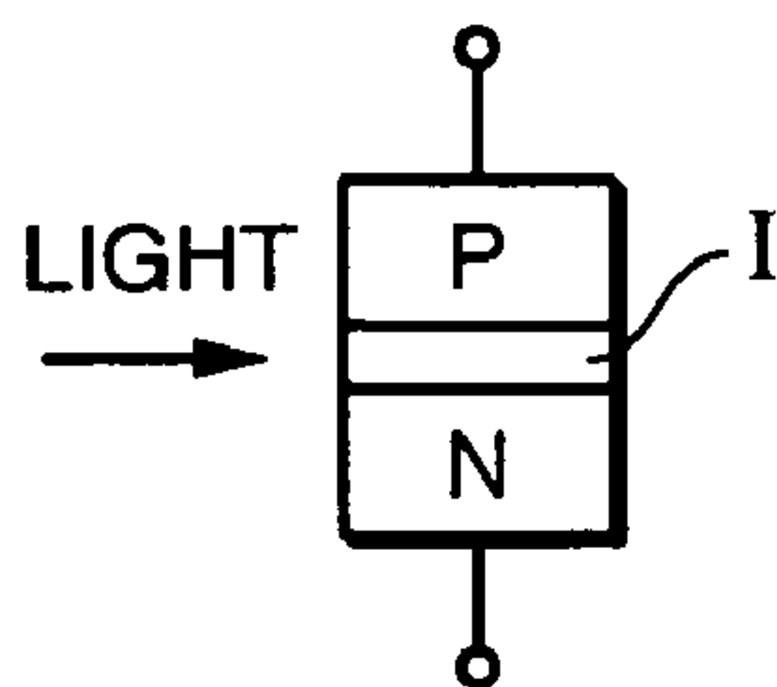
FIG. 25 (PRIOR ART)
