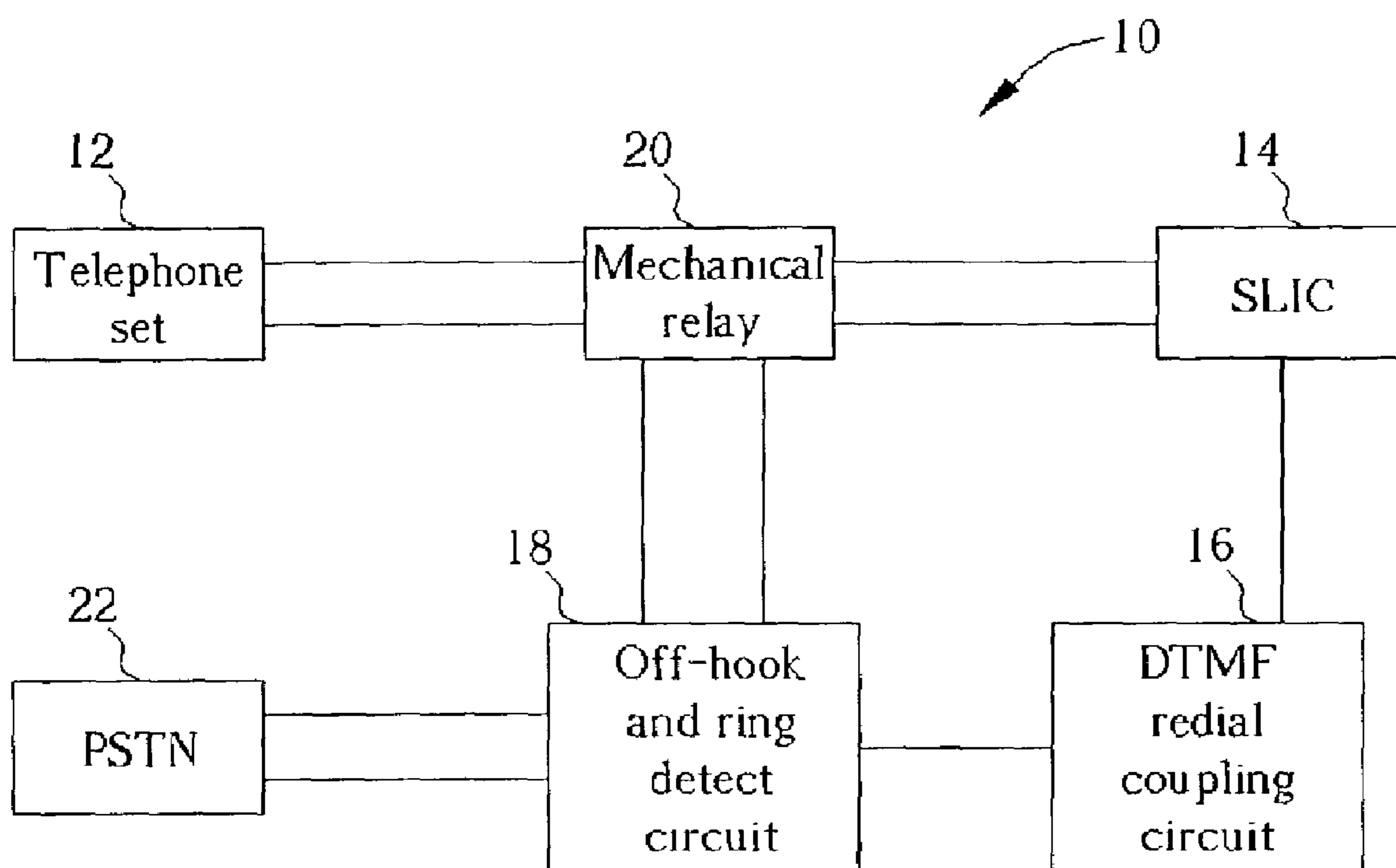
Fig. 1 Prior art
