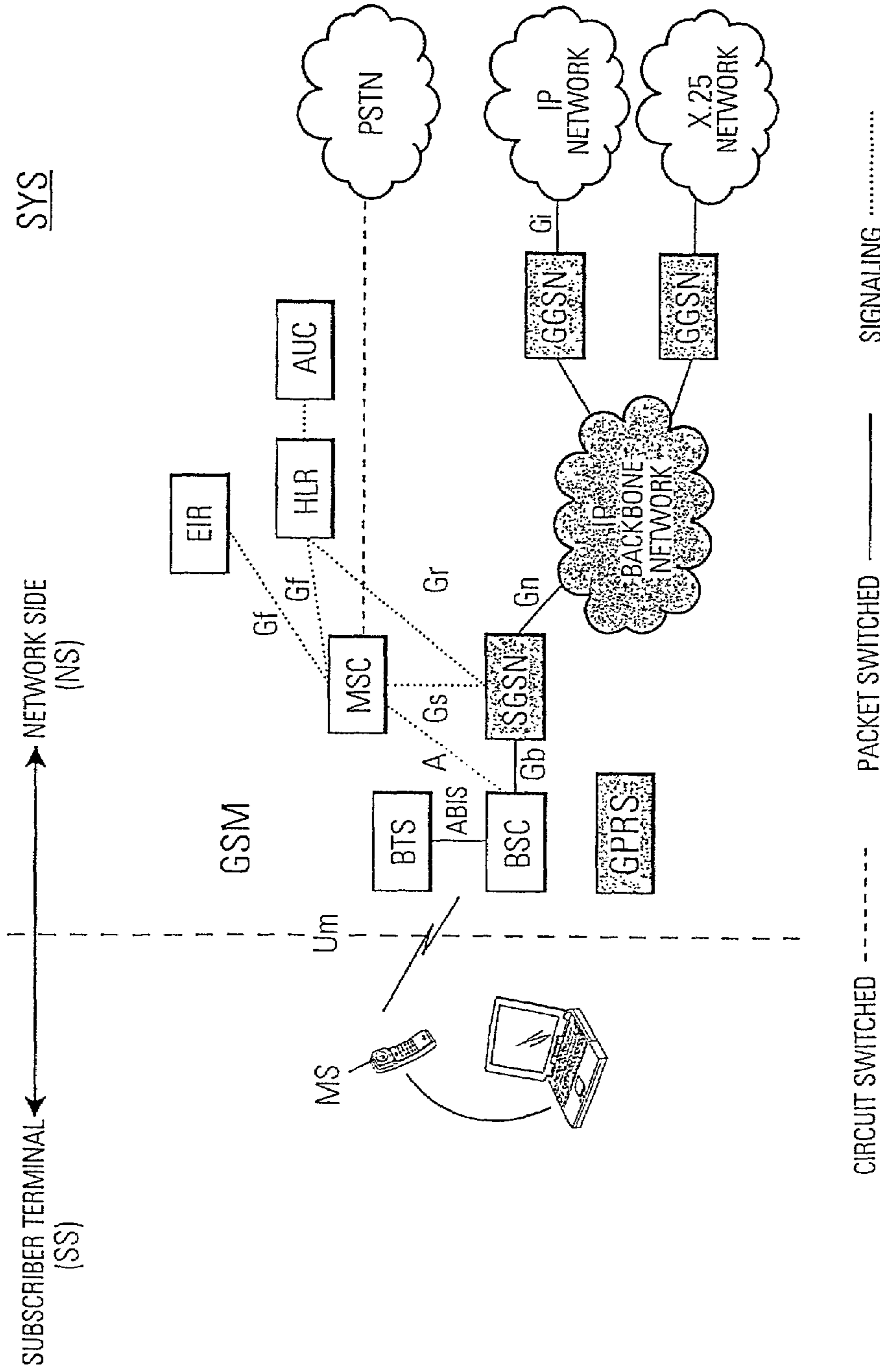
FIG. 1 PRIOR ART GPRS NETWORK ARCHITECTURE
