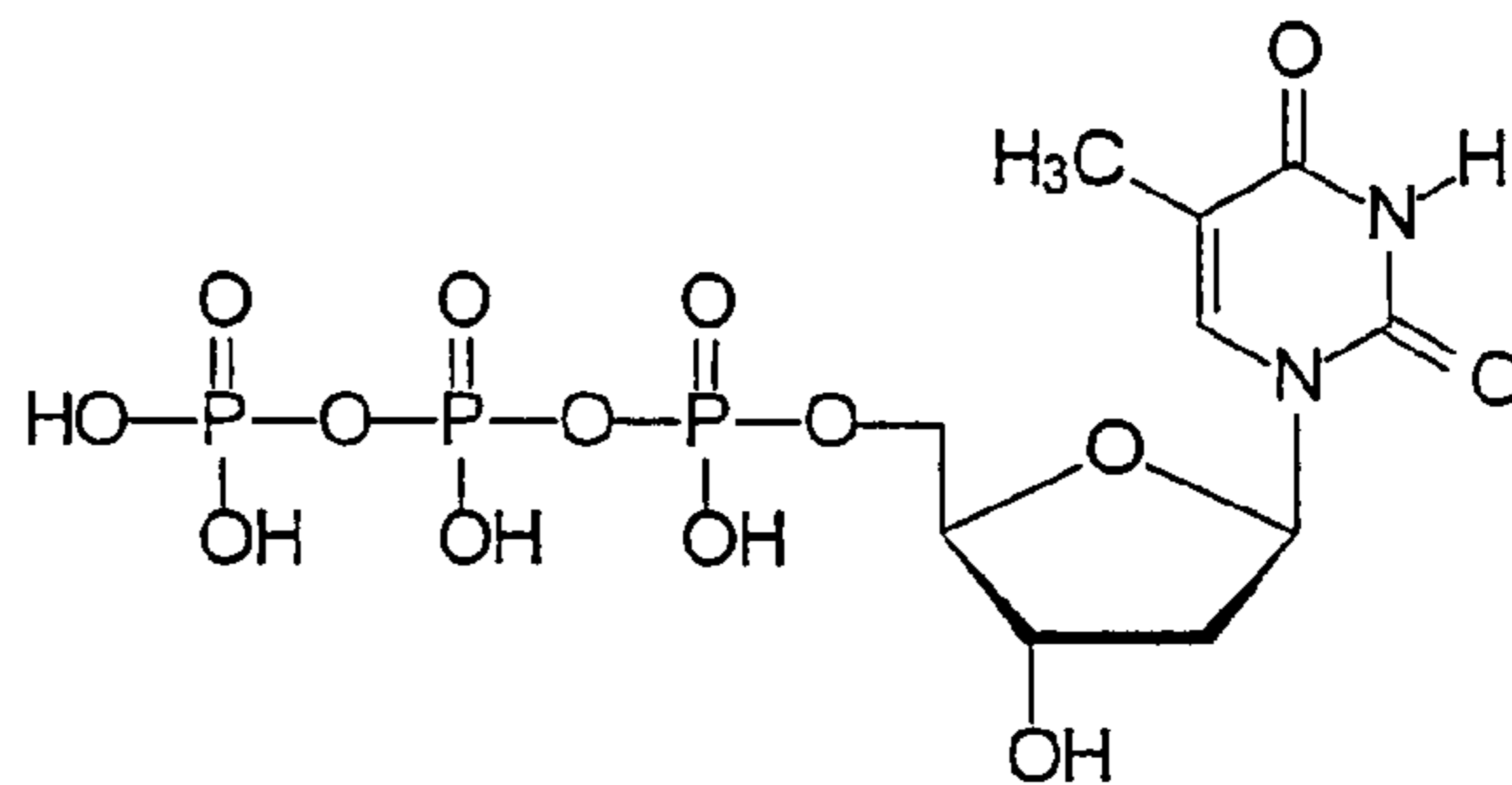
5' Thymidine triphosphate
