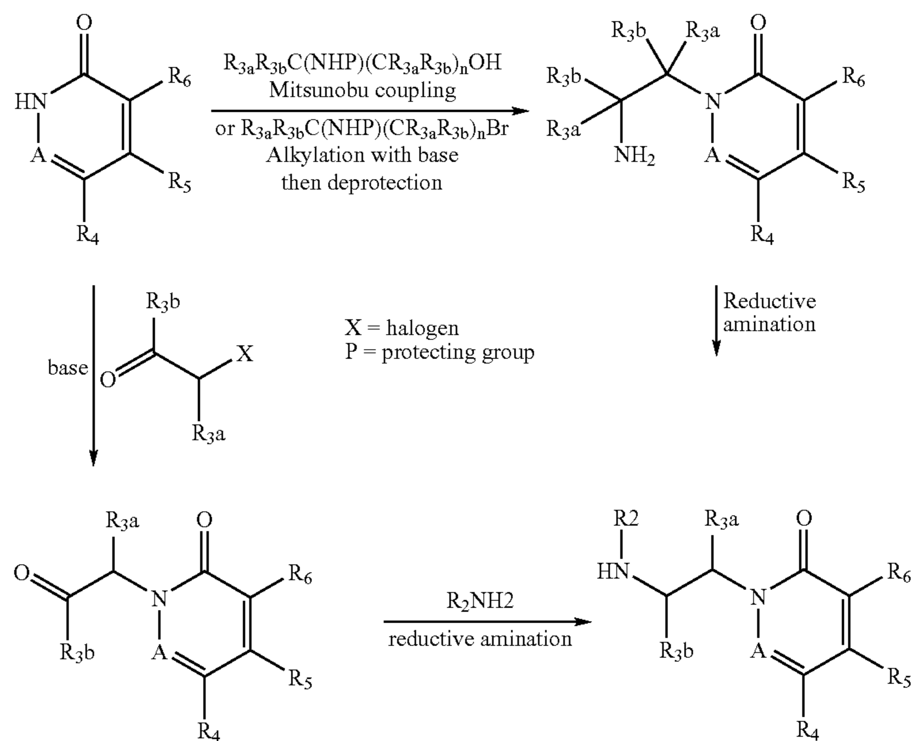
Reaction Scheme C
