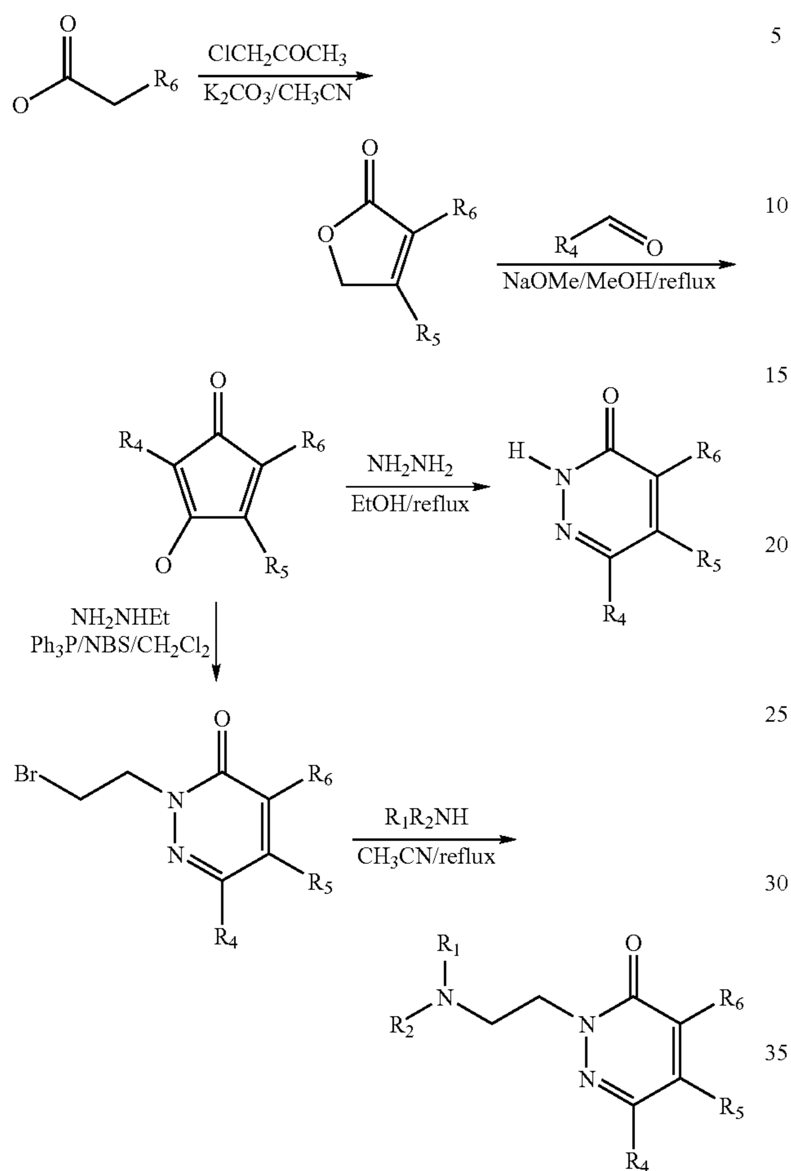
Reaction Scheme A
