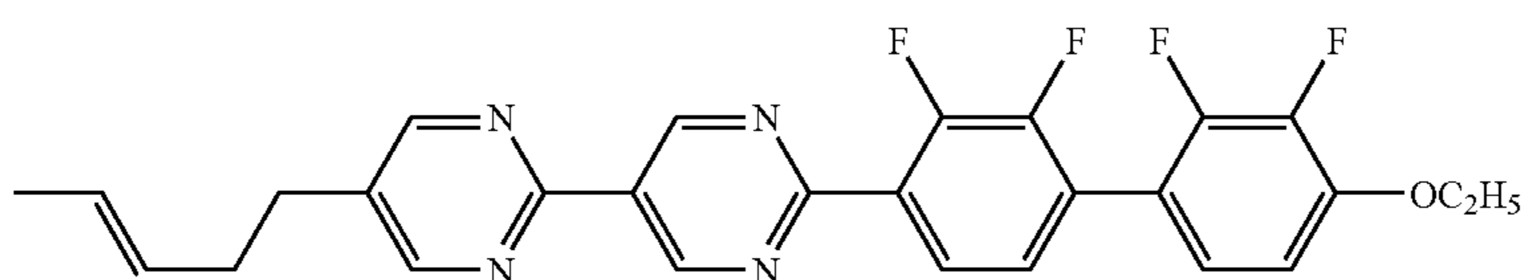
compound NO.283
