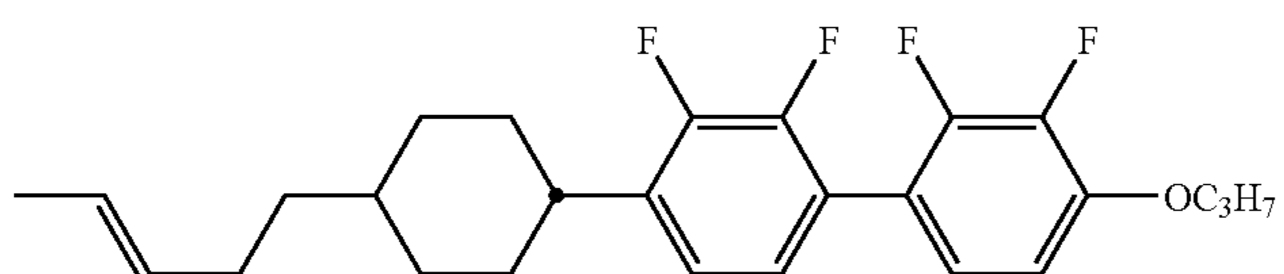
compound NO.99
