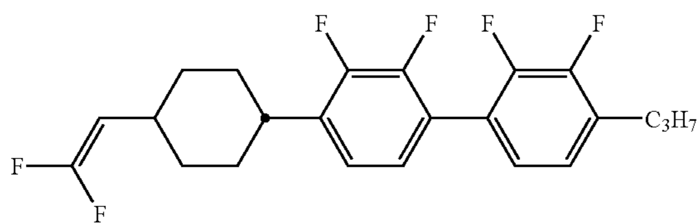
compound NO.311
