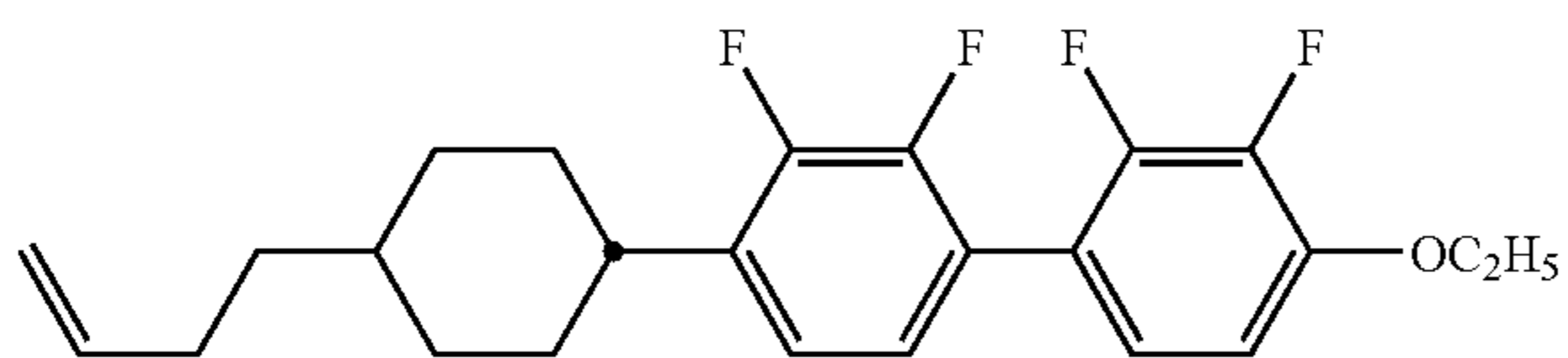
compound NO.95
