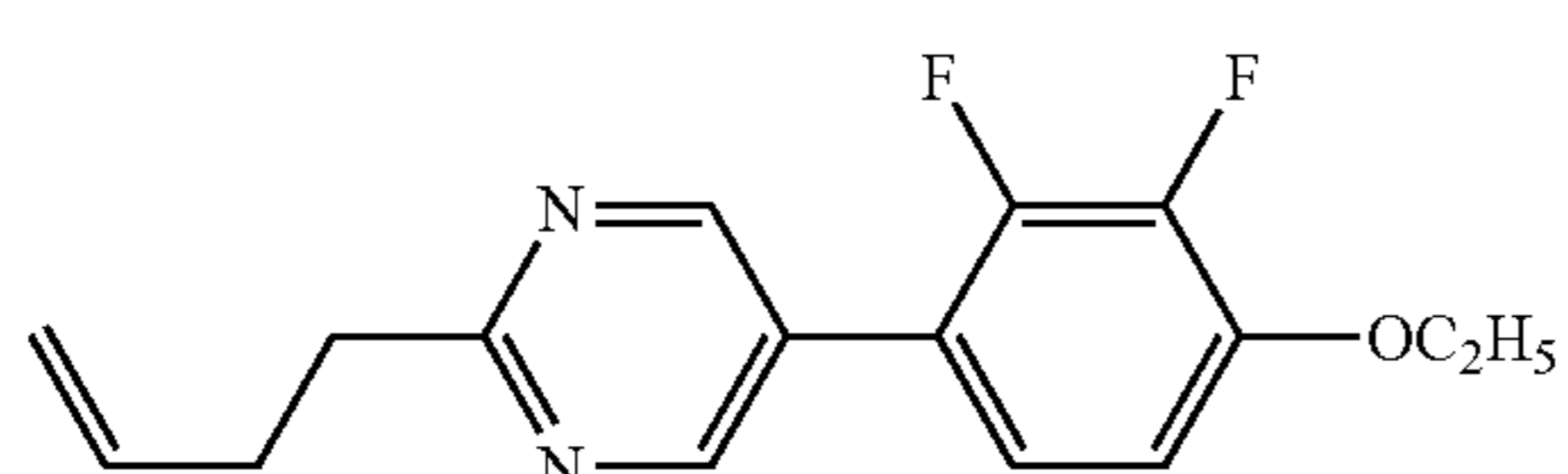
compound NO.242
