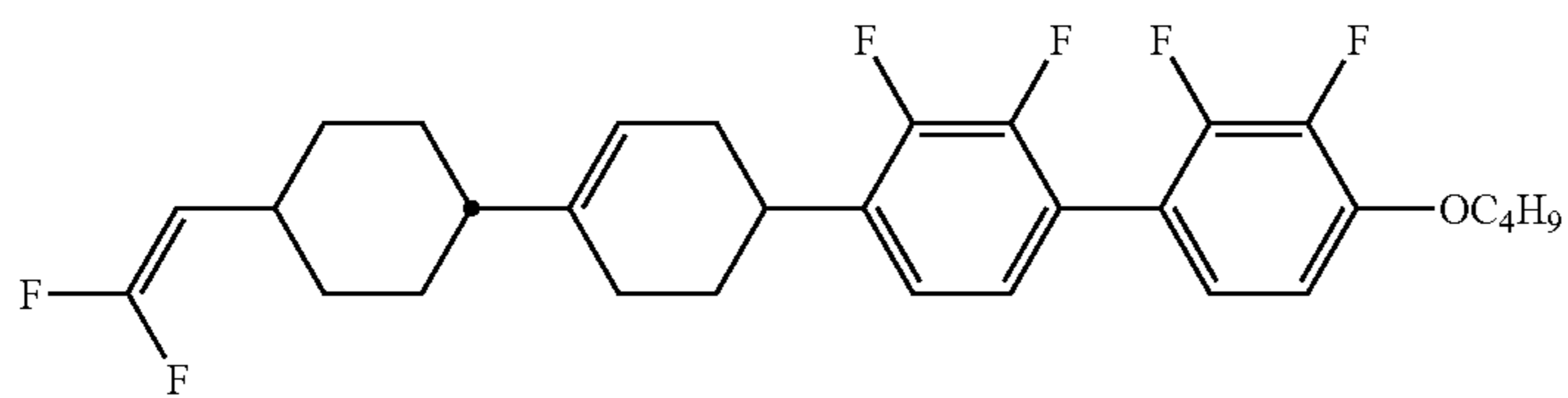
compound NO.313
