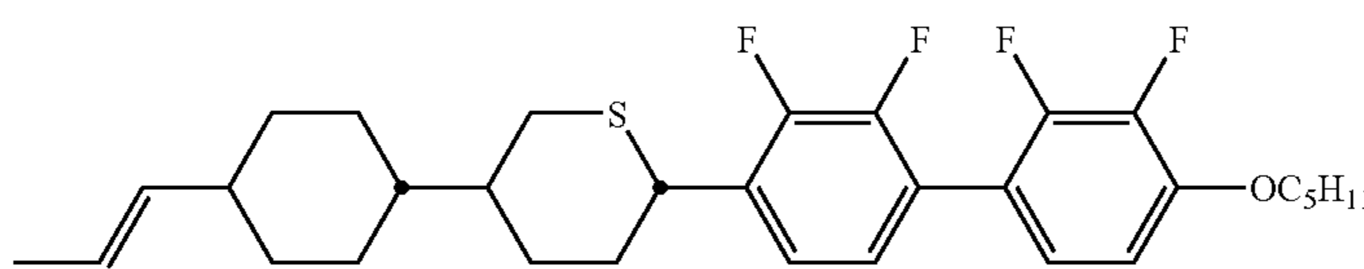
compound NO.228
