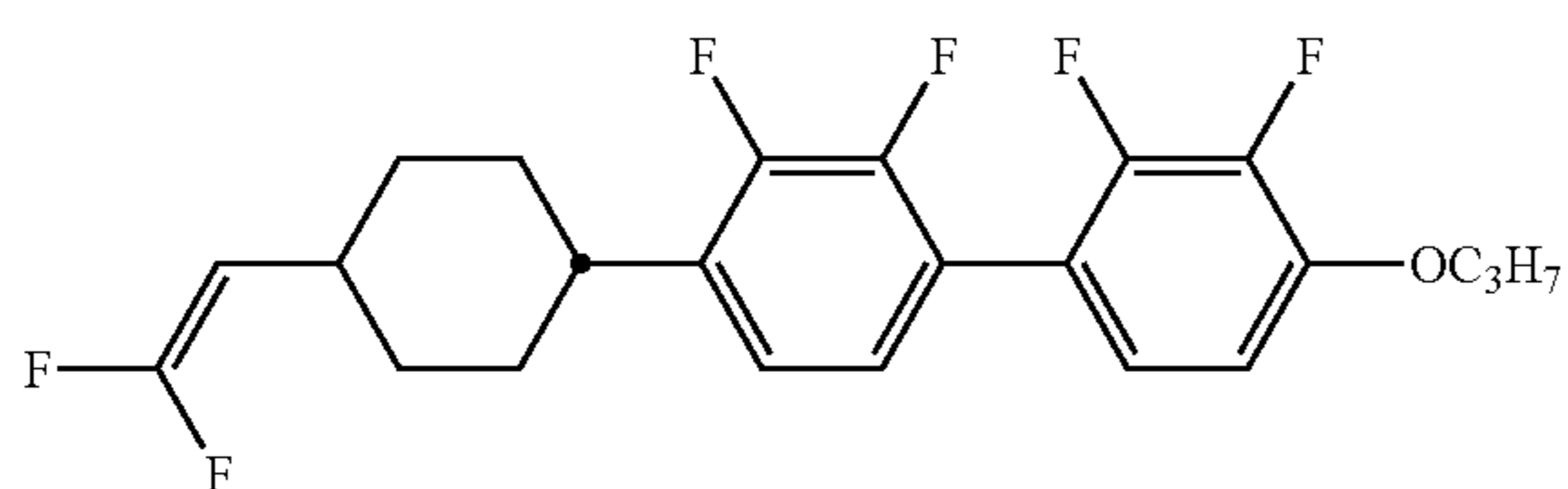
compound NO.310
