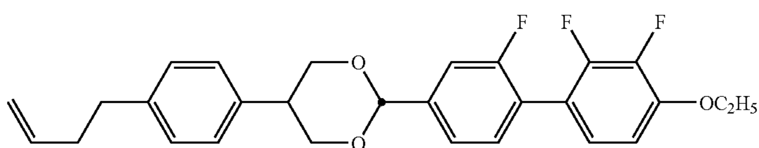
compound NO.286
