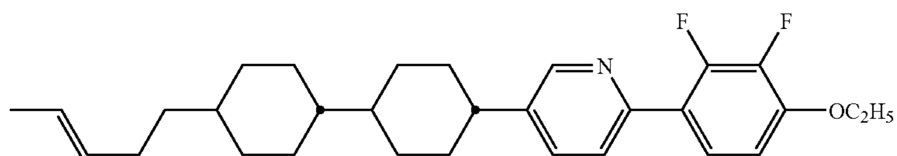
compound NO.259
