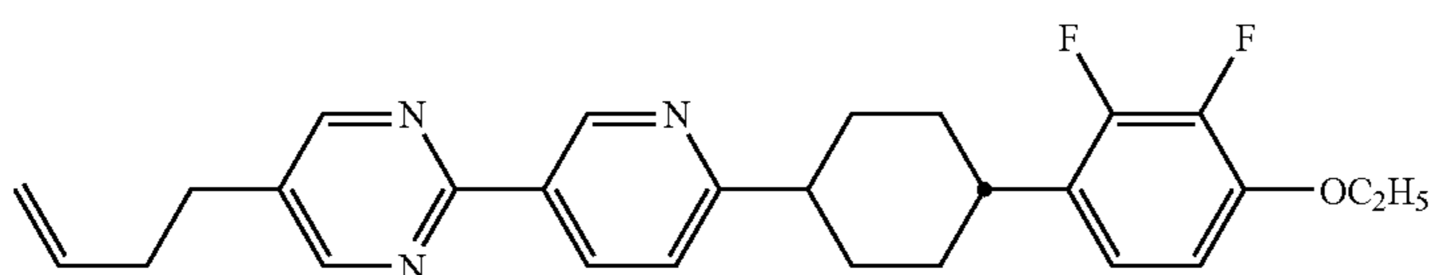
compound NO.282
