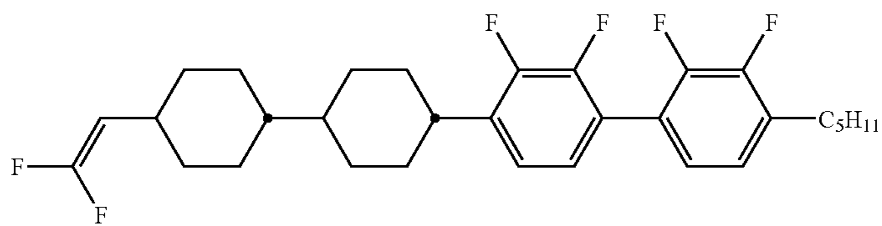
compound NO.314
