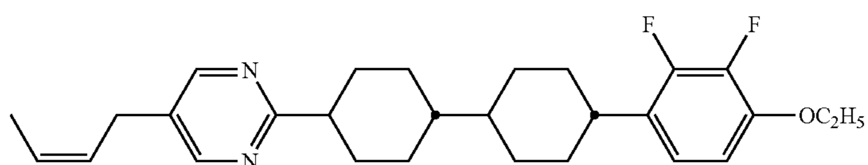
compound NO.257
