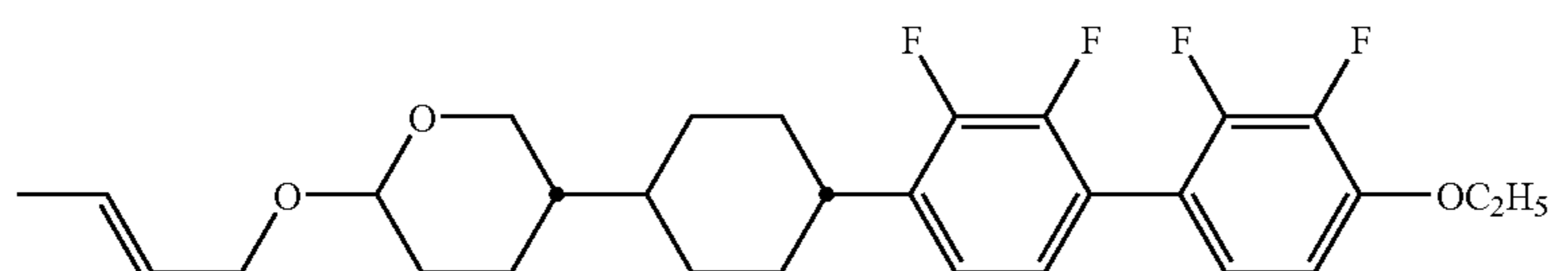
compound NO.186
