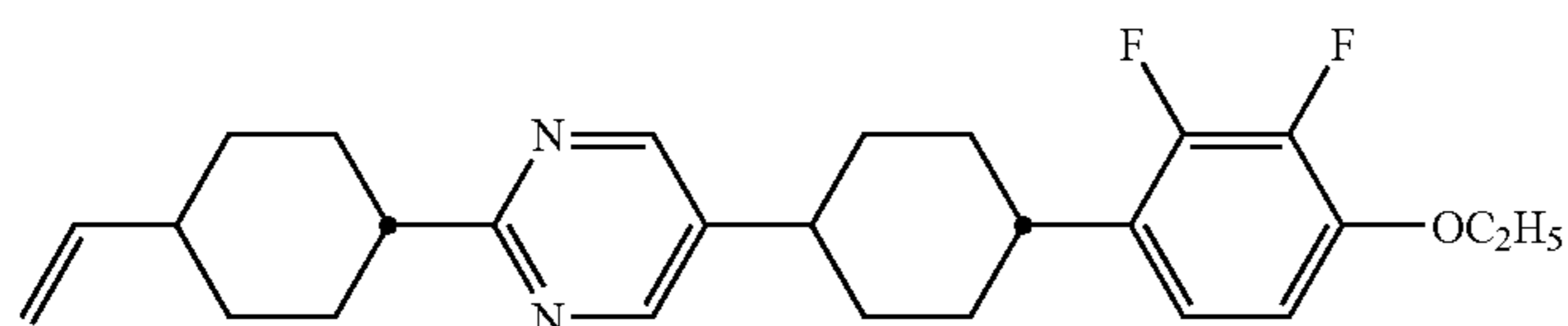
compound NO.256
