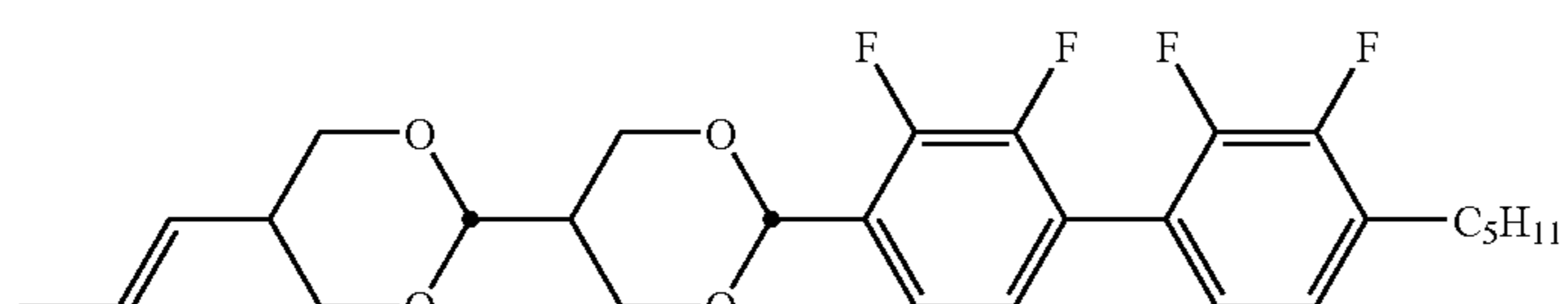
compound NO.191
