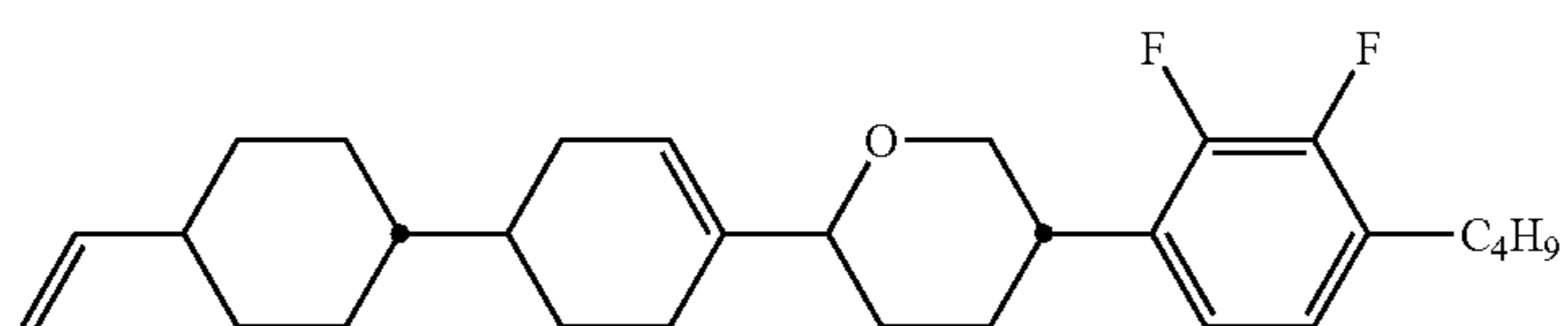
compound NO.170
