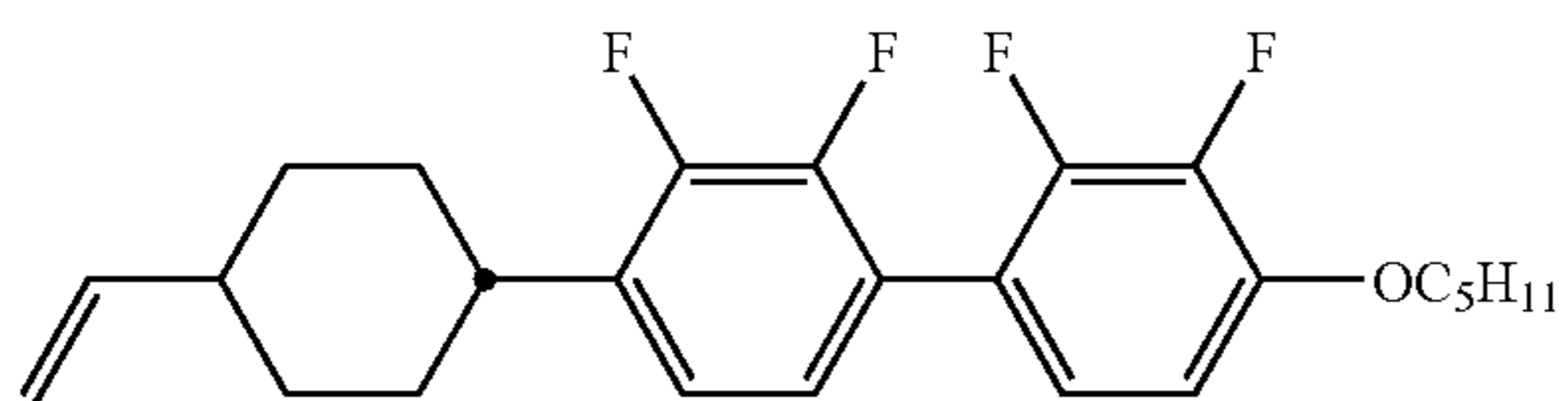
compound NO.101
