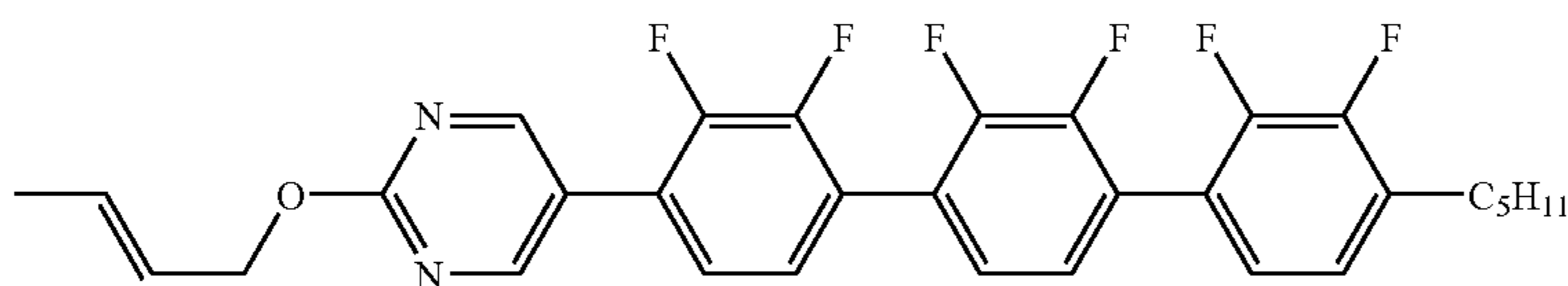
compound NO.278
