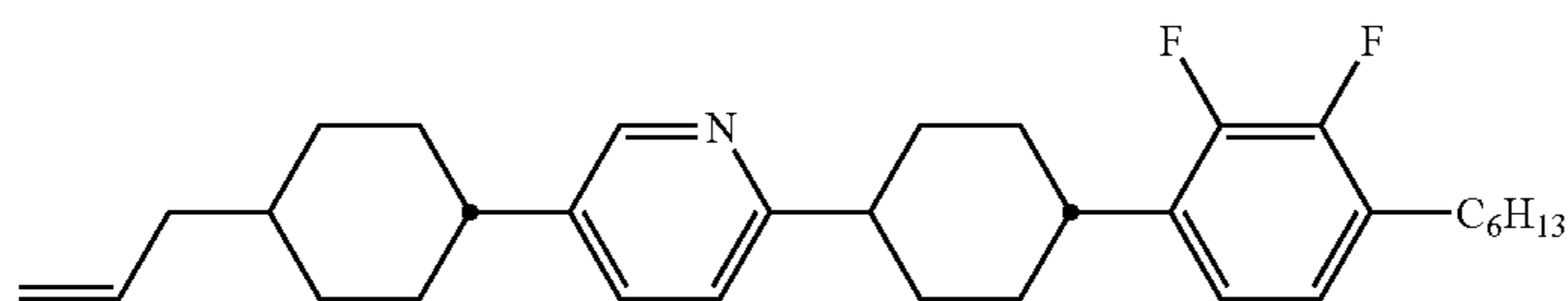
compound NO.261
