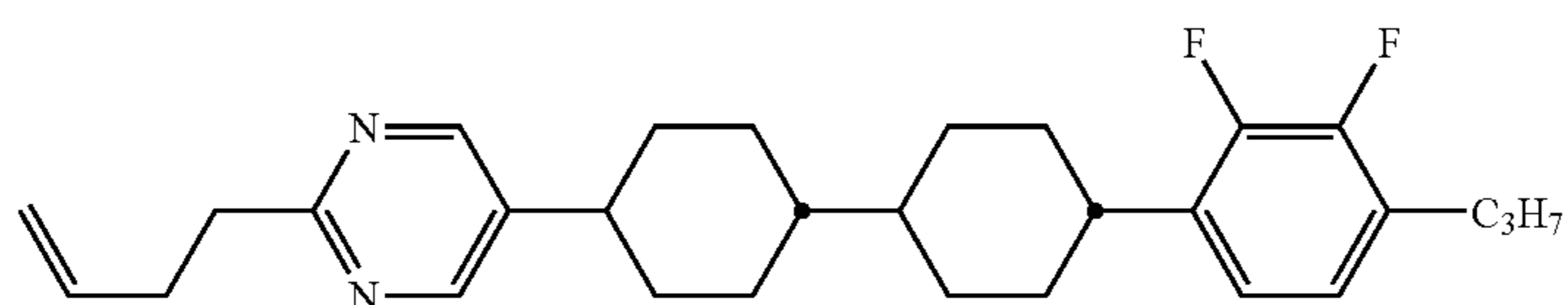
compound NO.258
