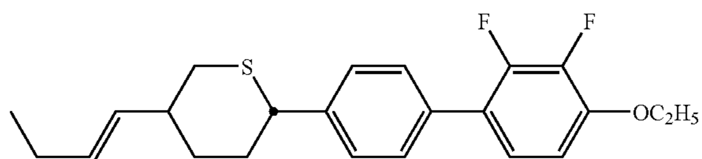
compound NO.206
