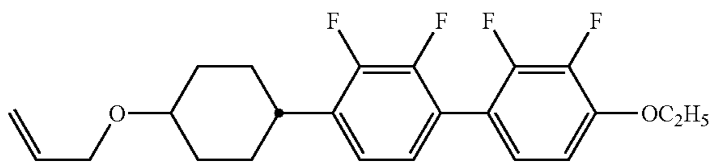
compound NO.104
