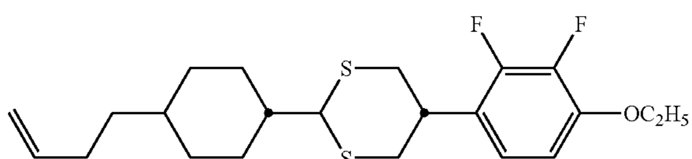
compound NO.201
