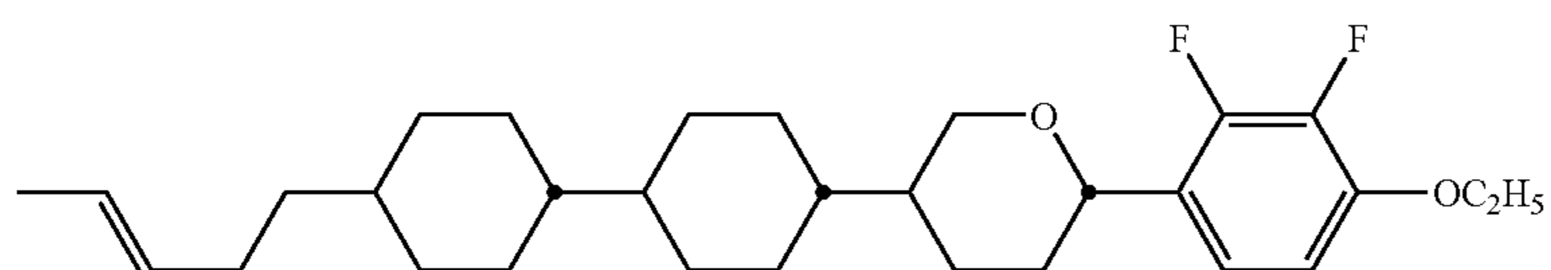
compound NO.169
