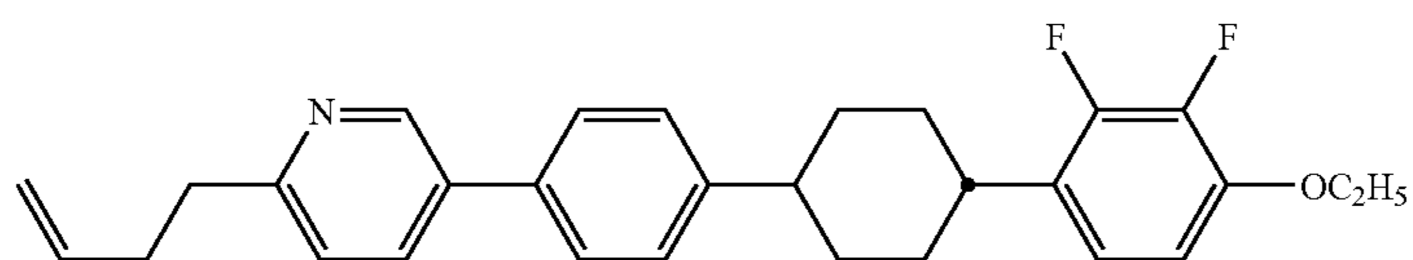
compound NO.264
