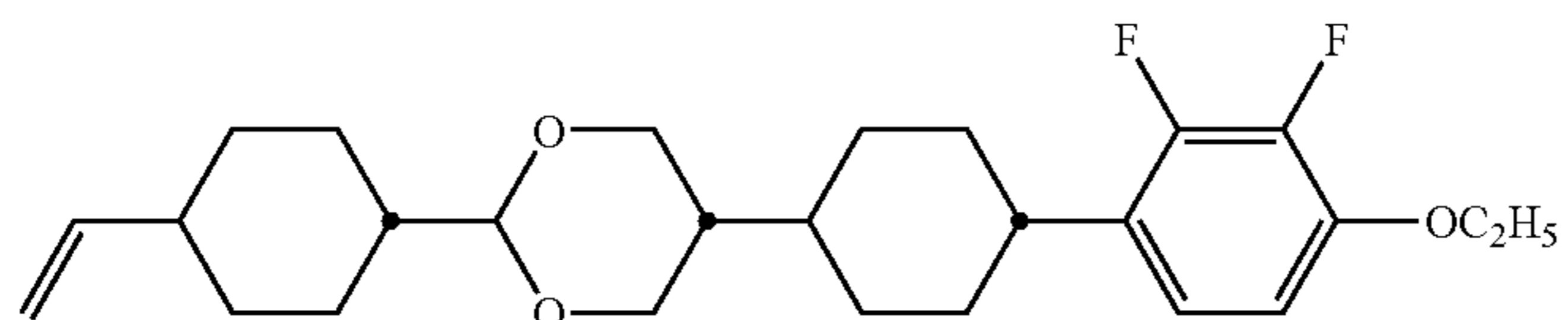
compound NO.166
