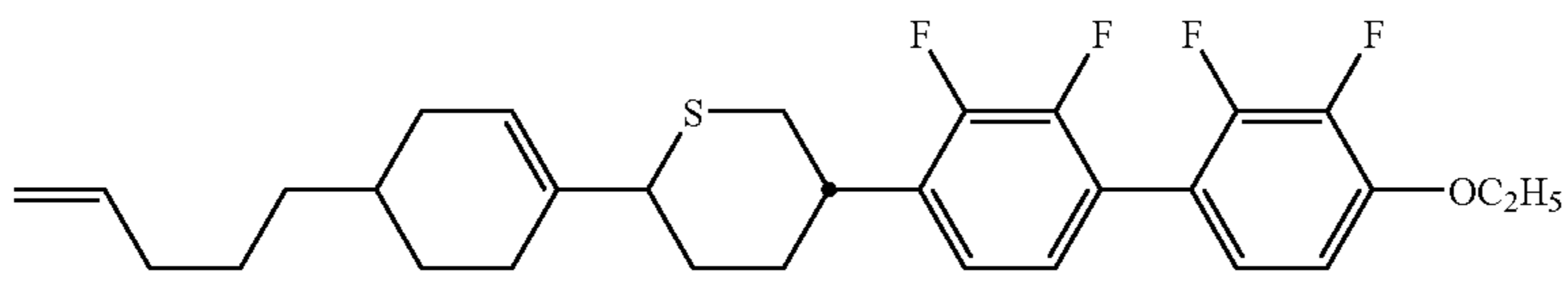
compound NO.229
