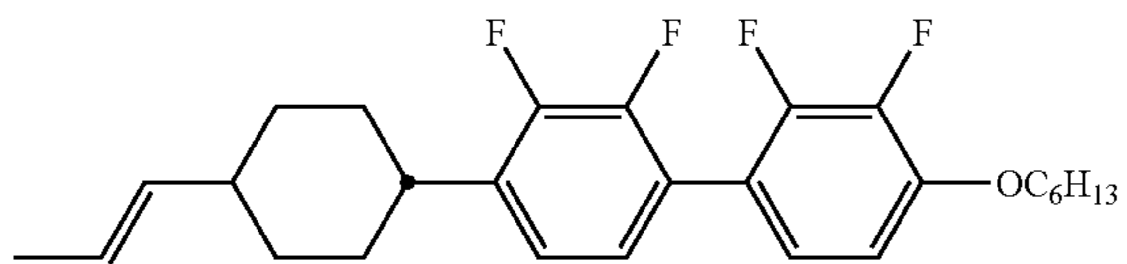
compound NO.102
