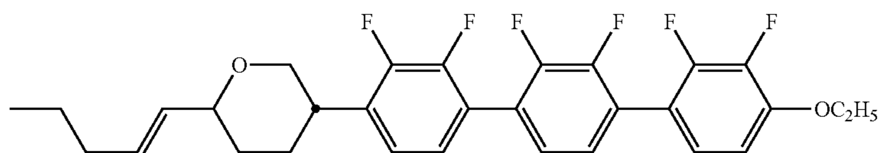
compound NO.190
