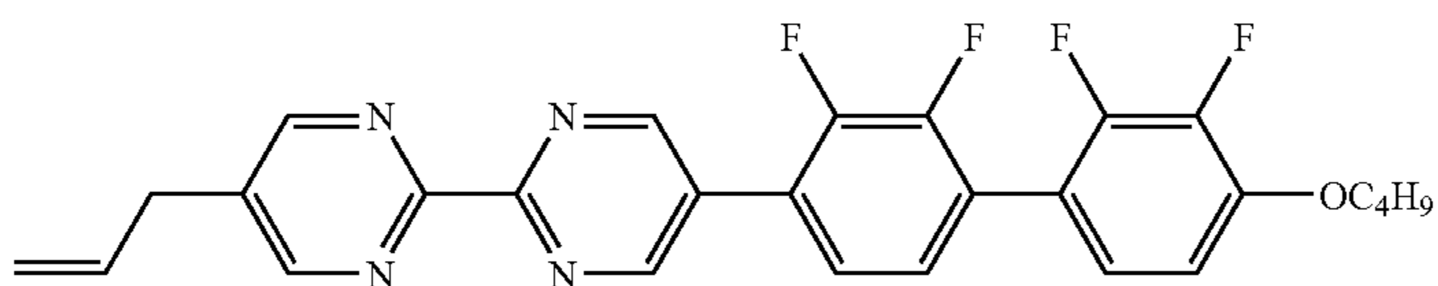
compound NO.281
