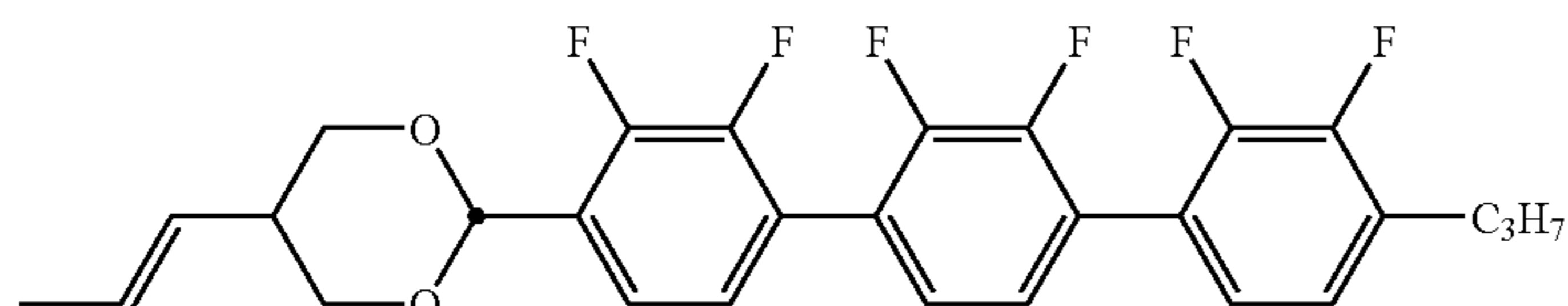
compound NO.187
