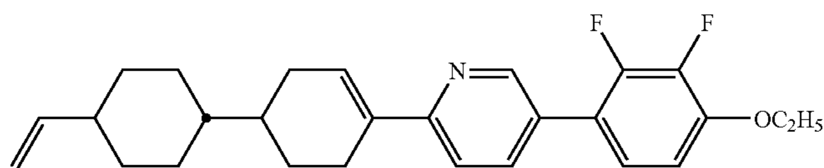
compound NO.260
