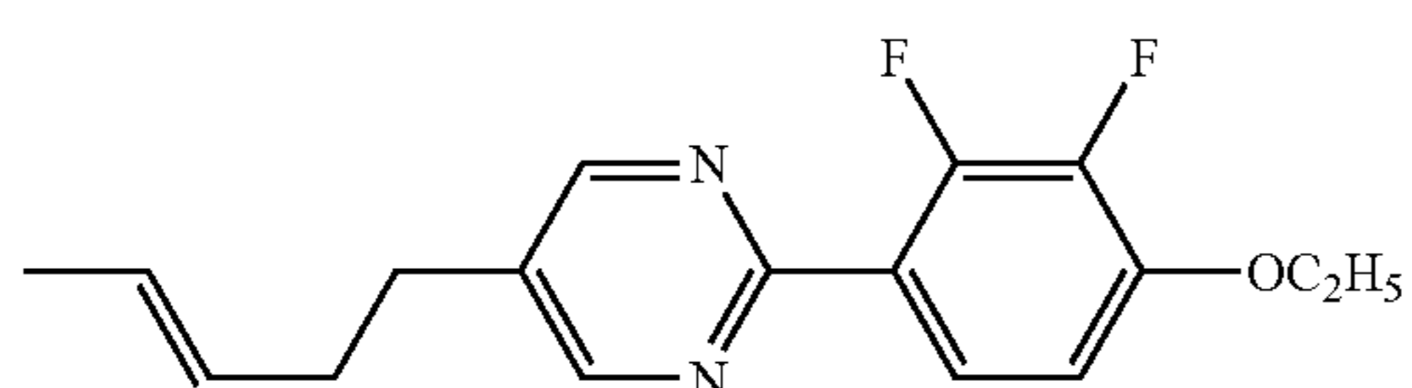
compound NO.241
