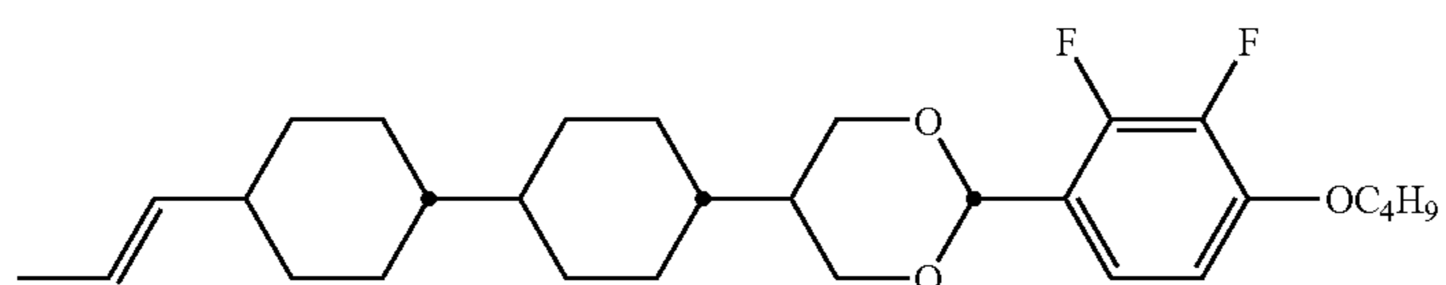
compound NO.163
