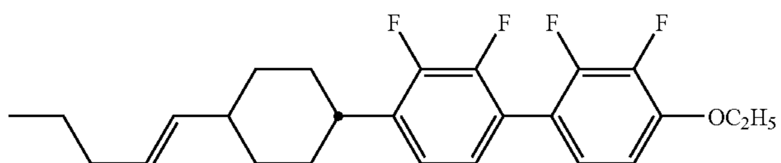
compound NO.96
