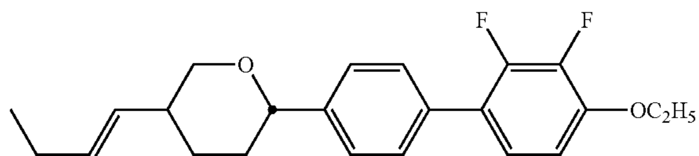
compound NO.161
