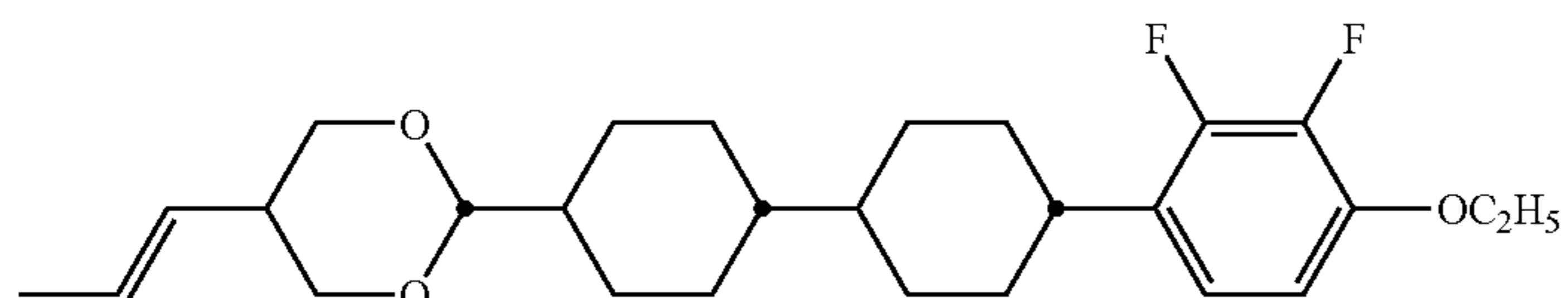
compound NO.167
