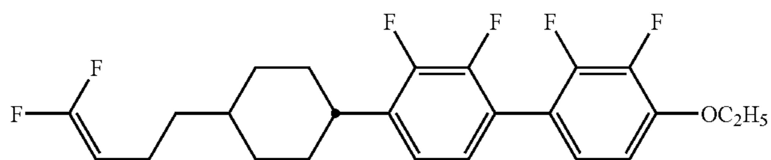
compound NO.312
