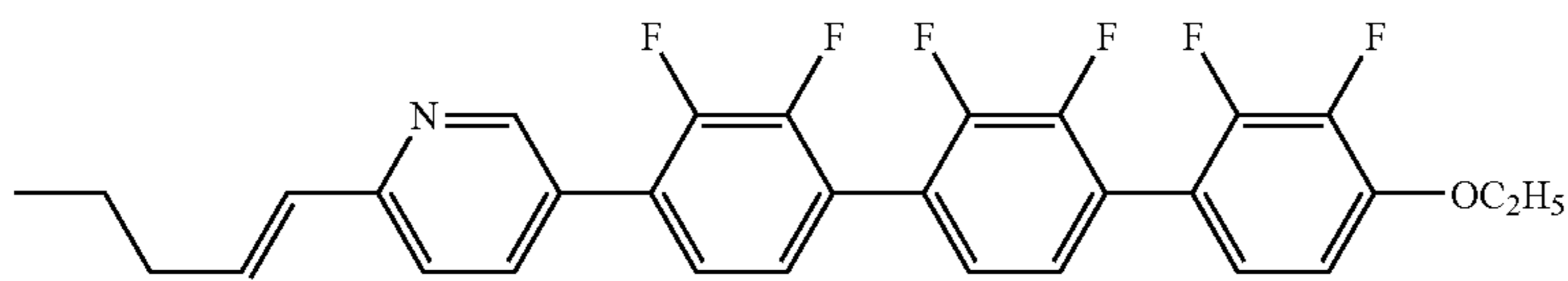
compound NO.280
