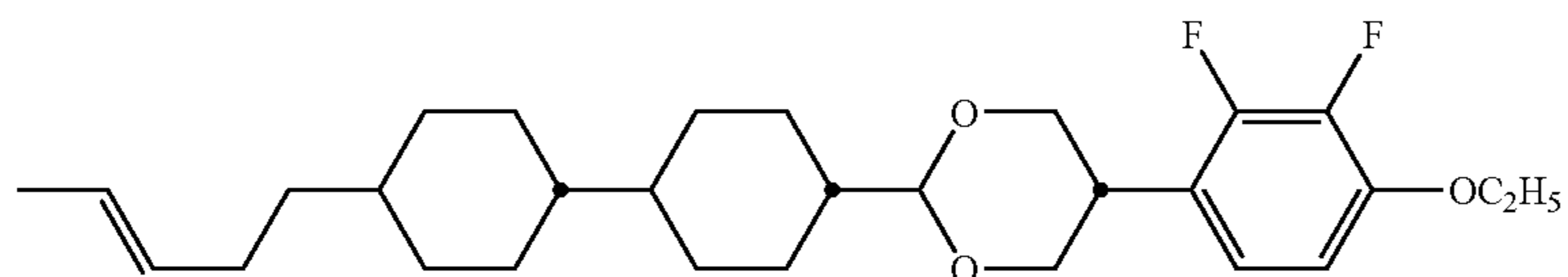
compound NO.164
