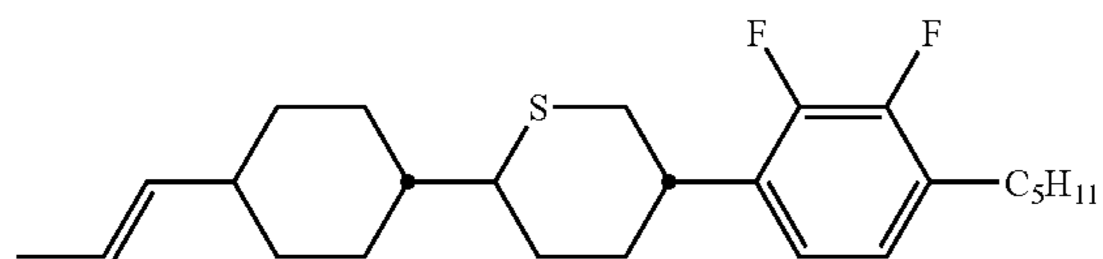
compound NO.205
