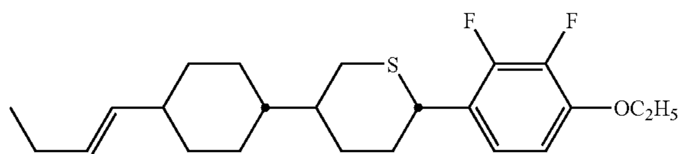
compound NO.204
