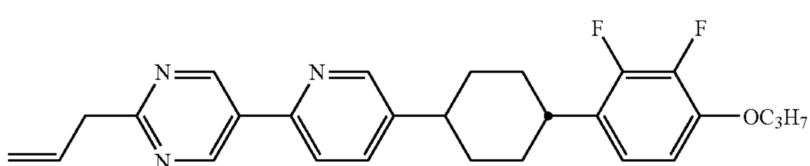
compound NO.284
