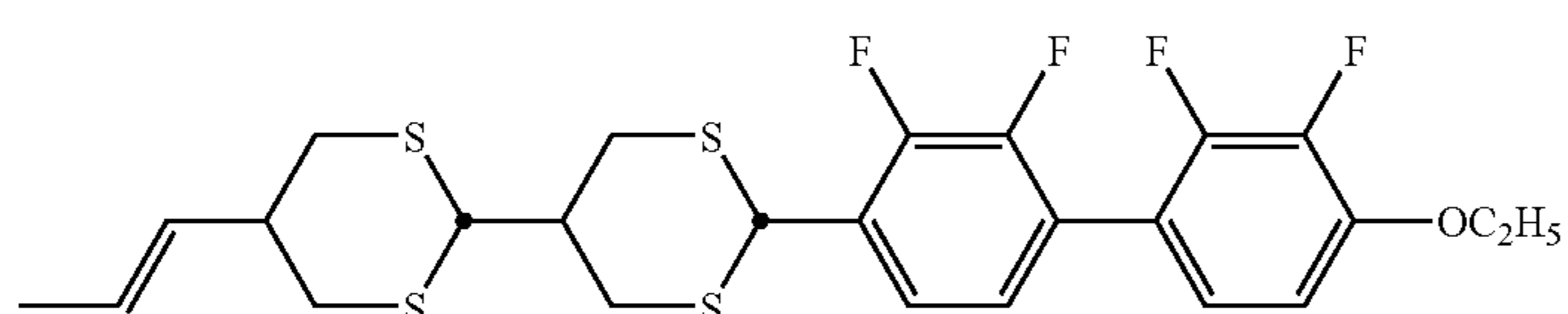
compound NO.236
