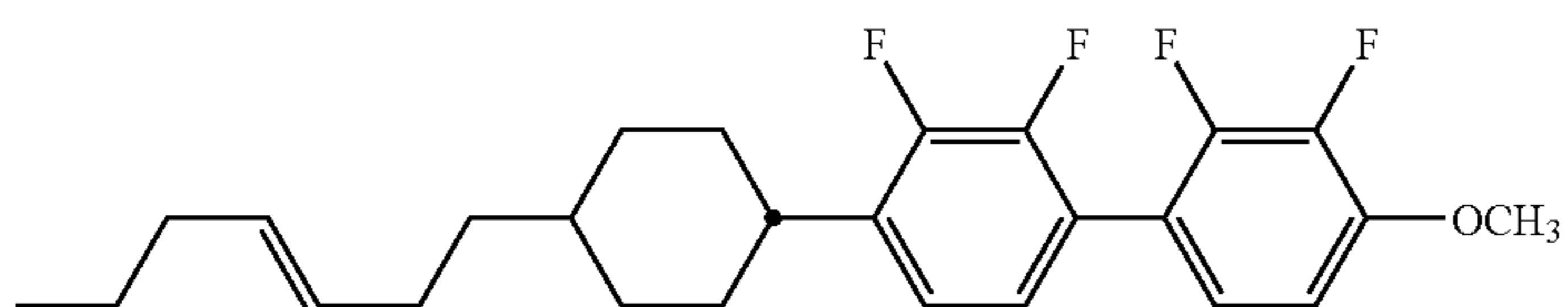
compound NO.105
