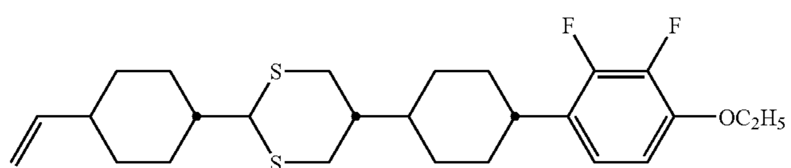
compound NO.211
