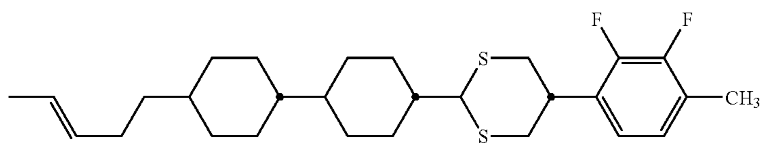
compound NO.209
