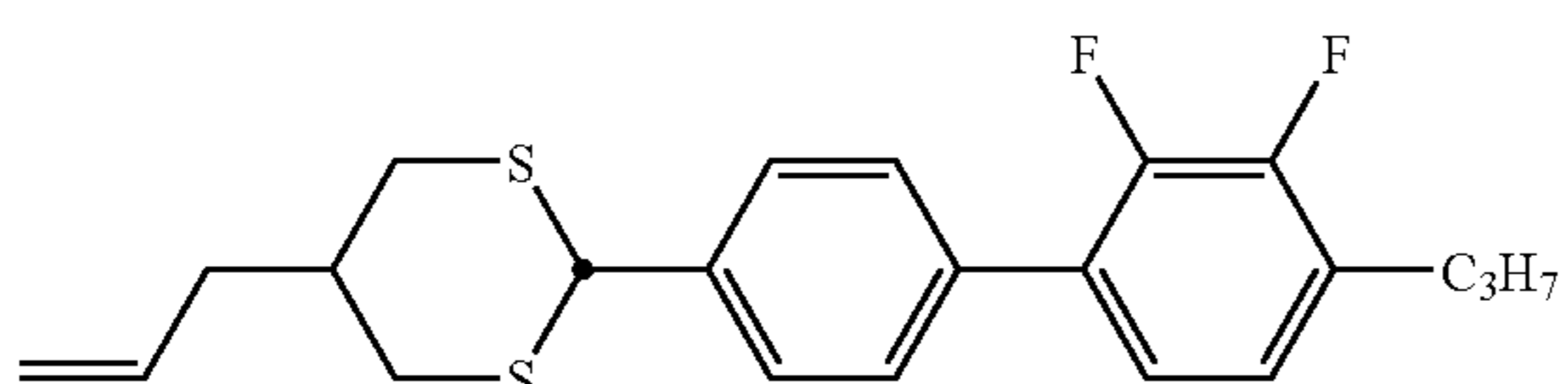
compound NO.202
