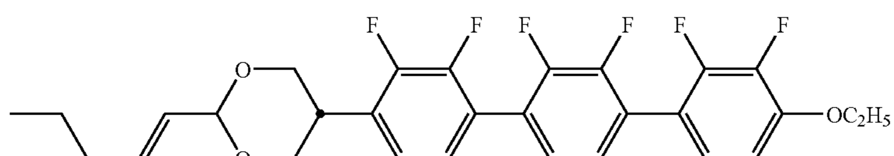
compound NO.188
