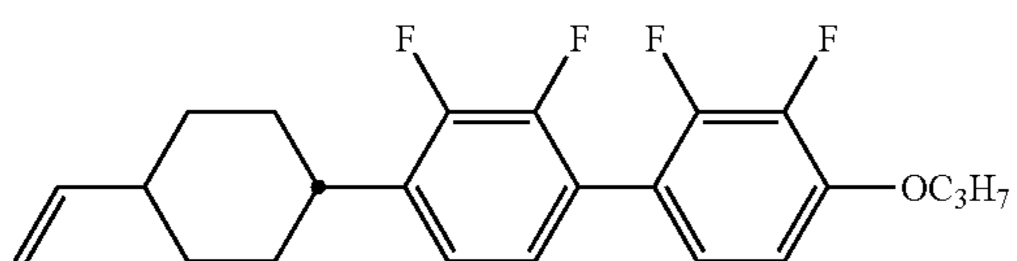
compound NO.97
