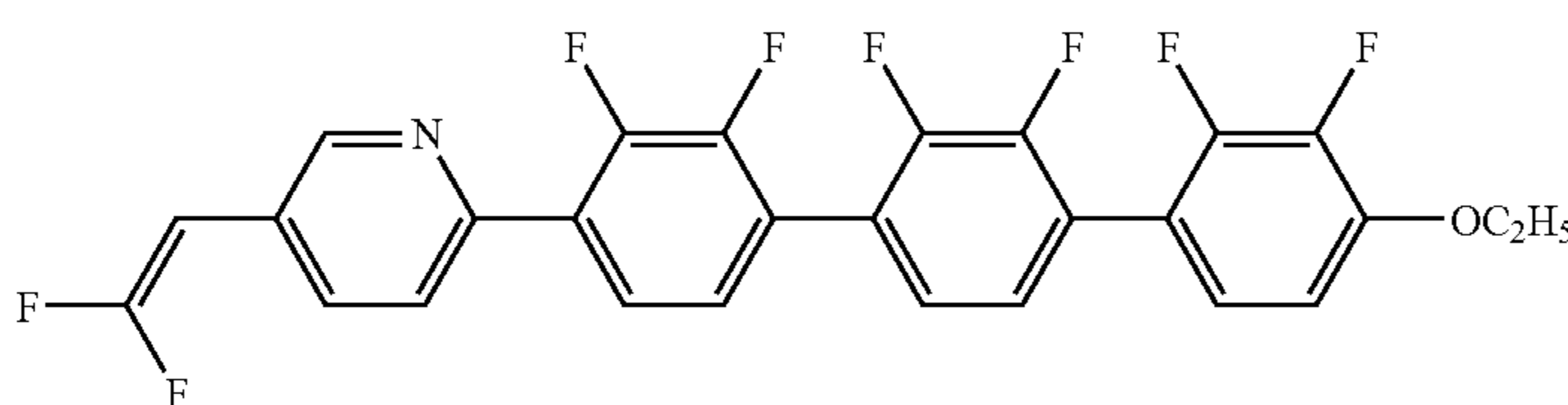
compound NO.279
