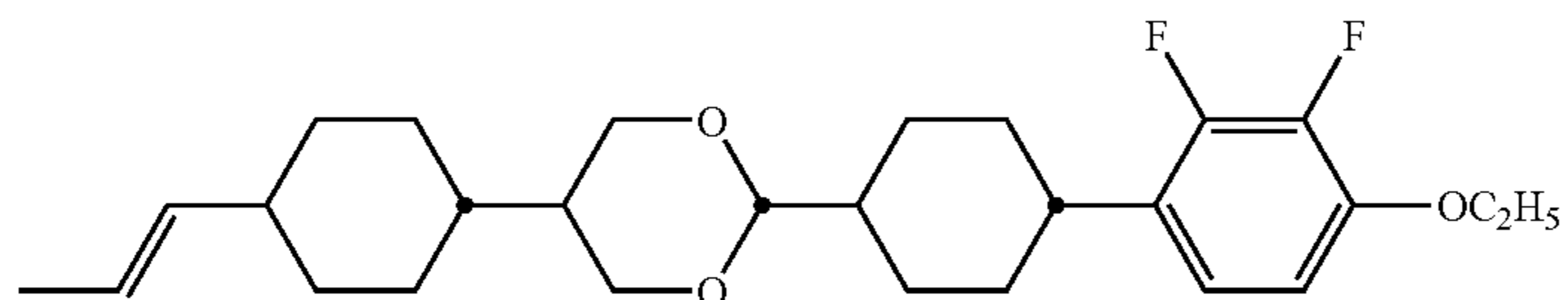
compound NO.165
