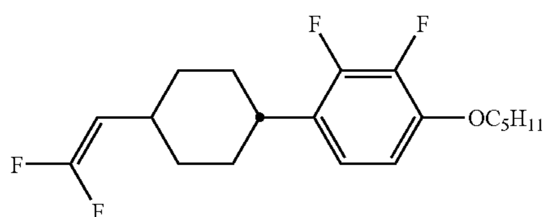
compound NO.303
