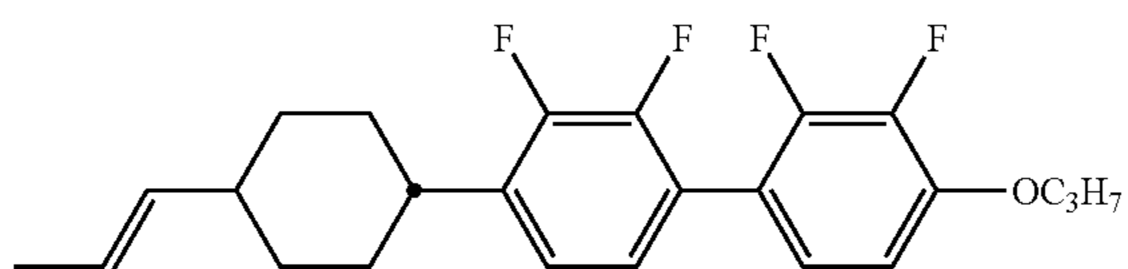
compound NO.98
