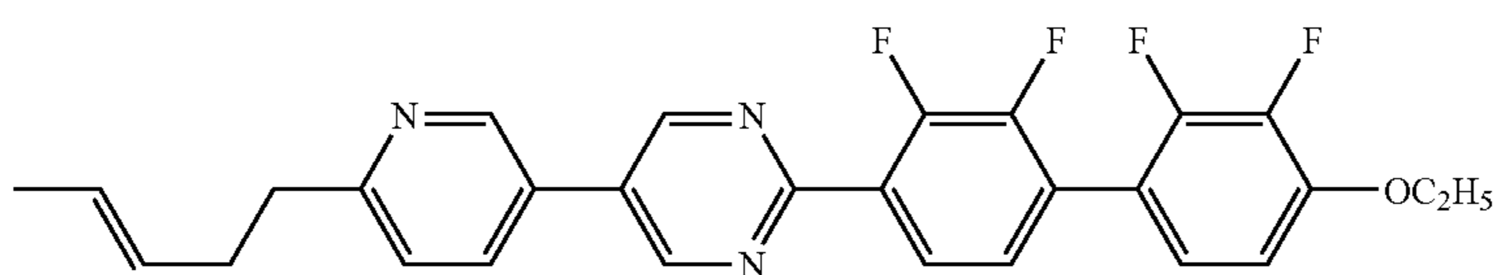
compound NO.285
