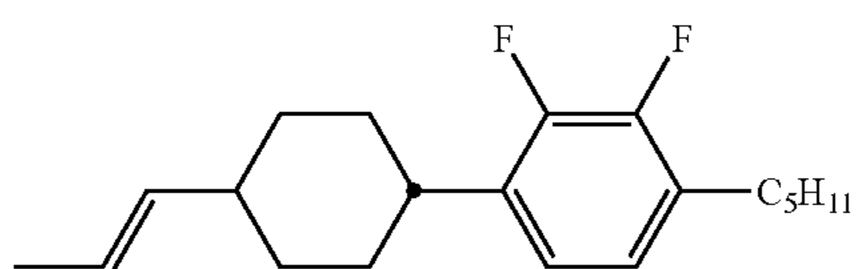
compound NO.20
