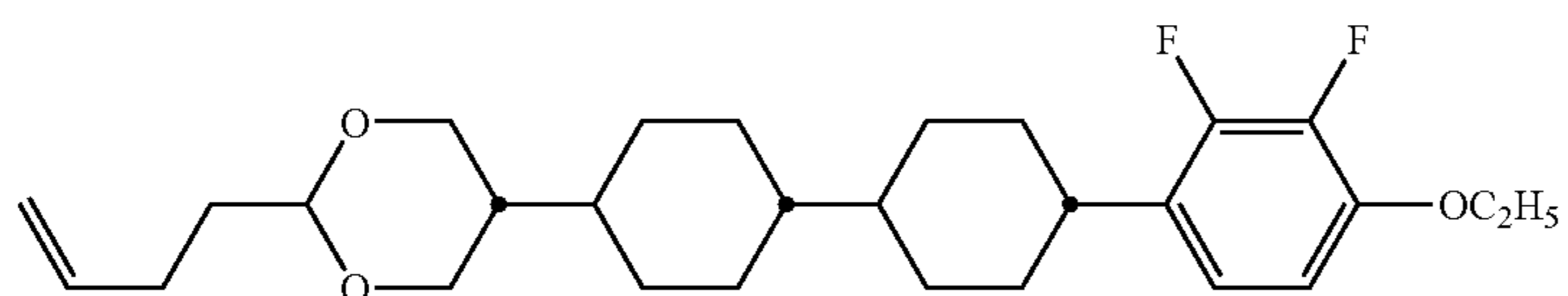
compound NO.168
