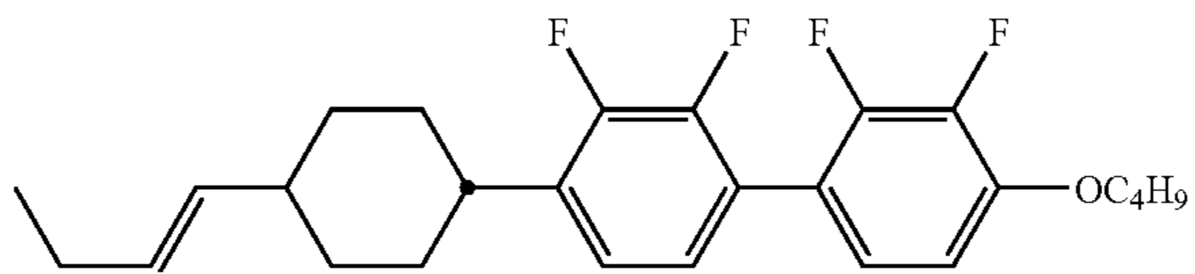
compound NO.100
