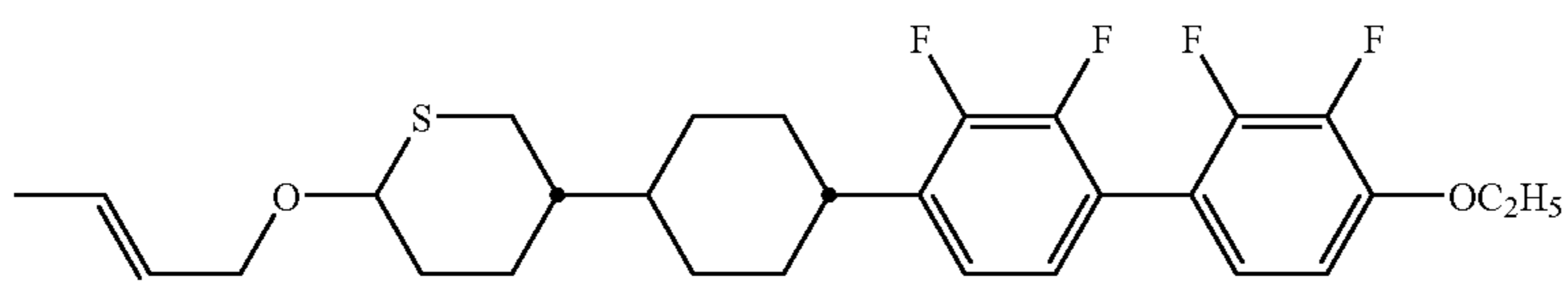
compound NO.231
