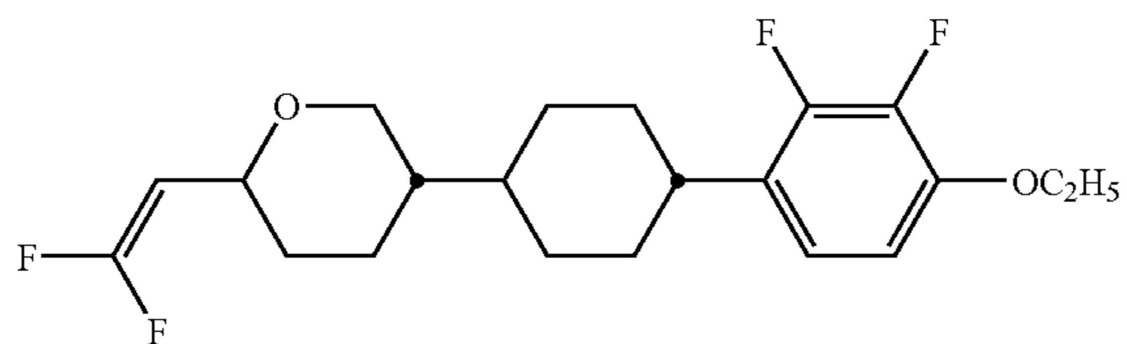
compound NO.162
