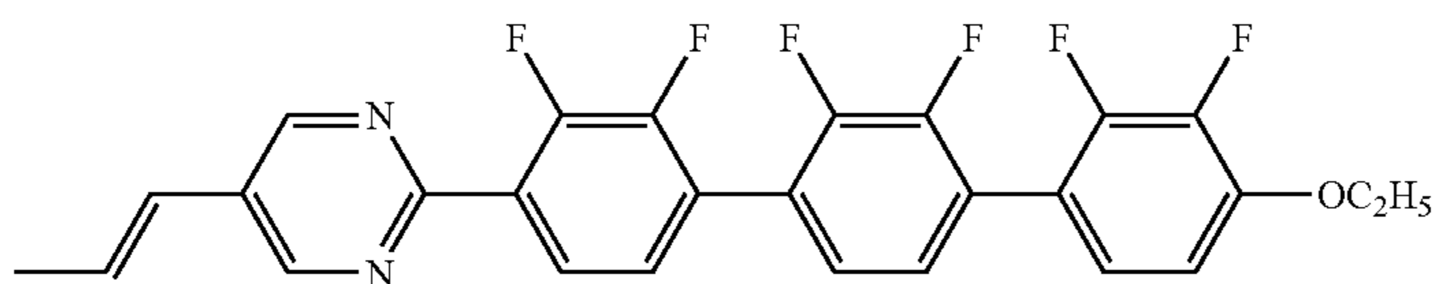
compound NO.277
