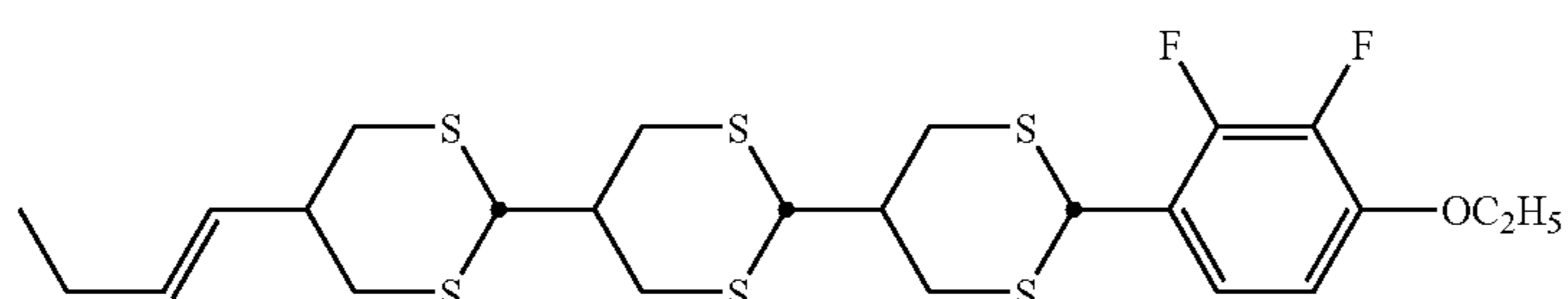
compound NO.239
