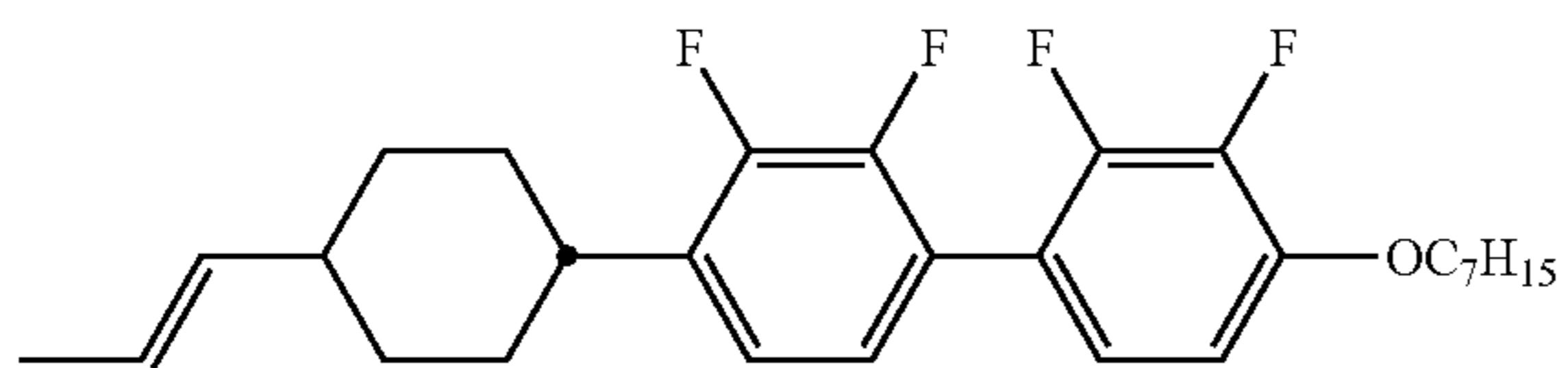
compound NO.103
