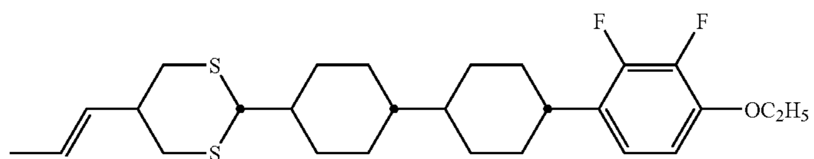
compound NO.212
