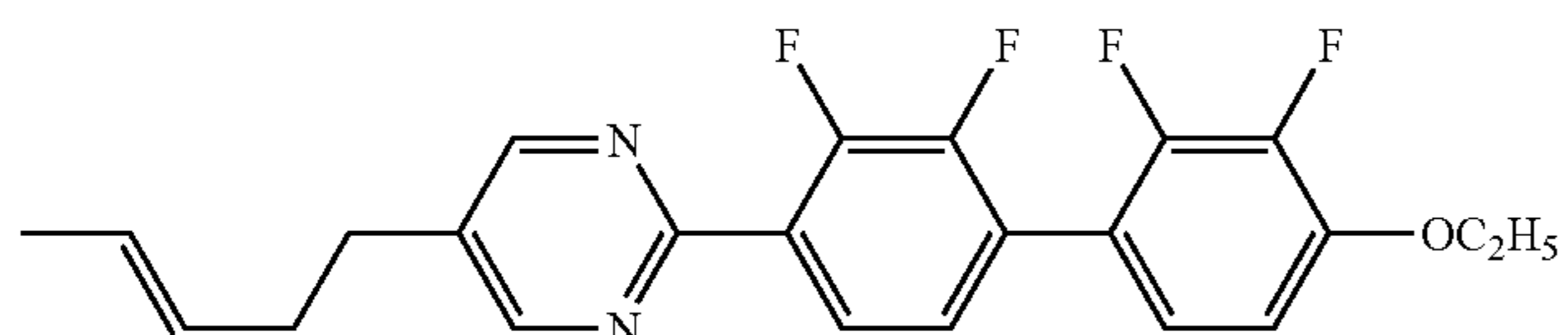
compound NO.265
