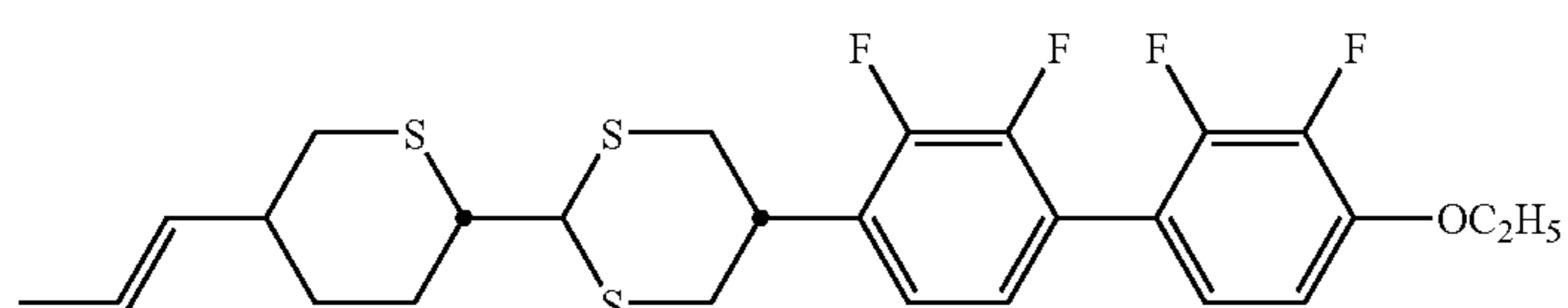
compound NO.240
