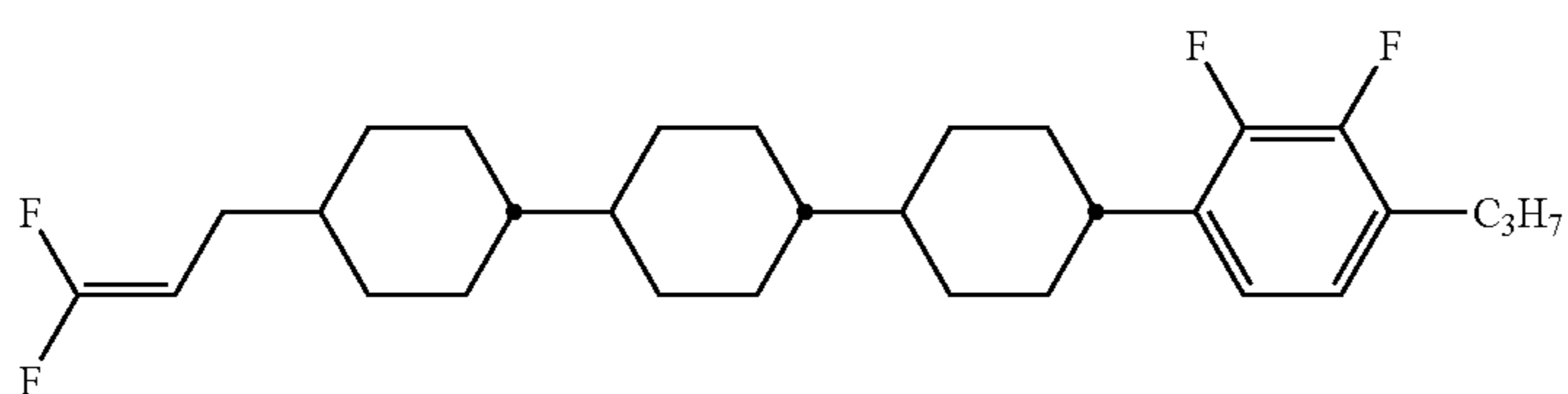
compound NO.308
