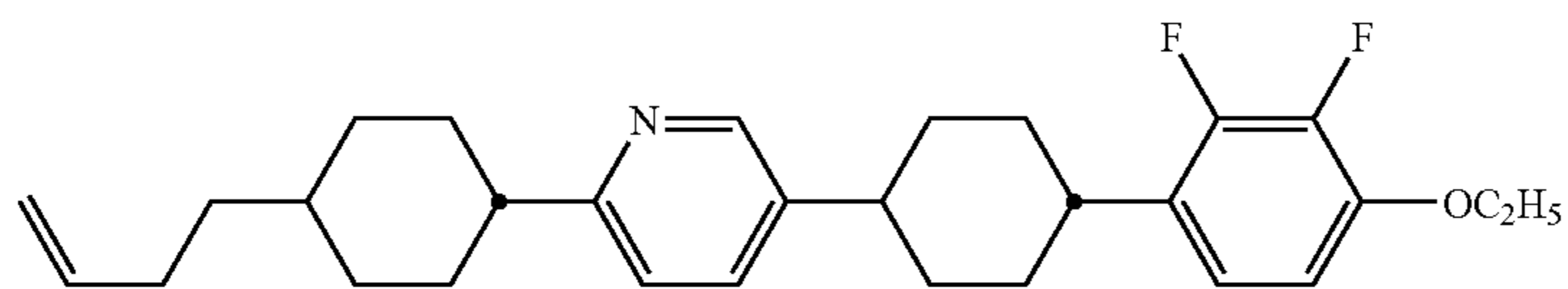
compound NO.262
