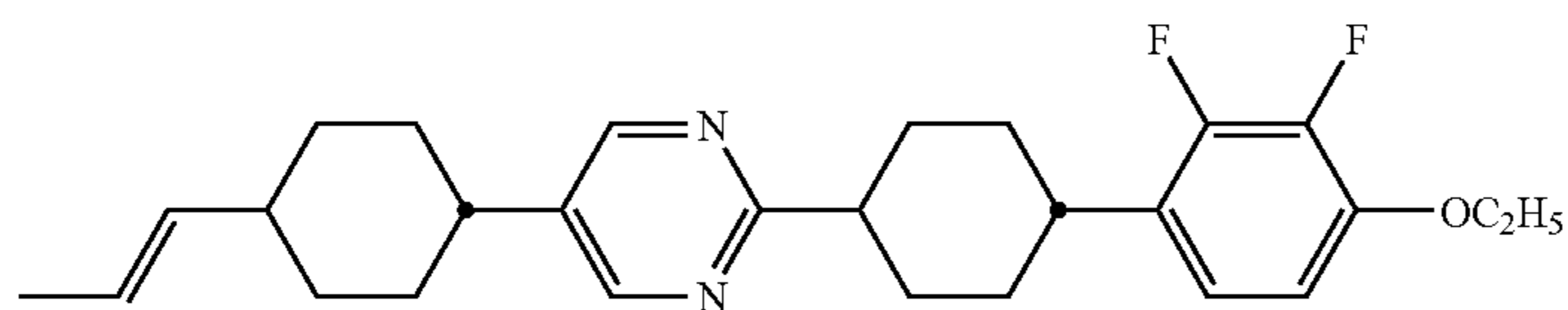
compound NO.255
