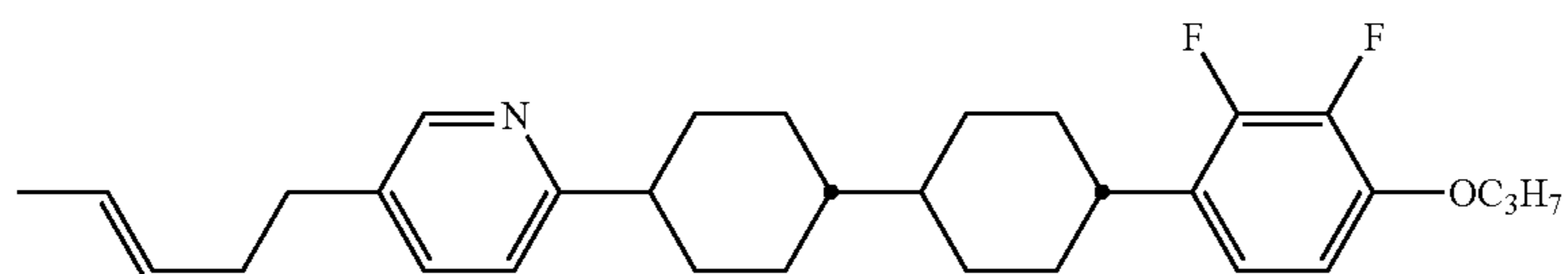
compound NO.263
