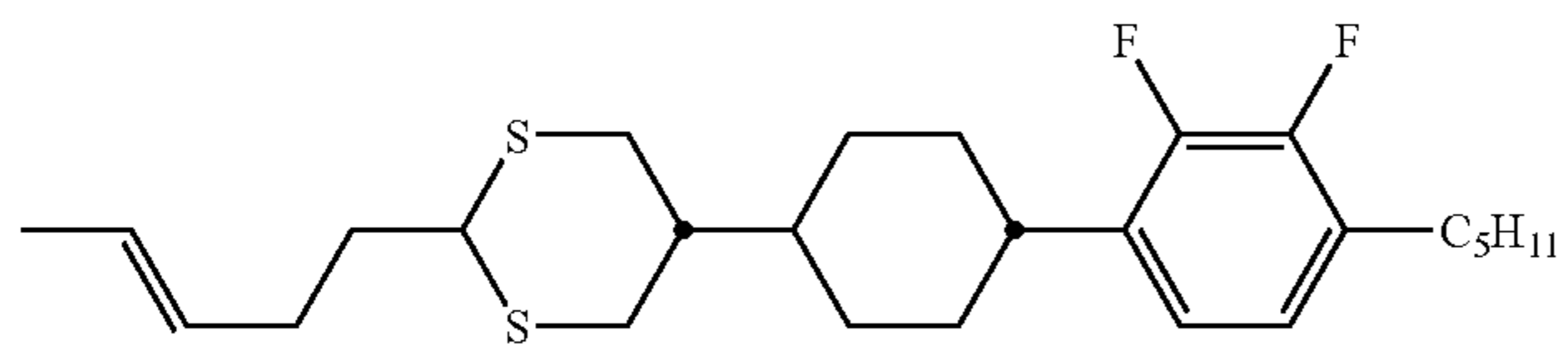
compound NO.203
