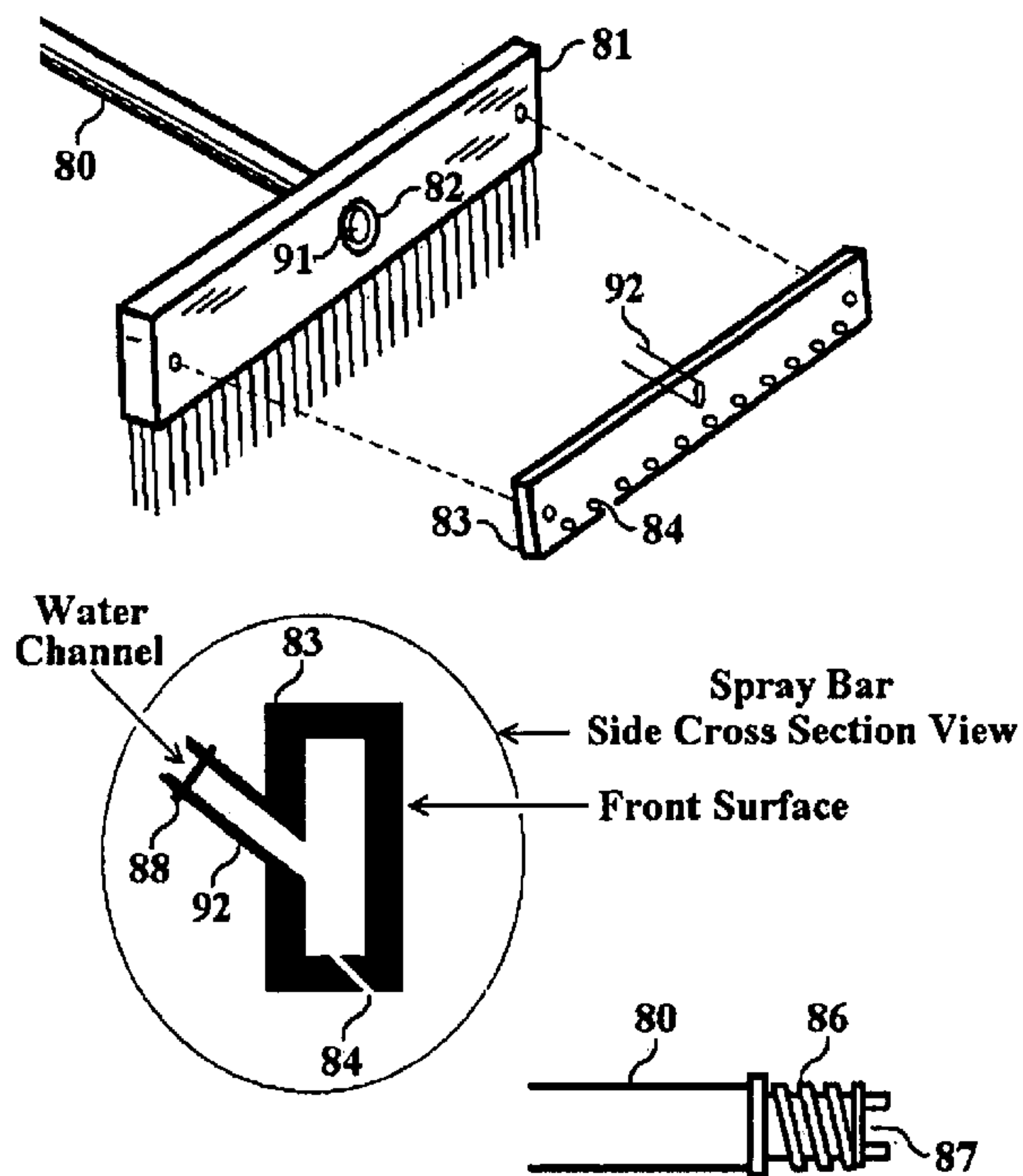
Figure 10A Spray Bar on Front of Broom Head
