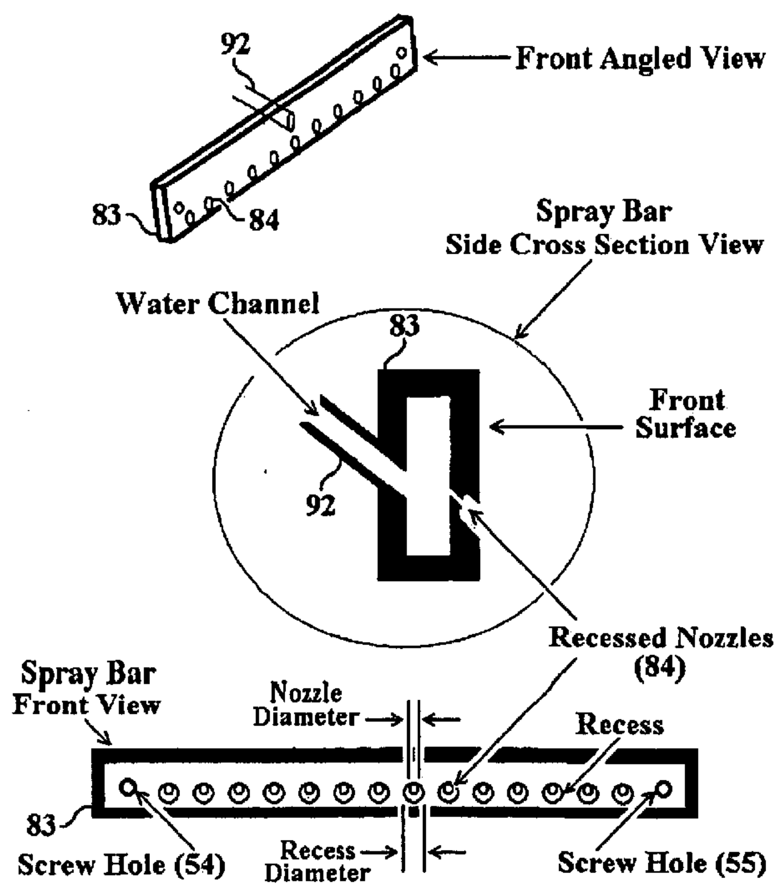
Figure 10B Alternative Configuration, Recessed Nozzles on Front of Spray Bar
