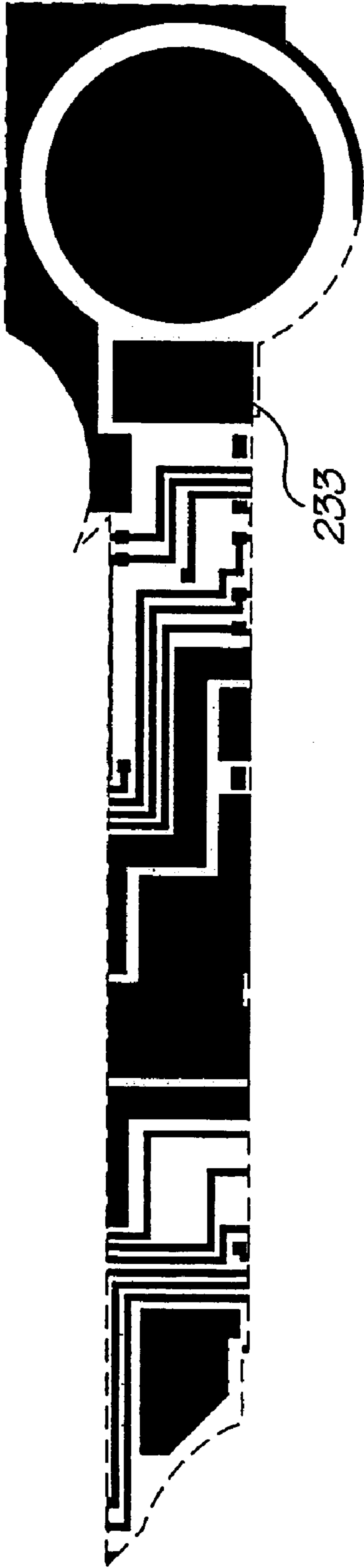
Metal 2 mask
