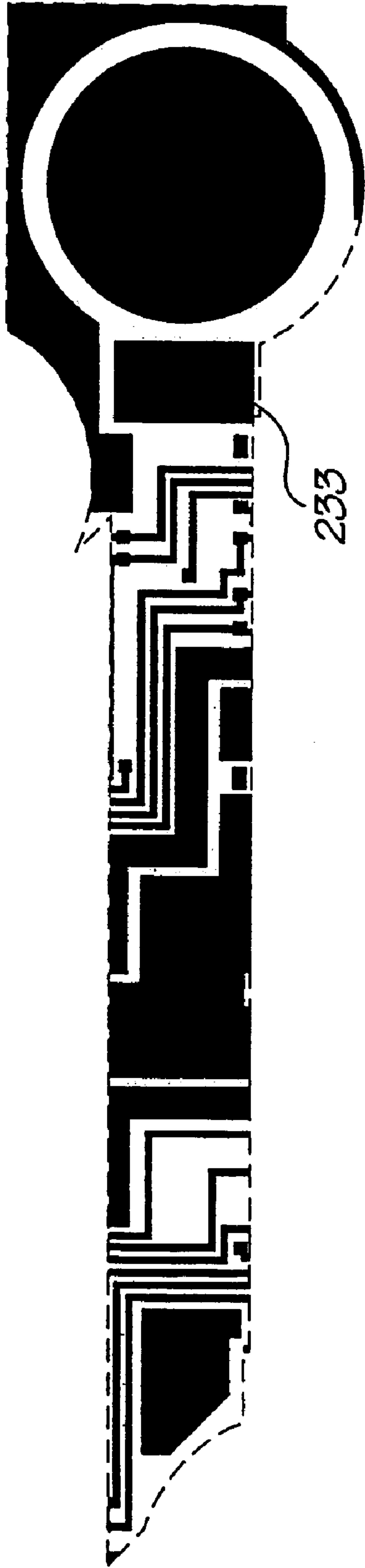
Metal 2 mask
