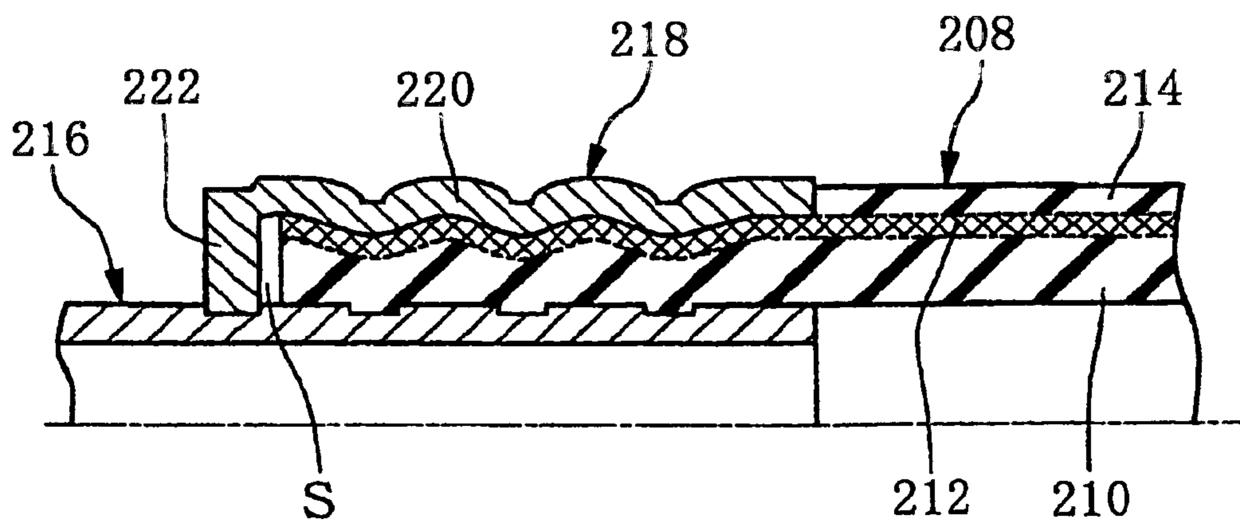
FIG. 12 (PRIOR ART)
