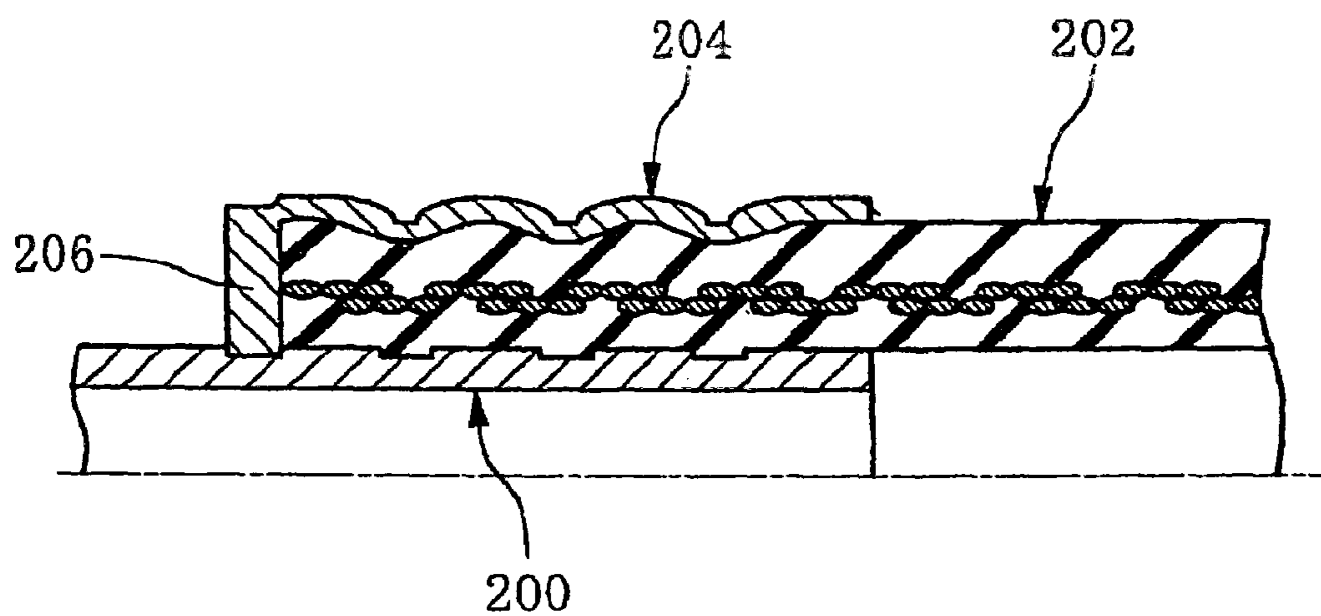
FIG. 11 (PRIOR ART)
