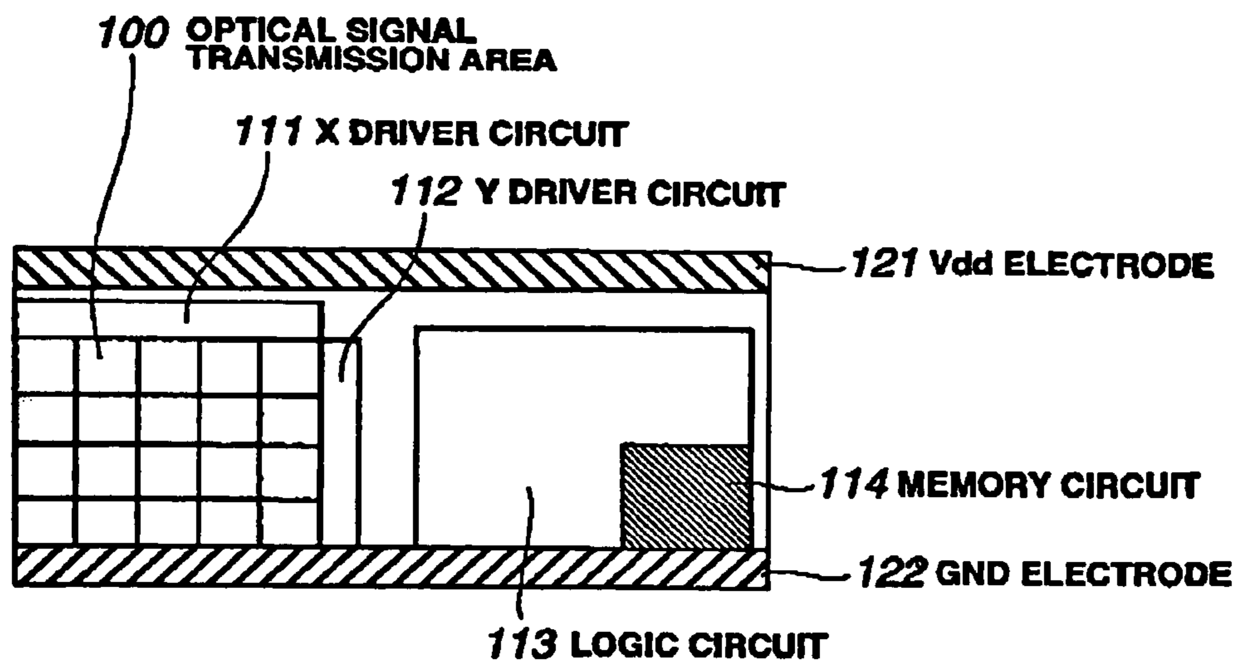
OPTICAL SIGNAL TRANSMISSION SUBSTRATE OF EXAMPLE
