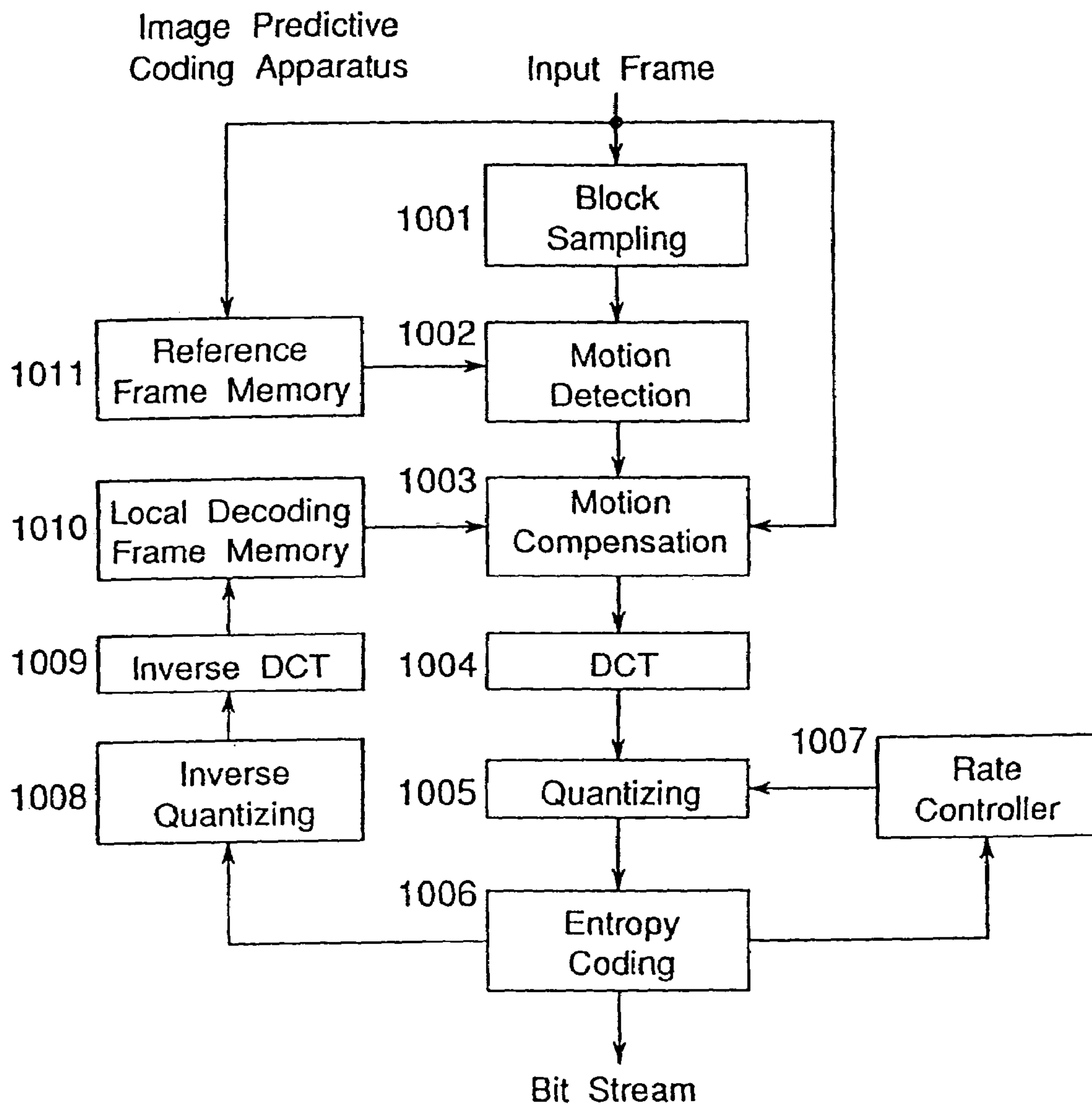
Fig. 14 PRIOR ART
