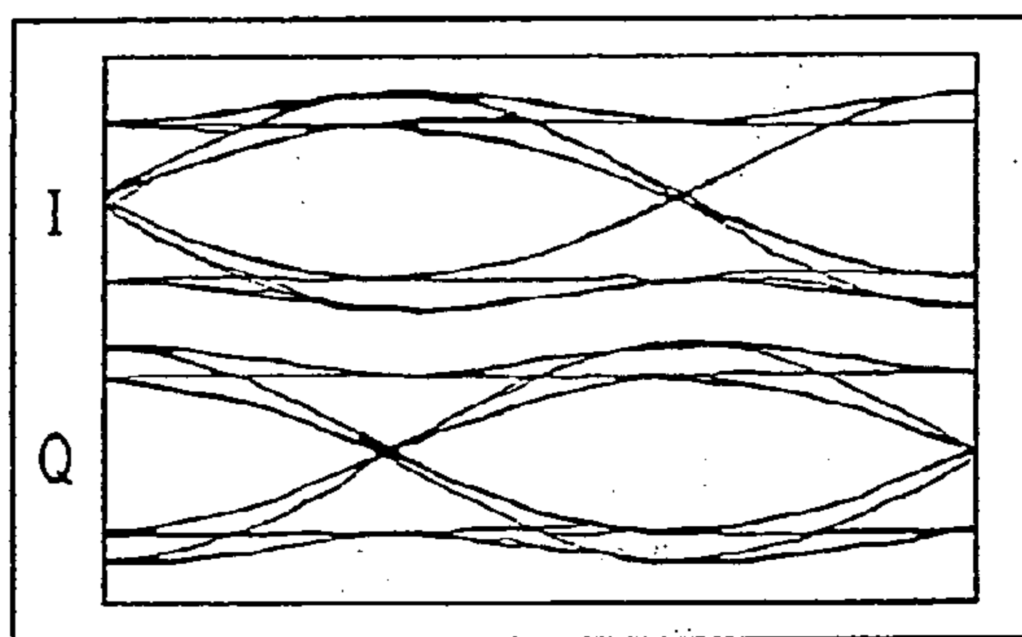
FQPSK-B MEAS. FIG. 19D
