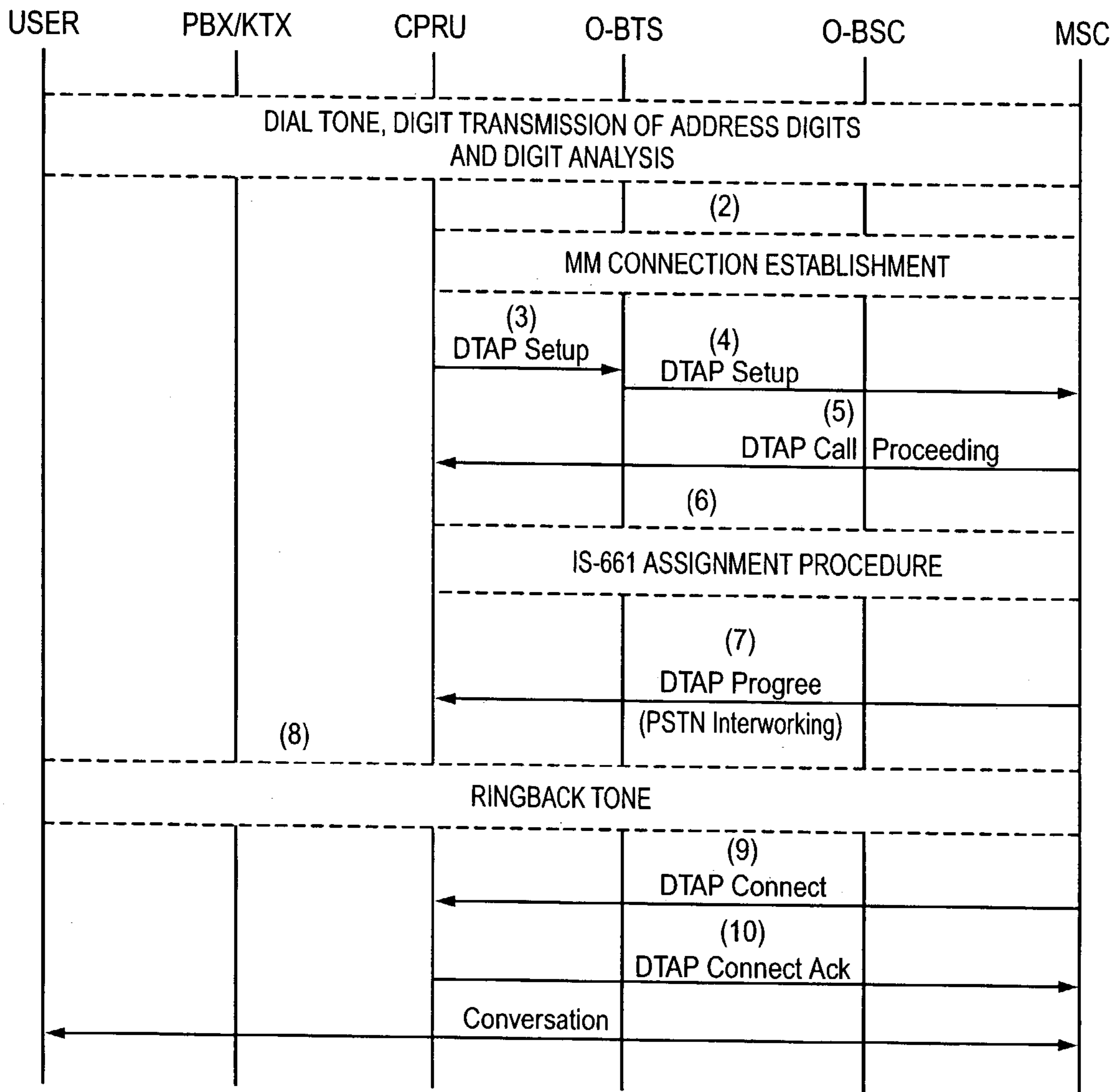
Successful Outgoing Call Setup (PSTN Interworking)
