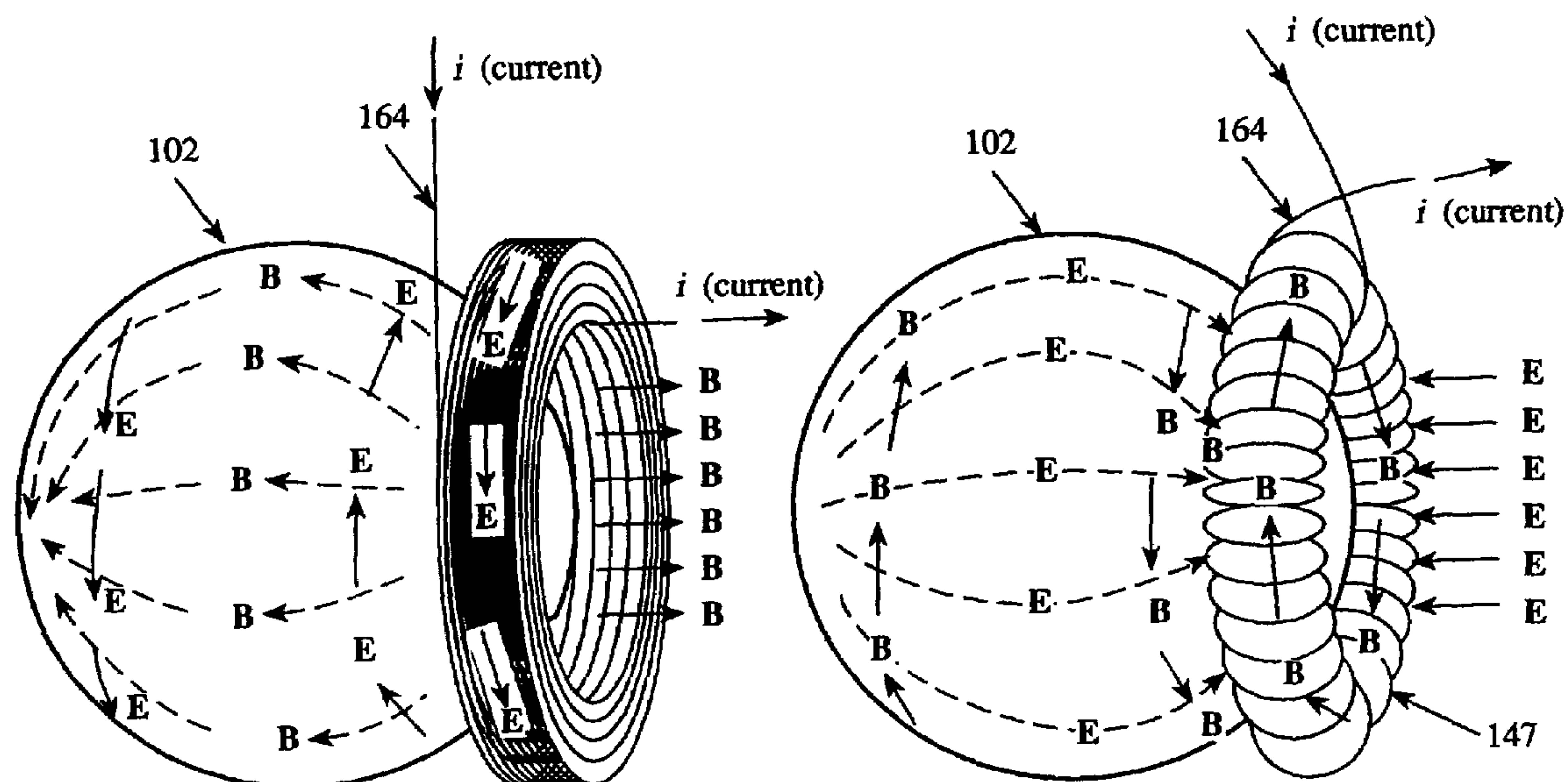
Interaction of a Rowland Ring coil's E & B fields with a conducting sphere's E & B fields.
