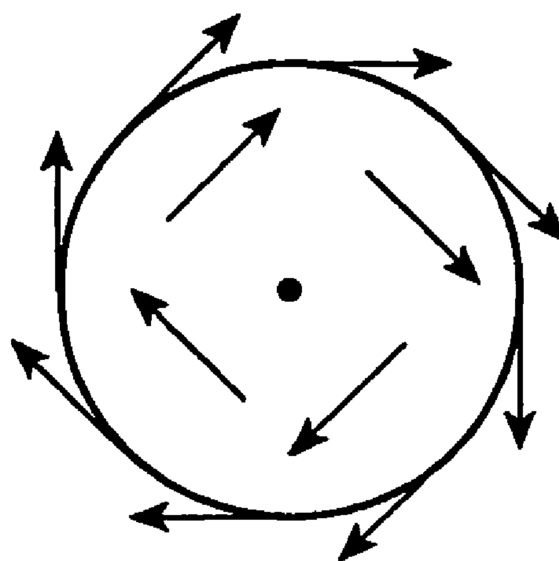
End View of Core Tangential Magnetic Field
