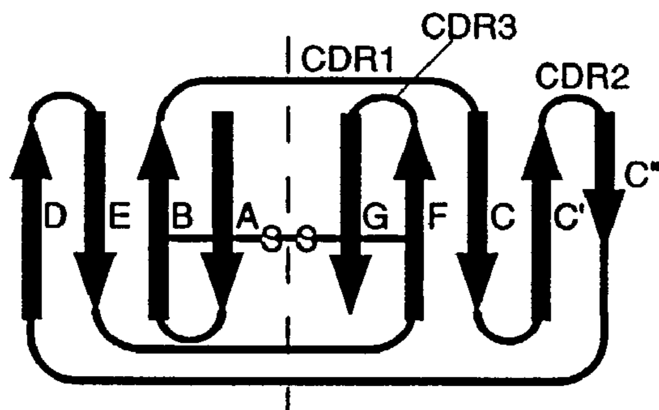
Immunoglobulin VH
