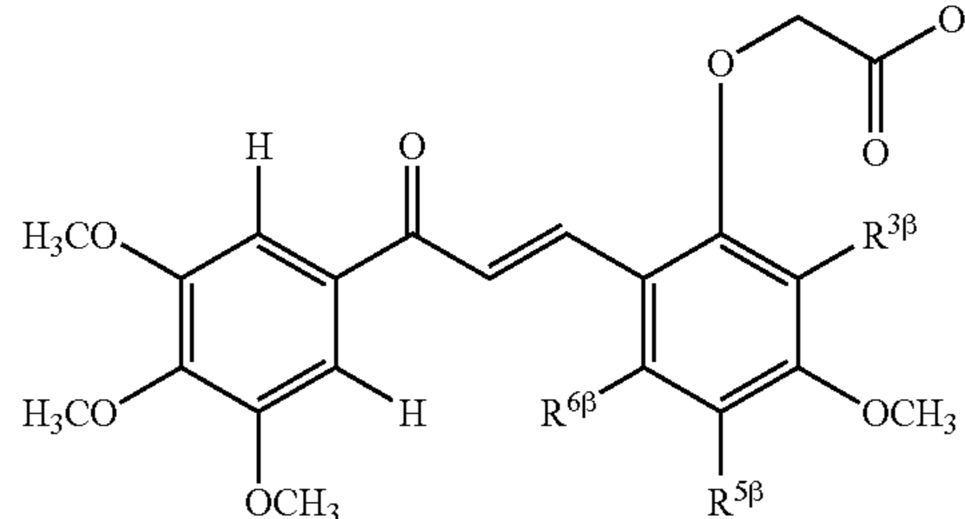
Example Table 12. 3-[3 or 6-(Heteroaryl)-2-carboxymethoxy-4-methoxyphenyl]-1-[(3,4,5-trimethoxy)phenyl]-2-propen-1-ones.
