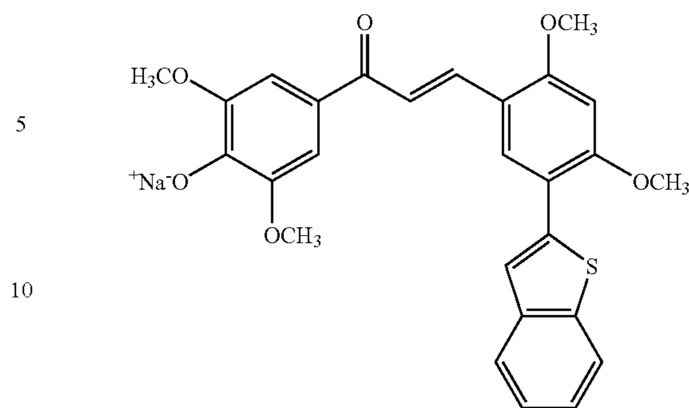
3-[5-(benzo[b]thien-2-yl)-2,4-dimethoxyphenyl]-1-(4-hydroxy-3,5-dimethoxyphenyl)-2-propen-1-one, sodium salt
