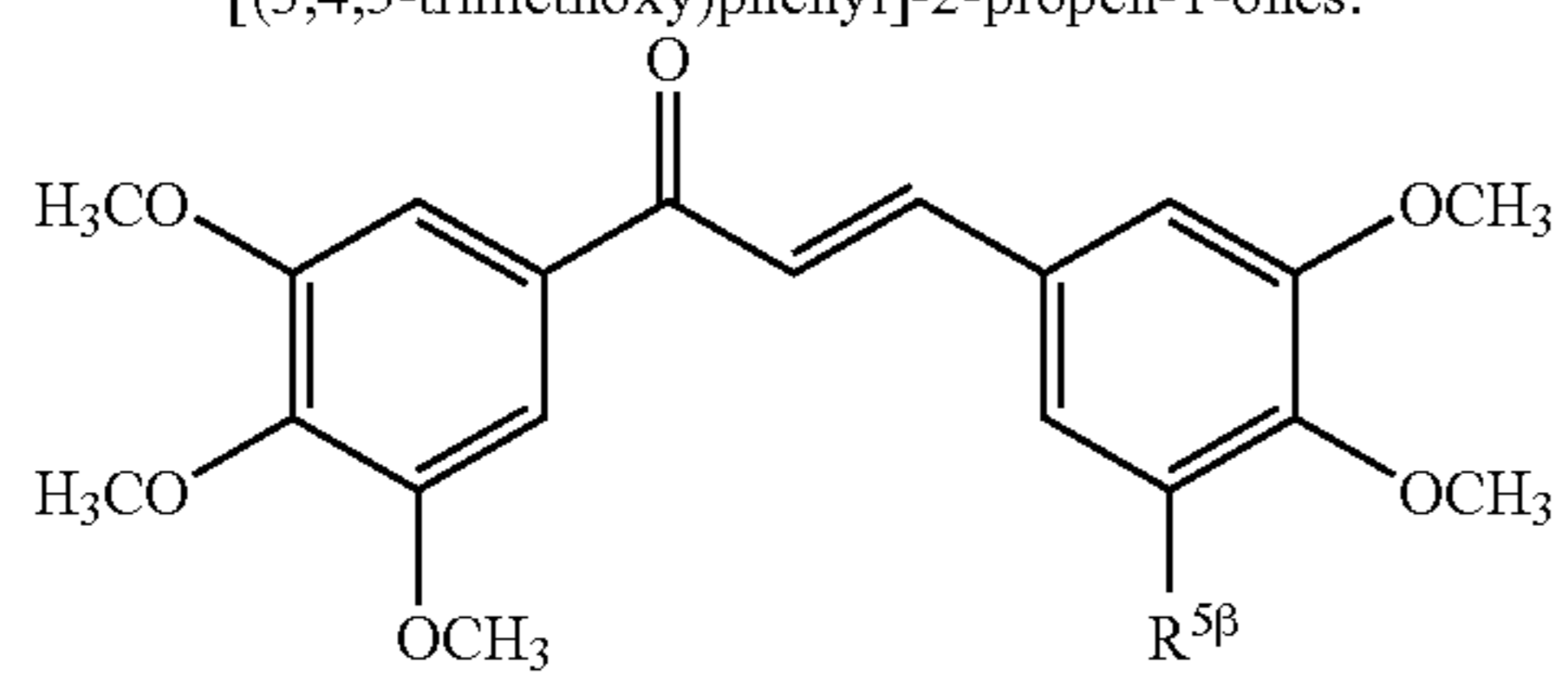
Example Table 9. 3-[5-(Heteroaryl or Heterocyclic)-3,4-dimethoxyphenyl]-1-[(3,4,5-trimethoxy)phenyl]-2-propen-1-ones.
