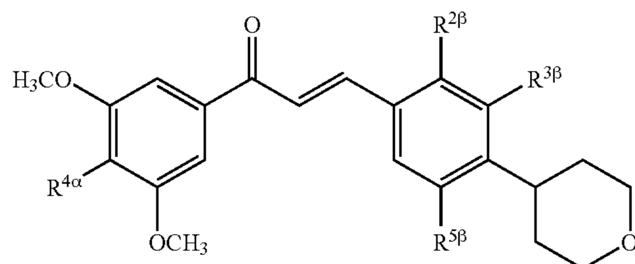
Example Table 28. Substituted 3-[4-(pyran-4-yl)phenyl]-1-[(3,5-dimethoxy)phenyl]-2-propen-1-ones.
