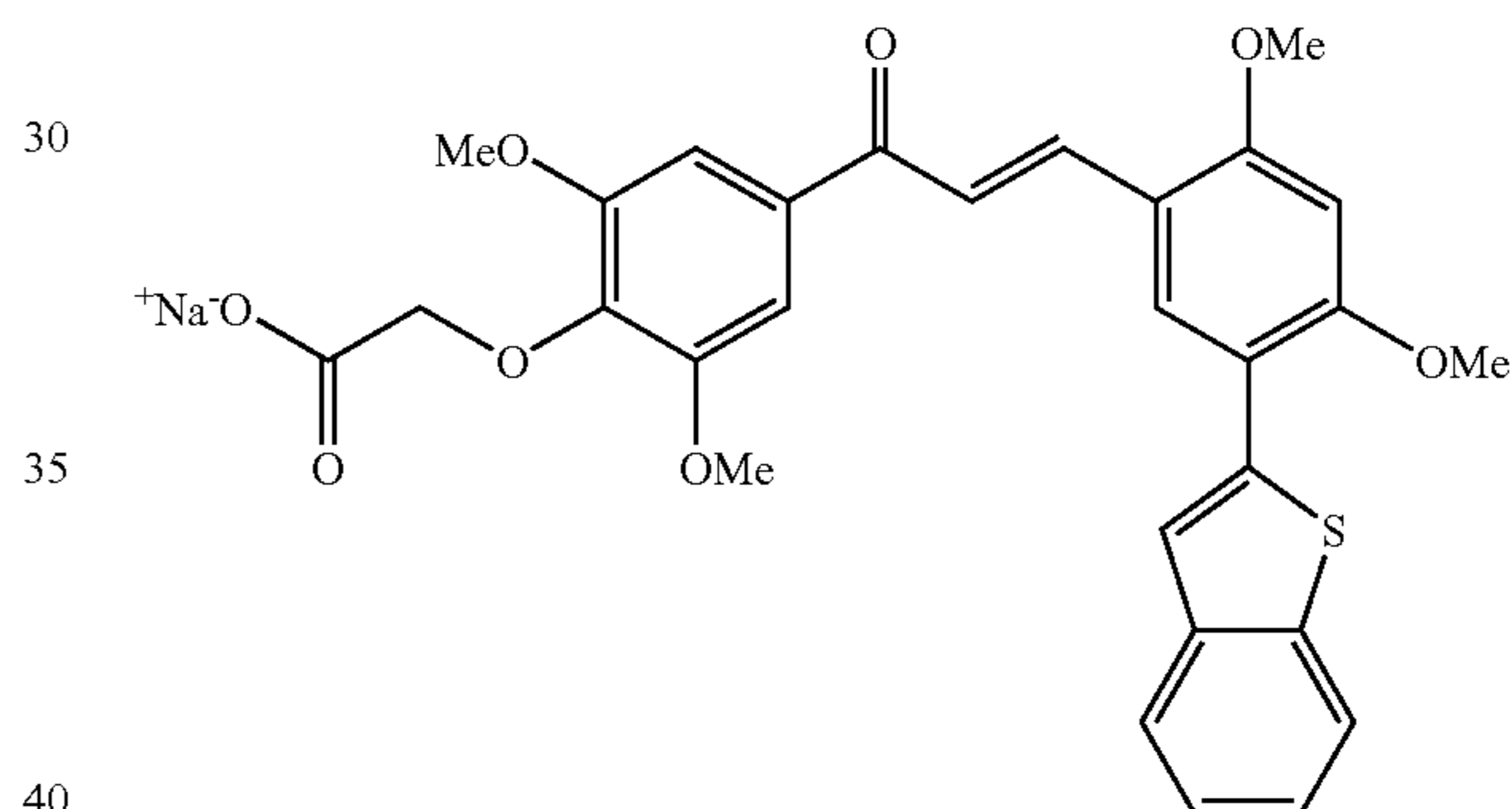
3-[5-(Benzo[b]thien-2-yl)-2,4-dimethoxyphenyl]-1-(4-carboxymethoxy-3,5-dimethoxyphenyl)-2-propen-1-one, sodium salt
