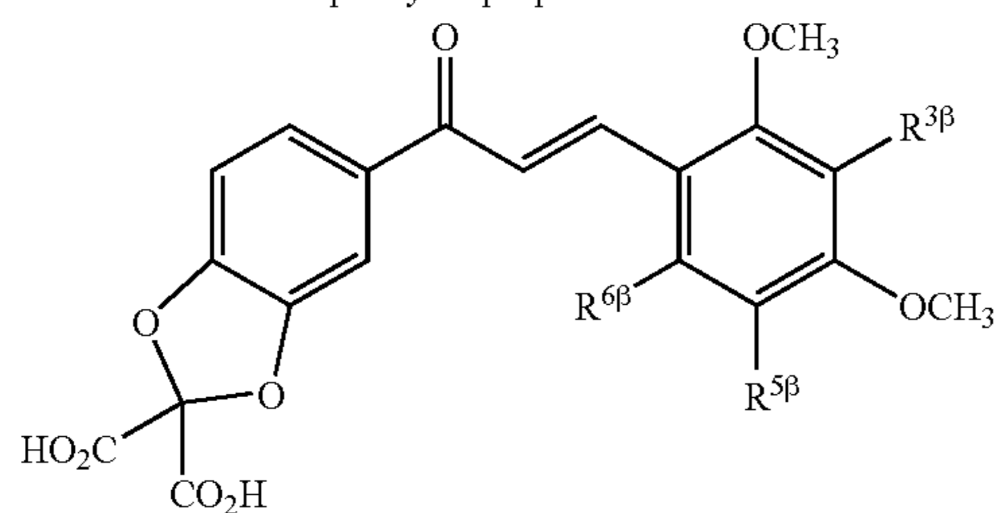
Example Table 19. Substituted 3-[3-, 5- or 6-(Heteroaryl)-2,4-dimethoxyphenyl]-1-phenyl-2-propen-1-ones.
