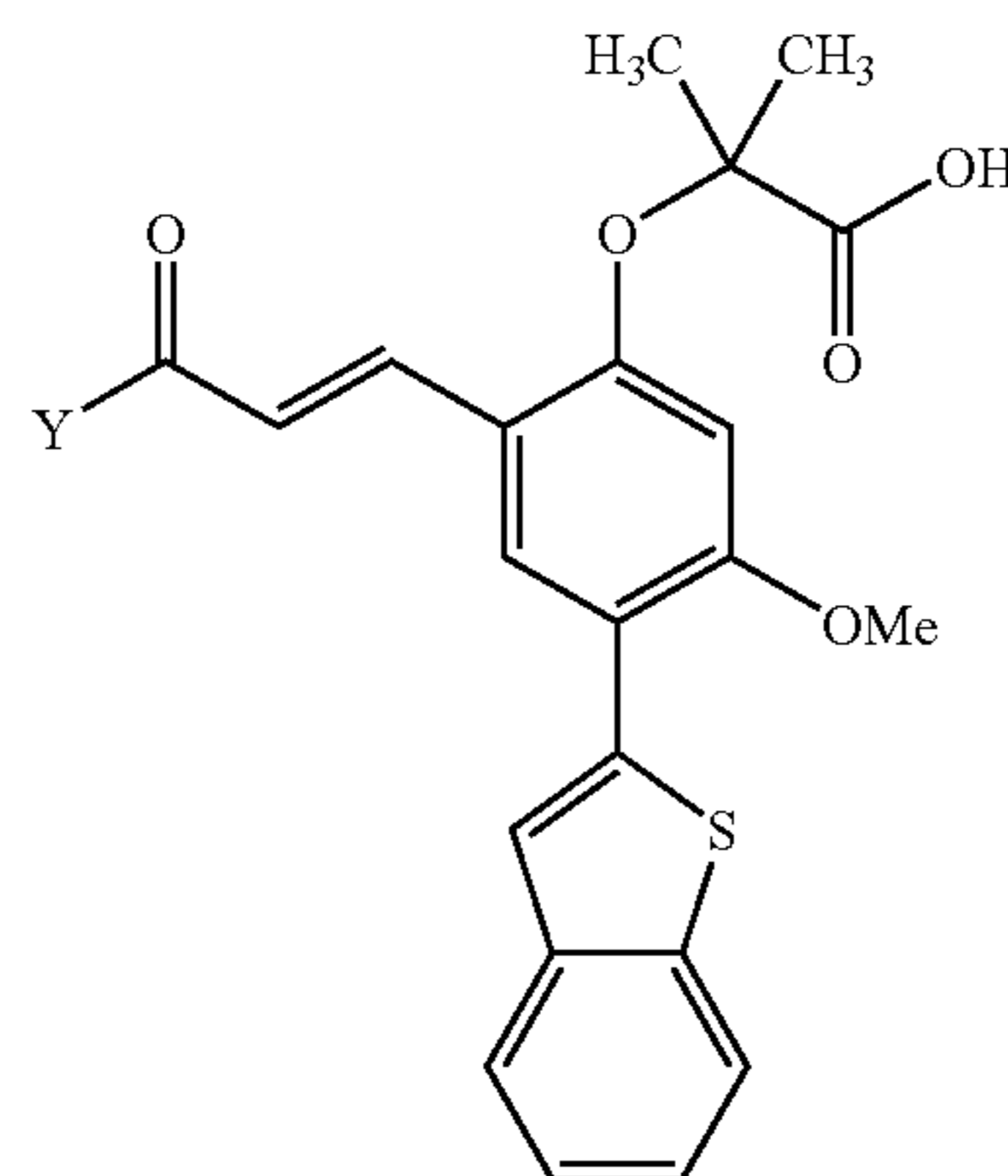
Example Table 29. Substituted 3-[5-(benzo[b]thien-2-yl)-2-(2-carboxy-2-propoxy)-4-methoxyphenyl]-1-phenyl-2-propen-1-ones.
