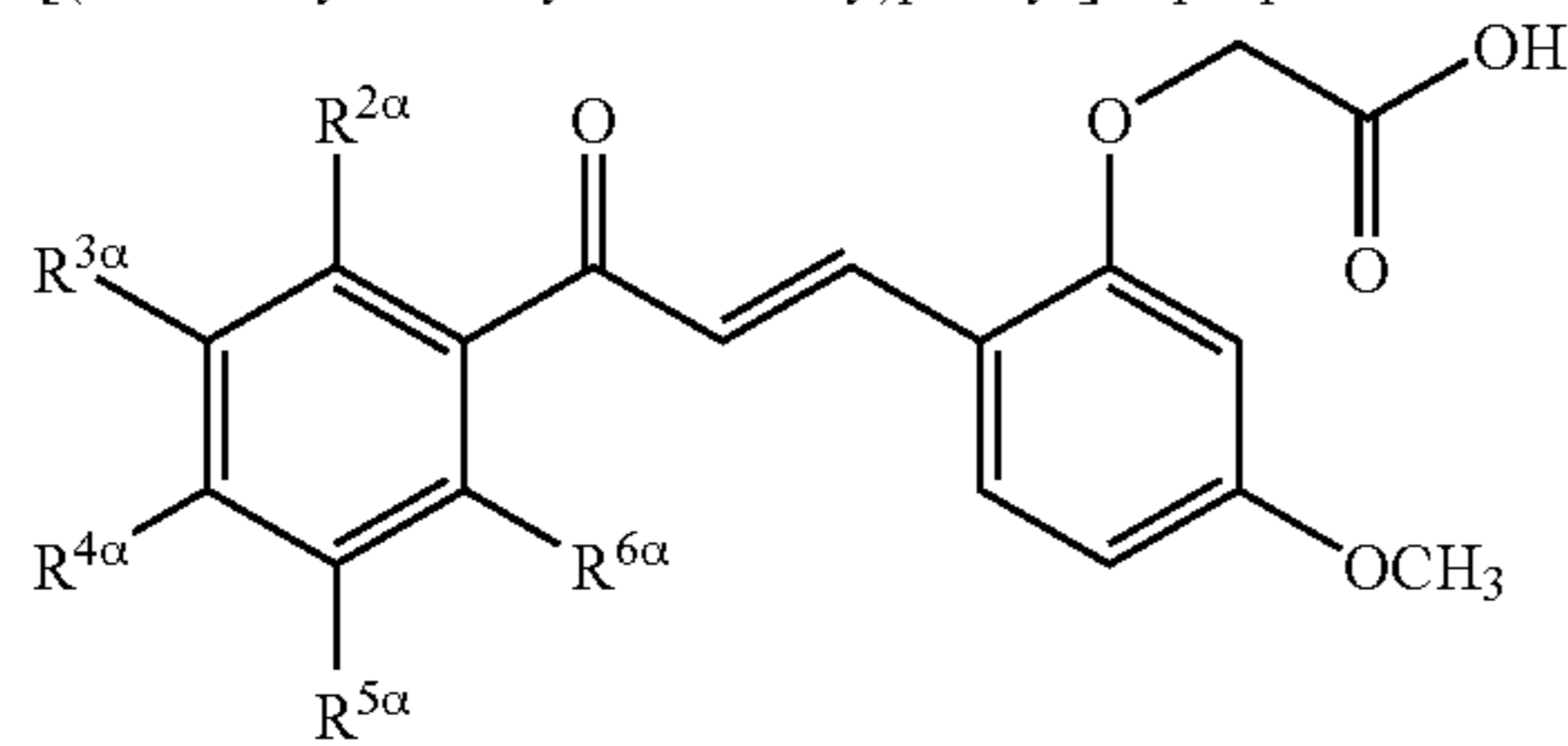
Example Table 11. 1-[4-(Heteroaryl or Heterocyclic)-phenyl]-3-[(2-carboxymethoxy-4-methoxy)phenyl]-2-propen-1-ones.
