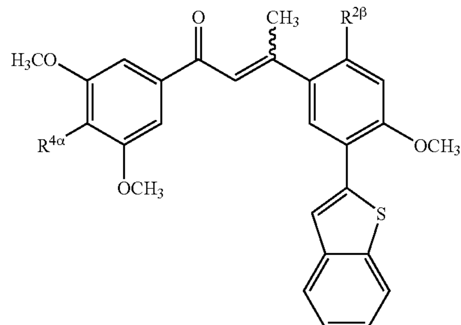
Example Table 10. Substituted 3-[5-(benzo[b]thien-2-yl)-4-methoxyphenyl]-1-[3,5-dimethoxyphenyl]-2-buten-1-ones.
