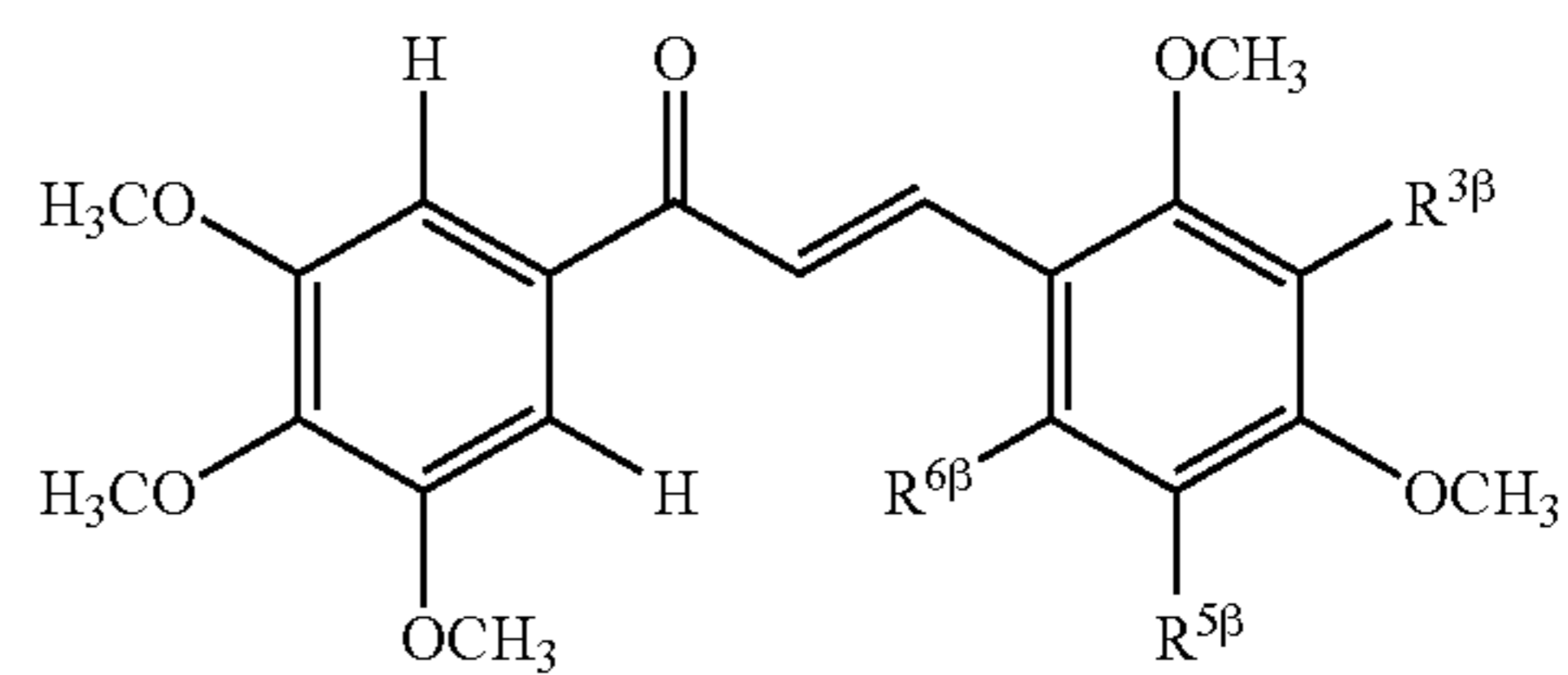
Example Table 13. 3-[3 or 6-(Heteroaryl)-2,4-dimethoxyphenyl]-1-[(3,4,5-trimethoxy)phenyl]-2-propen-1-ones.
