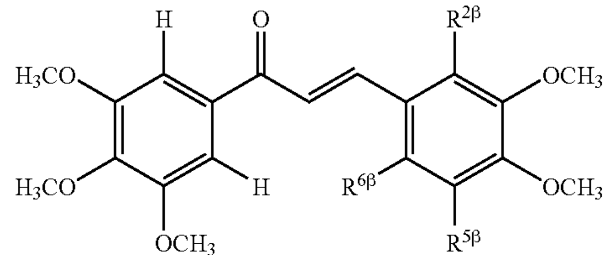
Example Table 14. 3-[2 or 6-(Heteroaryl)-3,4-dimethoxyphenyl]-1-[(3,4,5-trimethoxy)phenyl]-2-propen-1-ones.
