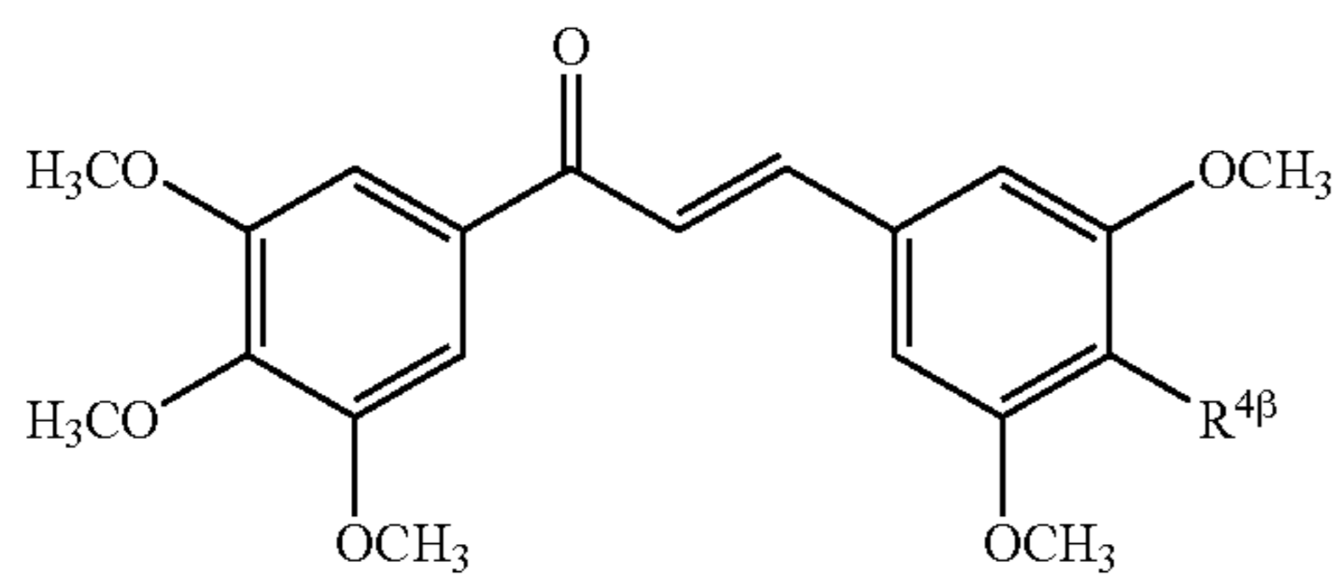
Example Table 26. 3-[4-(Heteroaryl or Heterocyclic)-3,5-dimethoxyphenyl]-1-[(3,4,5-trimethoxy)phenyl]-2-propen-1-ones.
