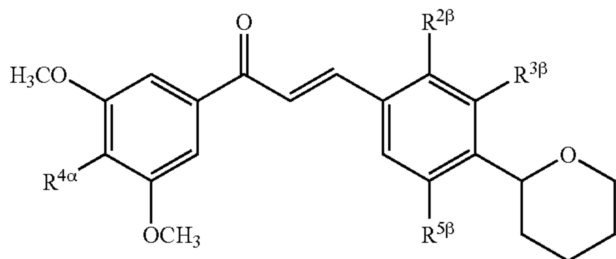
Example Table 27. Substituted 3-[4-(pyran-2-yl)phenyl]-1-[(3,5-dimethoxy)phenyl]-2-propen-1-ones.
