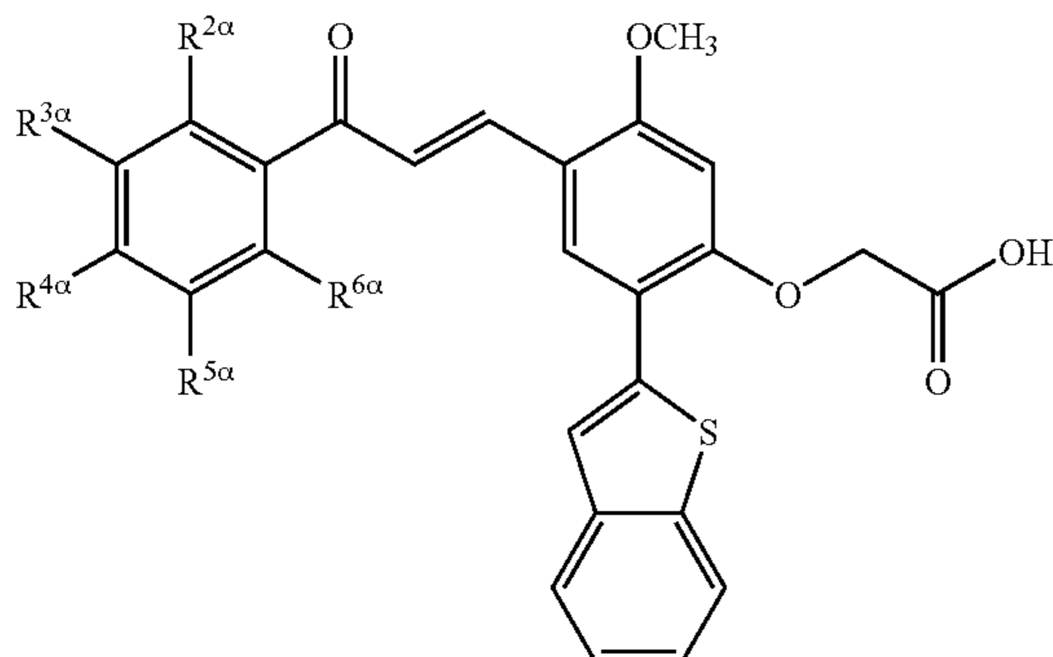
Example Table 21. Substituted 3-[5-(benzo[b]thien-2-yl)-4-carboxymethoxy-2-methoxyphenyl]-1-phenyl-2-propen-1-ones.
