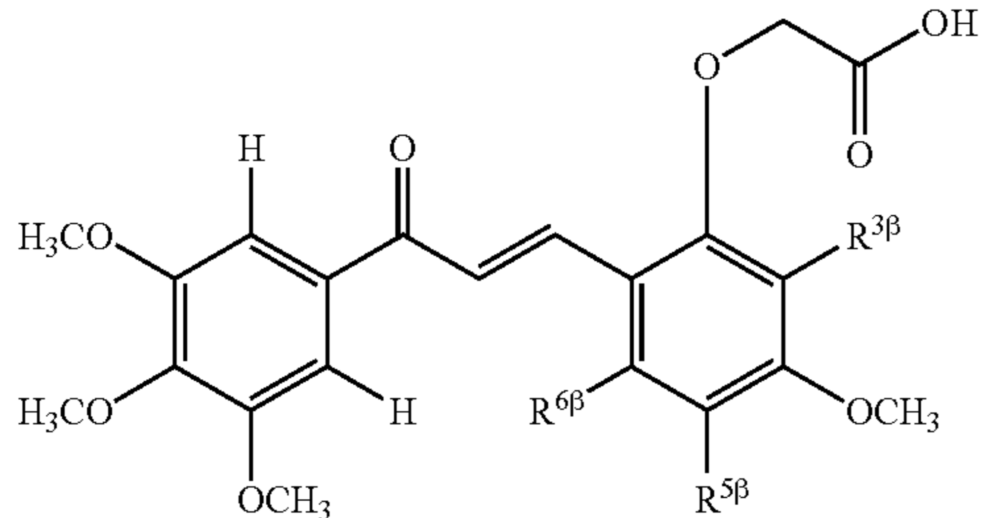
Example Table 12. 3-[3 or 6-(Heteroaryl)-2-carboxymethoxy-4-methoxyphenyl]-1-[(3,4,5-trimethoxy)phenyl]-2-propen-1-ones.
