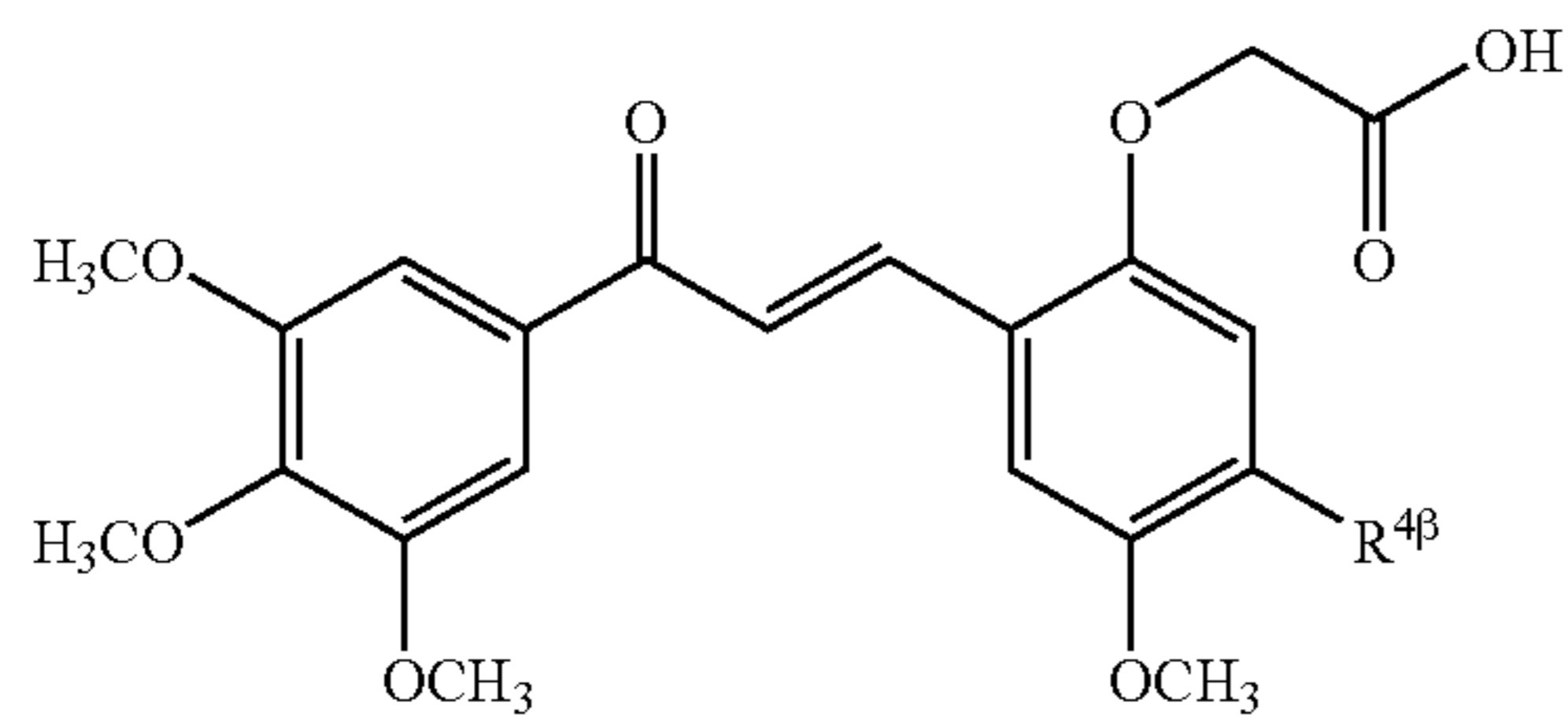
Example Table 24. 3-[4-(Heteroaryl or Heterocyclic)-2-carboxymethoxy-4-methoxyphenyl]-1-[(3,4,5-trimethoxy)phenyl]-2-propen-1-ones.
