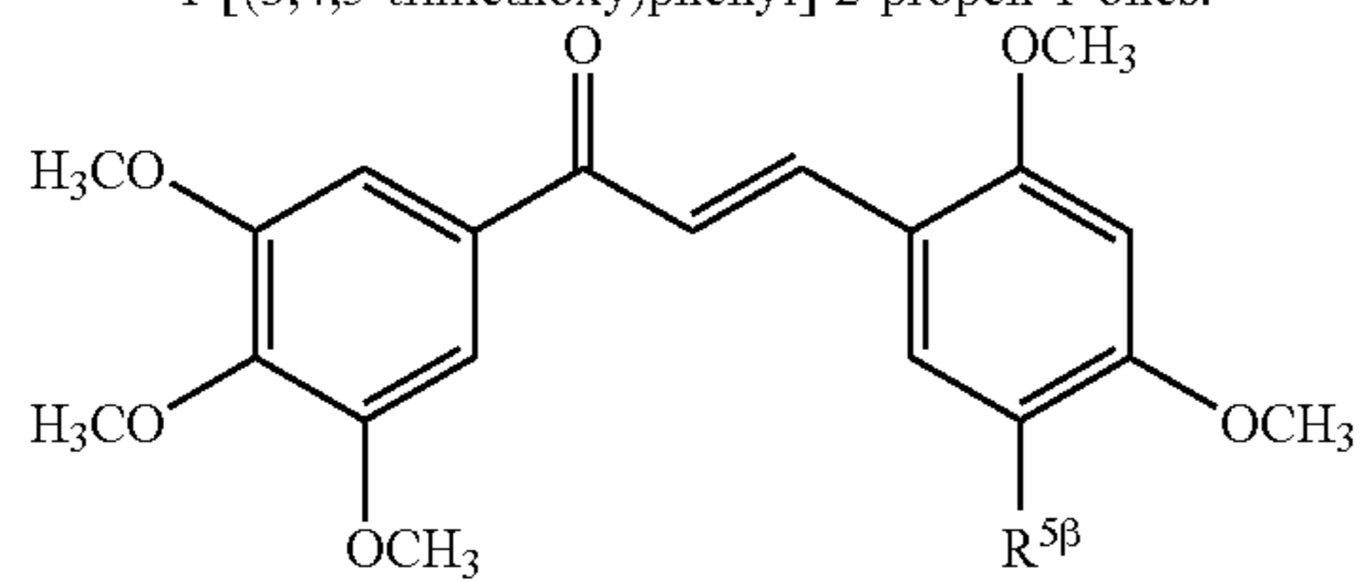
Example Table 8. 3-[5-(Heteroaryl or Heterocyclic)-2,4-dimethoxyphenyl]-1-[(3,4,5-trimethoxy)phenyl]-2-propen-1-ones.
