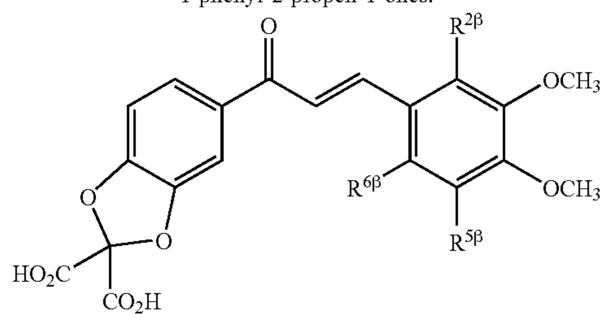
Example Table 20. Substituted 3-[2-, 5- or 6-(Heteroaryl)-3,4-dimethoxyphenyl]-1-phenyl-2-propen-1-ones.
