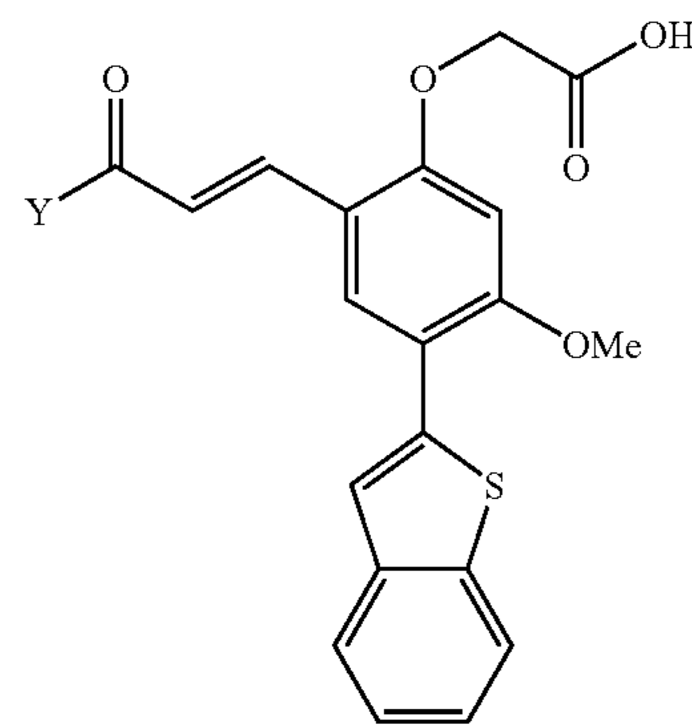
Example Table 22. Substituted 3-[5-(benzo[b]thien-2-yl)-2-carboxymethoxy-4-methoxyphenyl]-1-phenyl-2-propen-1-ones.
