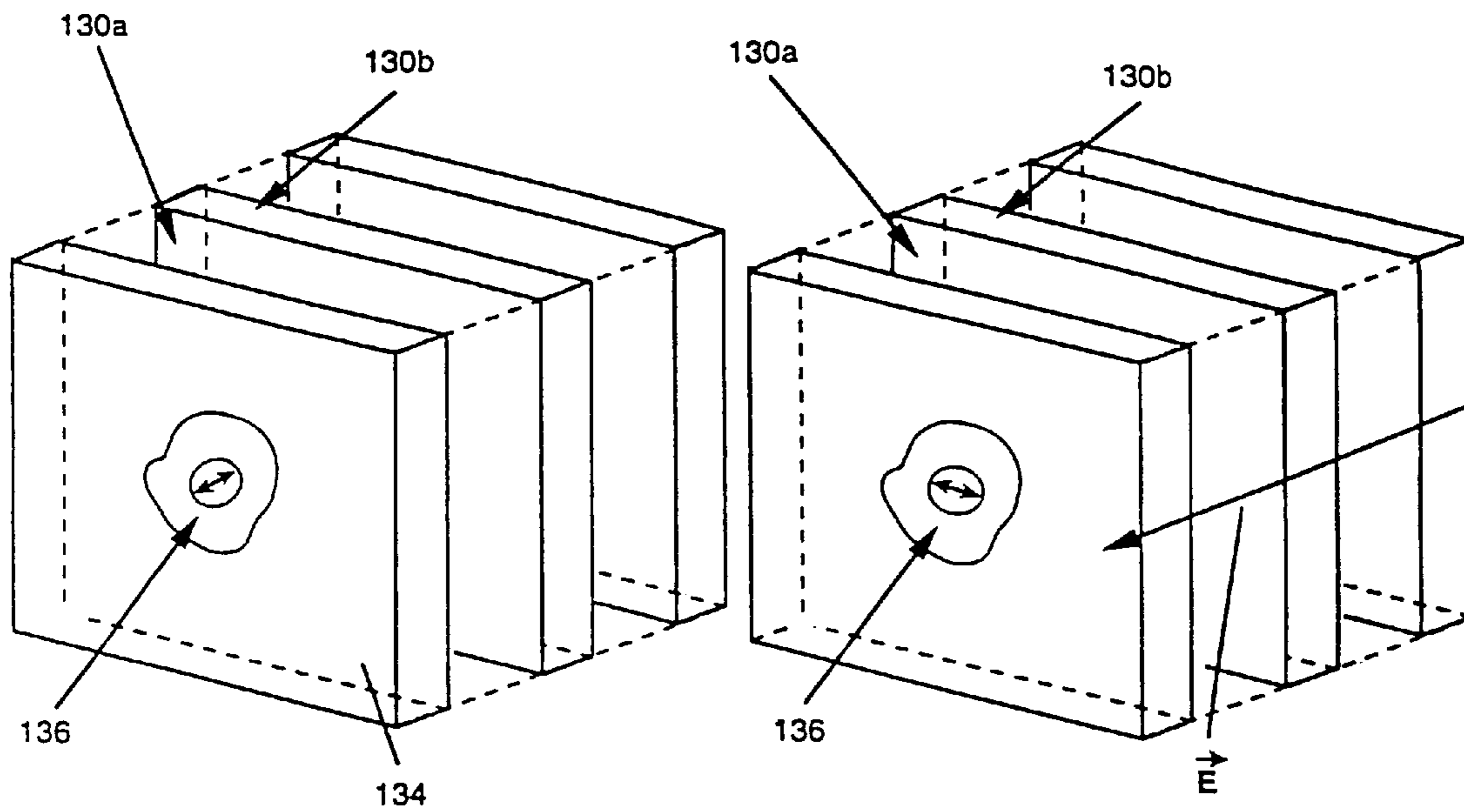
Reflection Grating
