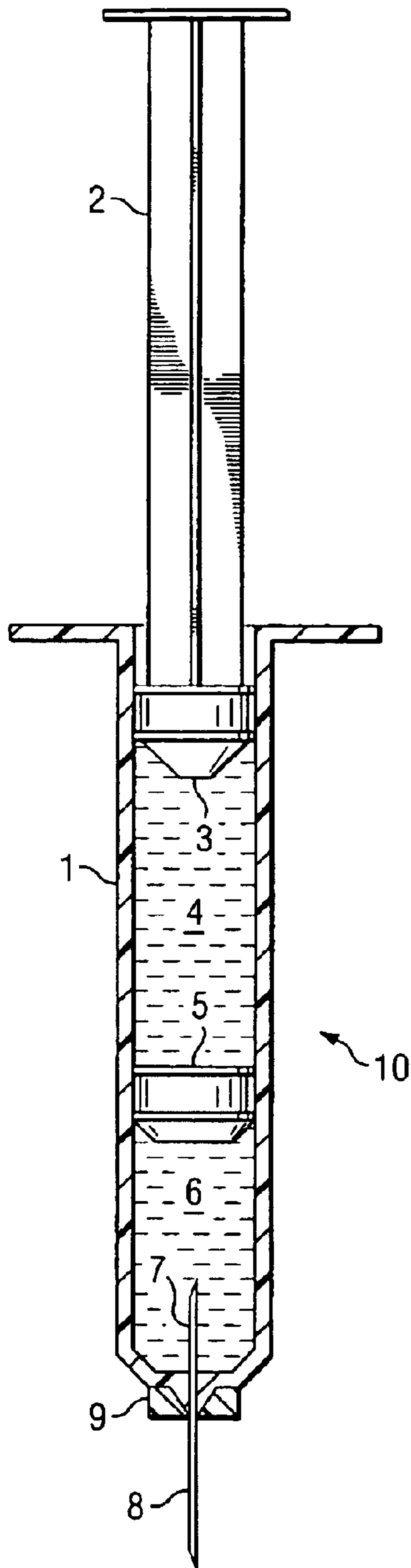
FIG. 1 (PRIOR ART)
