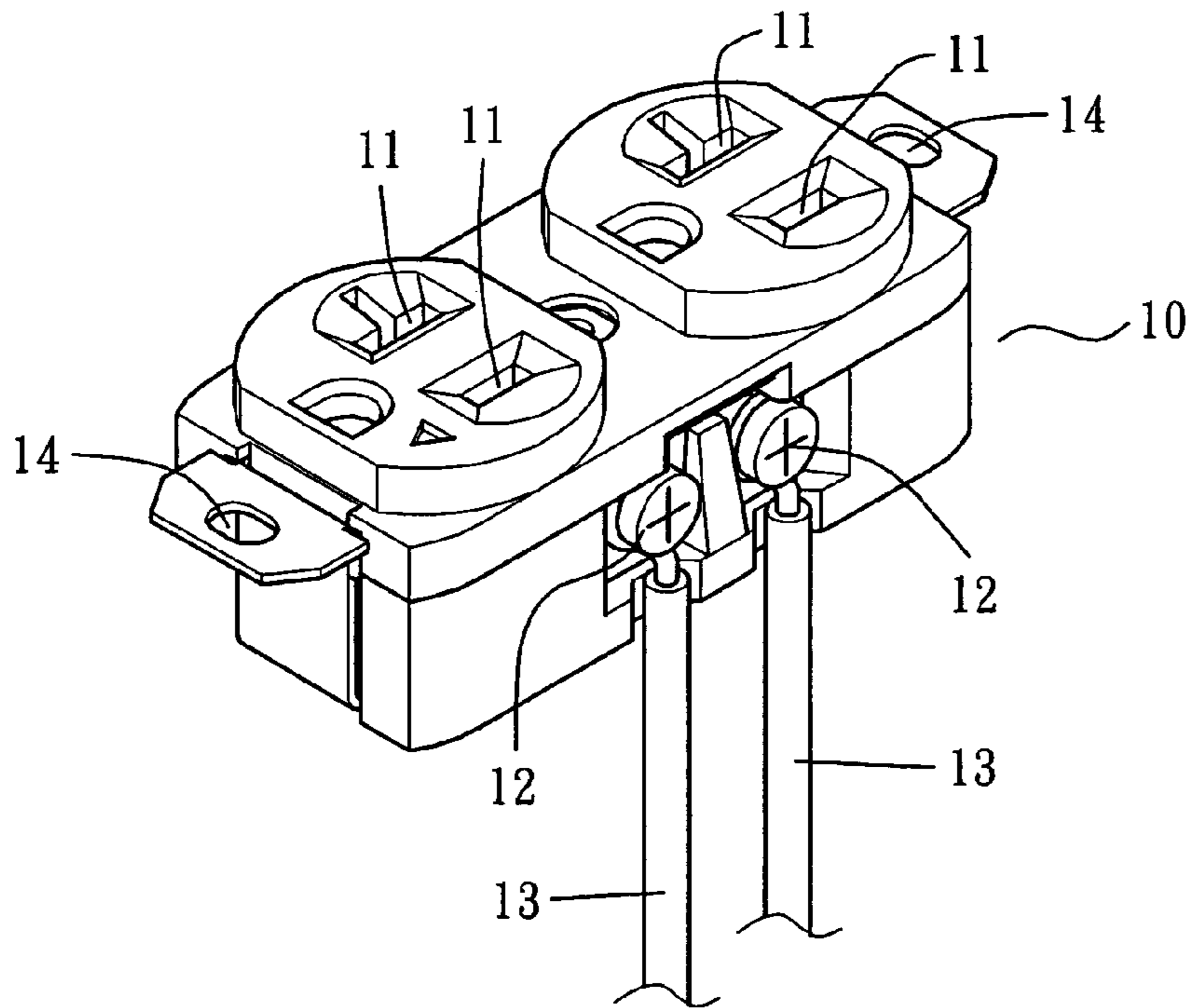
FIG. 2 (PRIOR ART)
