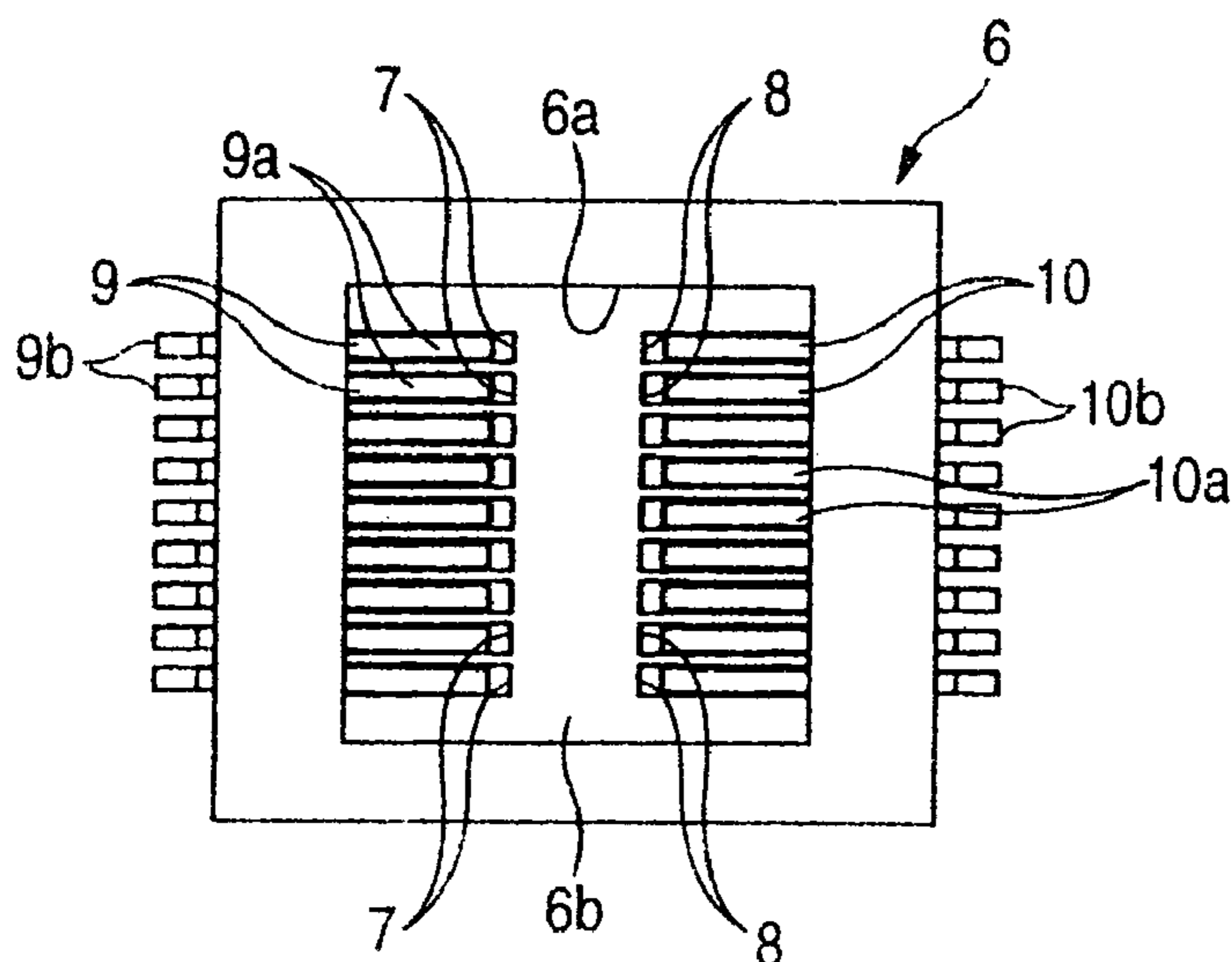
FIG. 5A Related Art
