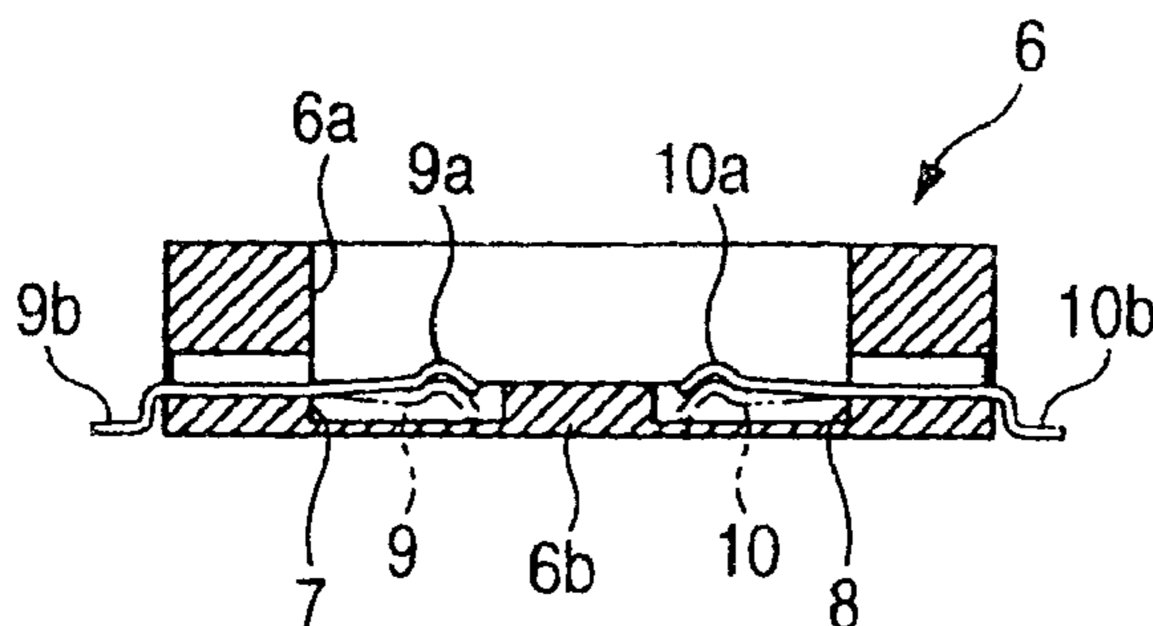
FIG. 5D Related Art
