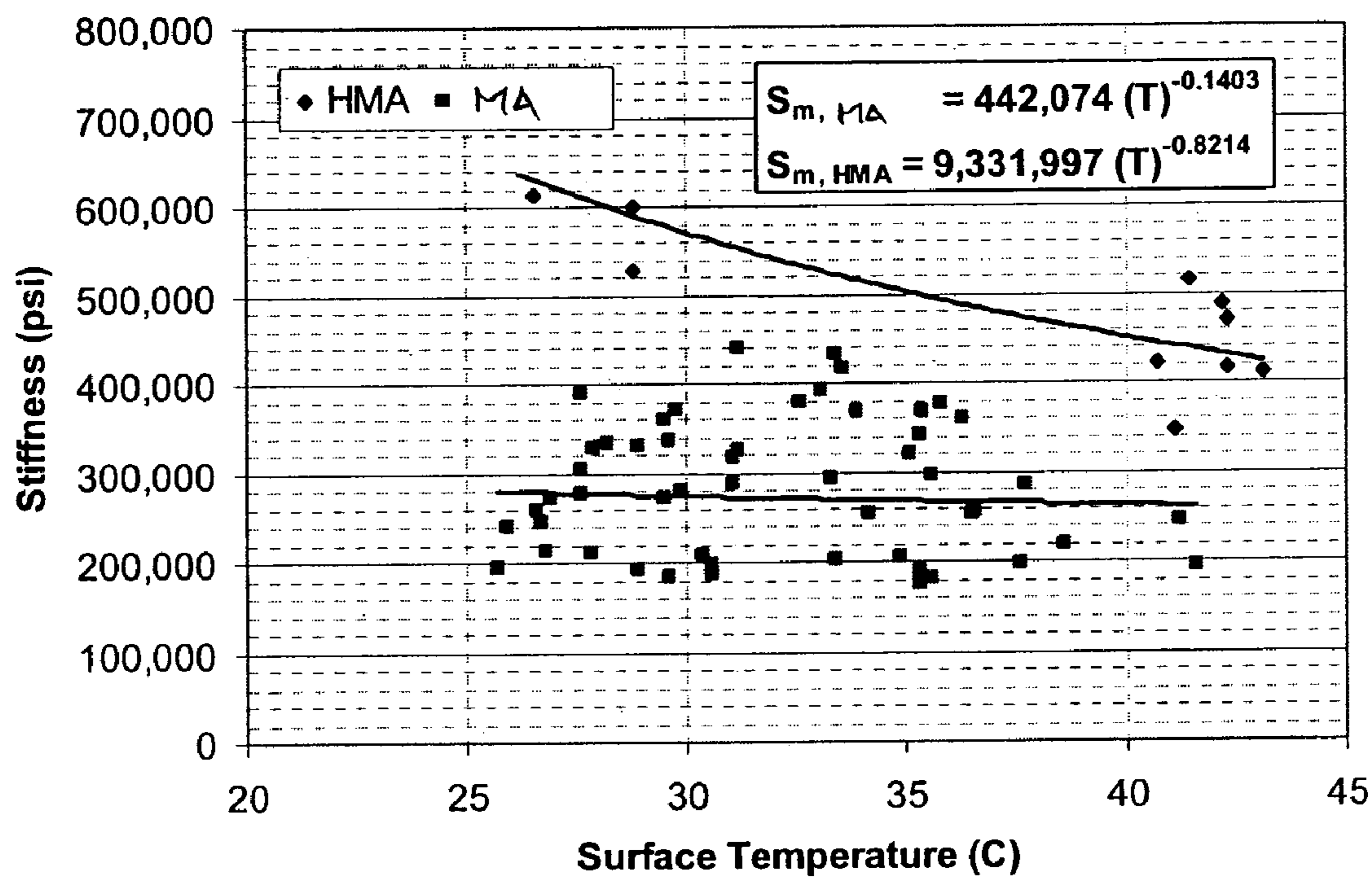
Figure 3. Surface temperature versus stiffness
