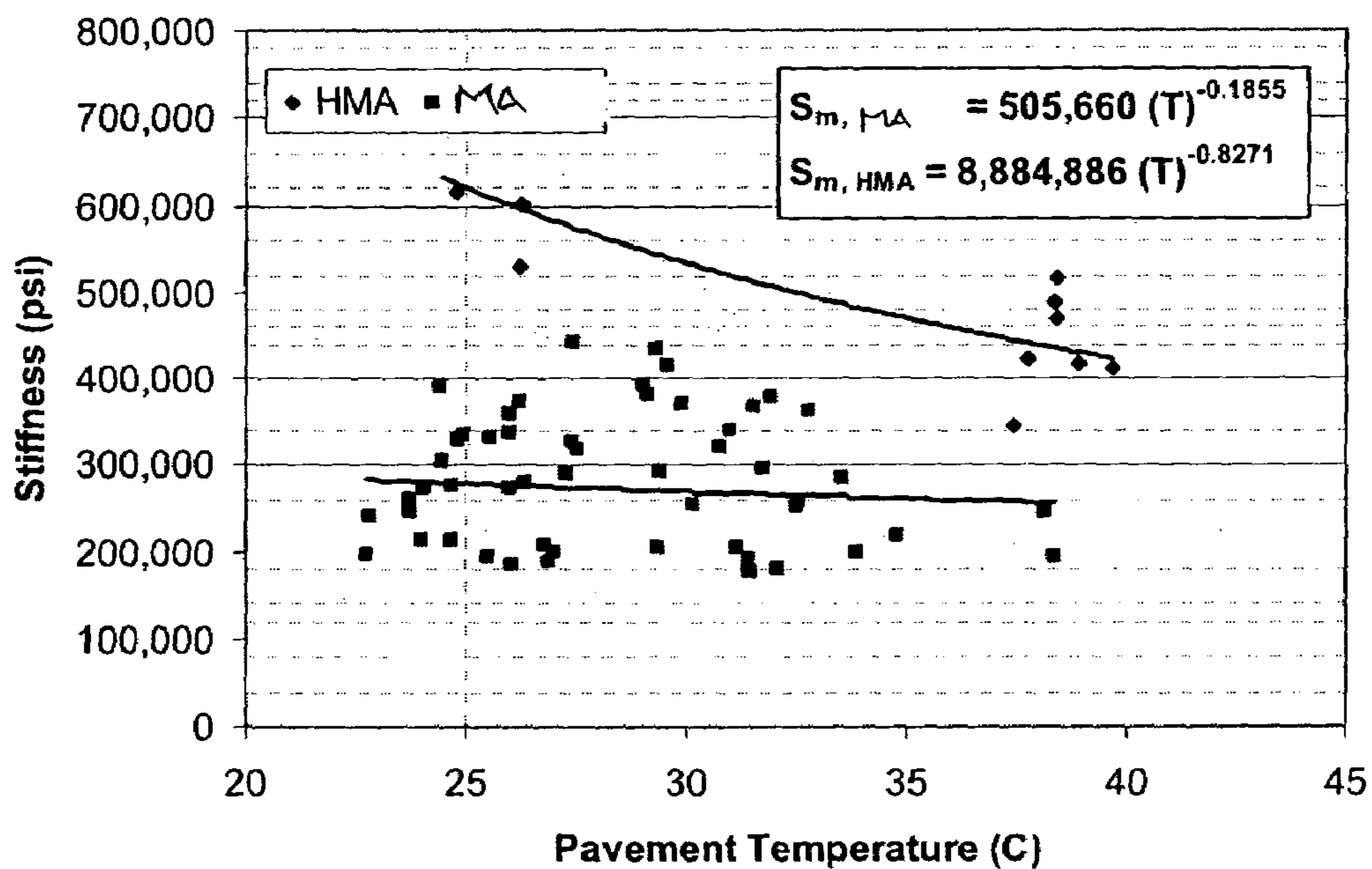
Figure 14: Pavement temperature versus stiffness
