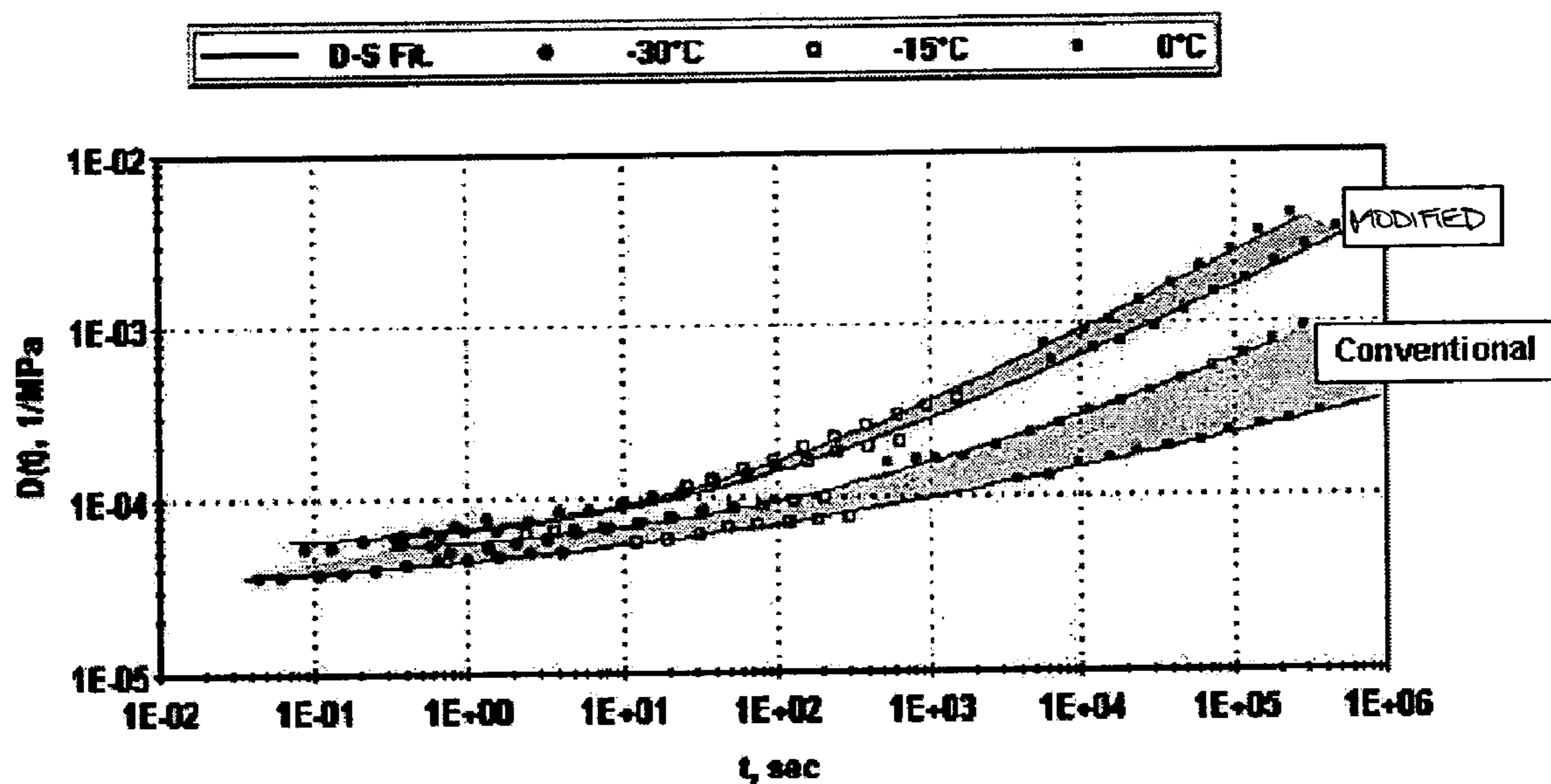
Figure 15: D(t) Mastercurves for conventional HMA and Modified ( T_{ref} = -18.1^{\circ}\text{C}/-0.6^{\circ}\text{F} ) (test temperatures of the individual shifted isotherms are identified by different symbols)
