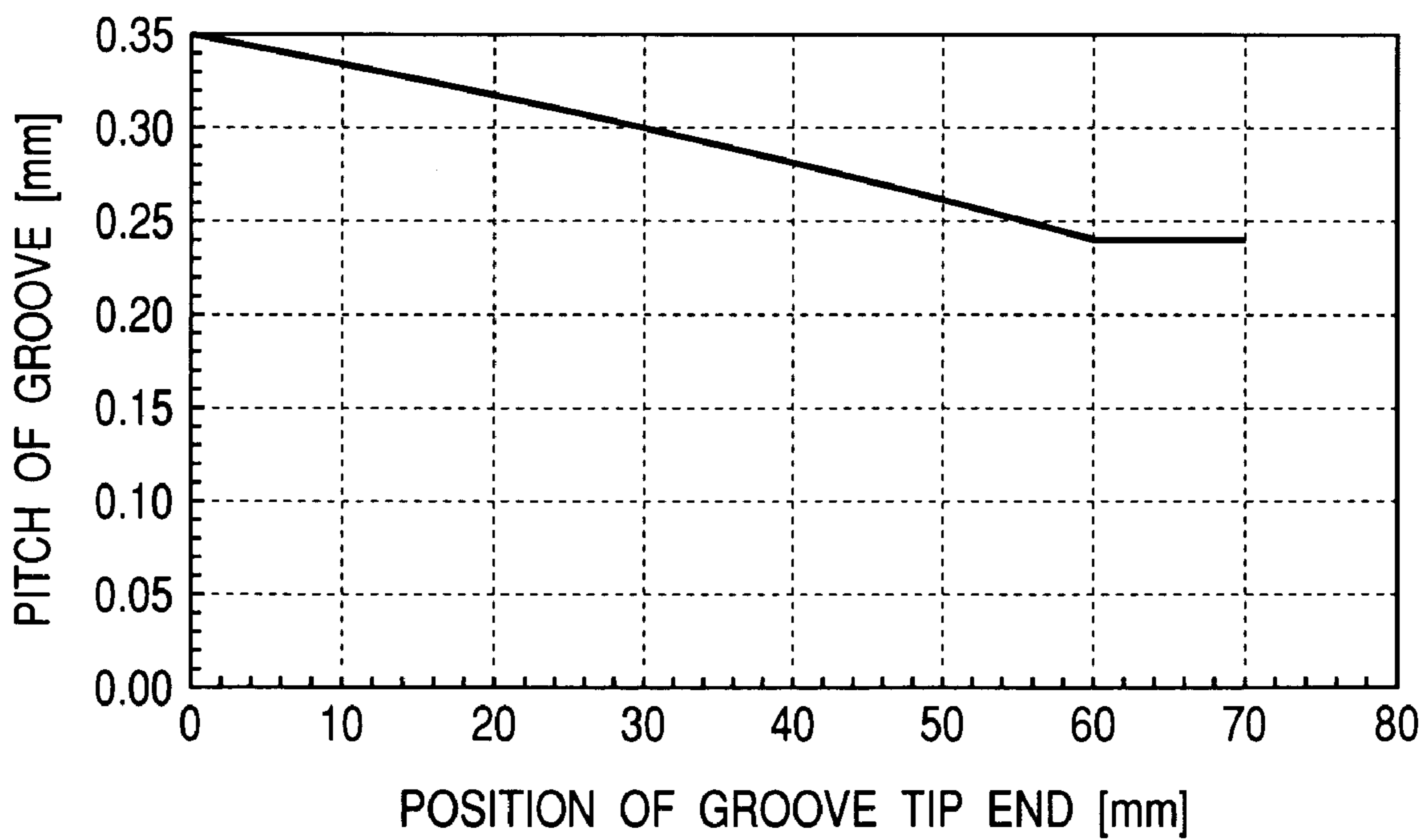
POSITION OF GROOVE TIP END VS PITCH
