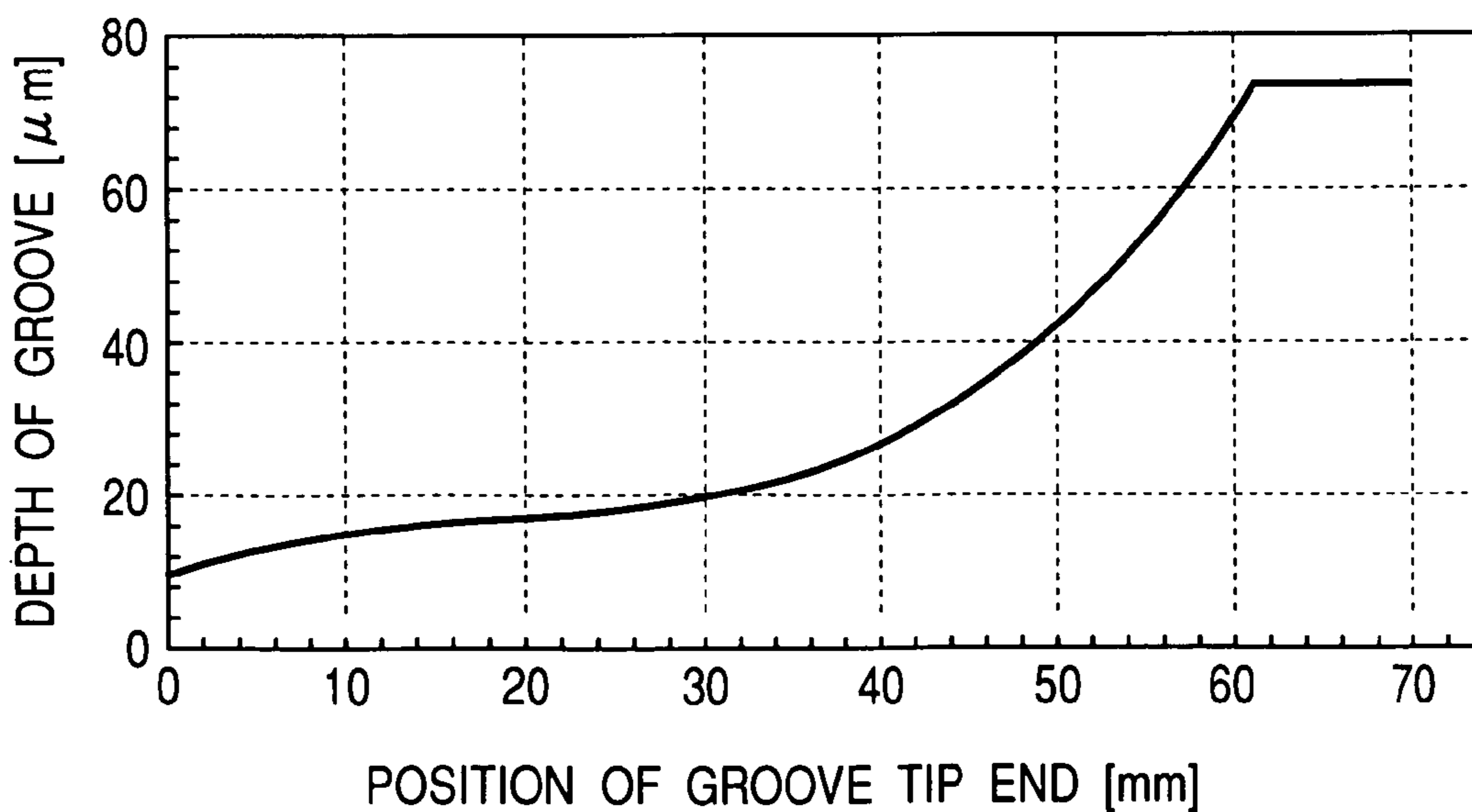
POSITION OF GROOVE TIP END VS DEPTH OF GROOVE
