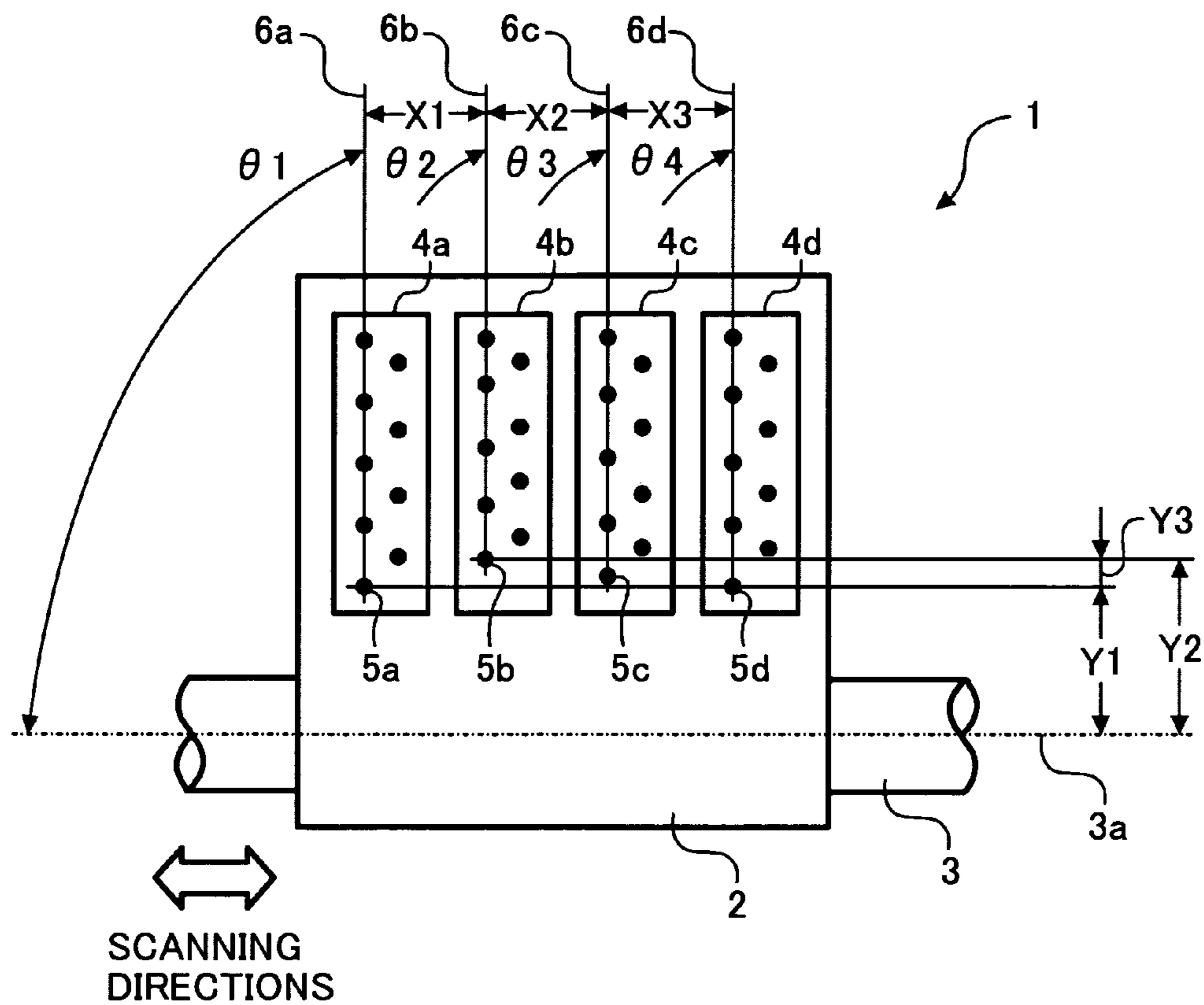
FIG. 1 PRIOR ART
