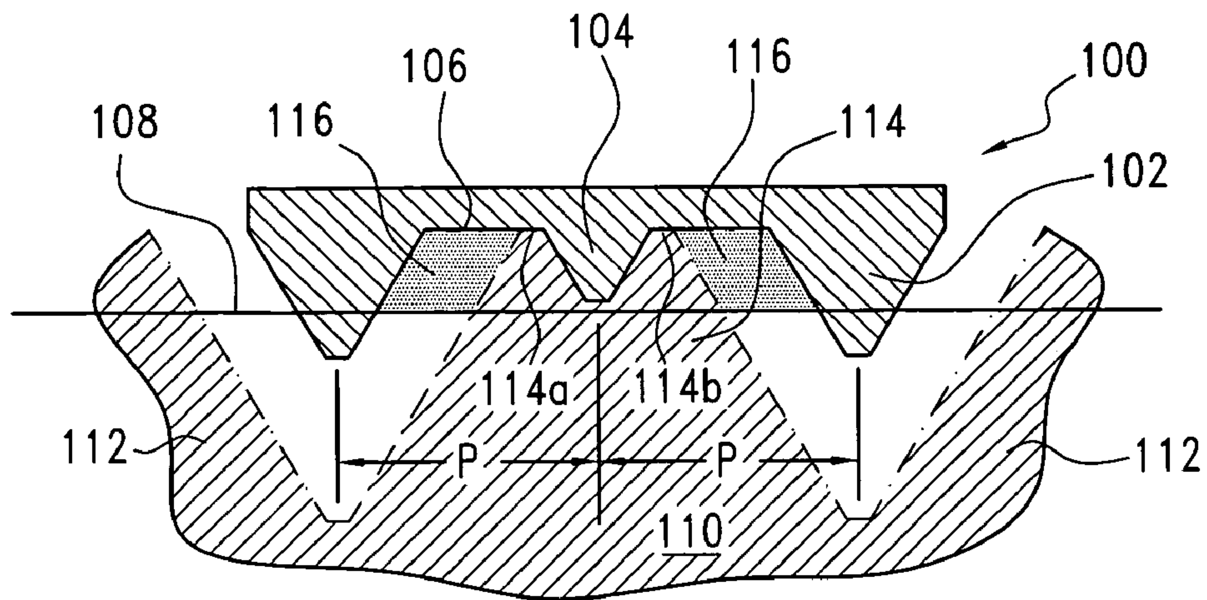
FIG. 4 (PRIOR ART)
