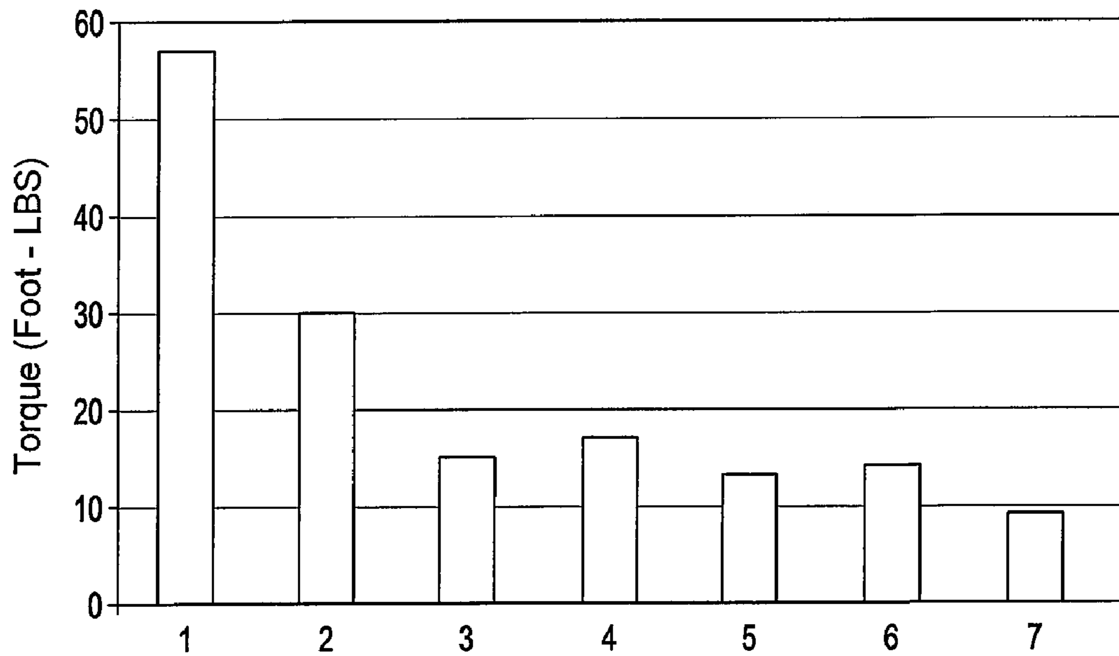
Grip breakaway torque at 1 minute
