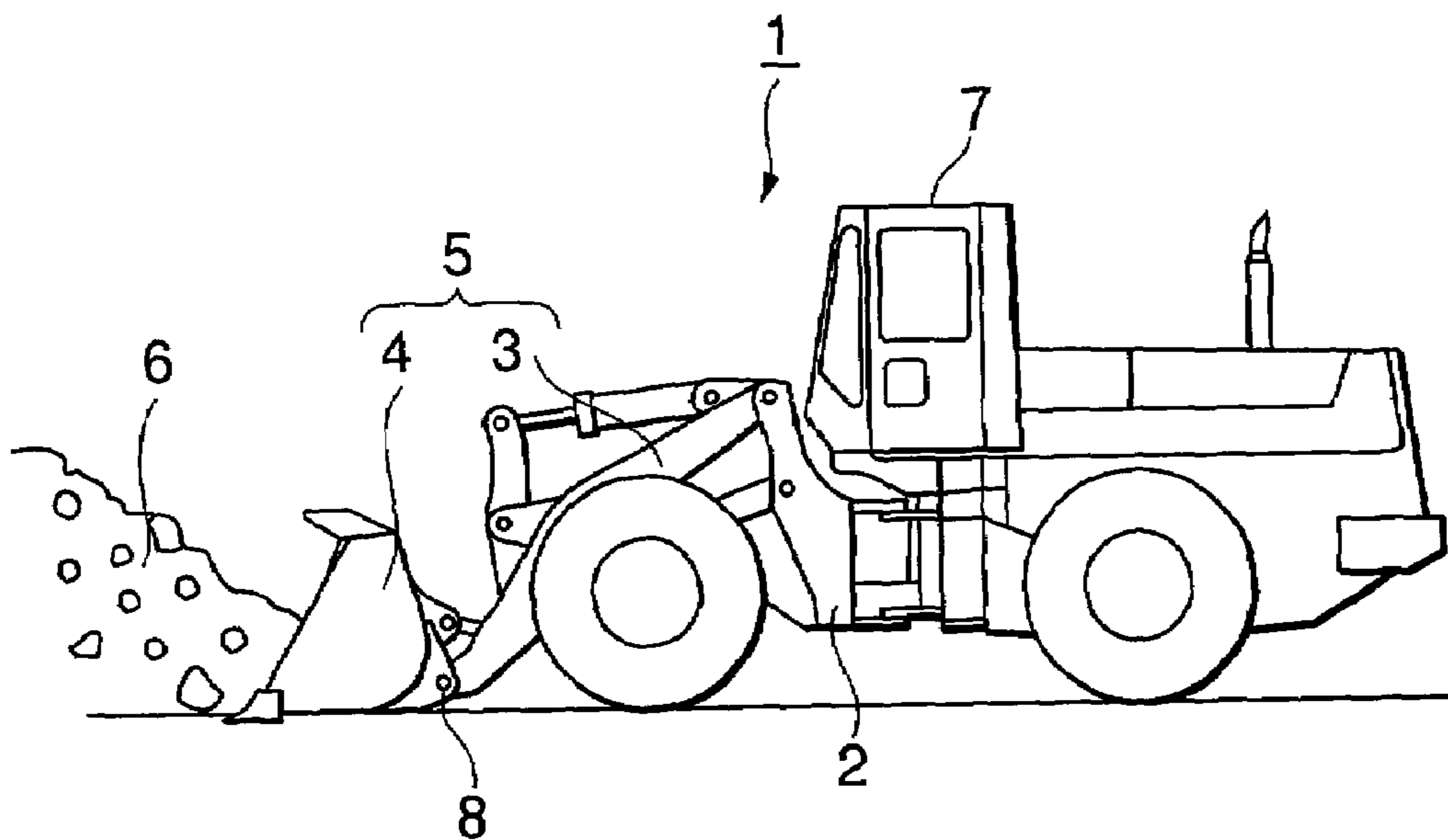
FIG.10 PRIOR ART
