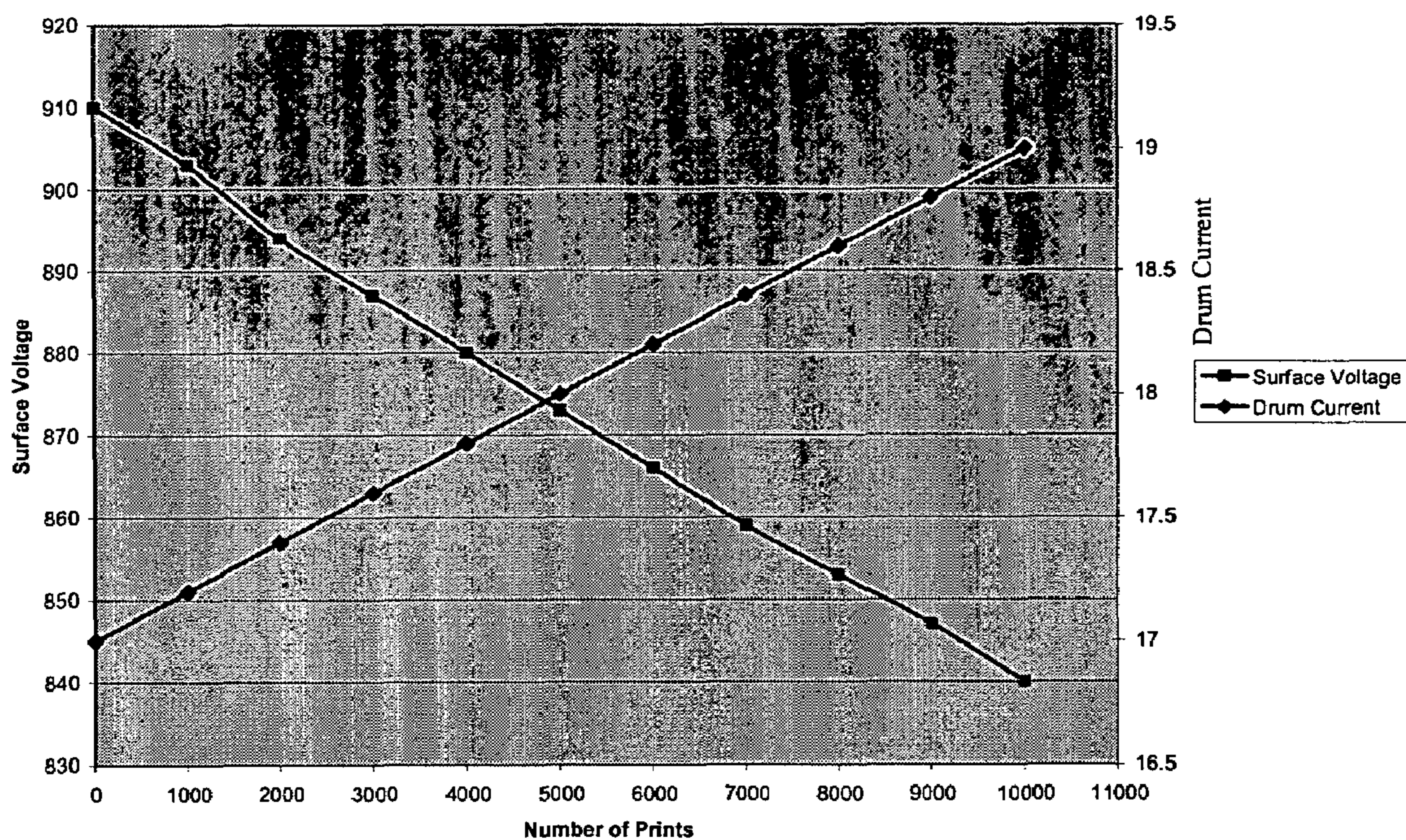
Drum Characteristic vs. Printing with Charge Device Voltage = 1.5KVDC
