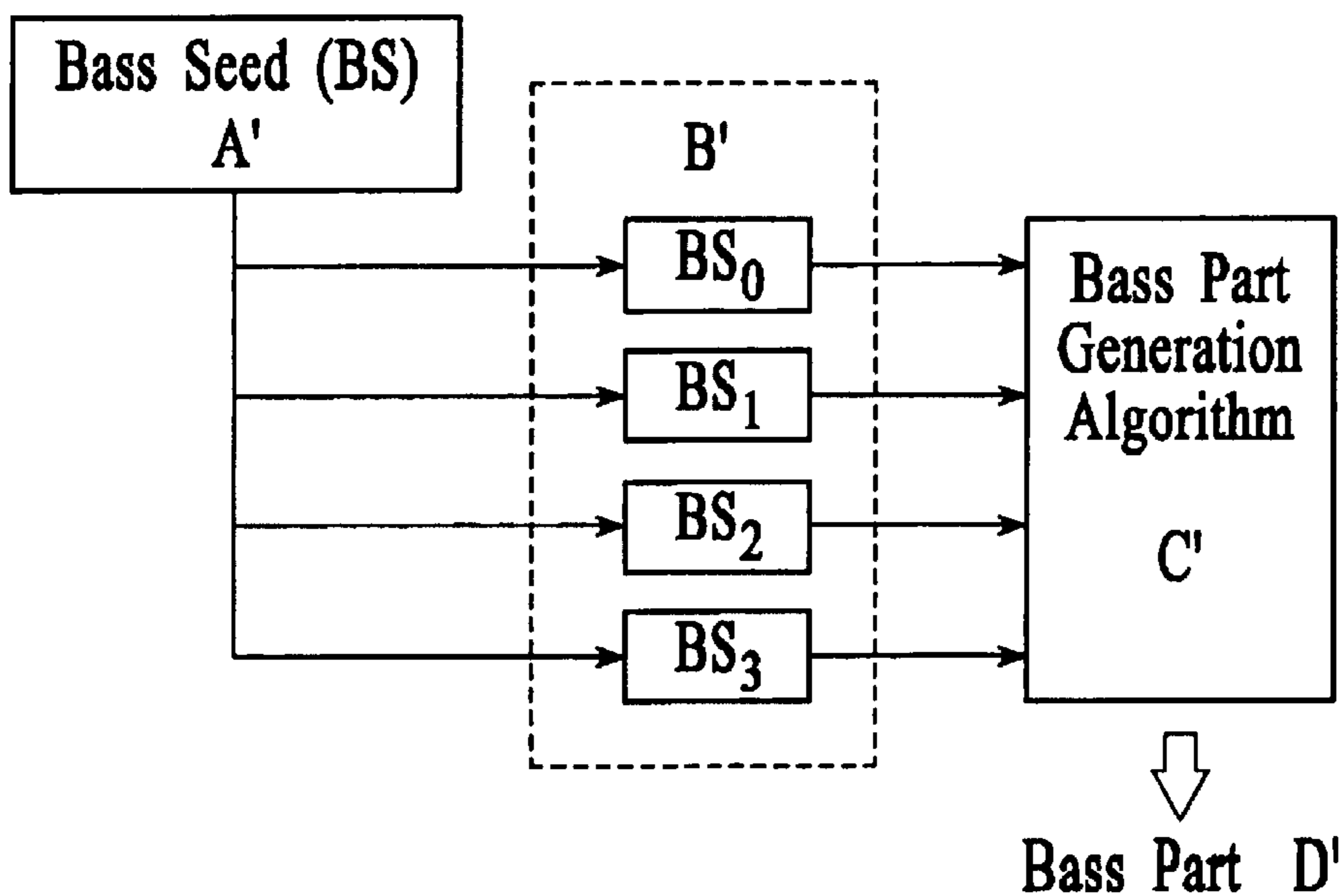
Pseudo-Random Number Implementation 2
