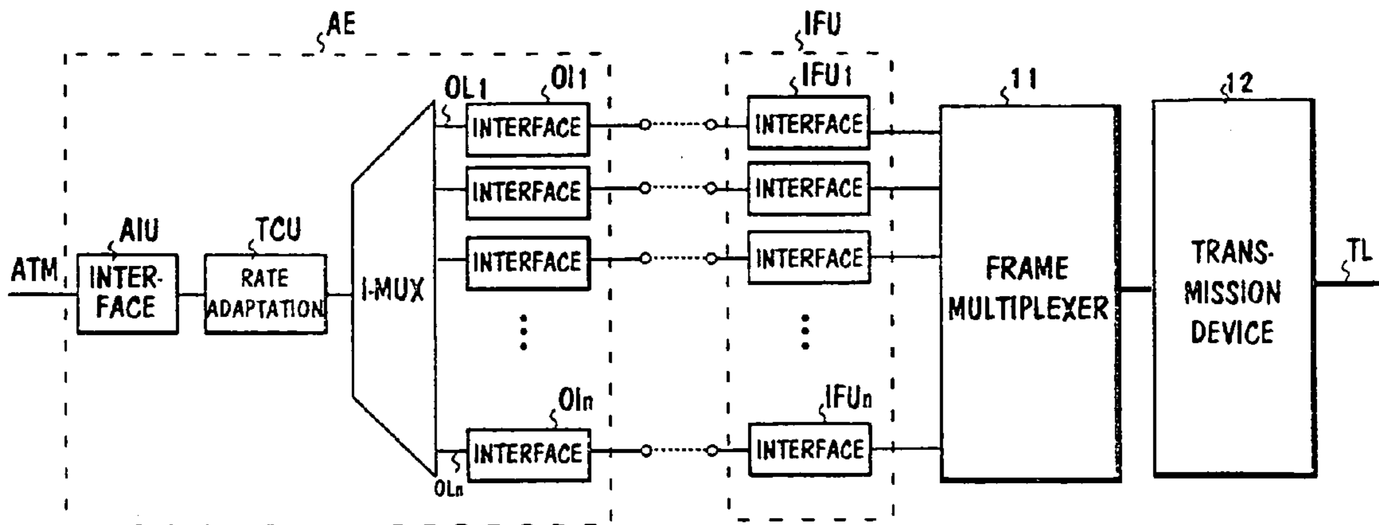
FIG. 3 PRIOR ART
