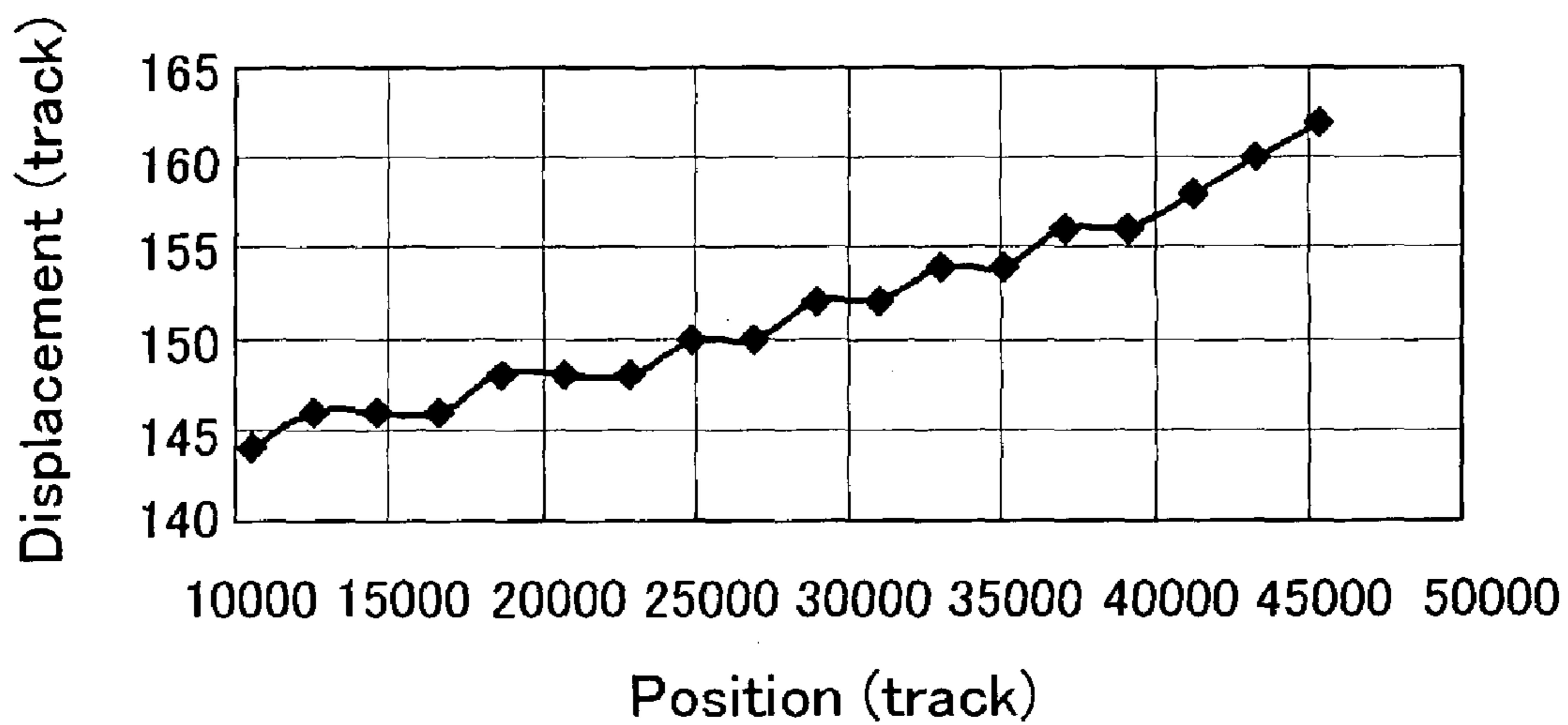
Head3 TrackDiff
