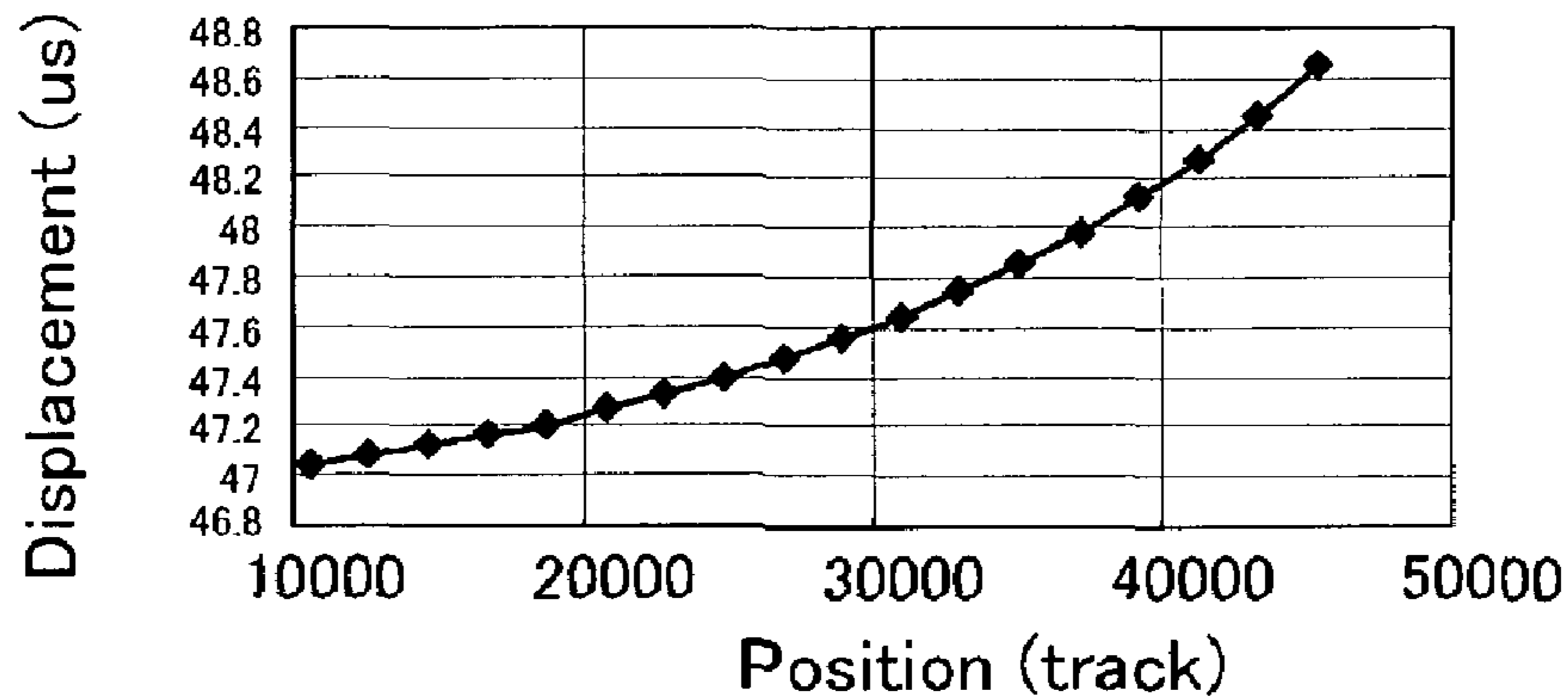
Head0 TimeDiff Ave
