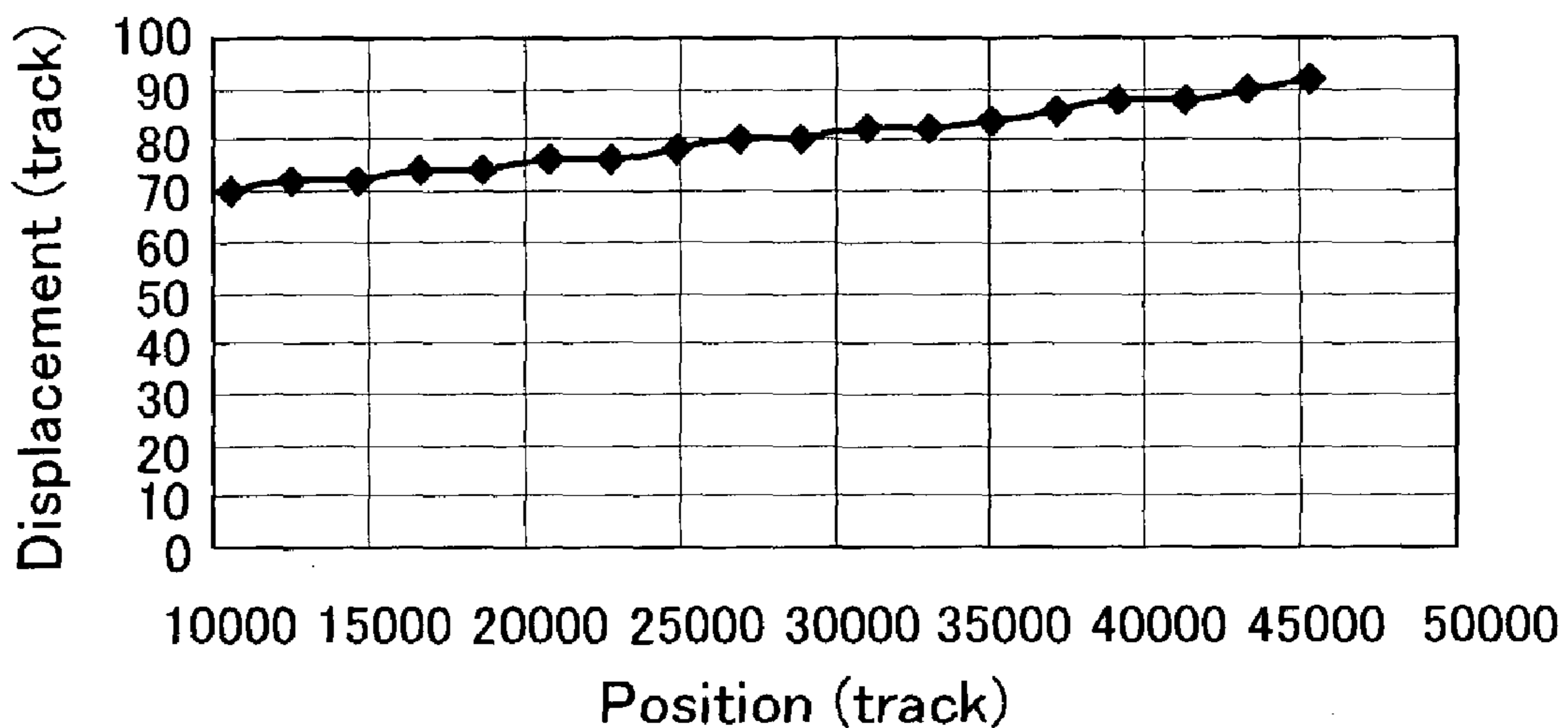
Head2 TrackDiff
