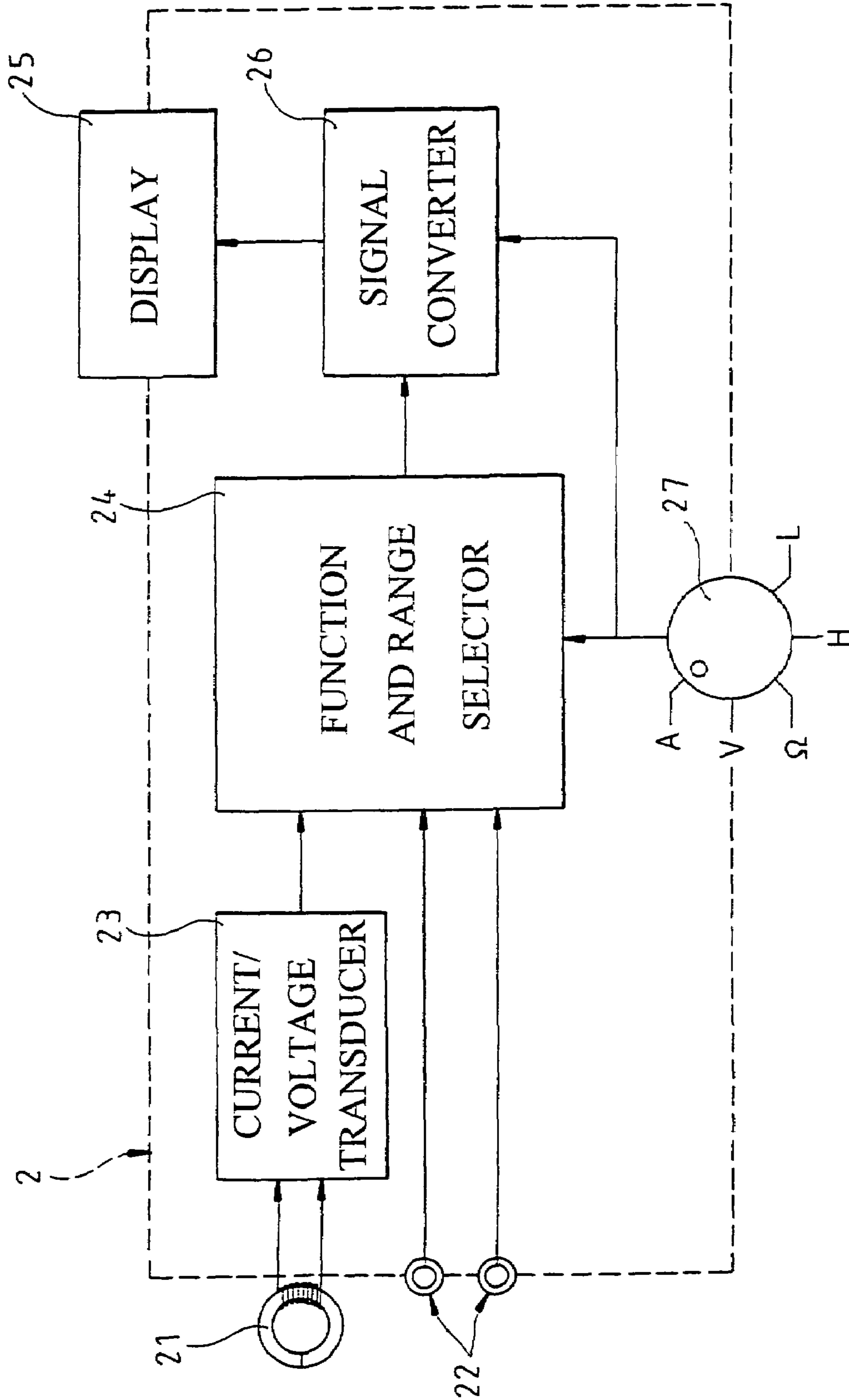
FIG. 2 (PRIOR ART)
