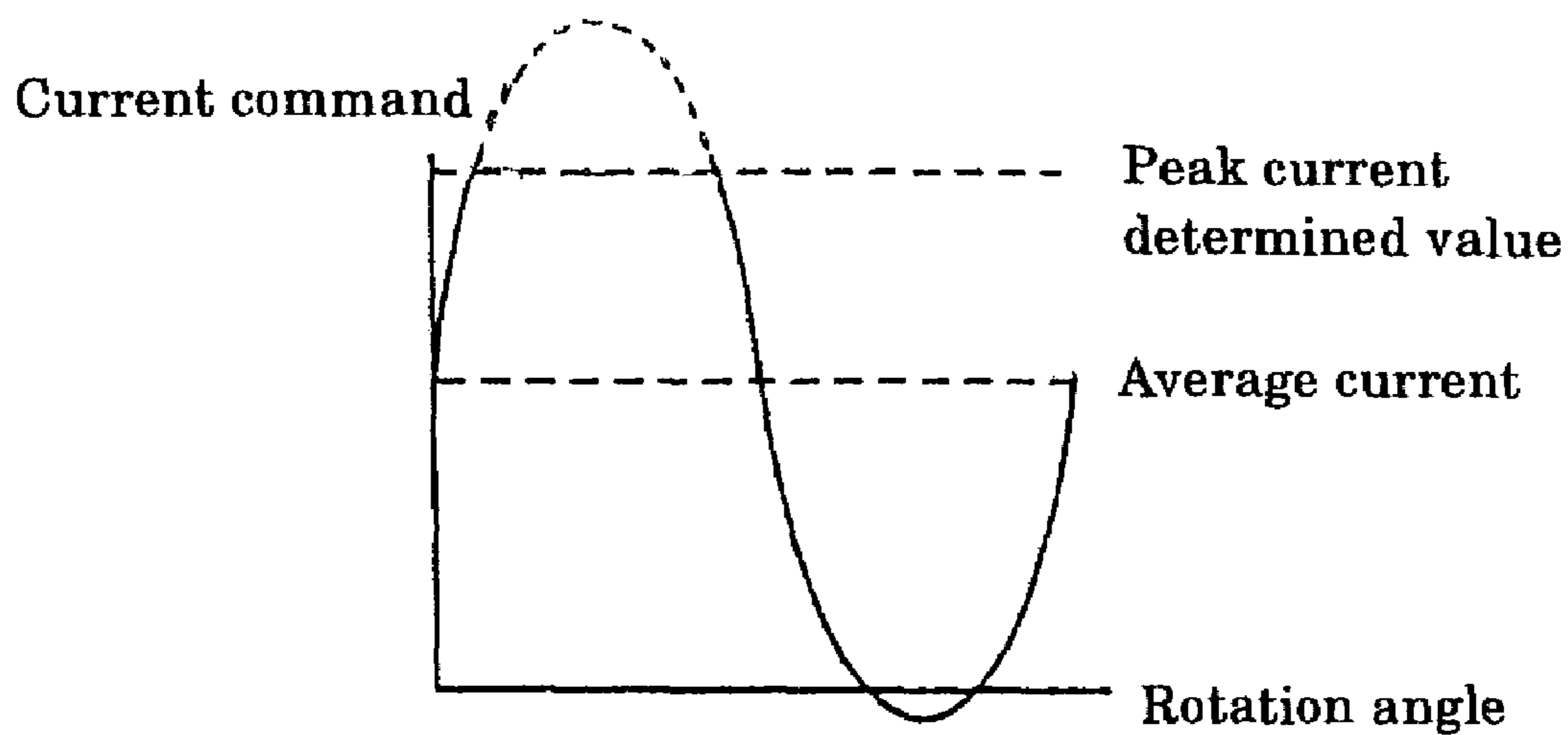
(B) Clipped current command
