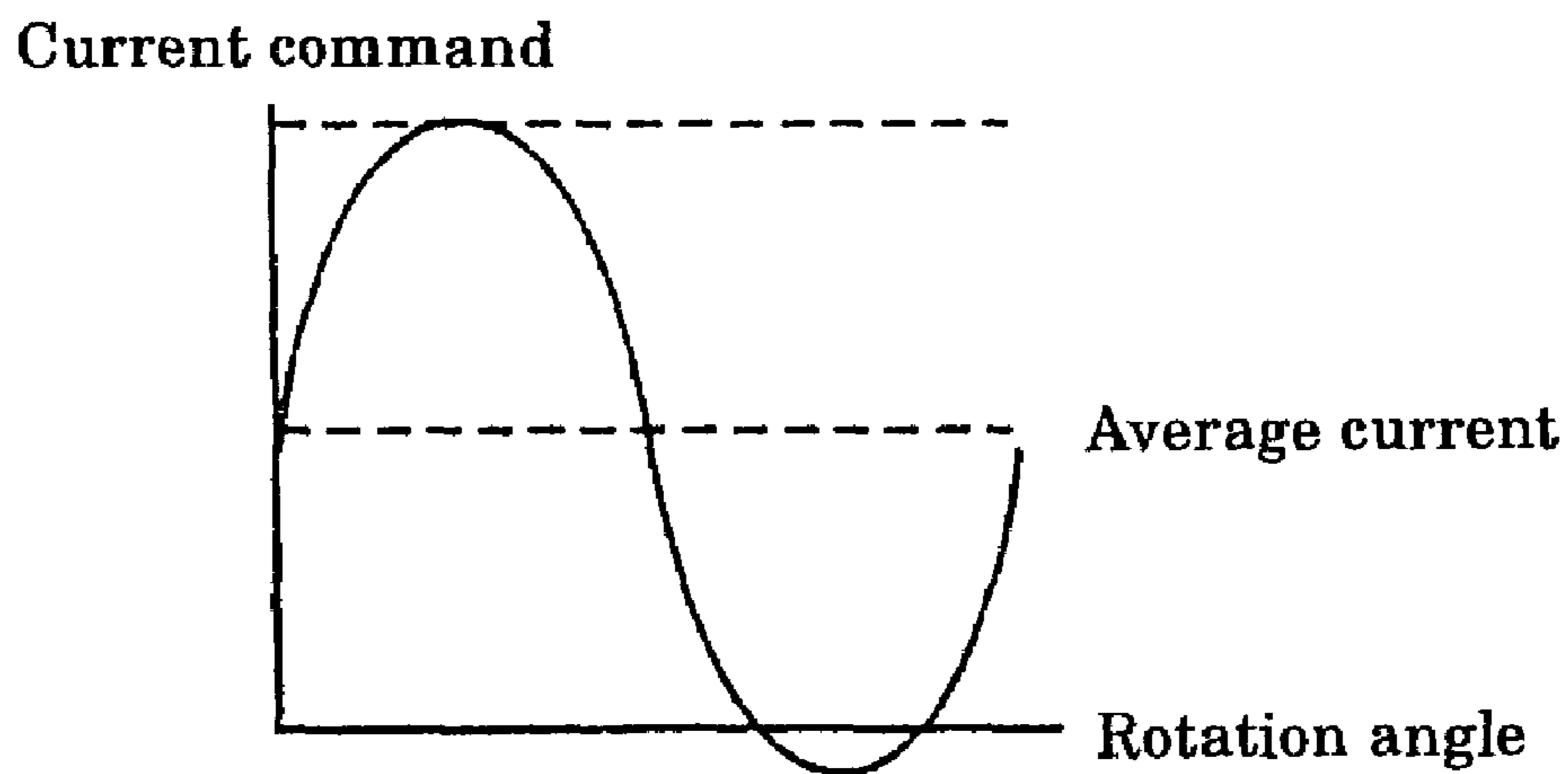
(A) Ordinary current command
