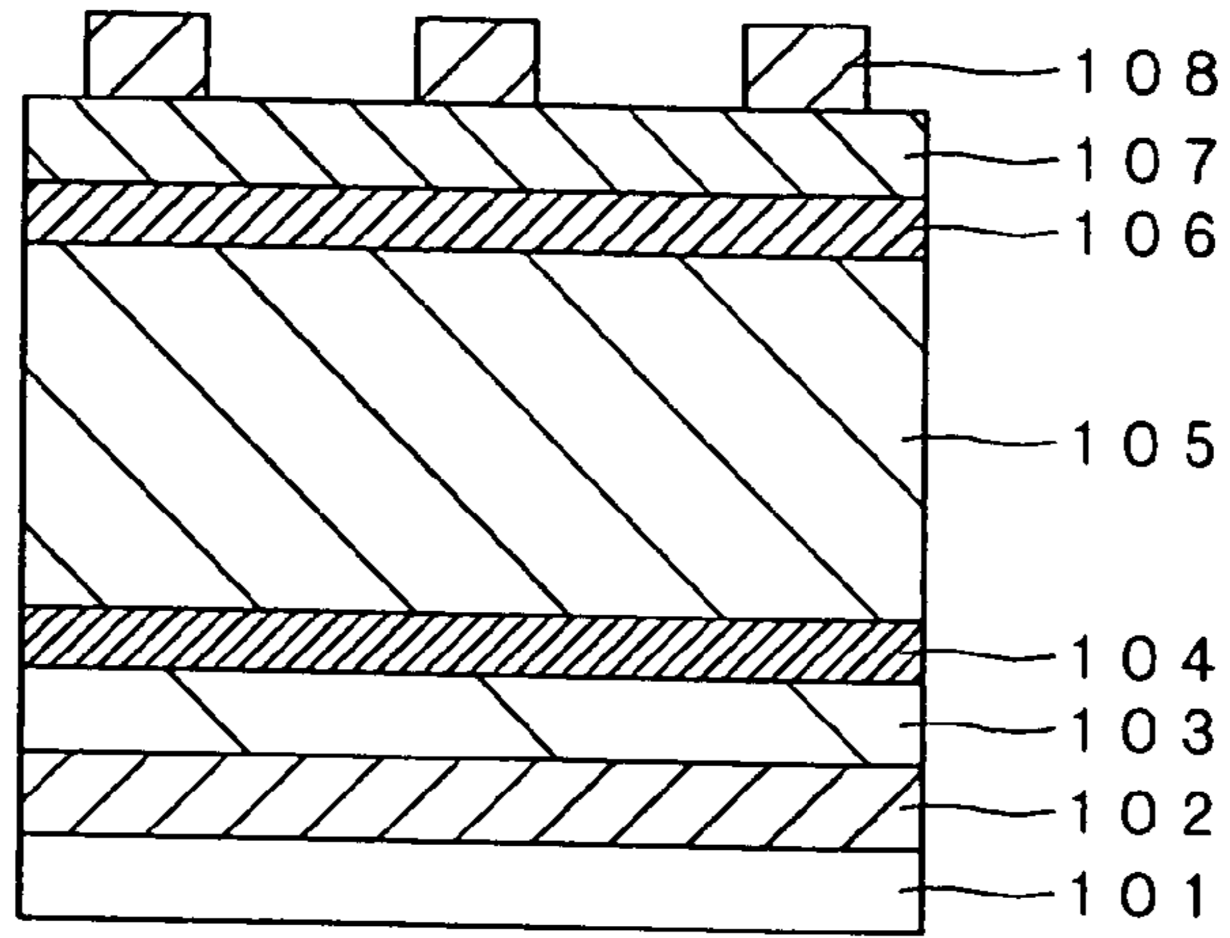
FIG.6 PRIOR ART
