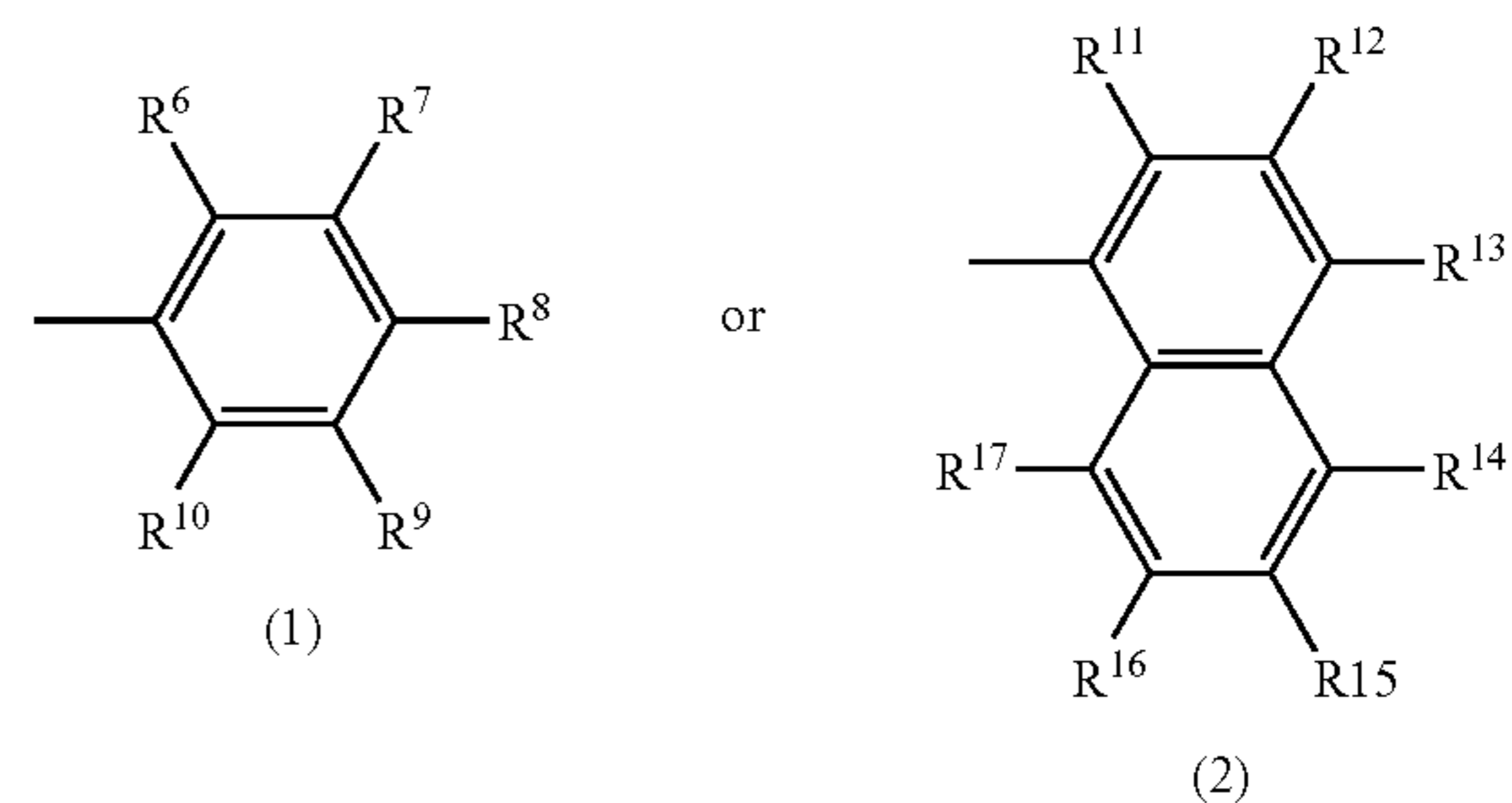
General Formula (7)
