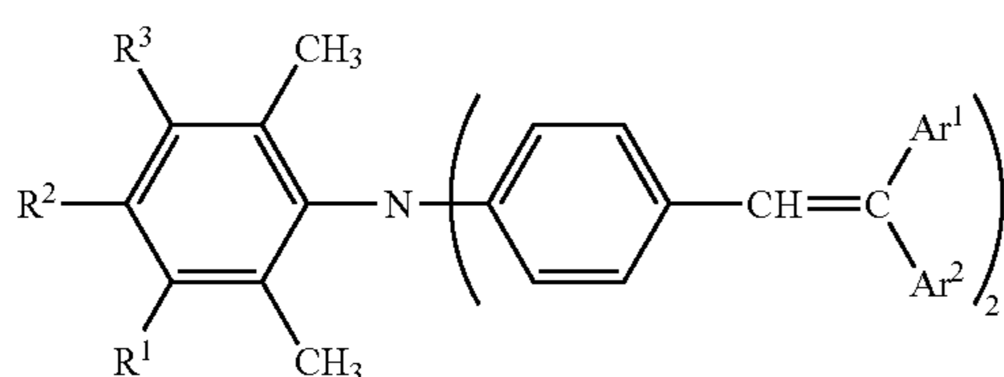
General Formula (4)
