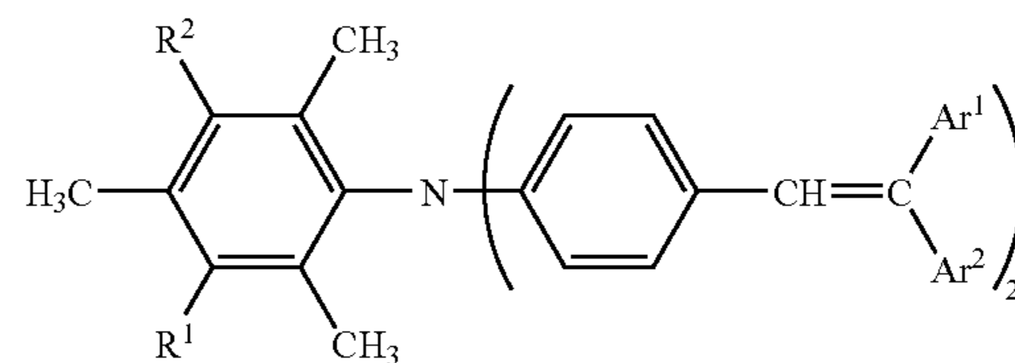
General Formula (6)
