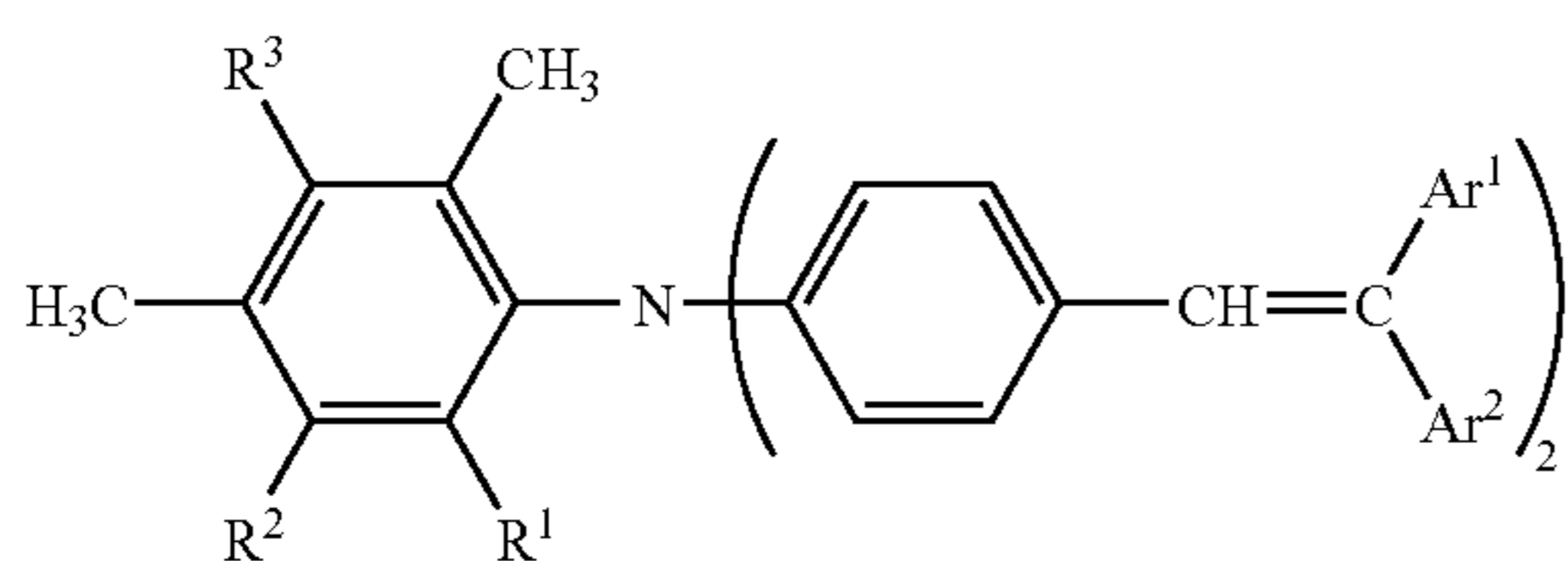
General Formula (5)
