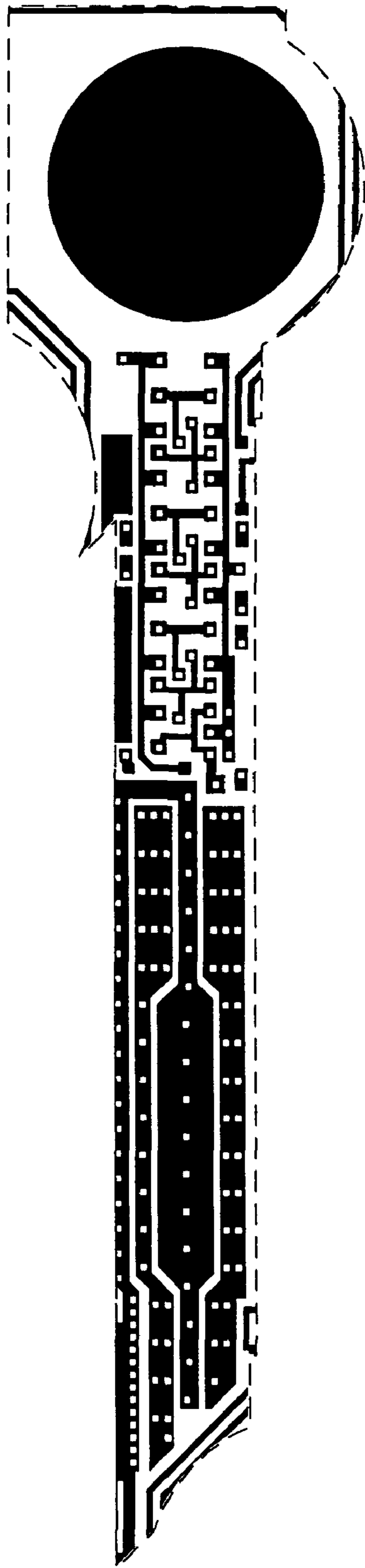
Metal 1 mask
