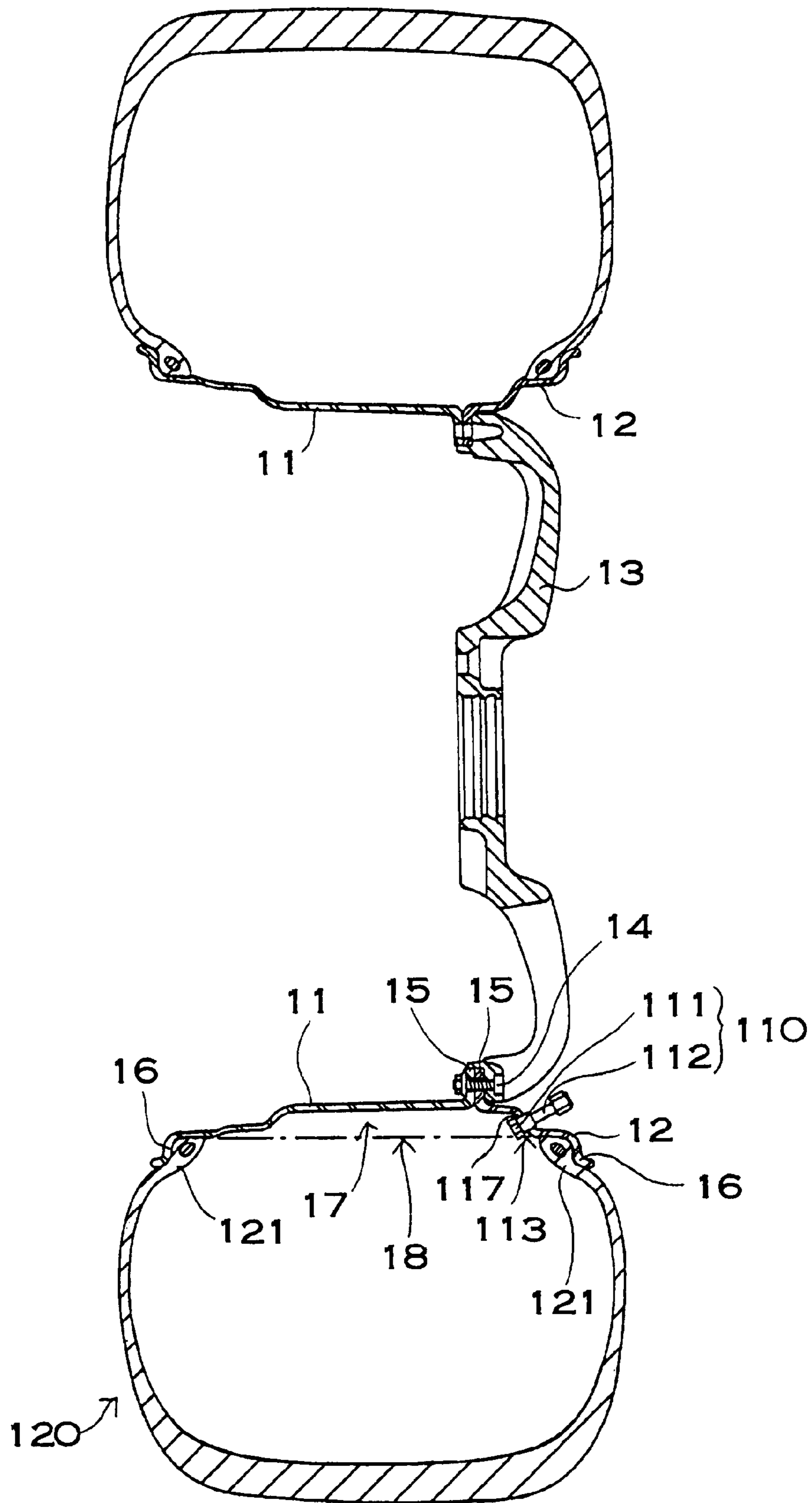
FIG. 1 PRIOR ART
