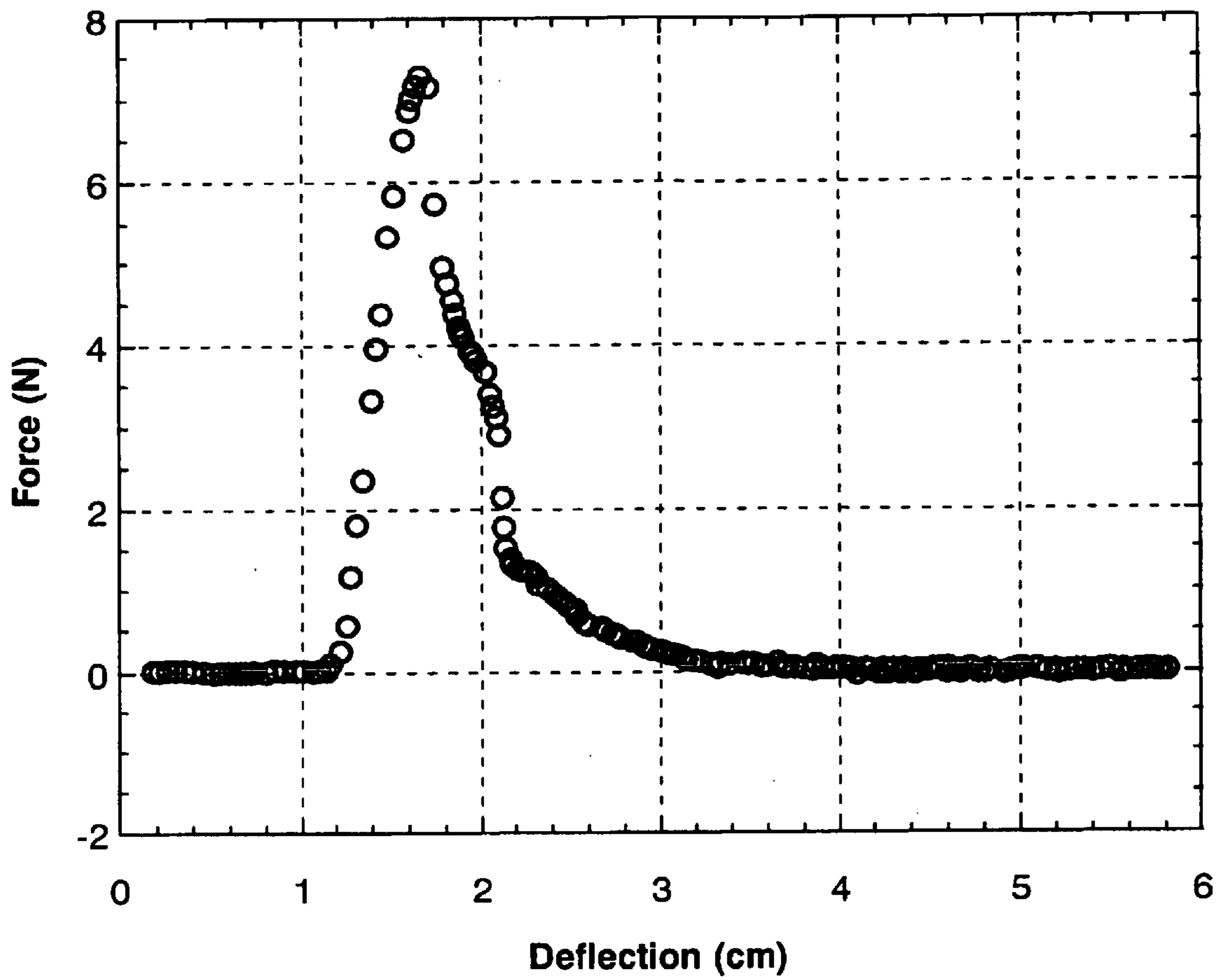
Force-Deflection Curve
