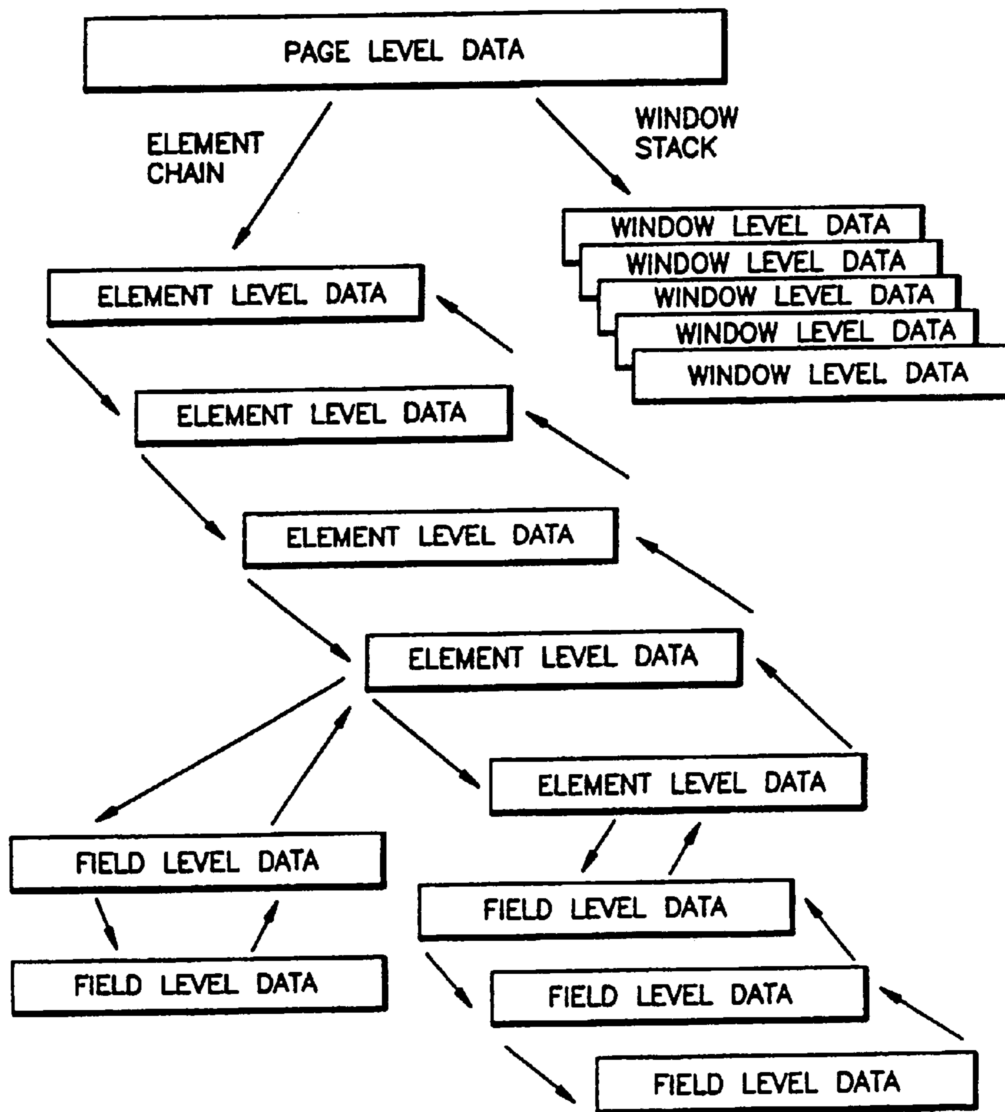
FIG. 10 PAGE PROCESSING TABLE (ppt)
