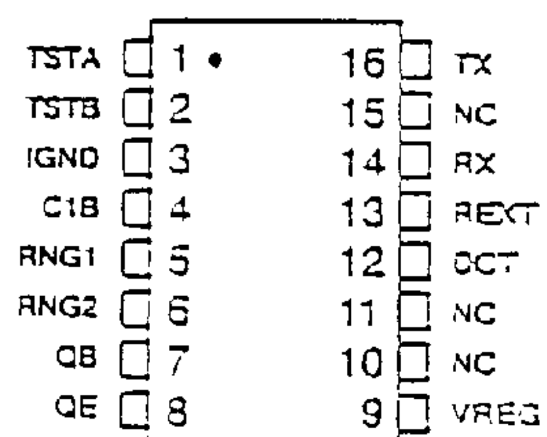
Figure 17. Si3032B Pin Configuration
