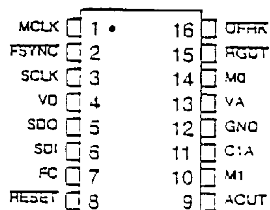
Figure 16. Si3032A Pin Configuration
