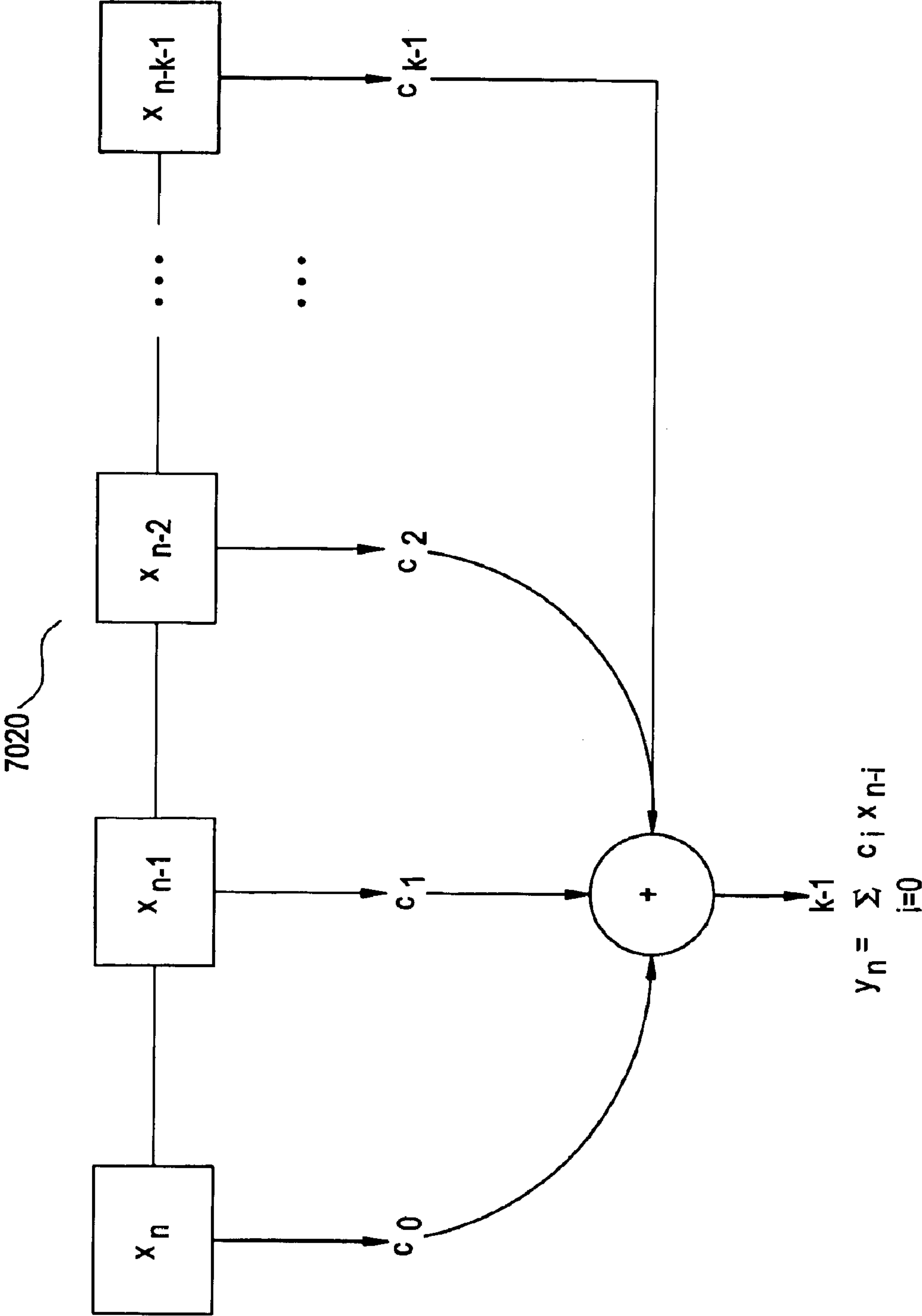
FIG. 72 PRIOR ART
