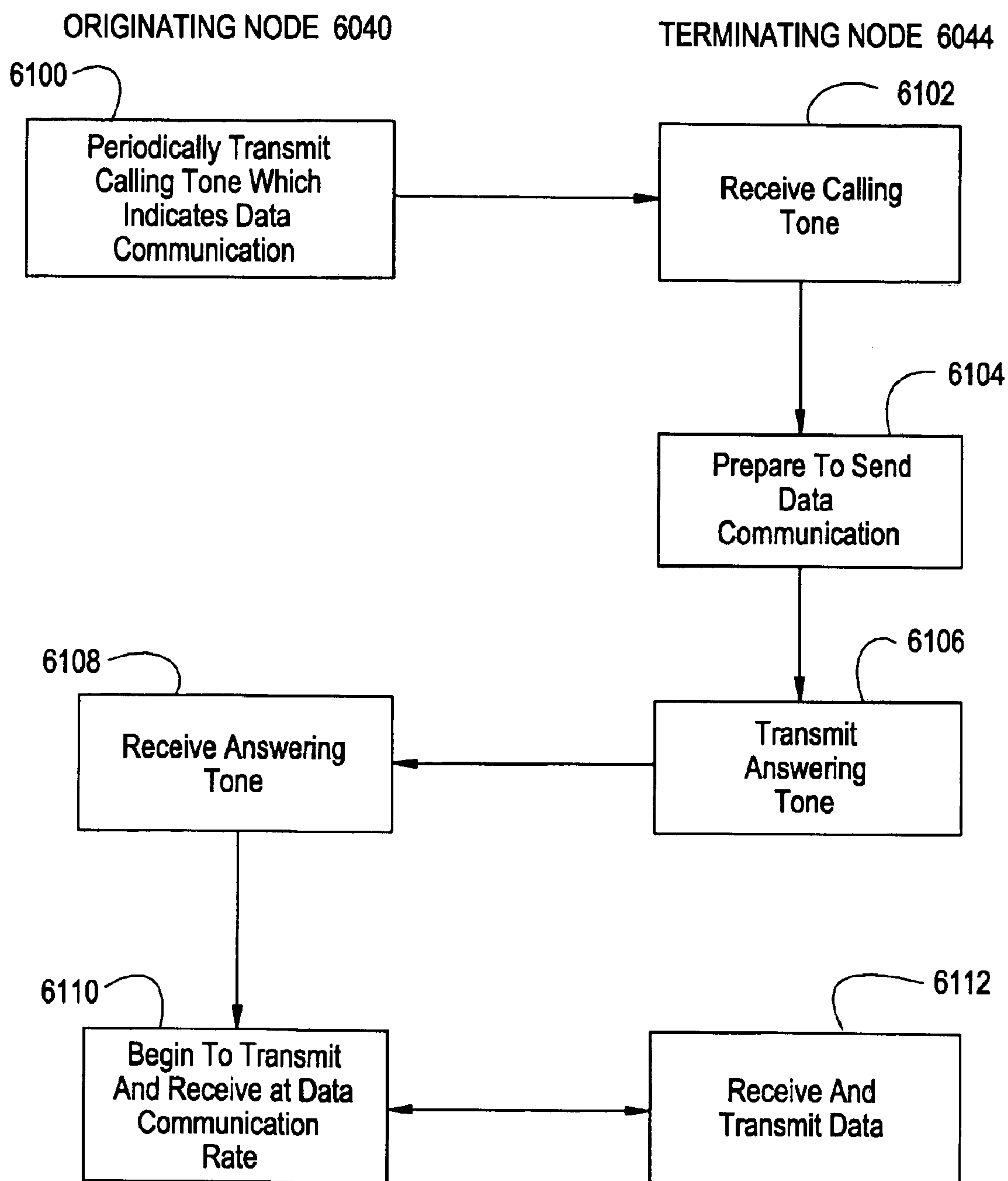
FIG. 69 PRIOR ART
