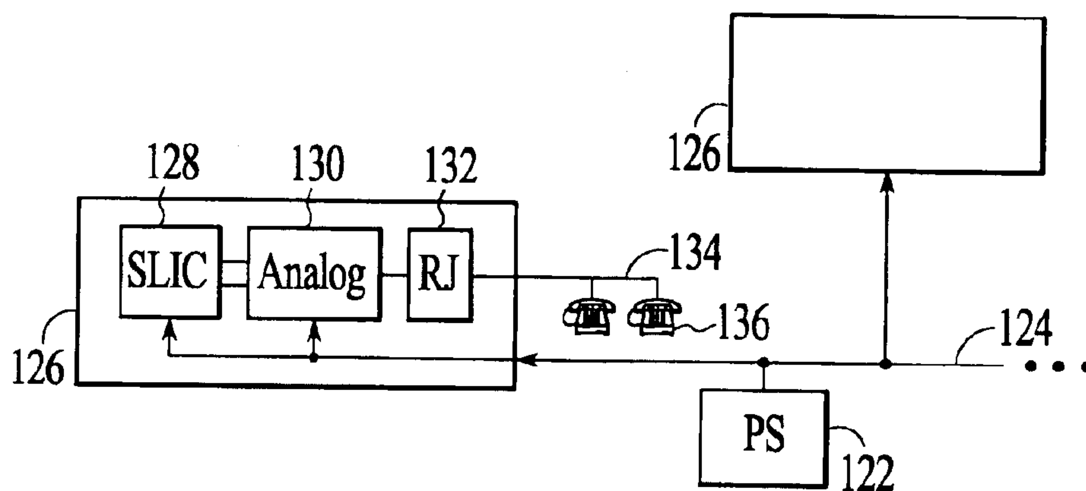
FIG. 7 (PRIOR ART)
