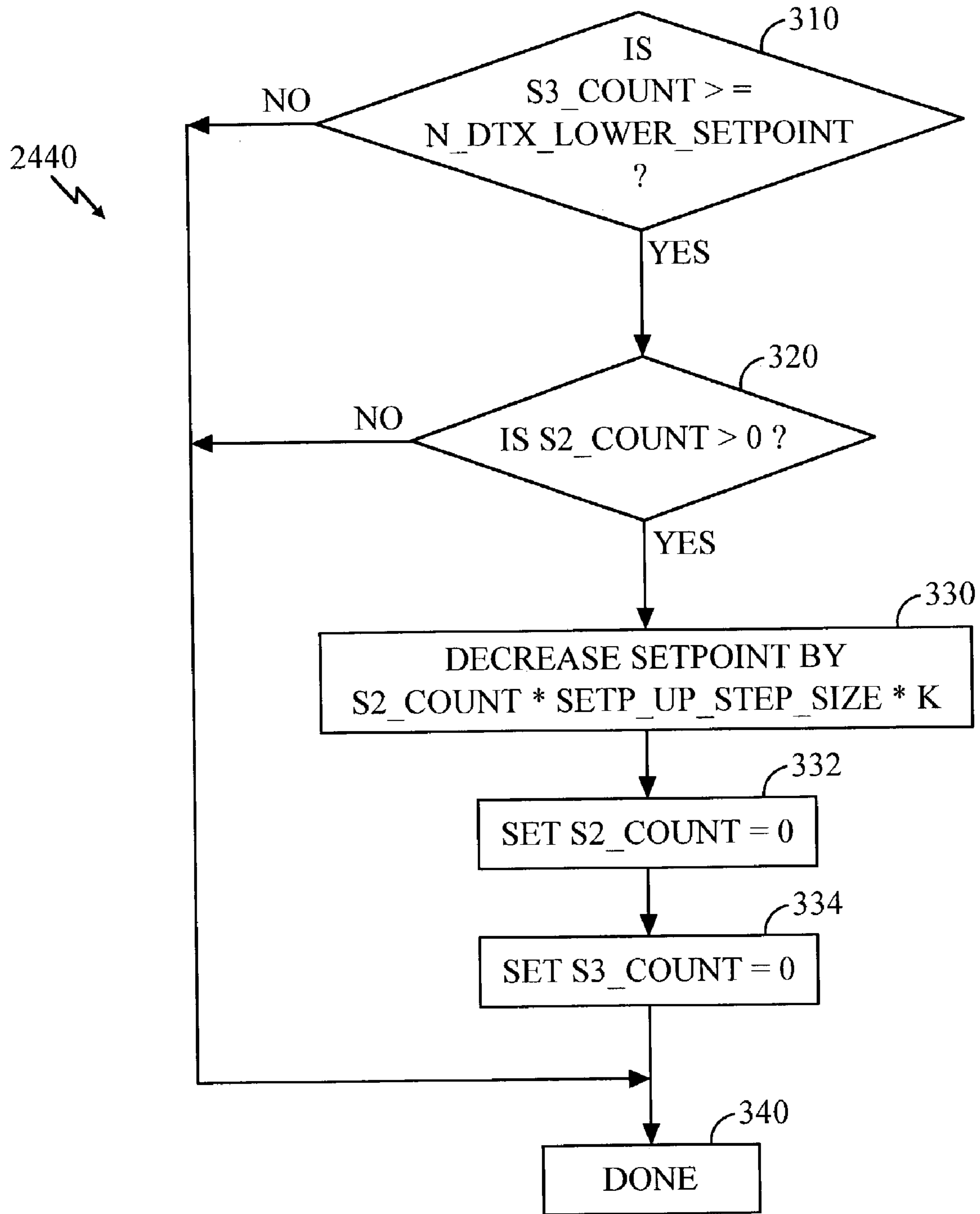
S3_COUNT COMPENSATION
