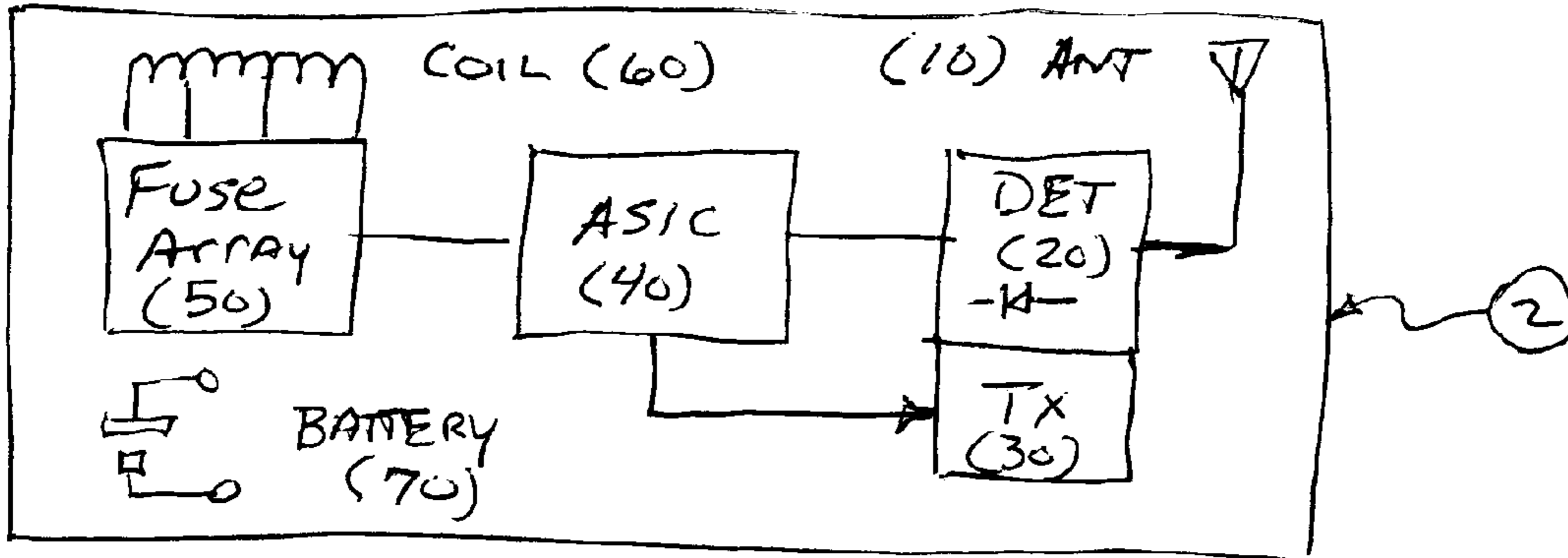
FAULTED Circuit Monitor (FCM) FIG 2
