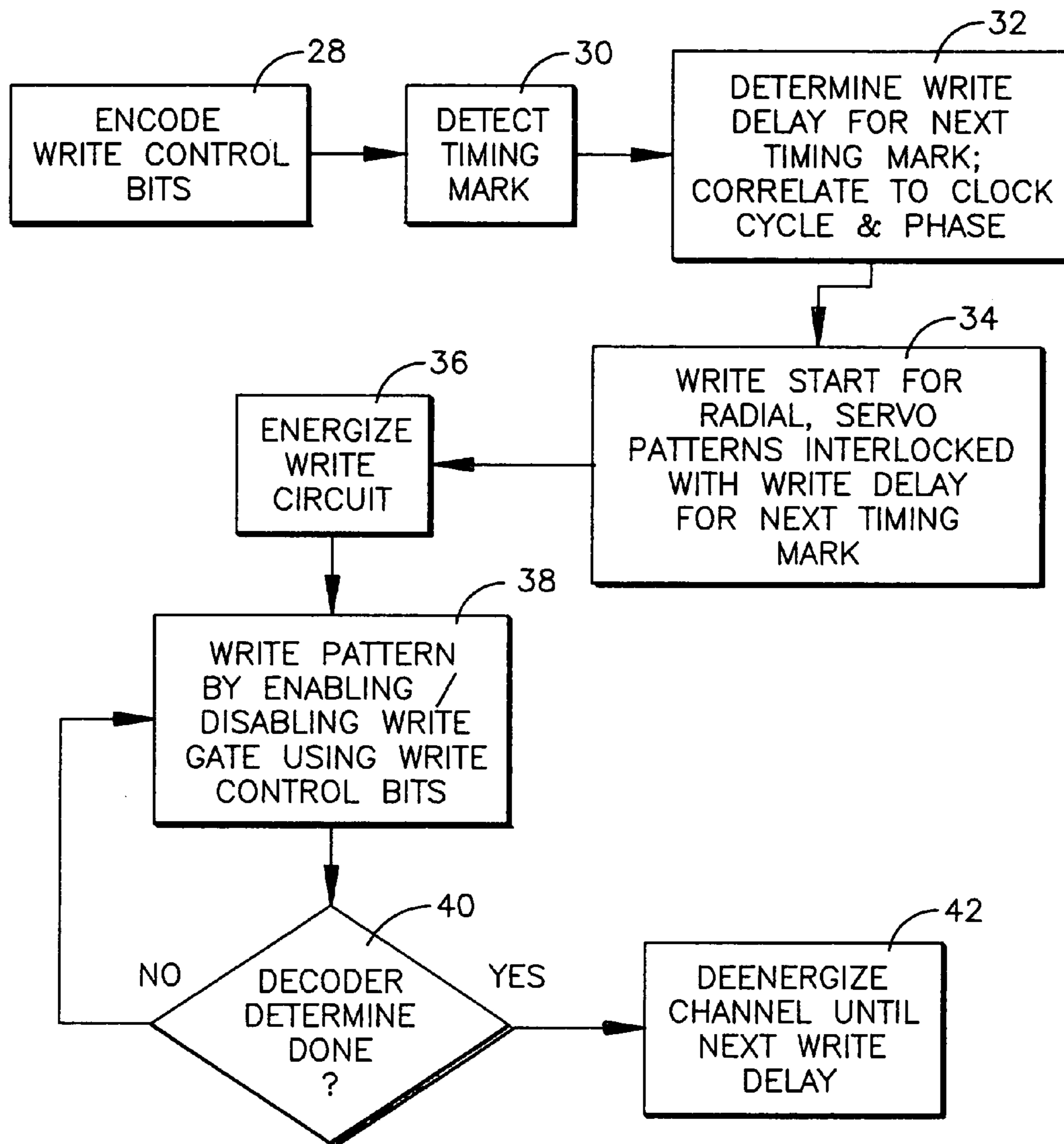
Fig. 3 LOGIC
