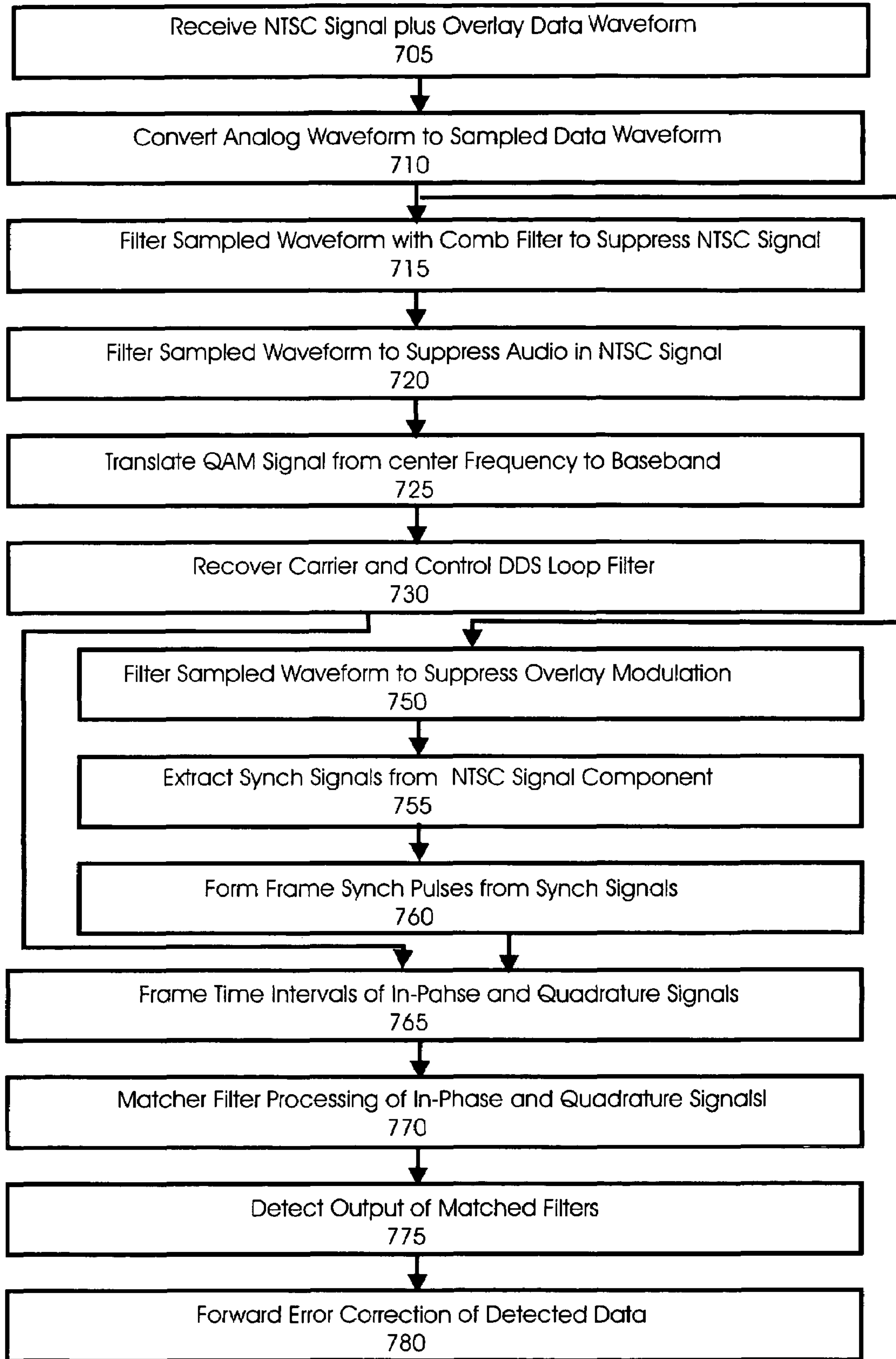
Figure 14. Signal Processing Flow through Demodulator
