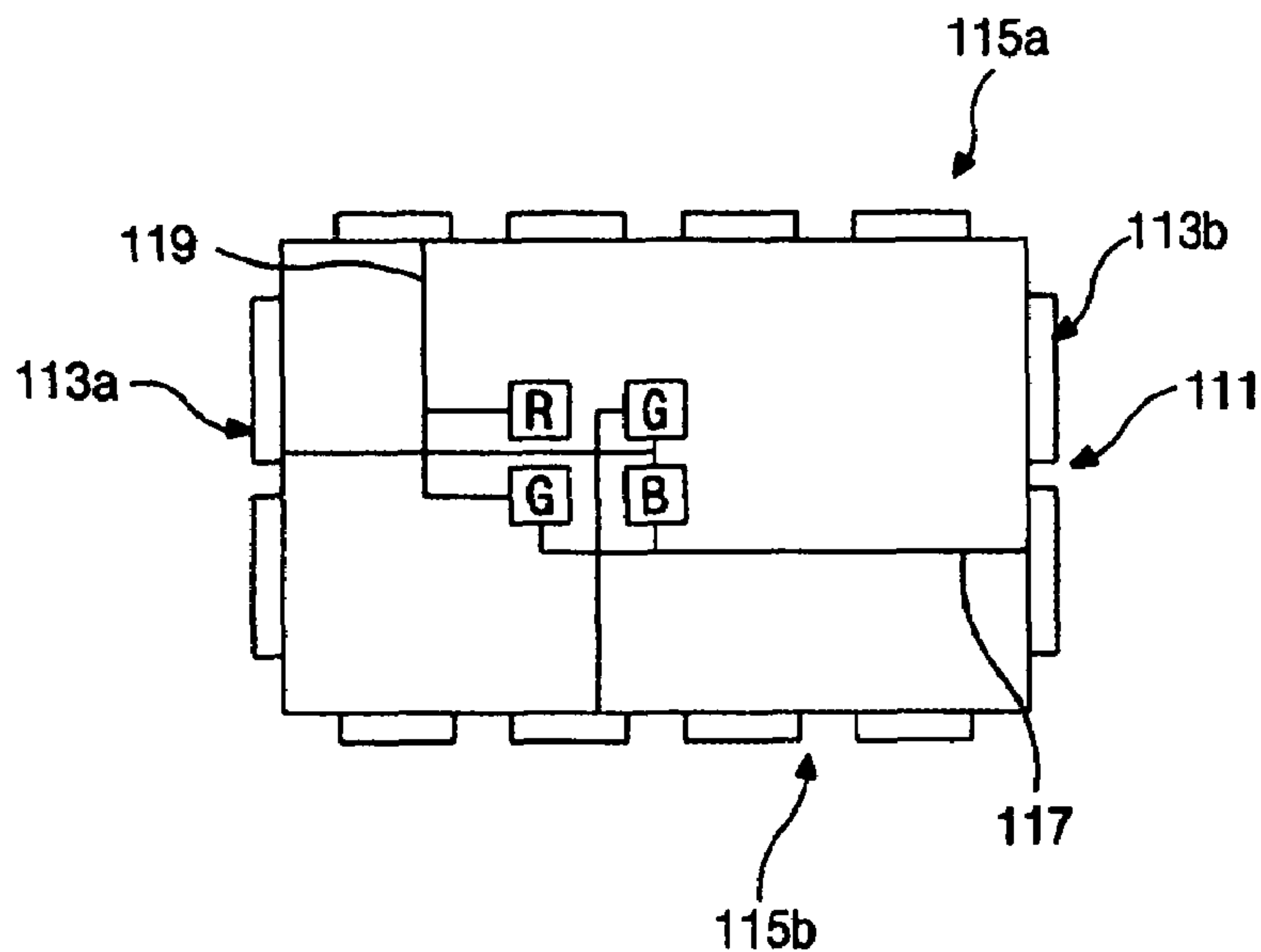
(RELATED ART) FIG. 3
