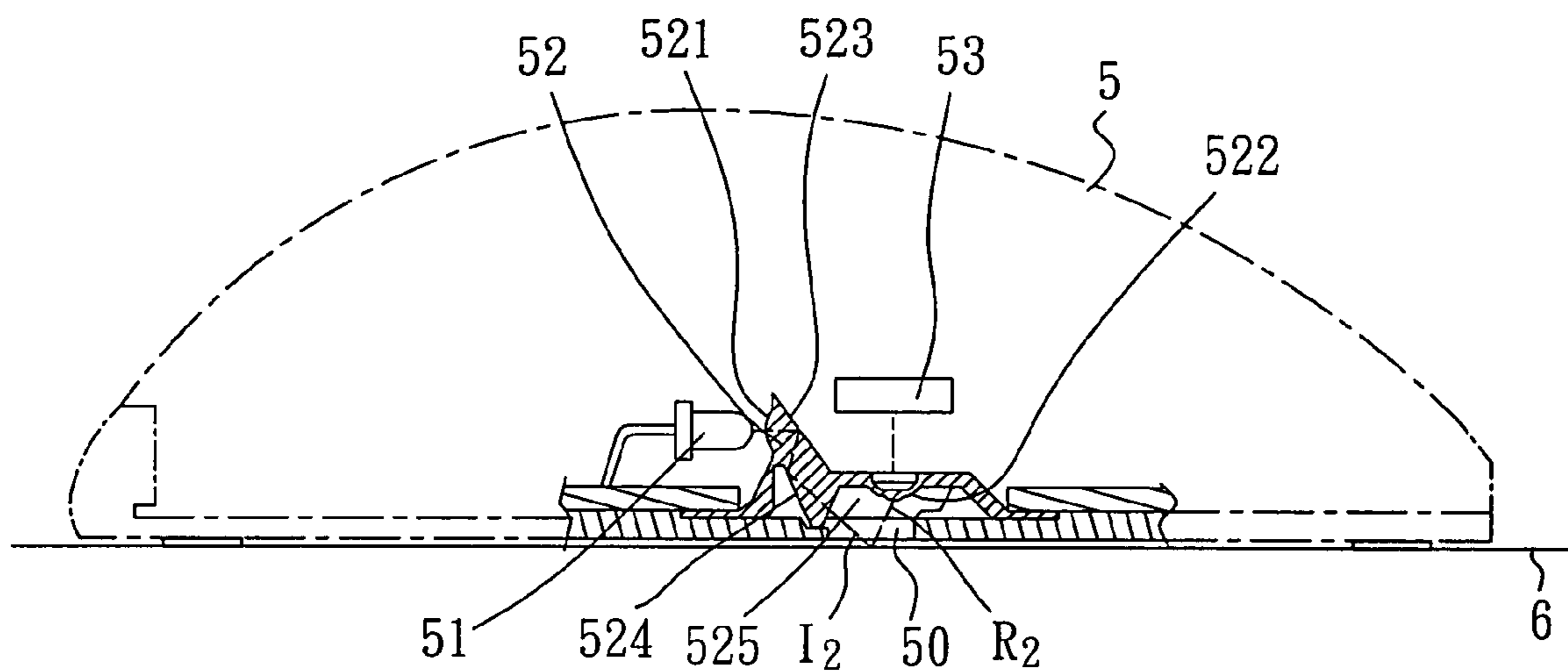
FIG. 1 (PRIOR ART)
