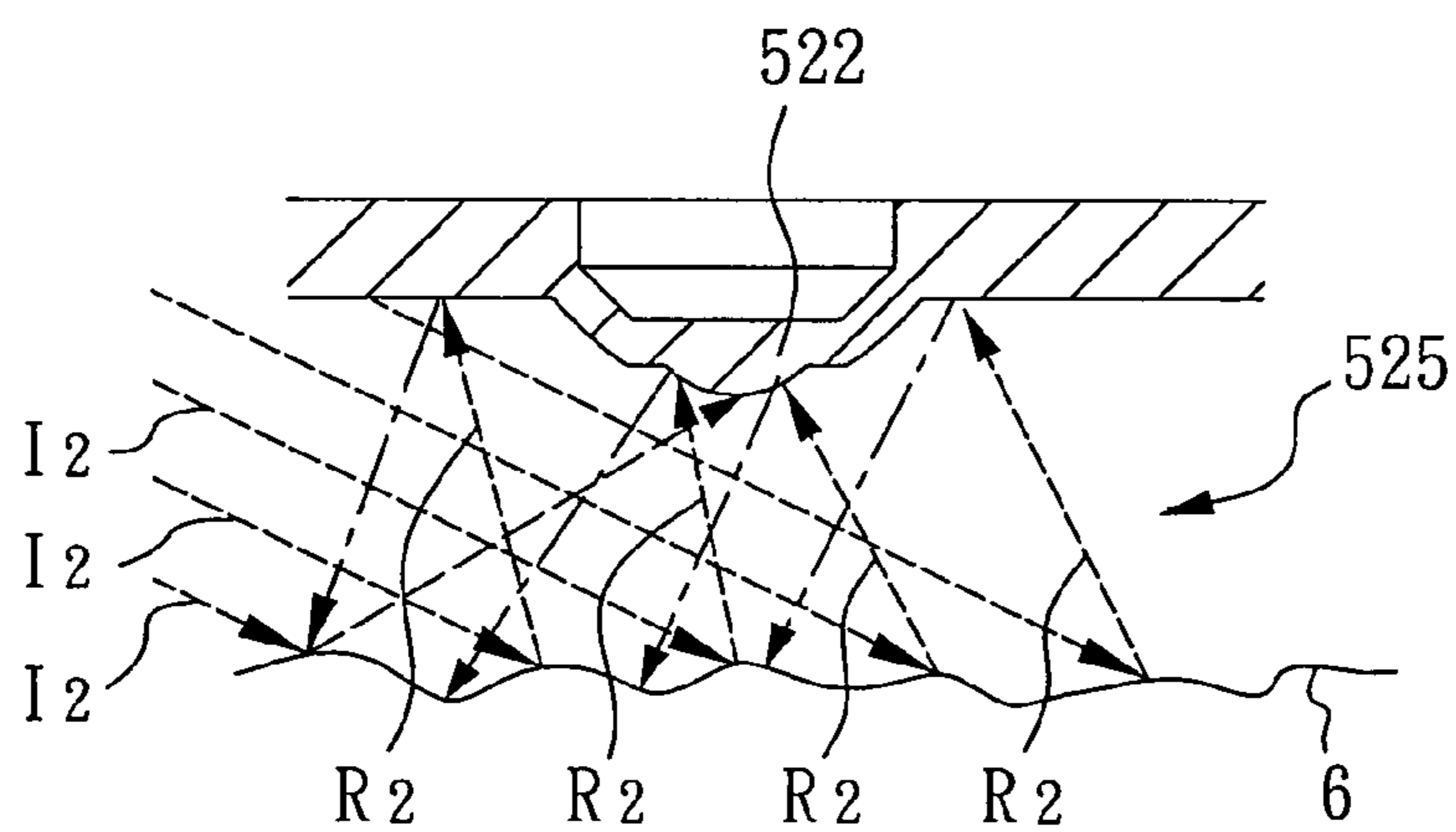
FIG. 2 (PRIOR ART)
