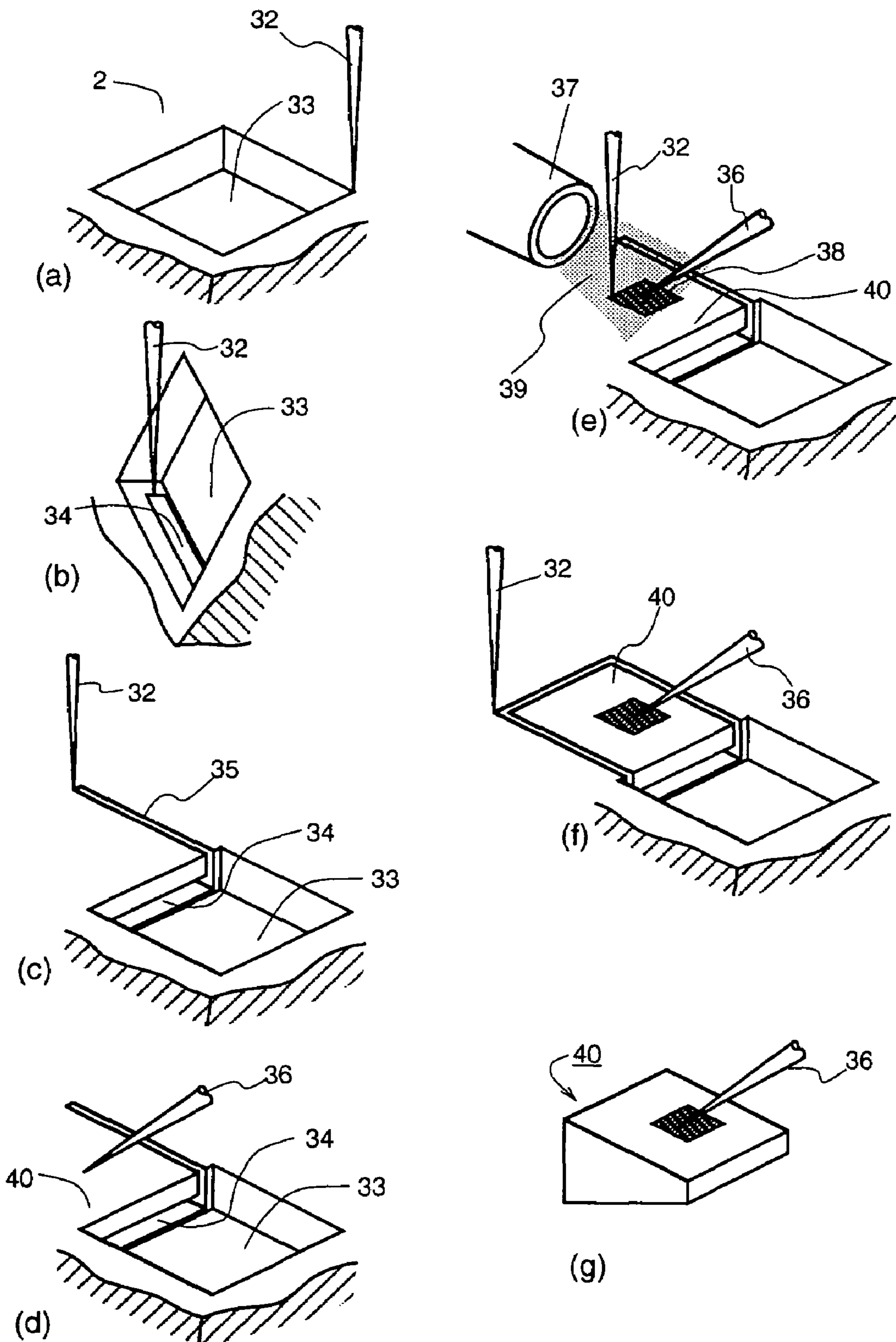
FIG.4 (PRIOR ART)
