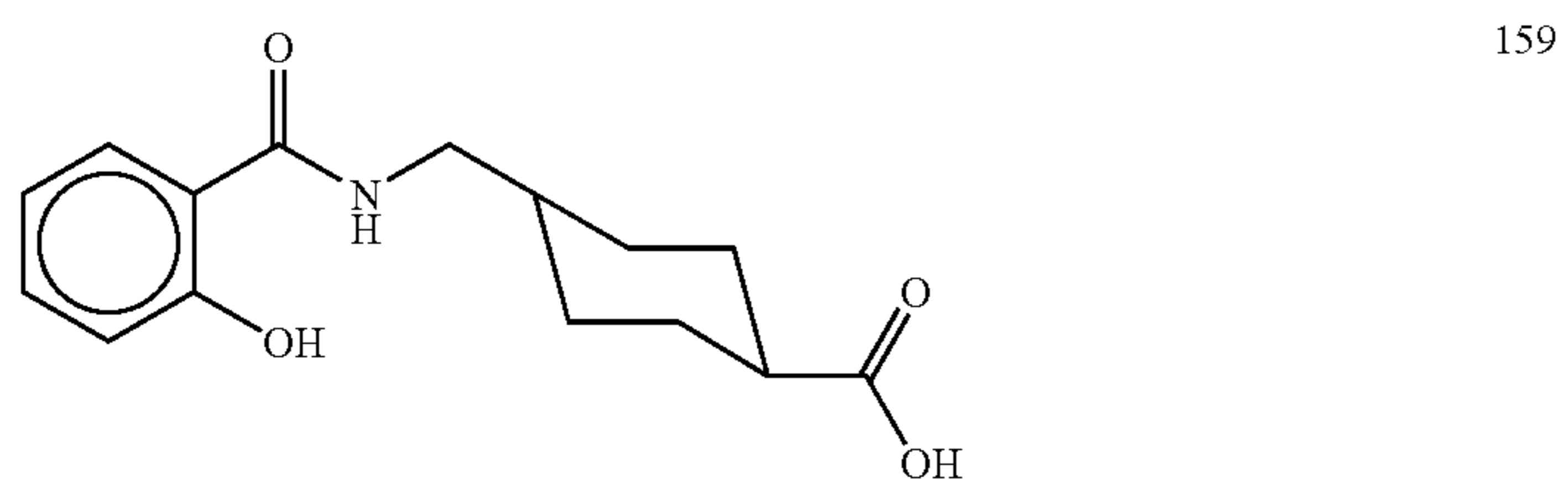
trans-4-(N-salicyloylaminomethyl)cyclohexane carboxylic acid
