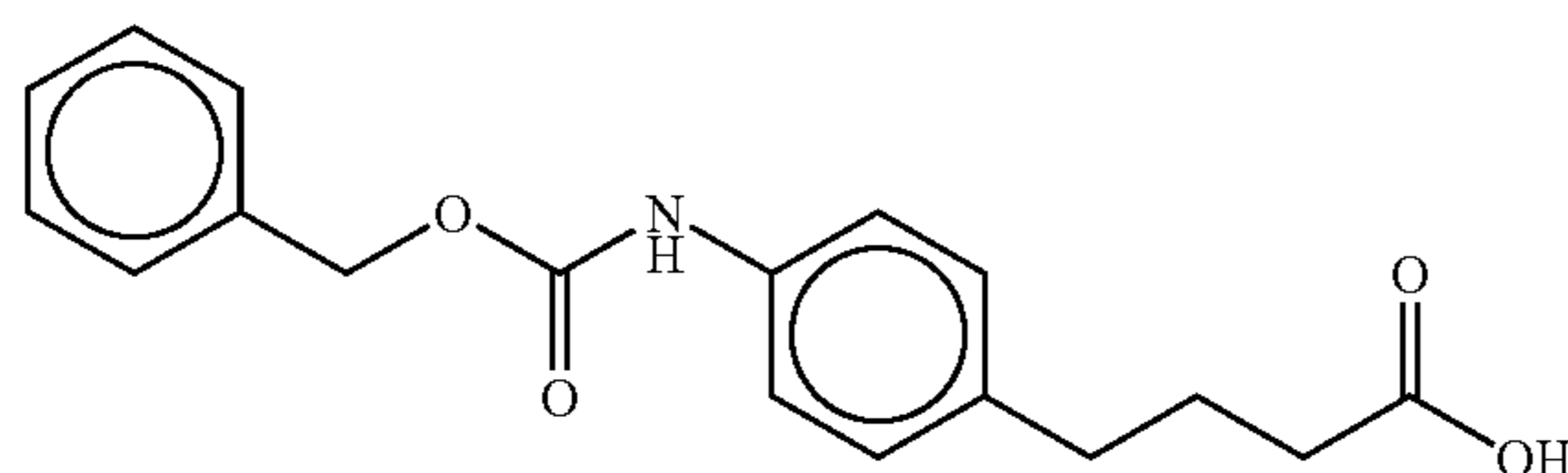
4-(4-benzoylcarbonylaminophenyl)butyric acid
