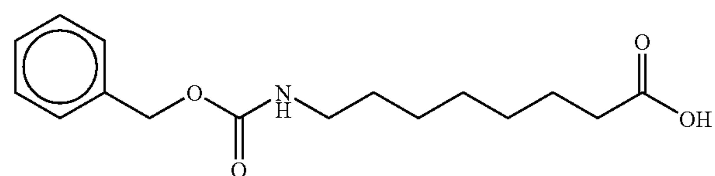
8-(Benzylcarbonylamino)caprylic acid
