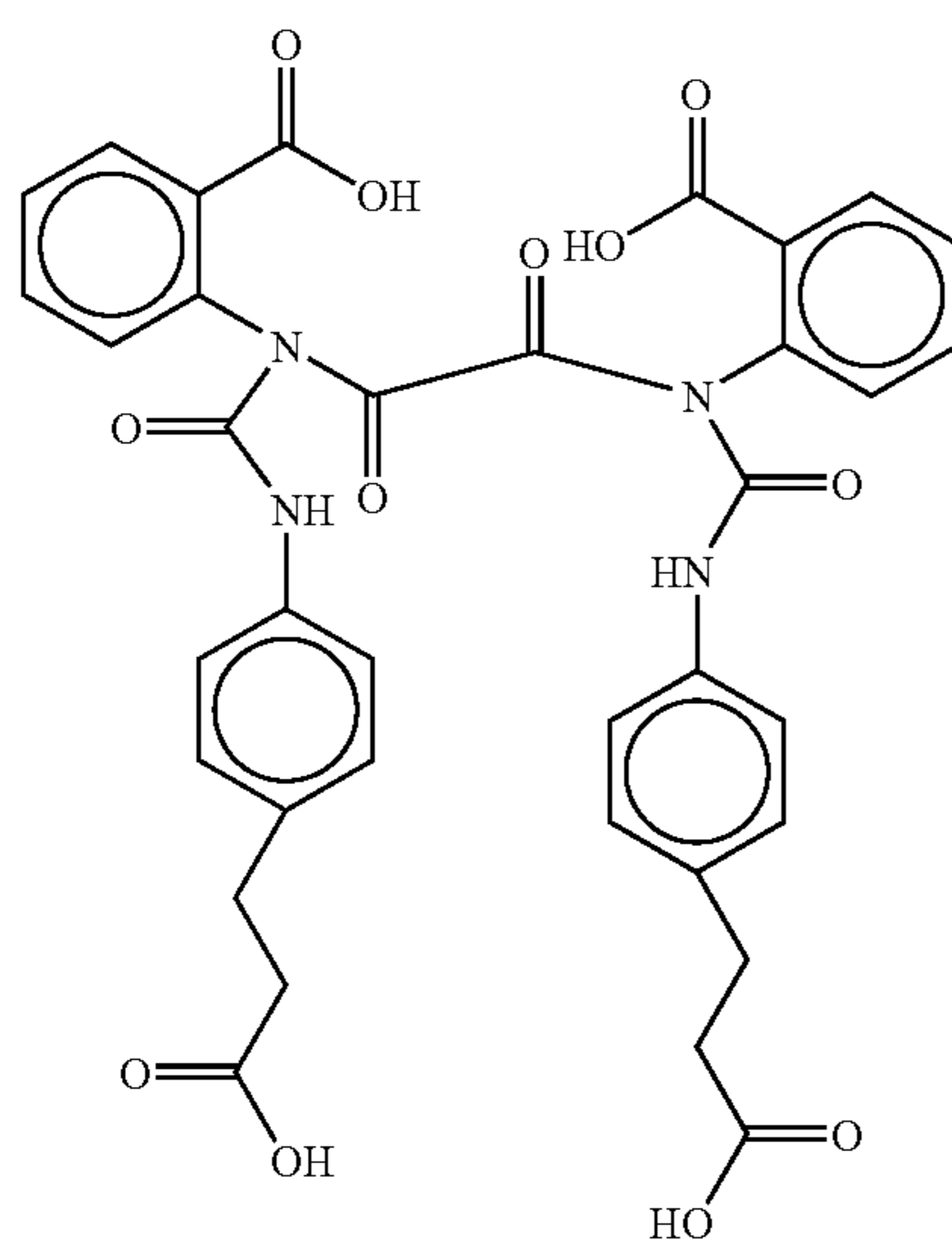
Bis(N-2-carboxyphenyl-N-(N'-3(4-aminophenyl)propionic acid)urea)oxalyl diamide
