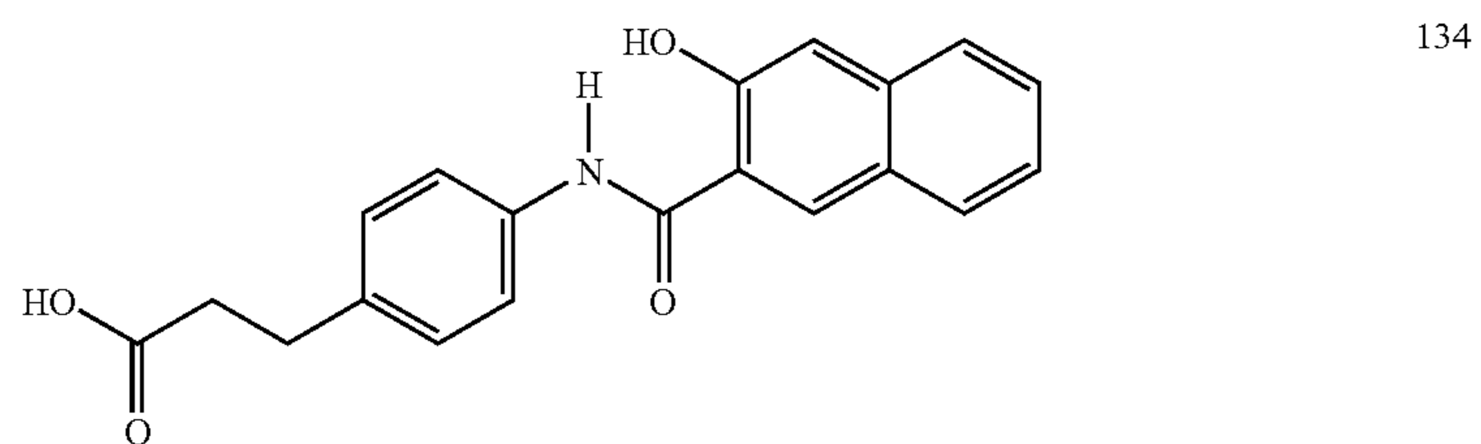
4-{4-[N-(3-hydroxy-2-naphthoyl)aminophenyl]}propanoic acid
