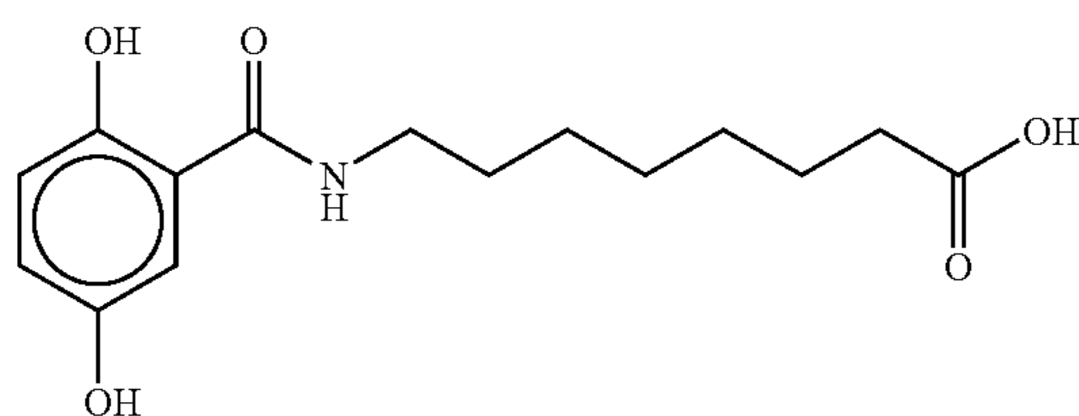
8-(N-2,5-Dihydroxybenzoyl)aminocaprylic acid
