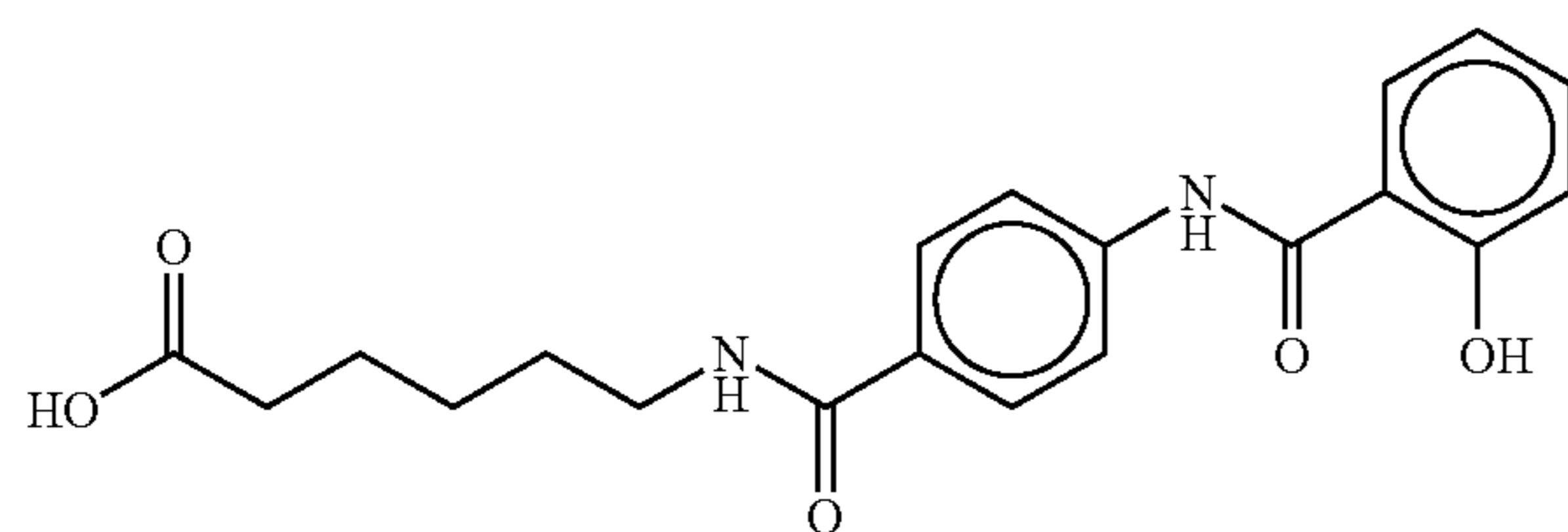
N-(4-saliyloylamino)-6-caproic acid
