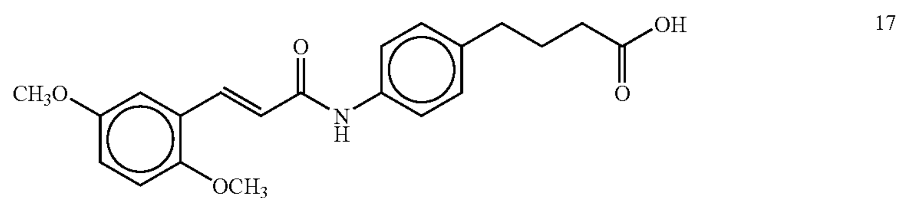
4-(4-(2,5-dimethoxycinnamoyl)aminophenyl)butyric acid
