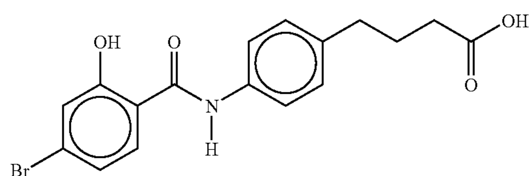
4-[N-(2-hydroxy-4-bromobenzoyl)aminophenyl]butyric acid
