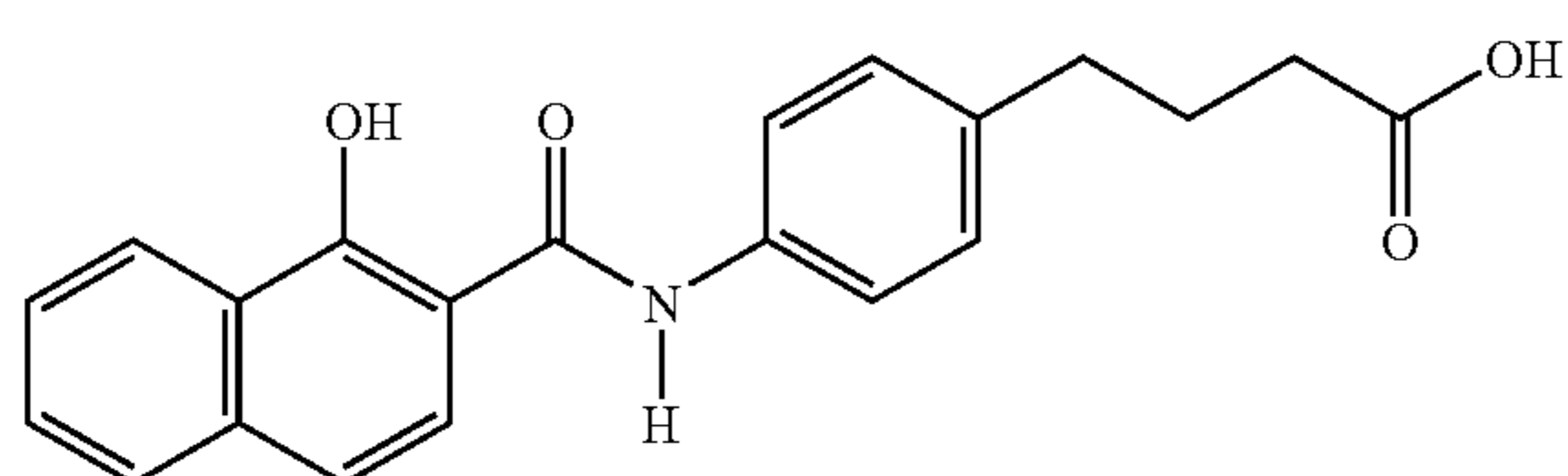
4-{4-[N-(1-hydroxy-2-naphthoyl)aminophenyl]}butyric acid
