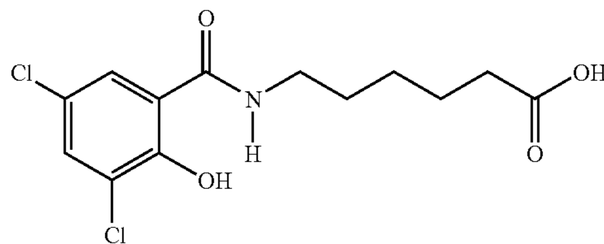
6-N-(3,5-dichloro-2-hydroxybenzoyl)aminocaproic acid
