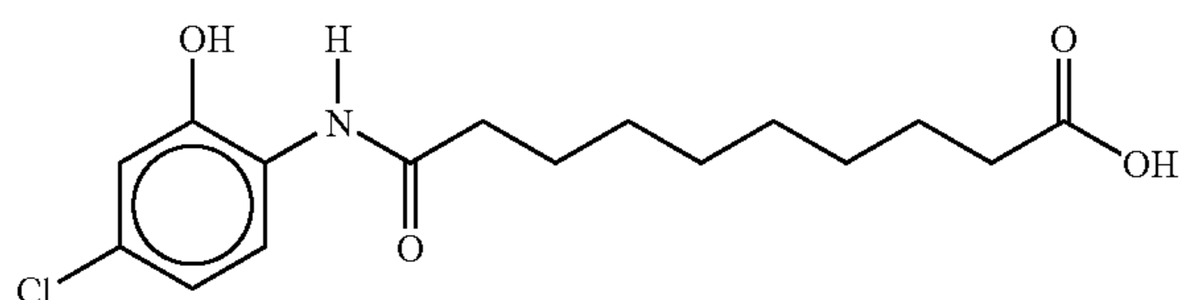
1-(4-chloro-2-hydroxyanilino)sebacic acid monoamide
