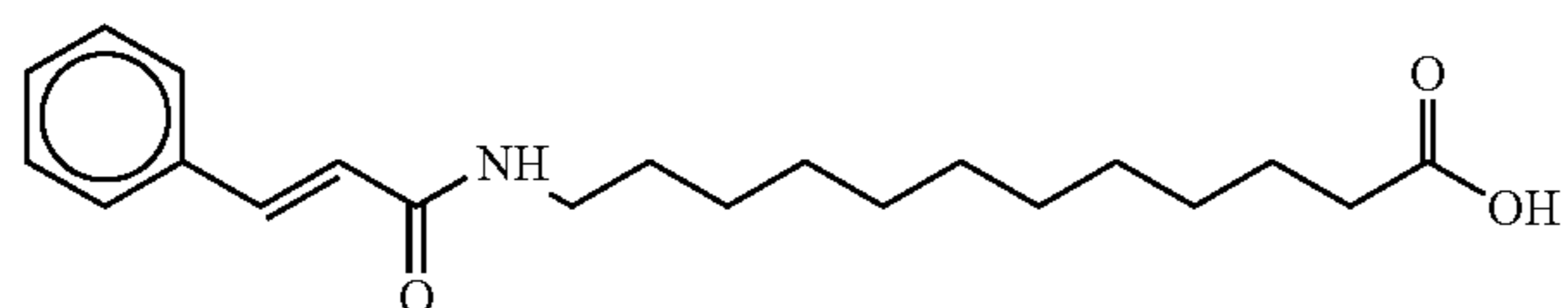
12-cinnamoyldodecanoic acid
