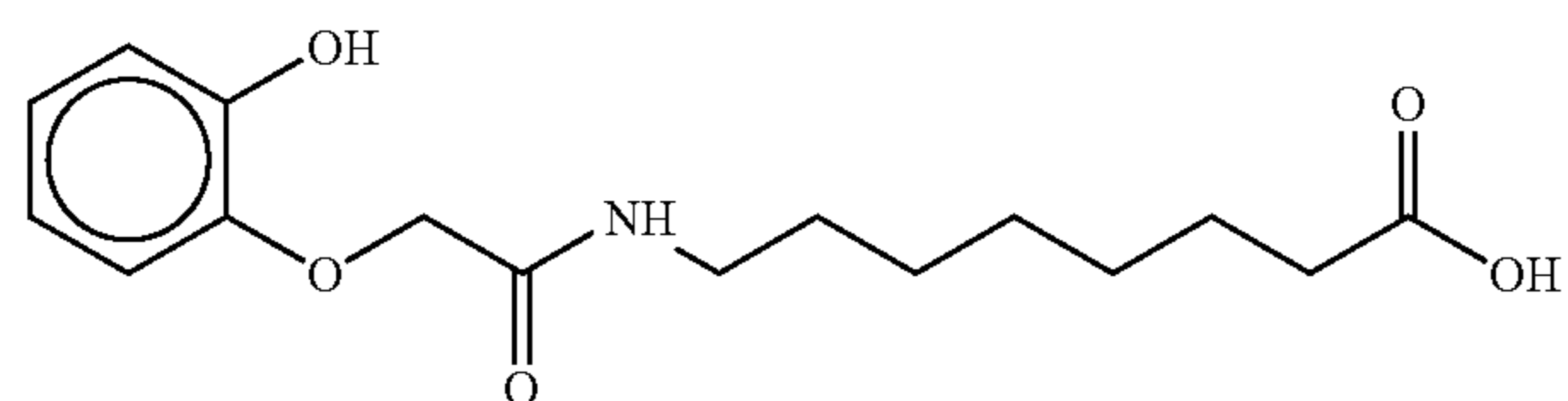
7-(2-hydroxyphenoxyacetyl)aminocaproic acid
