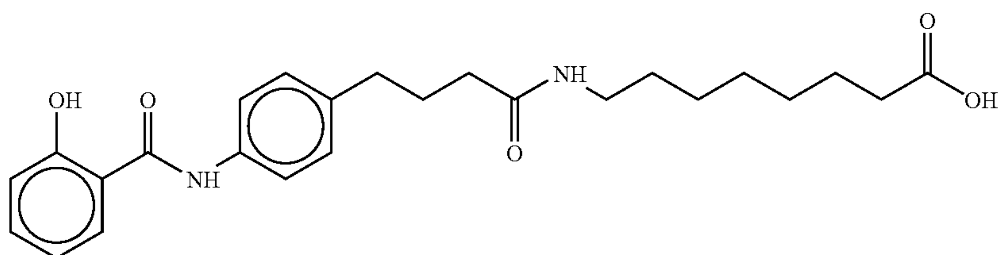
8-(4-(N-Salicyloyl-4-aminophenyl)butyric)aminocaprylic acid [sic]
