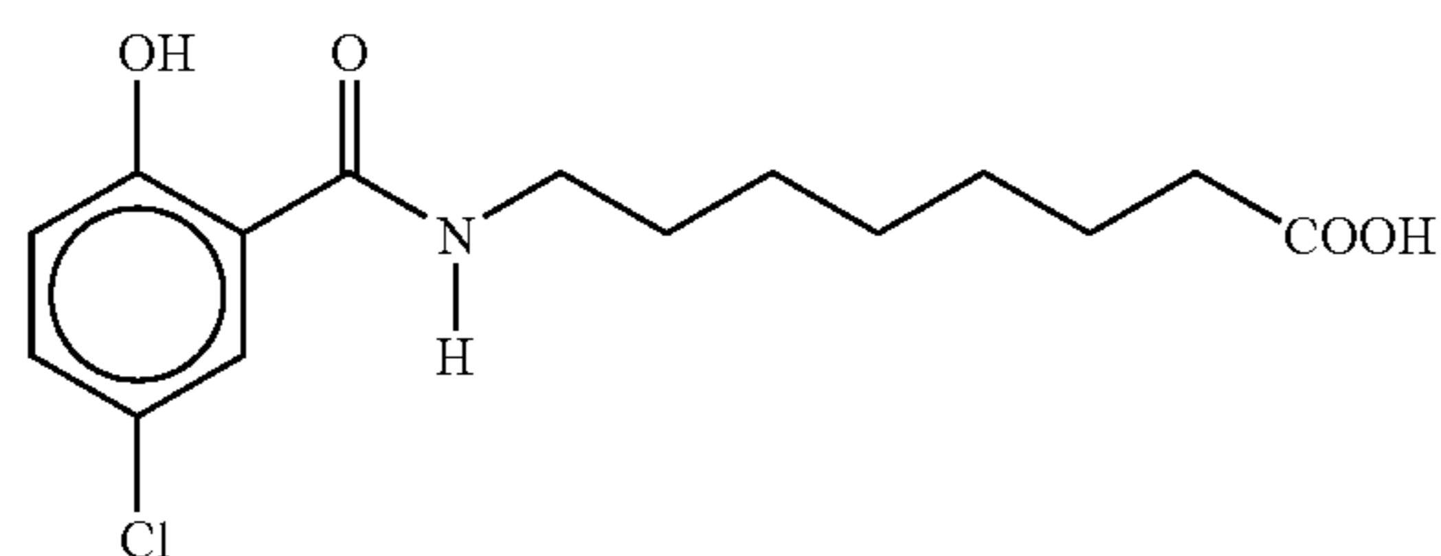
8-(N-2-hydroxy-5-chlorobenzoyl)aminocaprylic acid
