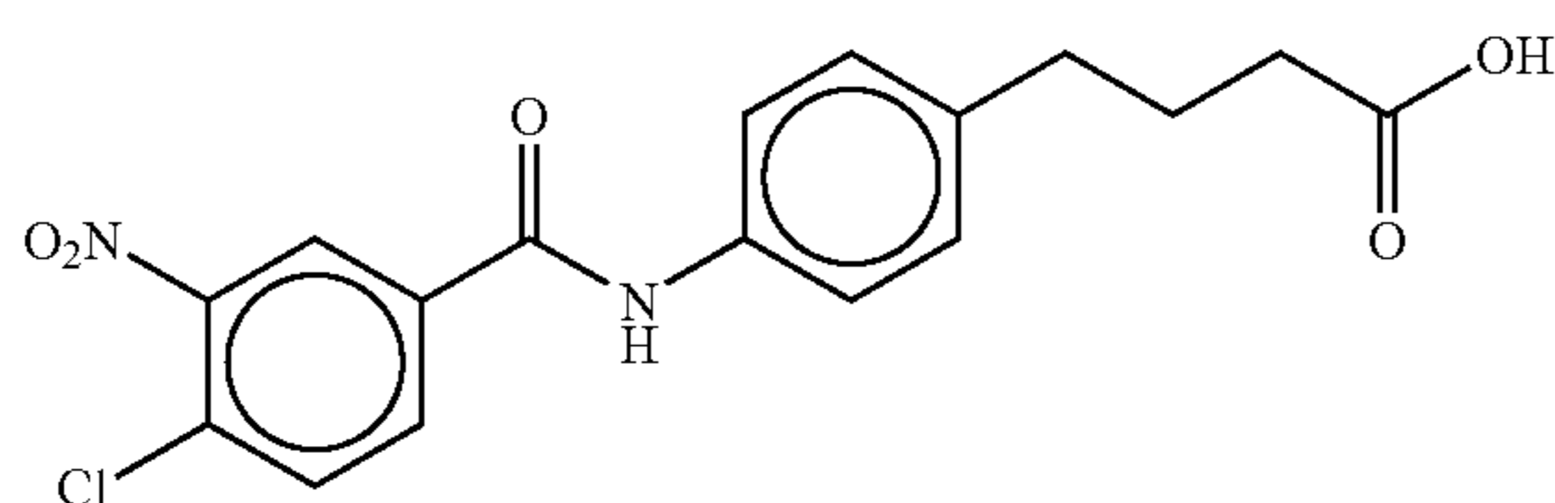
4-(4-(4-chloro-3-nitrobenzoyl)aminophenyl)butyric acid
