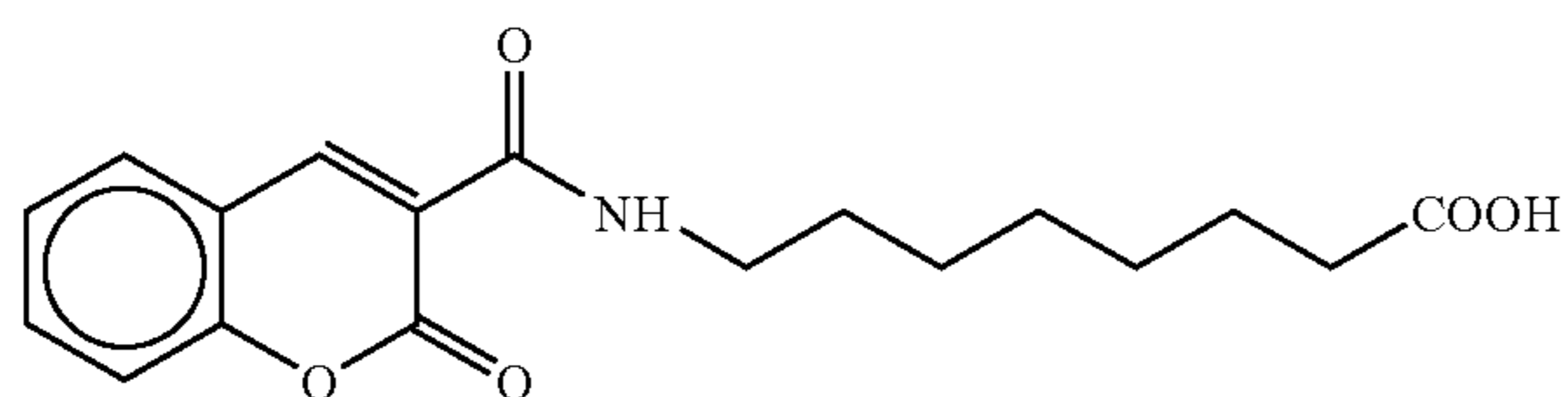
8-[N-(3-coumarincarboxyl)]aminocaprylic acid
