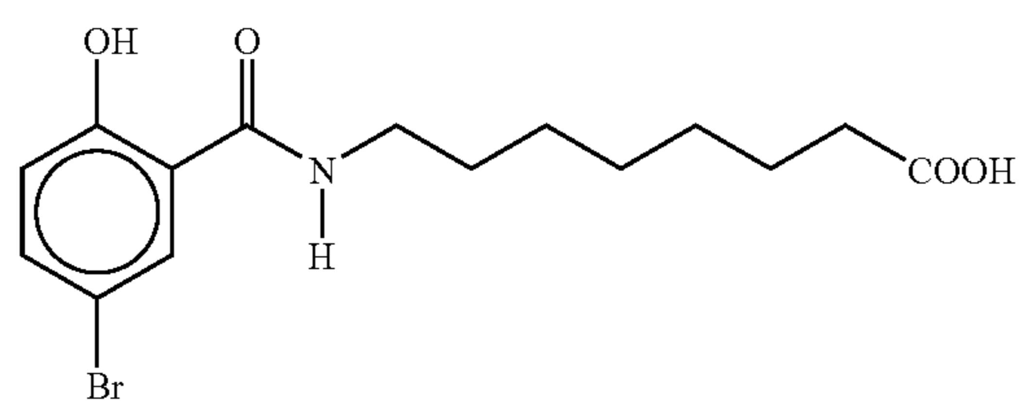
8-(N-(2-hydroxy-5-bromobenzoyl)aminocaprylic acid
