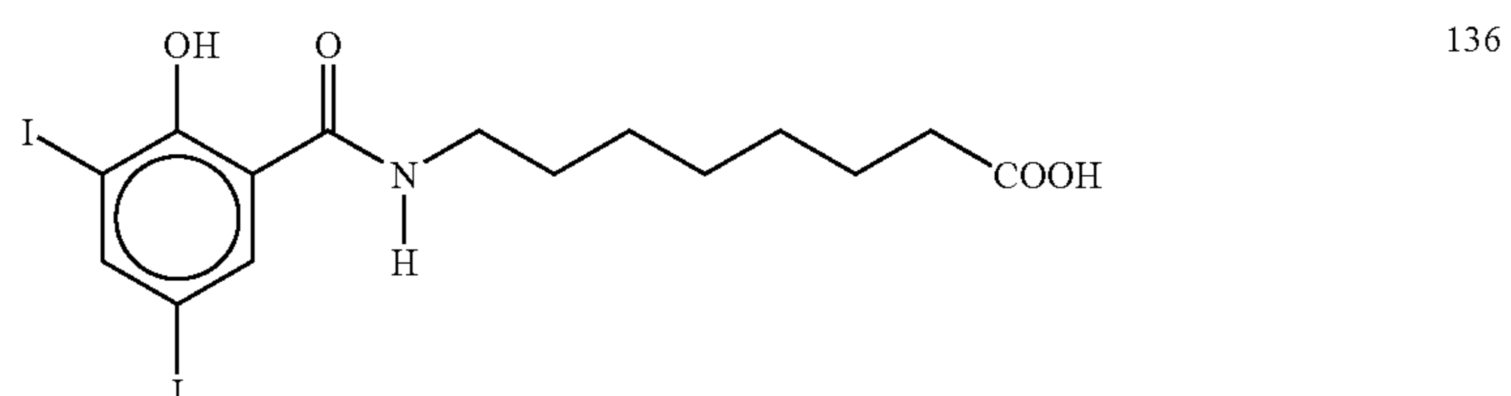
8-(N-2-hydroxy-3,5-diiodobenzoyl)aminocaprylic acid
