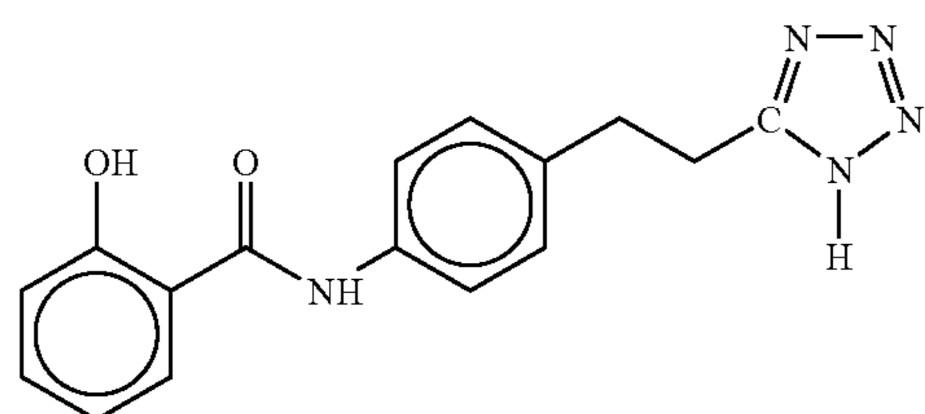
4-(Salicyloyl)aminophenylethyltetrazole
