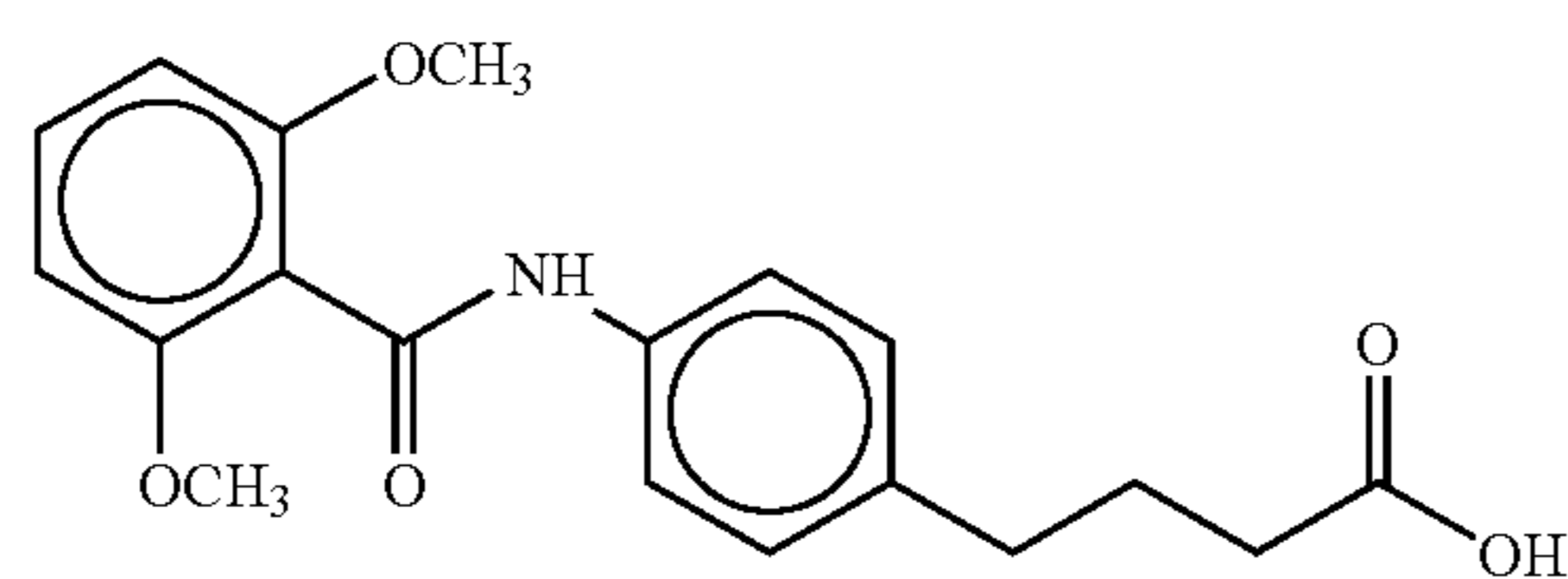
4-(4-(2,6-dimethoxybenzoyl)aminophenyl)butyric acid
