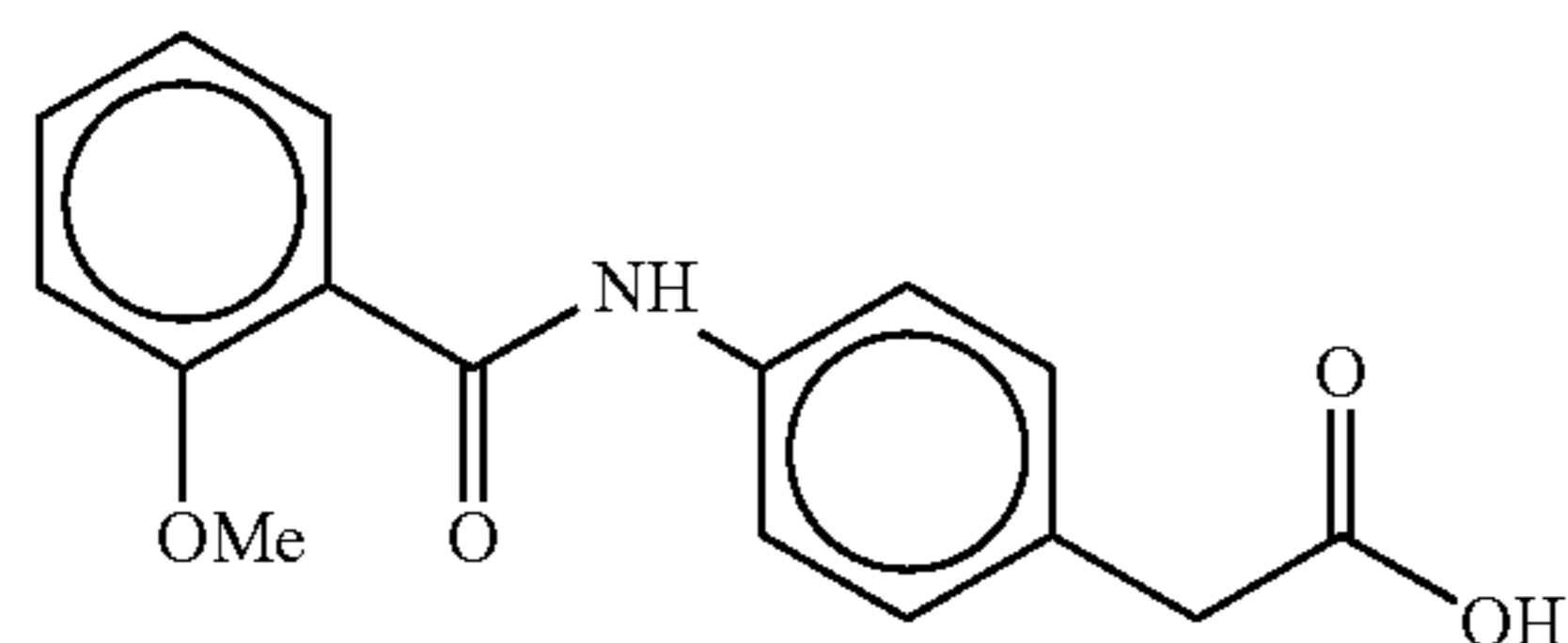
4-(o-anisoyl)aminophenylacetic acid
