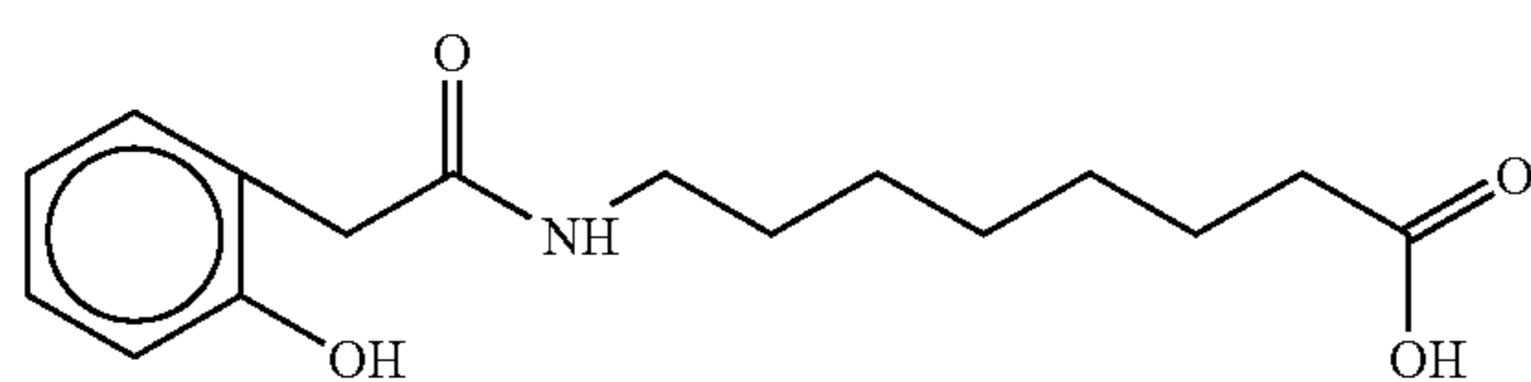
8-(2-hydroxyphenoxy)aminocaproic acid
