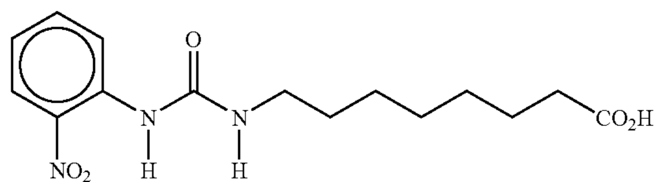
N-2-bi(phenyl)-N'-(8-octanoic acid) urea
