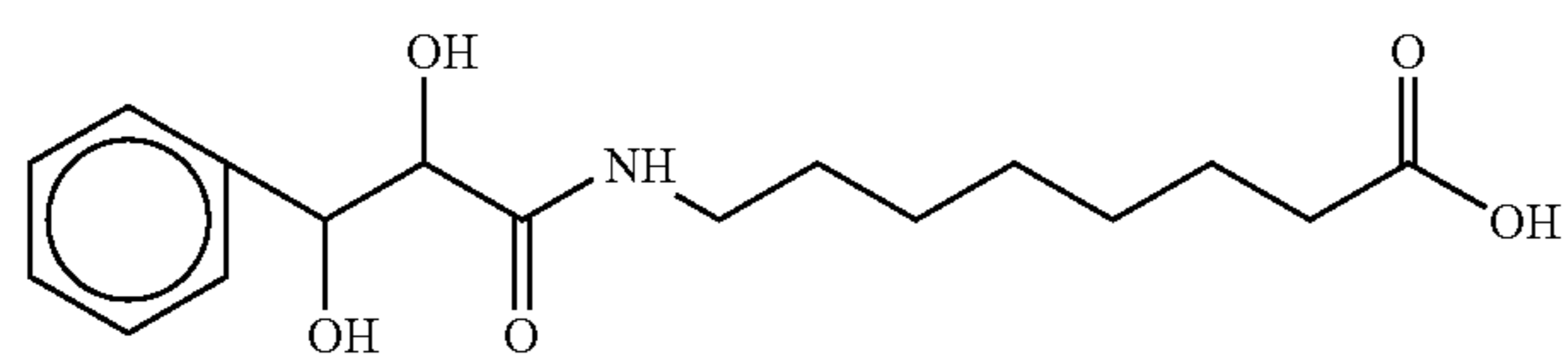
(3-Phenyl-2,3-dihydroxypropanoyl)8aminocaprylic acid
