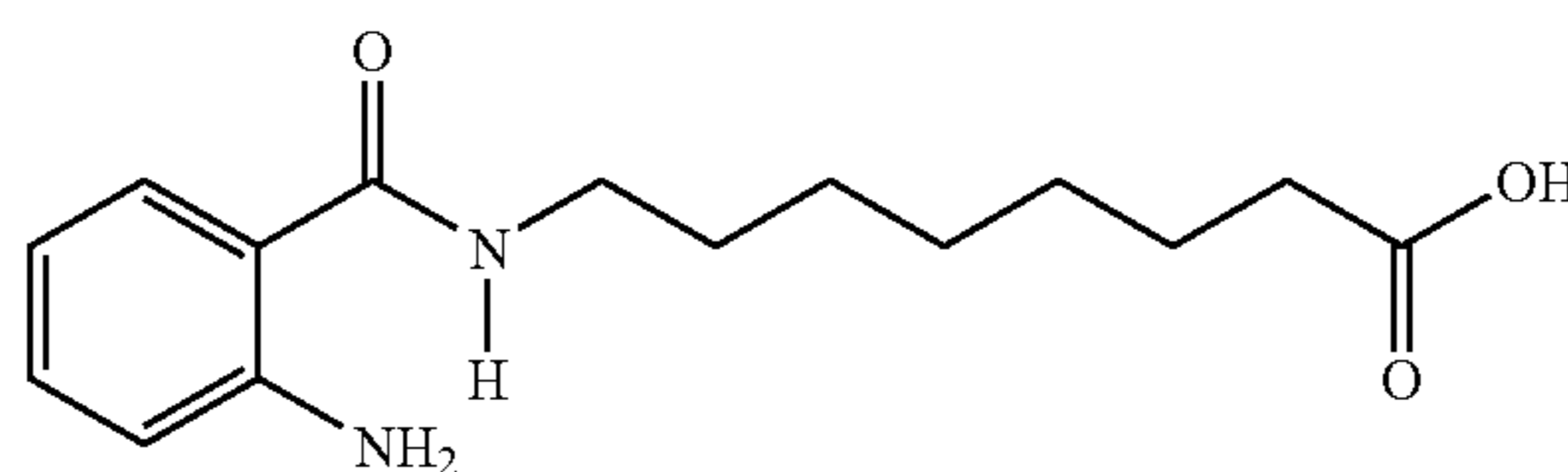
8(2-aminobenzoylamino)caprylic acid
