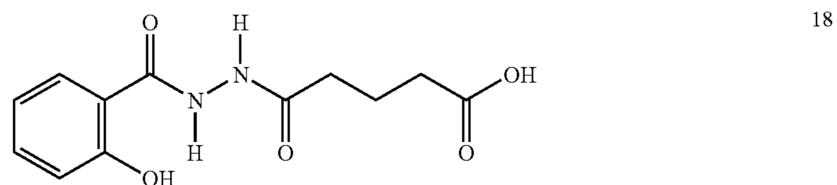
1-salicyloyl-2-glutaryl hydrazide
