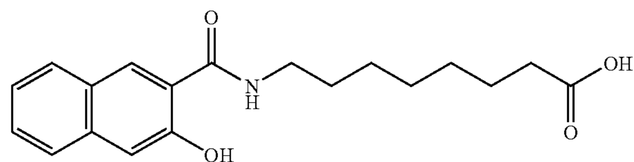
8-(3-hydroxy-2-naphthoyl)aminocaprylic acid
