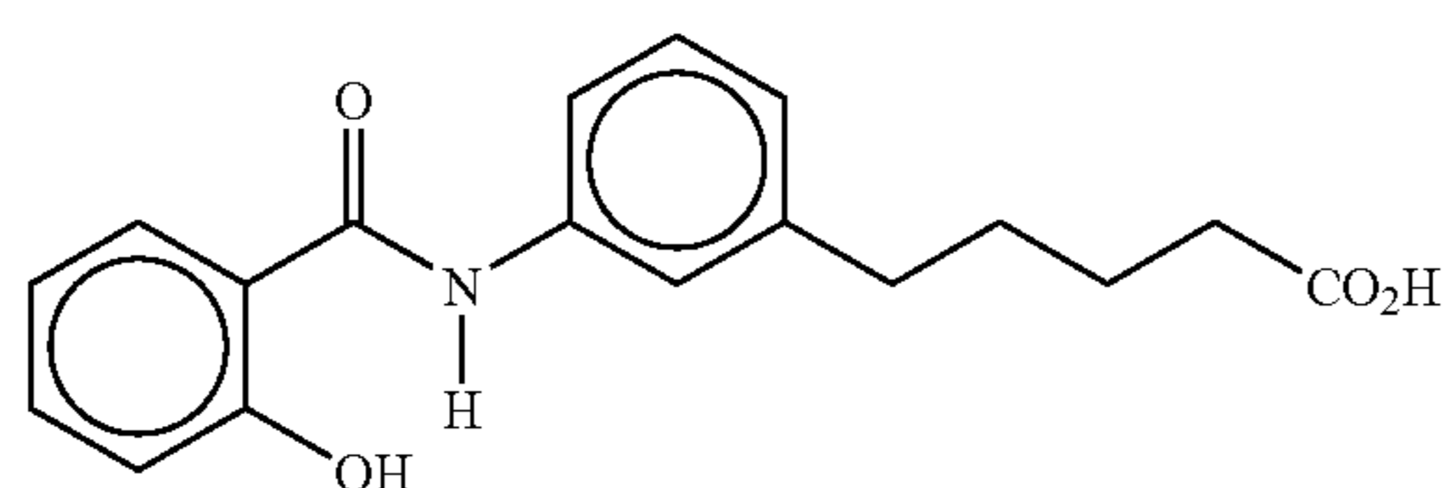
N-Saliyloyl-5-(3-aminophenyl)valeric acid
