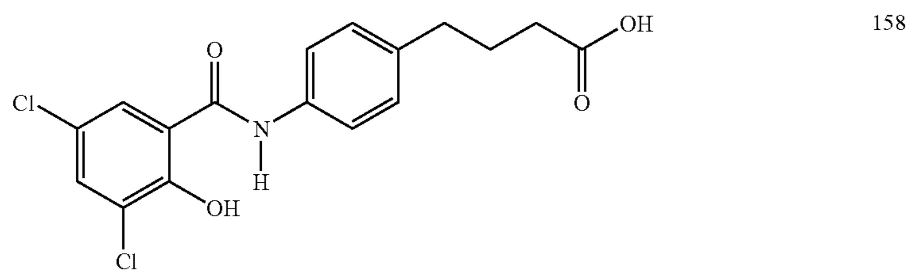
N-[3,5-dichloro-2-hydroxybenzoyl-4(4-aminophenyl)]butyric acid
