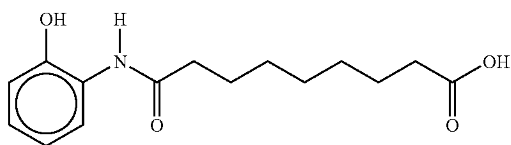
9-(2-hydroxybenzamido)nonanoic acid
