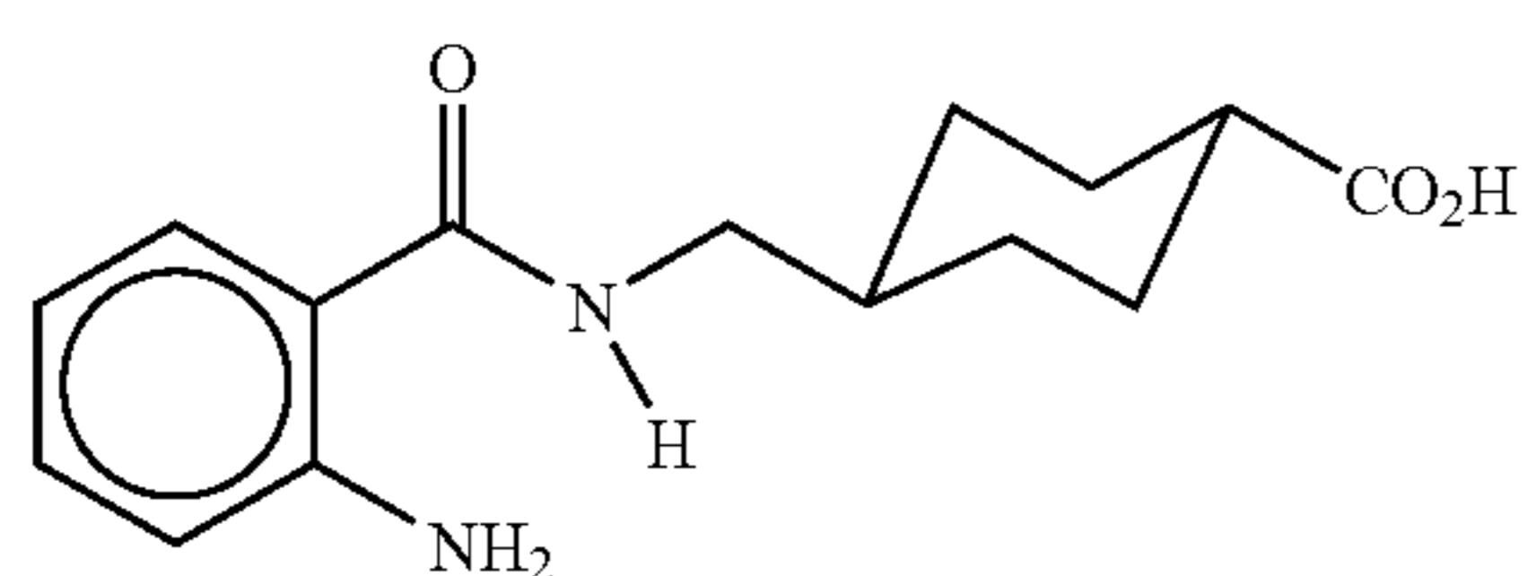
trans-4-(2-aminobenzamidomethyl)cyclohexanecarboxylic acid
