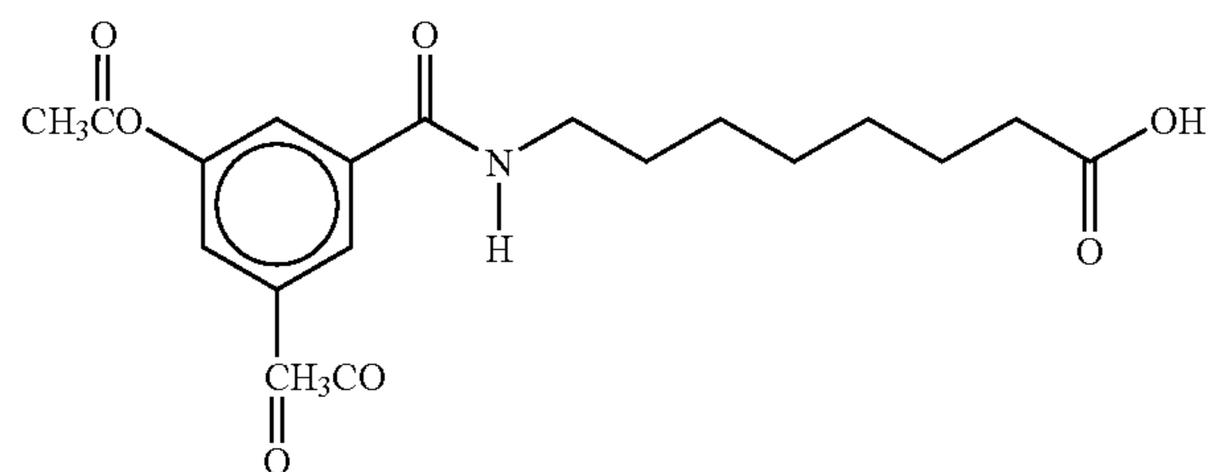
8-(N-3,5-Diacetylbenzoyl)aminocaprylic acid
