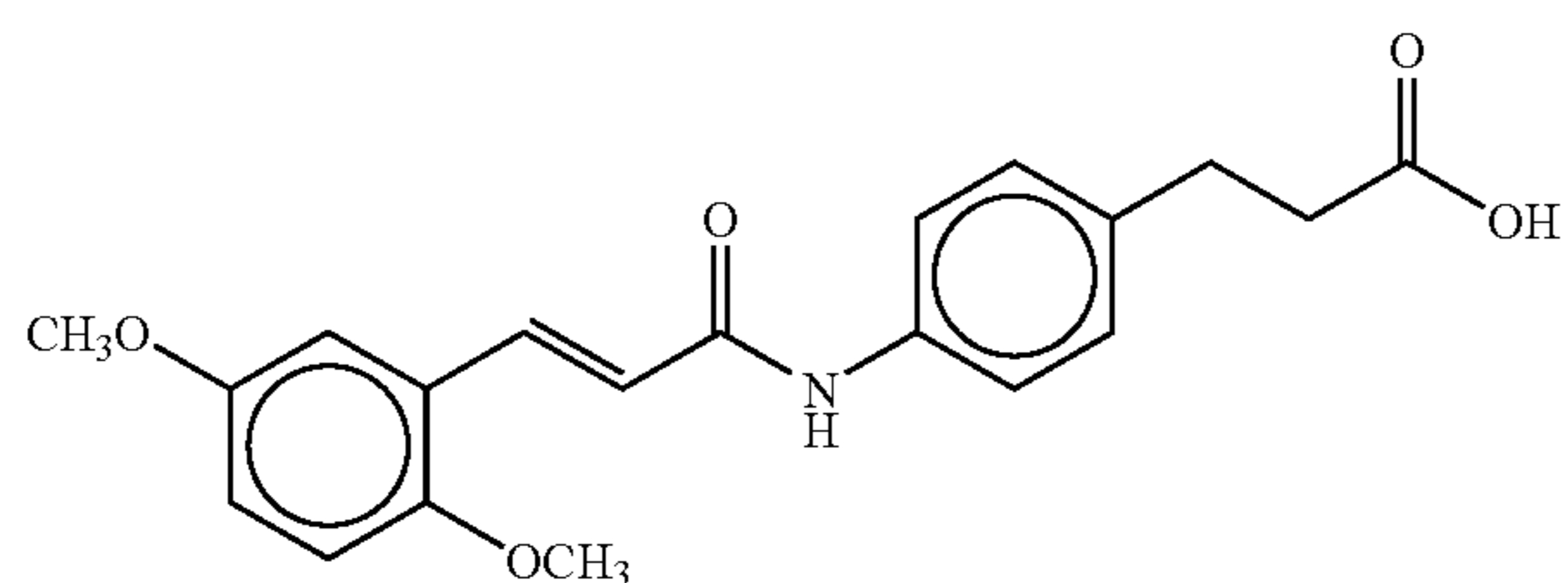
3-(4-(2,5-dimethoxycinnamoyl)aminophenyl)propionic acid
