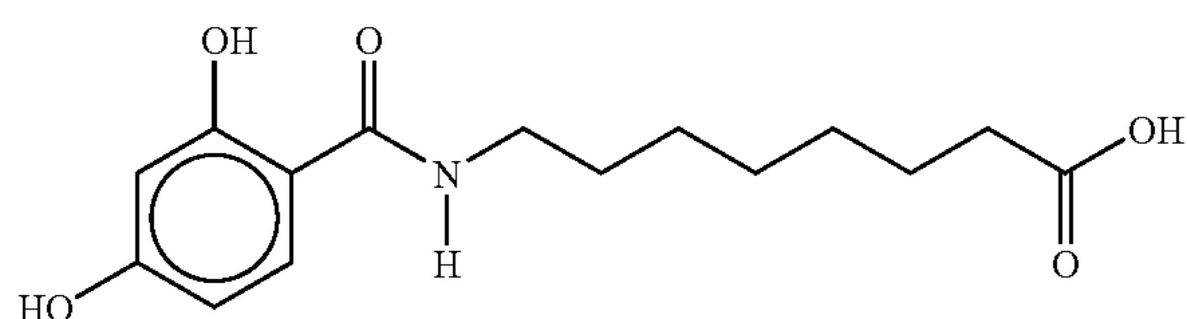
8-(N-2,4-Dihydroxybenzoyl)aminocaprylic acid
