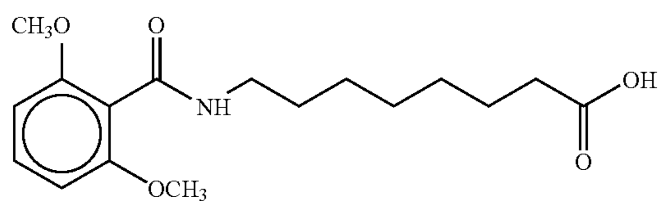
8-(N-2-6-Dimethoxybenzoyl)aminocaprylic acid
