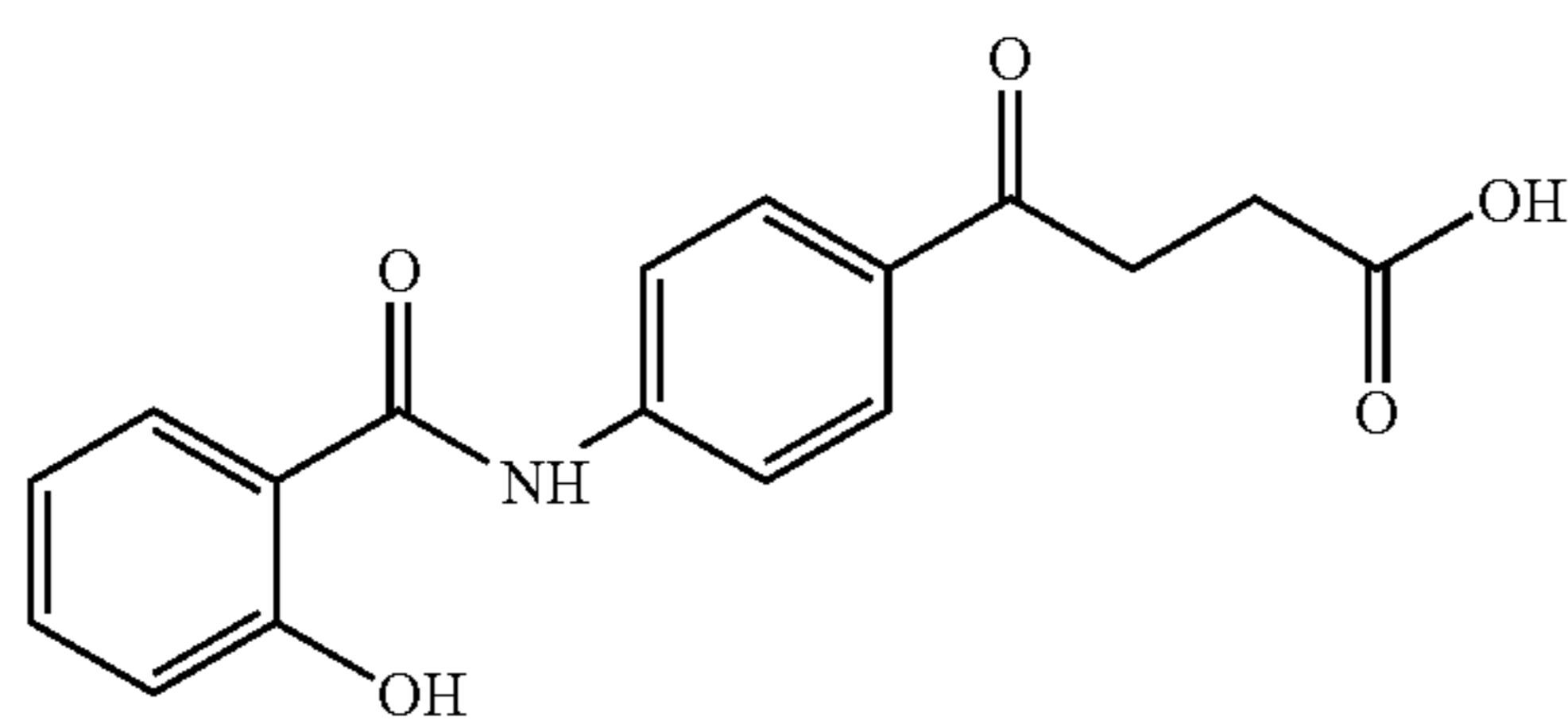
4-(4-(4-(2-hydroxybenzoyl)aminophenyl)butyryl)phenylacetic acid
