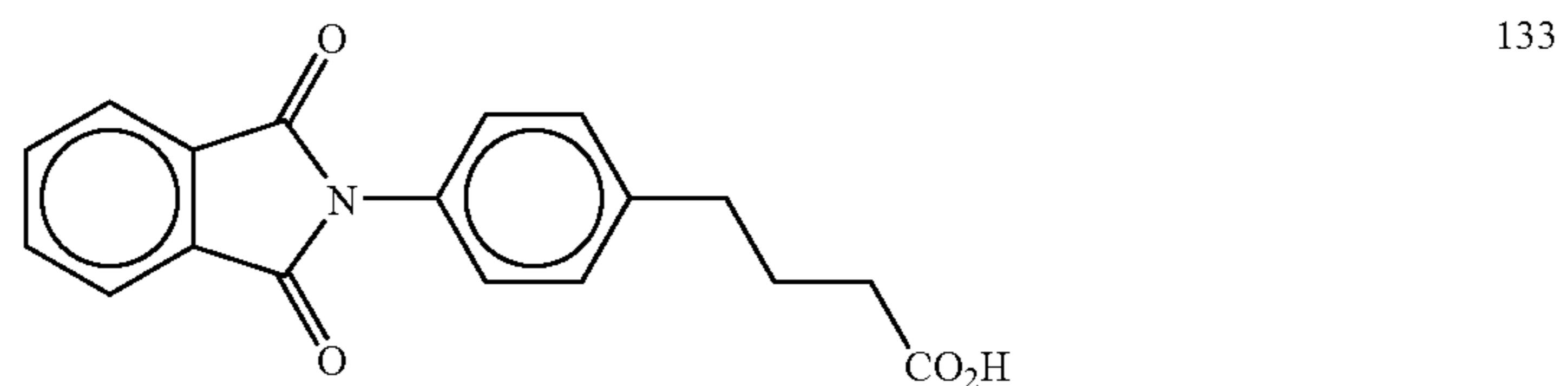
4-(4-phthalimidophenyl)butyric acid
