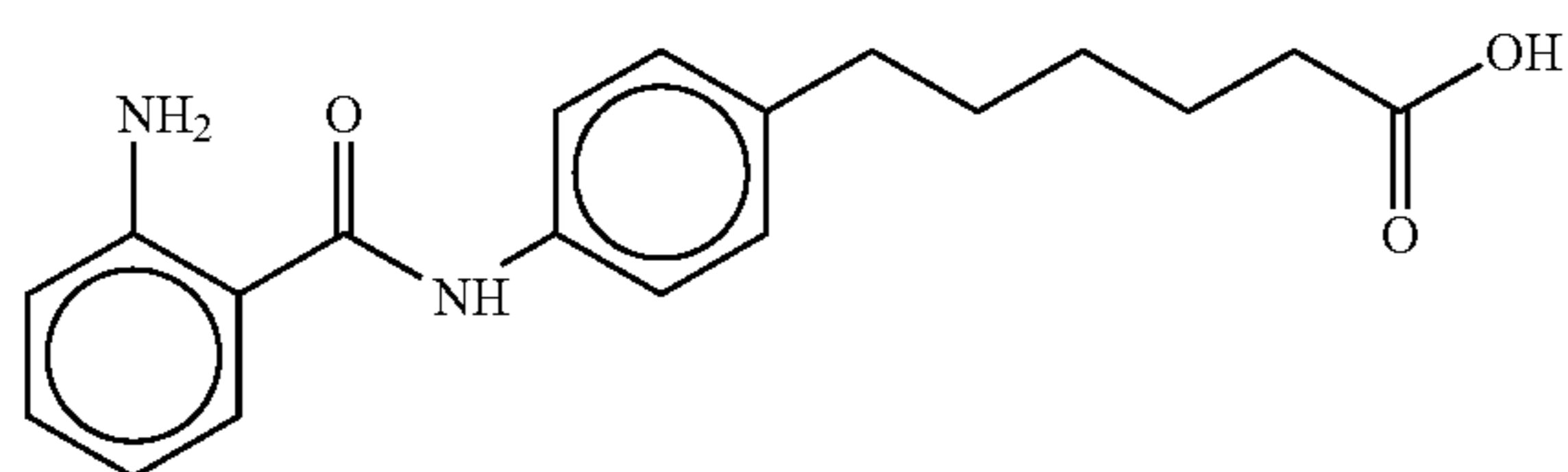
6-(4-(N-2-aminobenzoyl)aminophenyl)hexanoic acid
