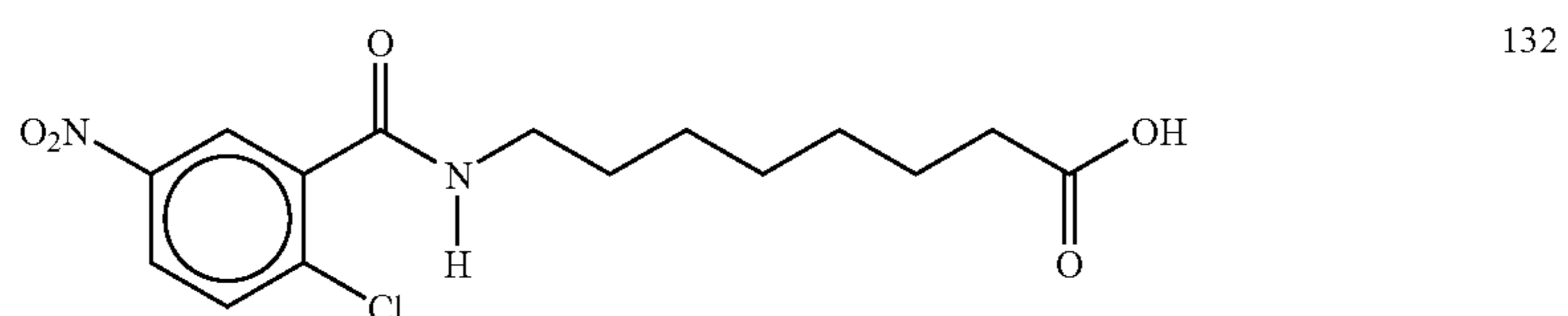
8-(2-chloro-5-nitrobenzoyl)aminocaprylic acid
