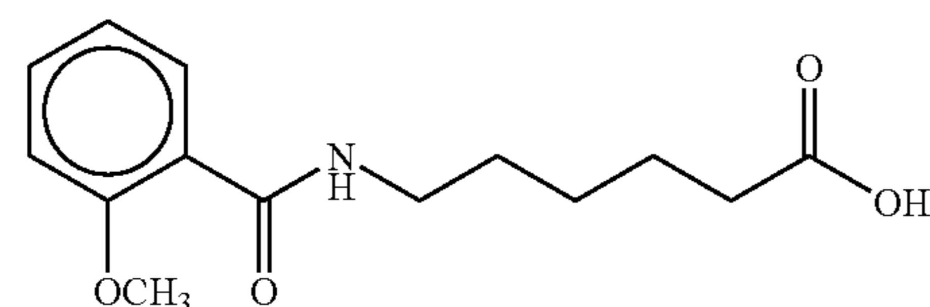
6-(anisoyl)aminocaprylic acid
