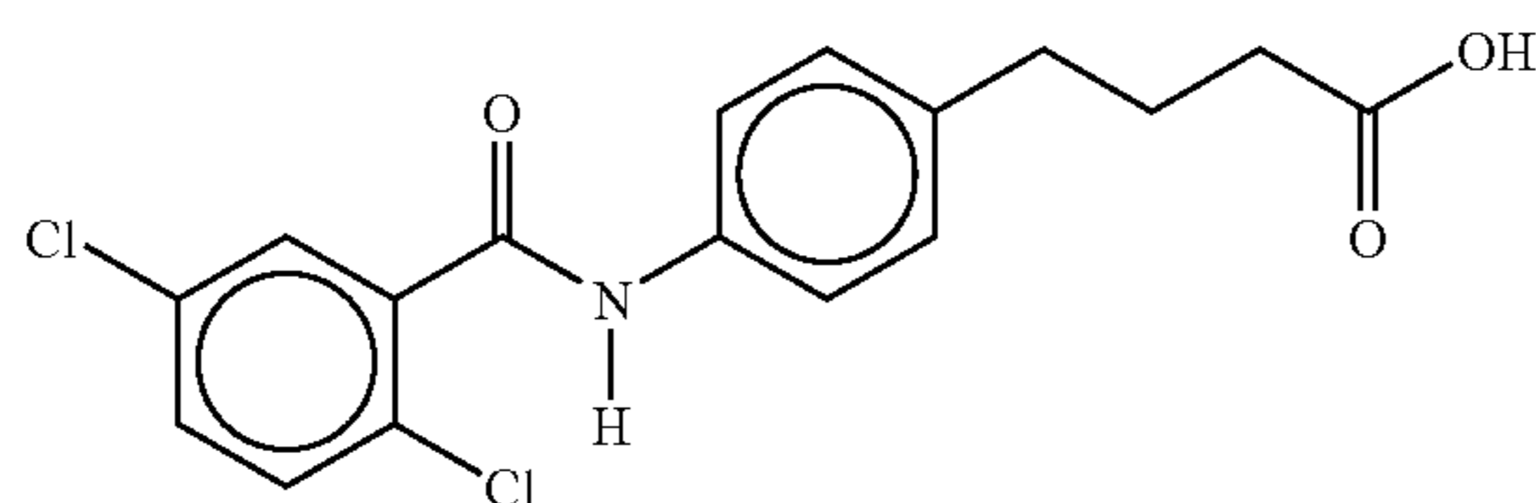
4-(4-(2-chloro-5-nitrobenzoyl)aminophenyl)butyric acid
