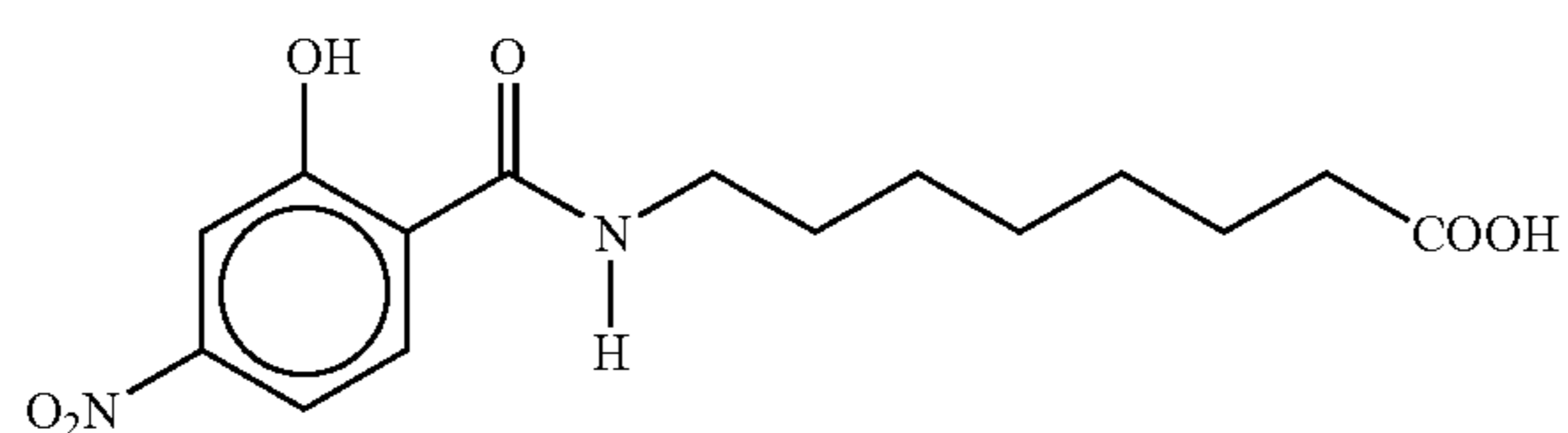
8-(N-2-hydroxy-4-nitrobenzoyl)aminocaprylic acid
