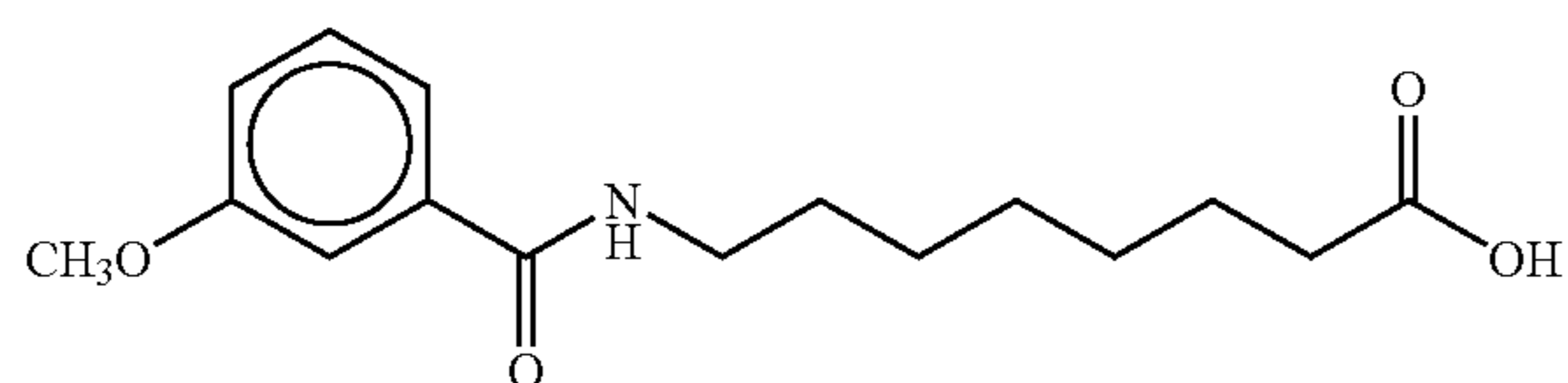
8-(3-anisoyl)aminocaprylic acid
