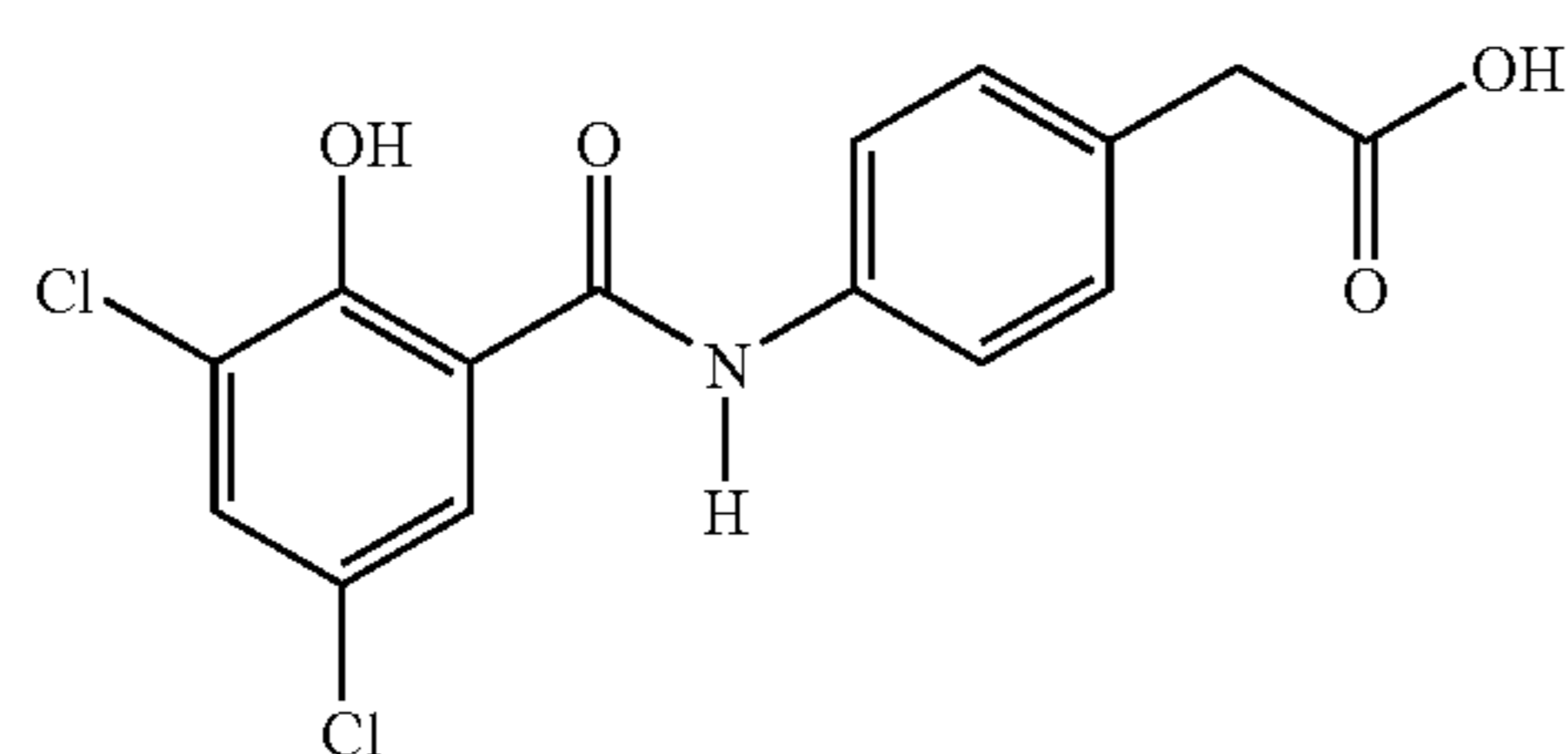
4-[N-(3,5-dichloro-2-hydroxybenzoyl)]aminophenylacetic acid
