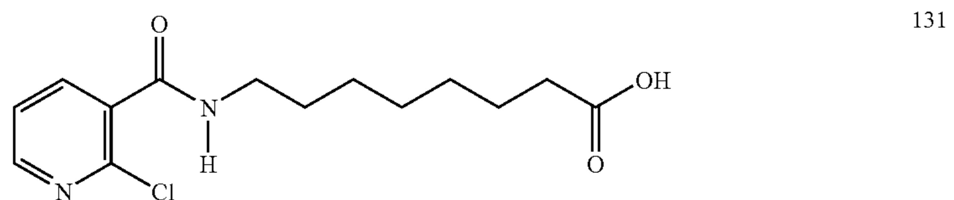
8-(2-chloronicotinoyl)aminocaprylic acid
