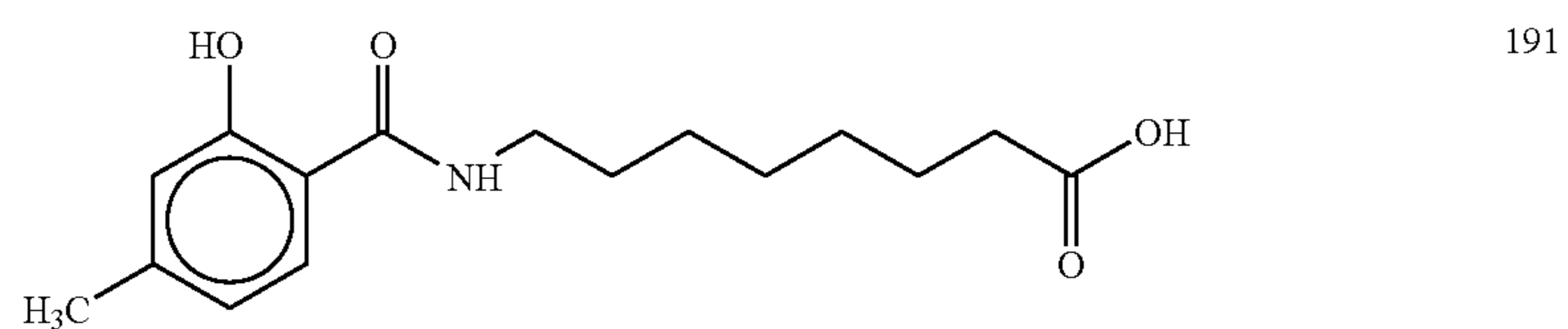
8-(N-4-Methylsalicyloyl)aminocaprylic acid [sic]
