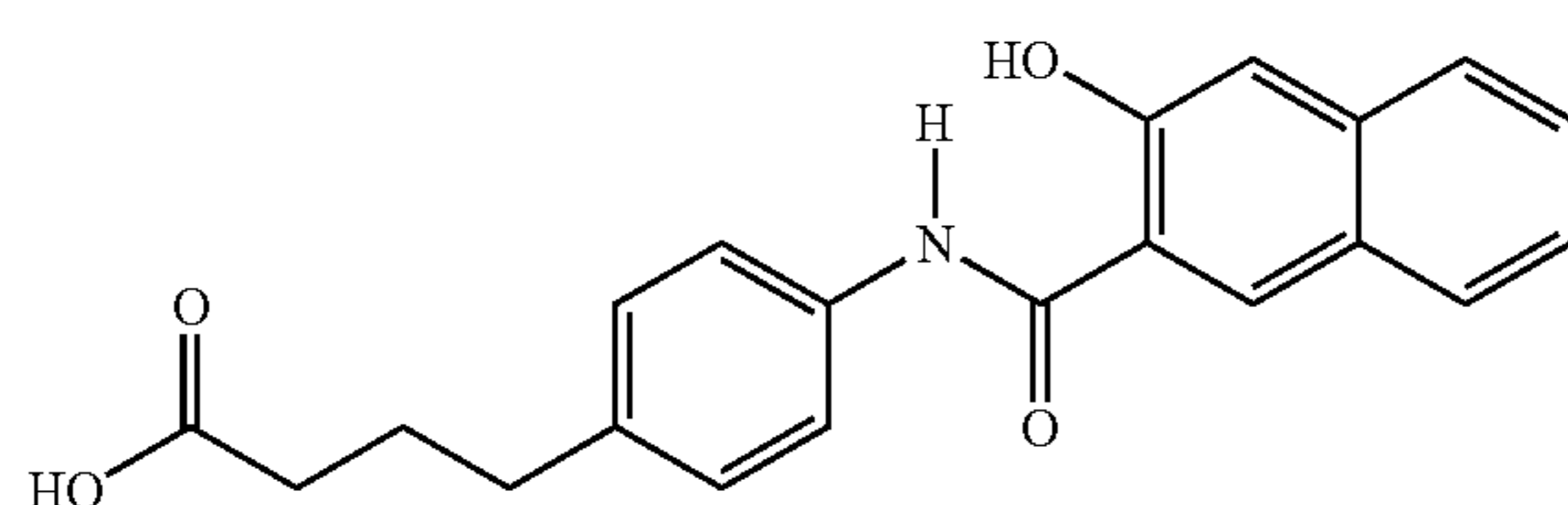
4-{4-[N-(3-hydroxy-2-naphthoyl)aminophenyl]}butyric acid
