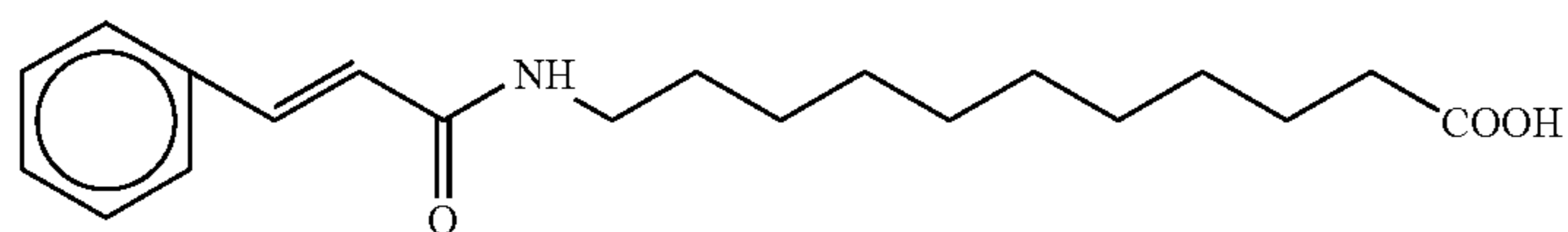
11-cinnamoylaminoundecanoic acid
