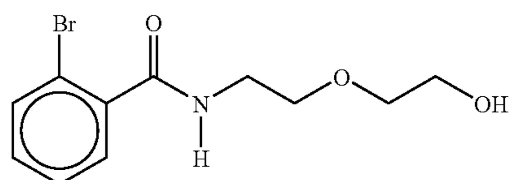
2-[N-(2-bromobenzoyl)aminoethoxy]ethanol
