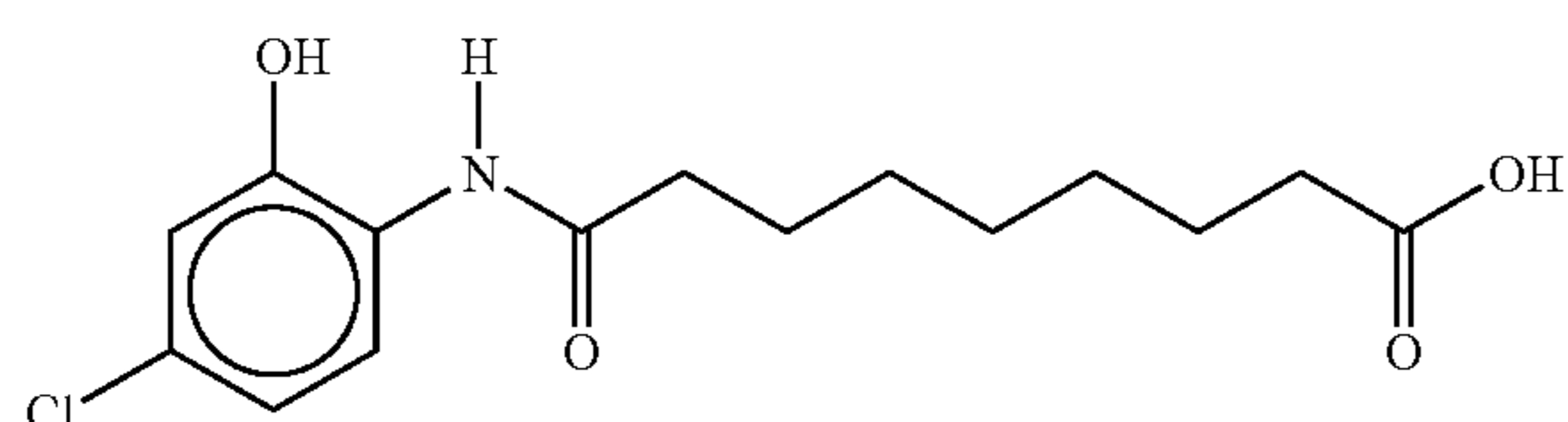
8-(2-hydroxy-5-chloroanilino)octanoic acid
