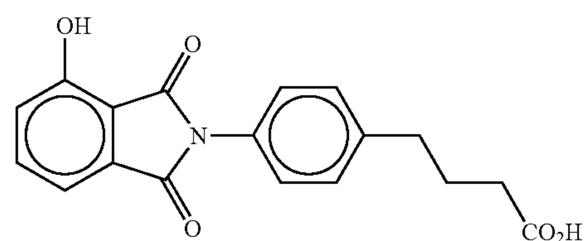
4-(4-(3-hydroxyphthalimido)phenyl)butyric acid
