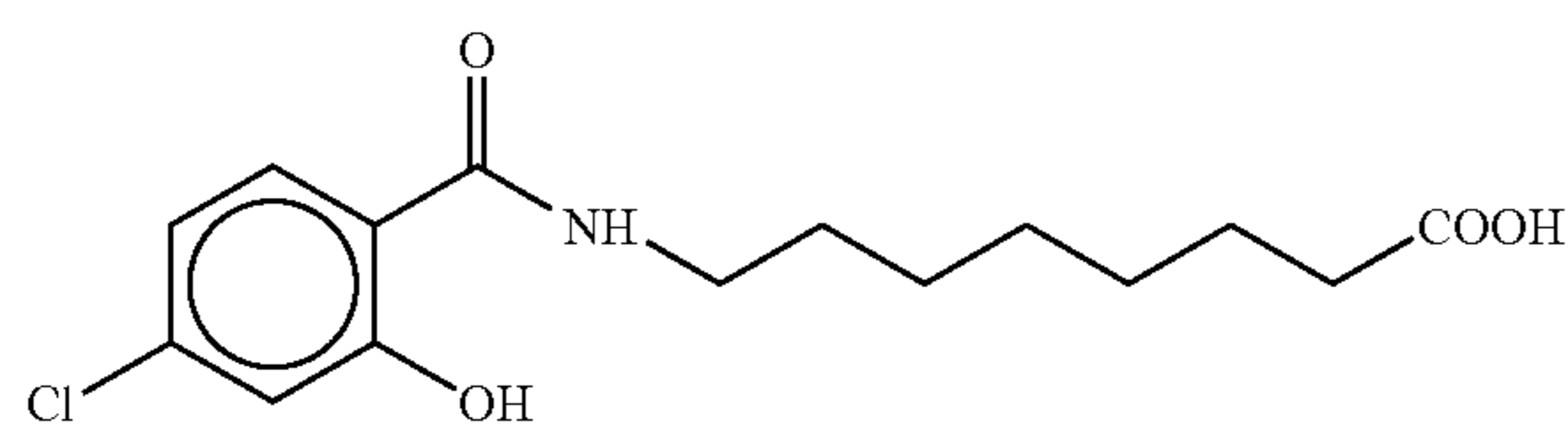
8-(2-hydroxy-4-chlorobenzoyl)aminocaprylic acid
