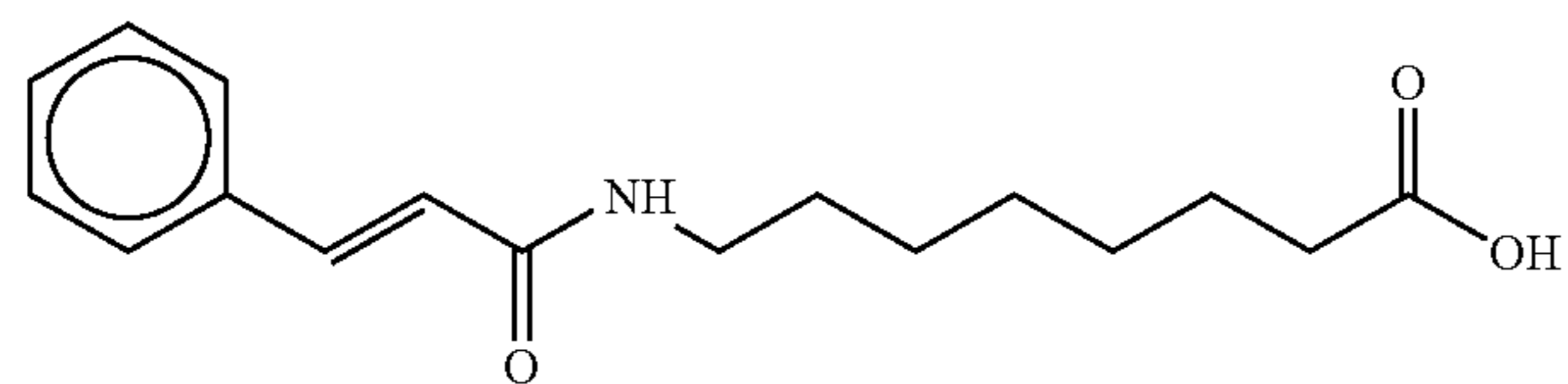
8-cinnamoylaminovaleric acid
