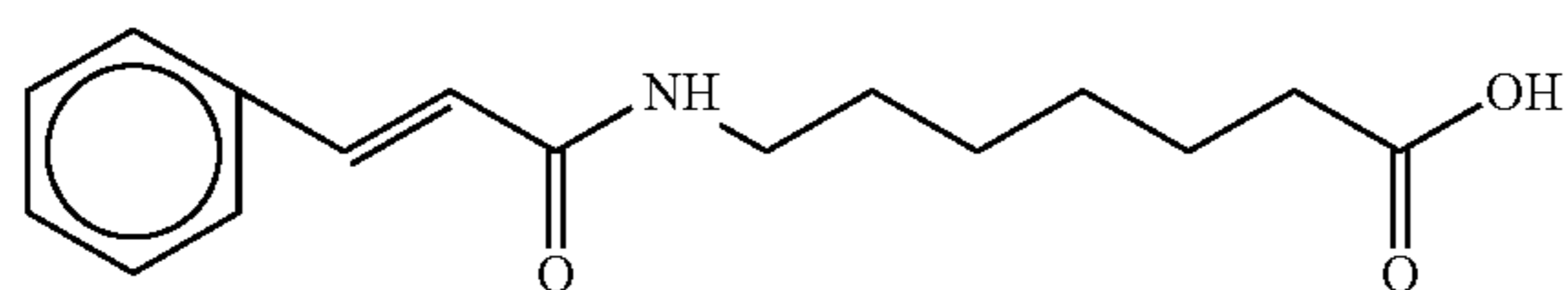
7-cinnamoylaminoheptanoic acid
