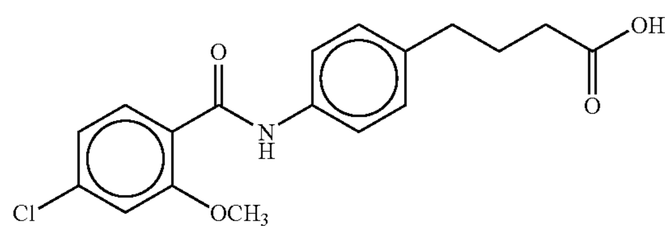
4-(4-(4-chloro-o-anisoyl)aminophenyl)butyric acid
