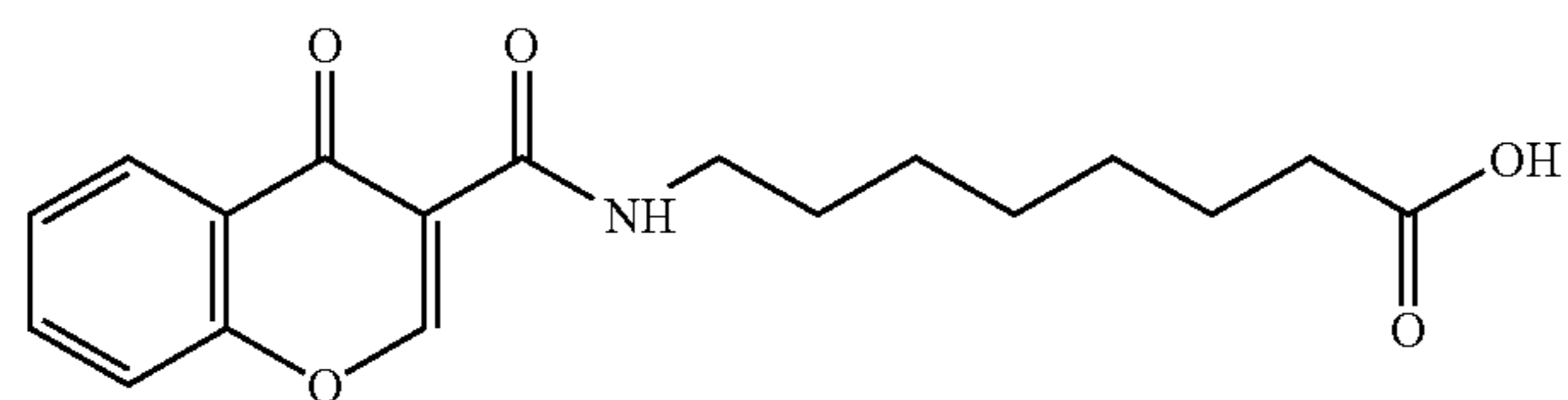
8-(chromone-3-carbonyl)aminocaprylic acid
