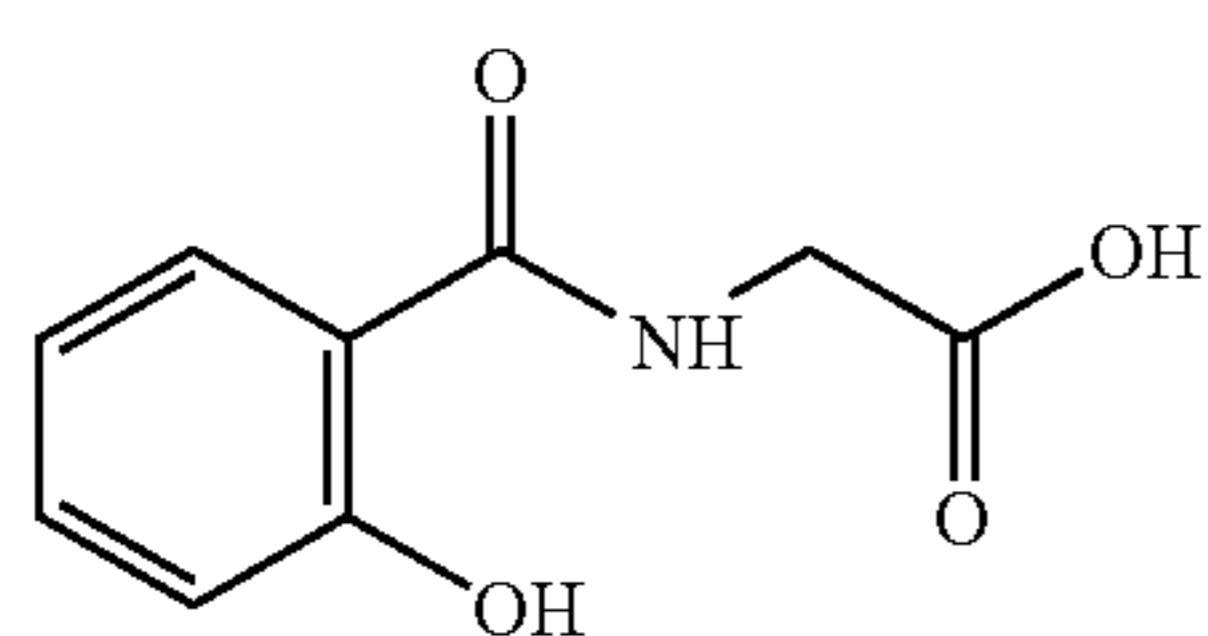
salicyloylglycine
