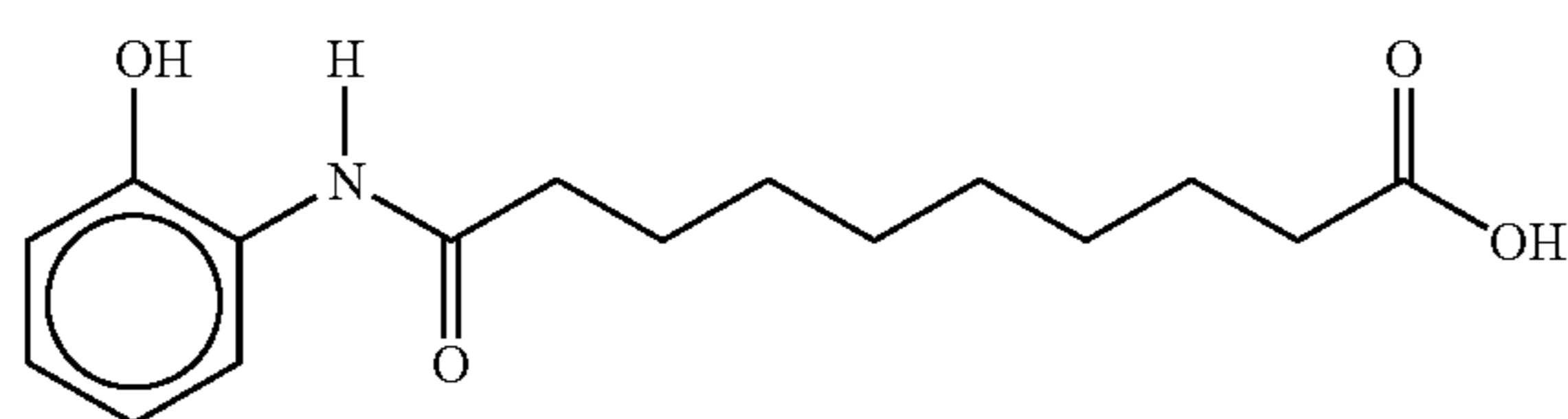
10-(N-2-Hydroxyanilino)sebacic acid
