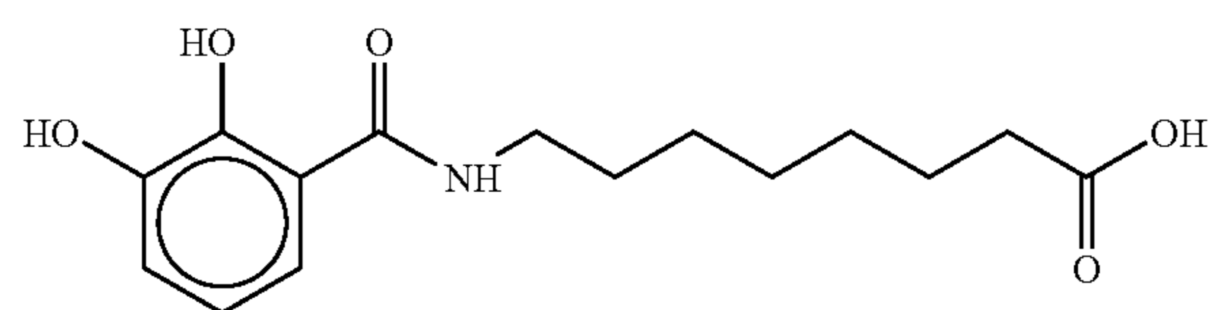
8-(N-2,3-Dihydroxybenzoyl)aminocaprylic acid
