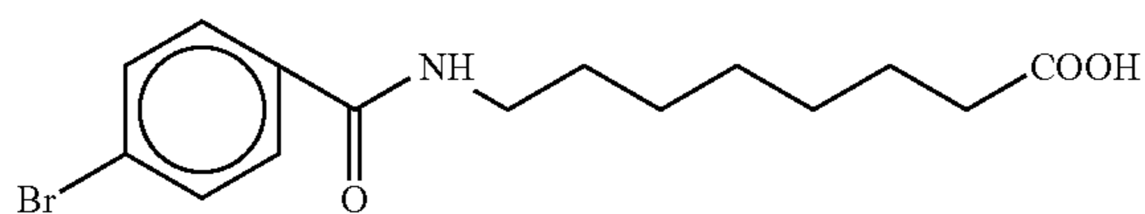
8-[N-(4-bromobenzoyl)]aminocaprylic acid
