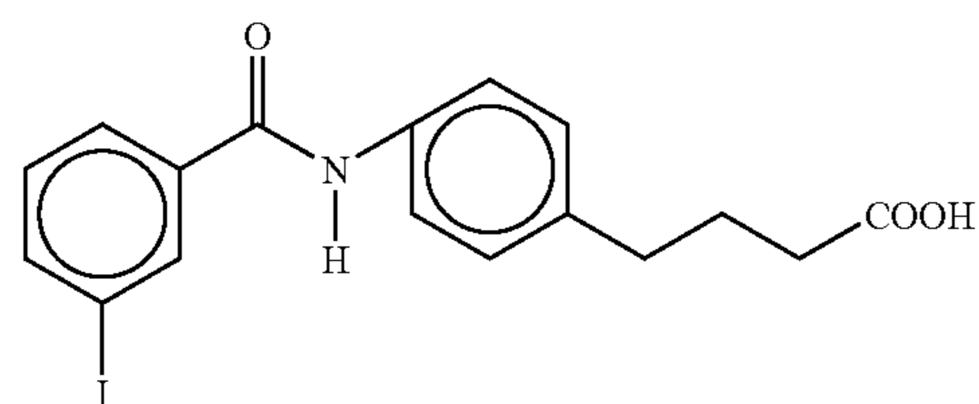
4-{N-[4-(3-iodobenzoyl)aminophenyl]}butyric acid
