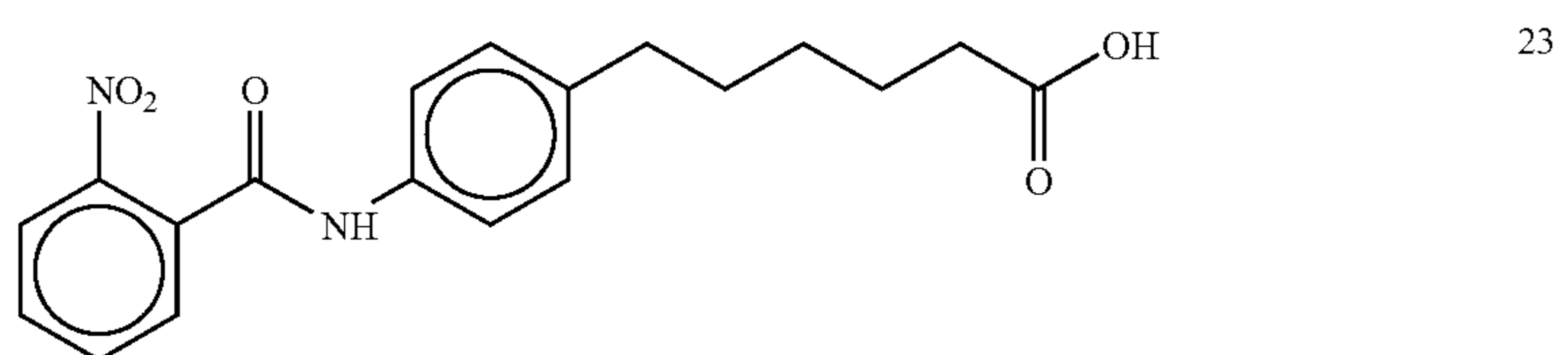
6-(4-(N-2-Nitrobenzoyl)aminophenyl)hexanoic acid
