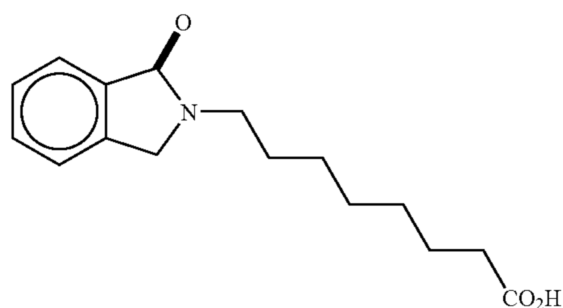
8-(2-(1,2-dihydroisindole-1-one)octanoic acid
