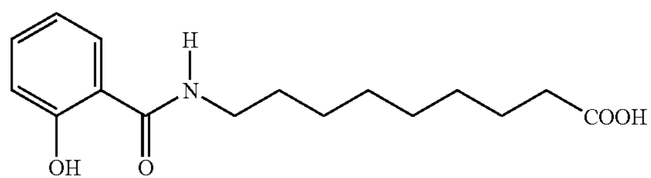
9-Salicyloylaminononanic acid
