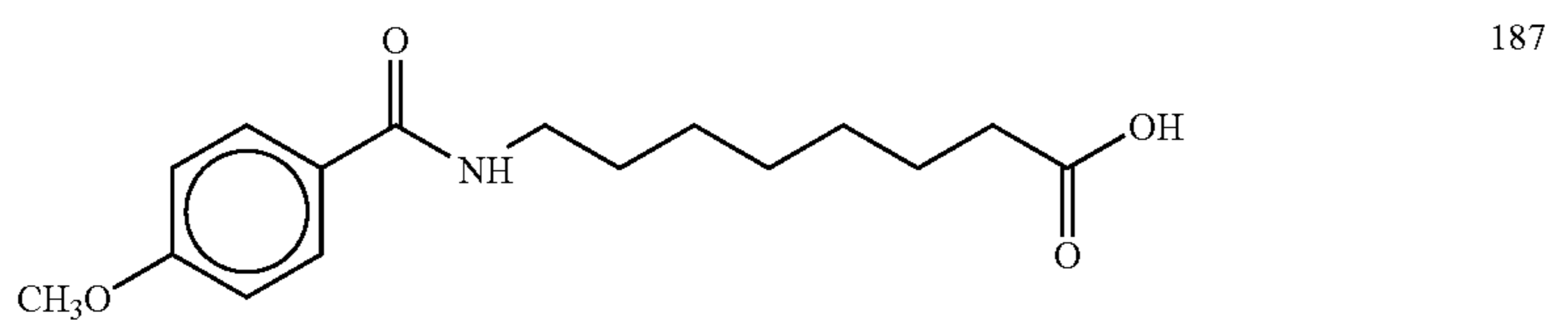
8-(p-anisoyl)aminocaprylic acid
