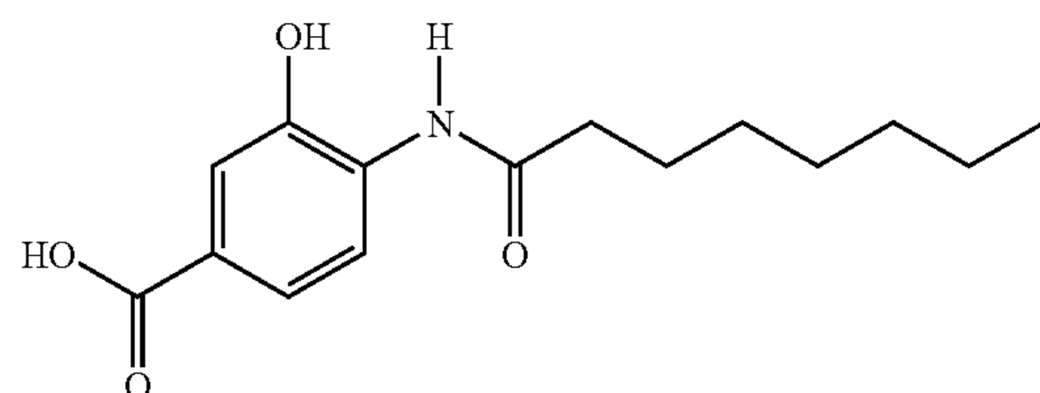
4-octylamino-3-hydroxybenzoic acid
