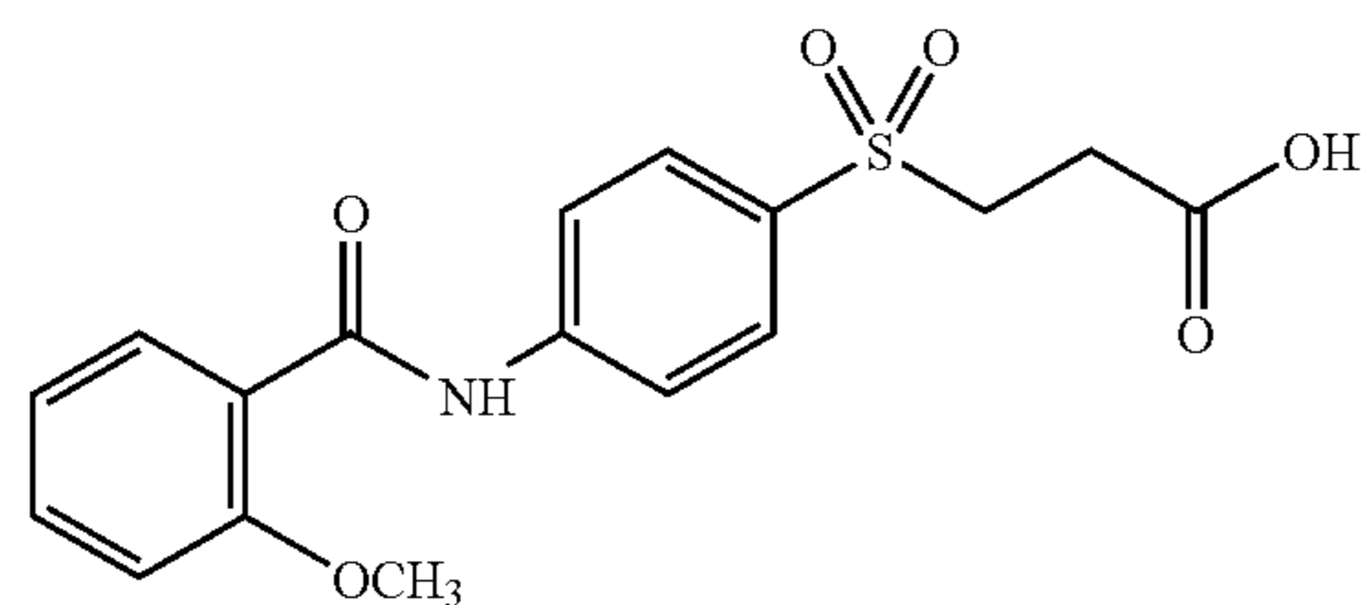
4-(2-methoxybenzoyl)amino 3-carboxypropylsulfone
