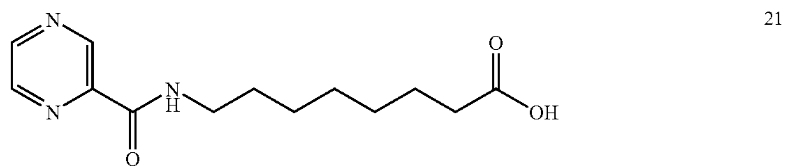
8-(2-pyrazinecarbonyl)aminocaprylic acid
