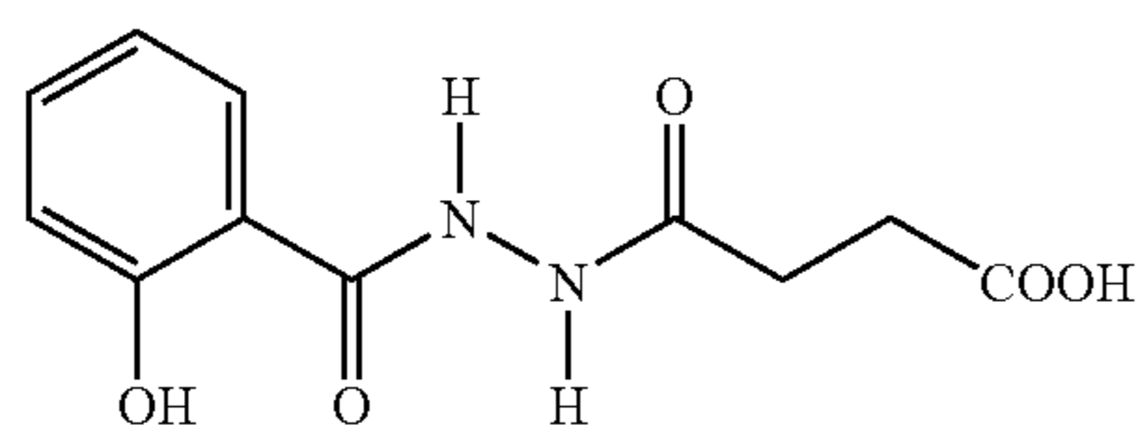
1-salicyloyl-2-succinyl hydrazide
