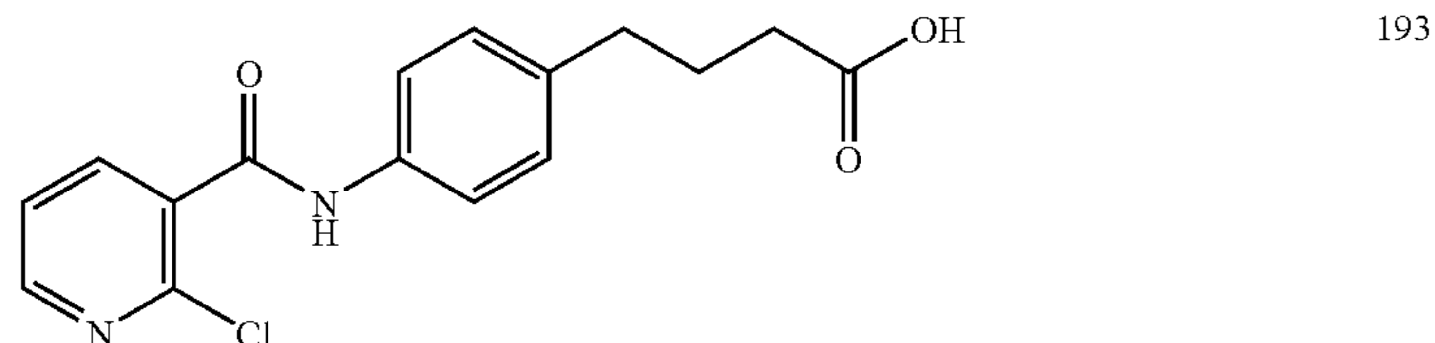
4-(4-(2-chloronicotinoyl)aminophenyl)butyric acid
