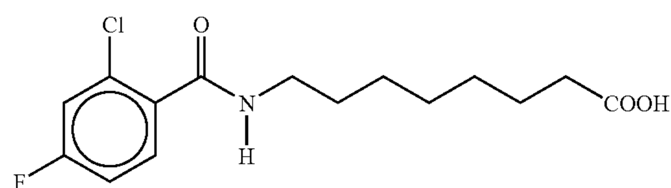
8-(N-(2-chloro-4-fluorobenzoyl)aminocaprylic acid
