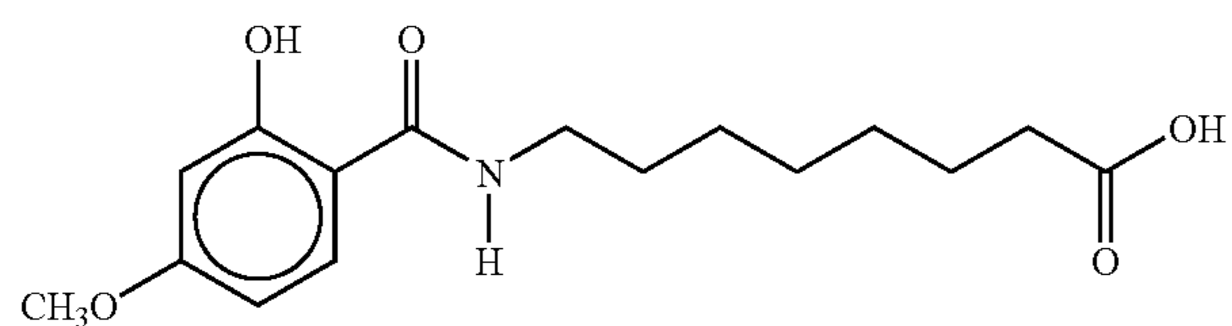
8-(N-(2-Hydroxy-4-methoxybenzoyl)aminocaprylic acid
