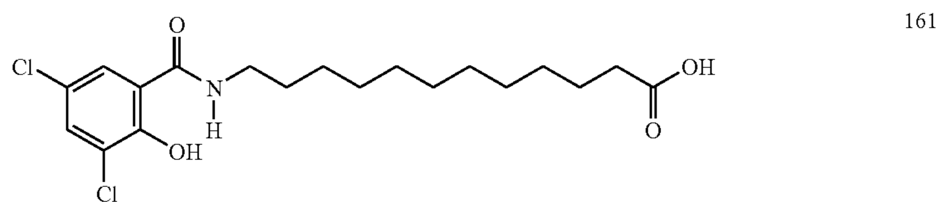
12-N-(3,5-dichloro-2-hydroxybenzoyl)aminododecanoic acid
