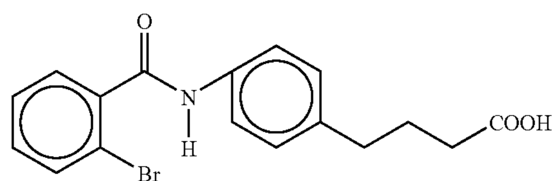
4-[4-[N-(2-bromobenzoyl)]aminophenyl]butyric acid
