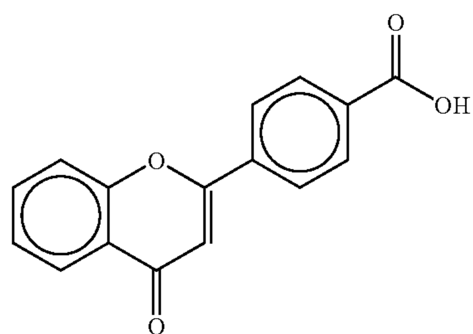
4'-flavonic acid
