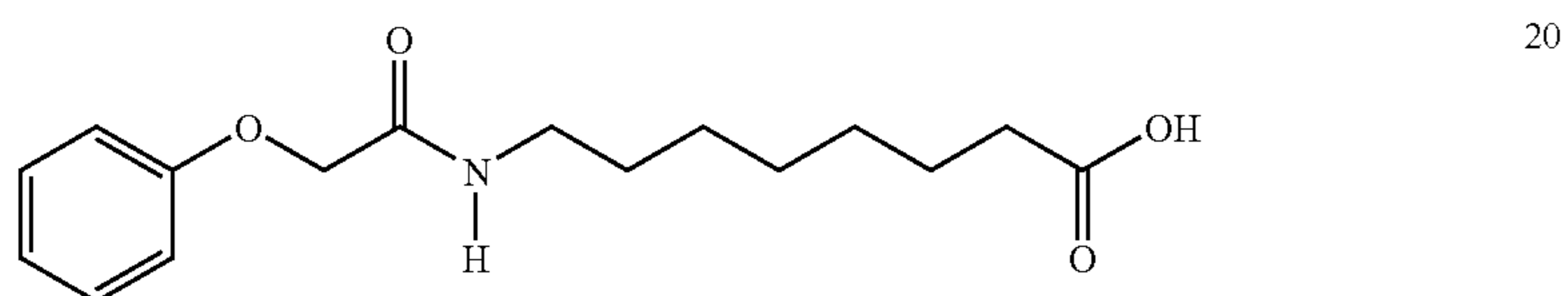
8-(Phenoxyacetyl)caprylic acid
