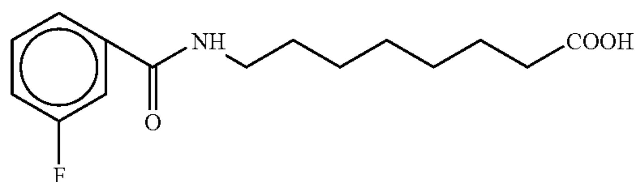
8-[N-(3-fluorobenzoyl)]aminocaprylic acid
