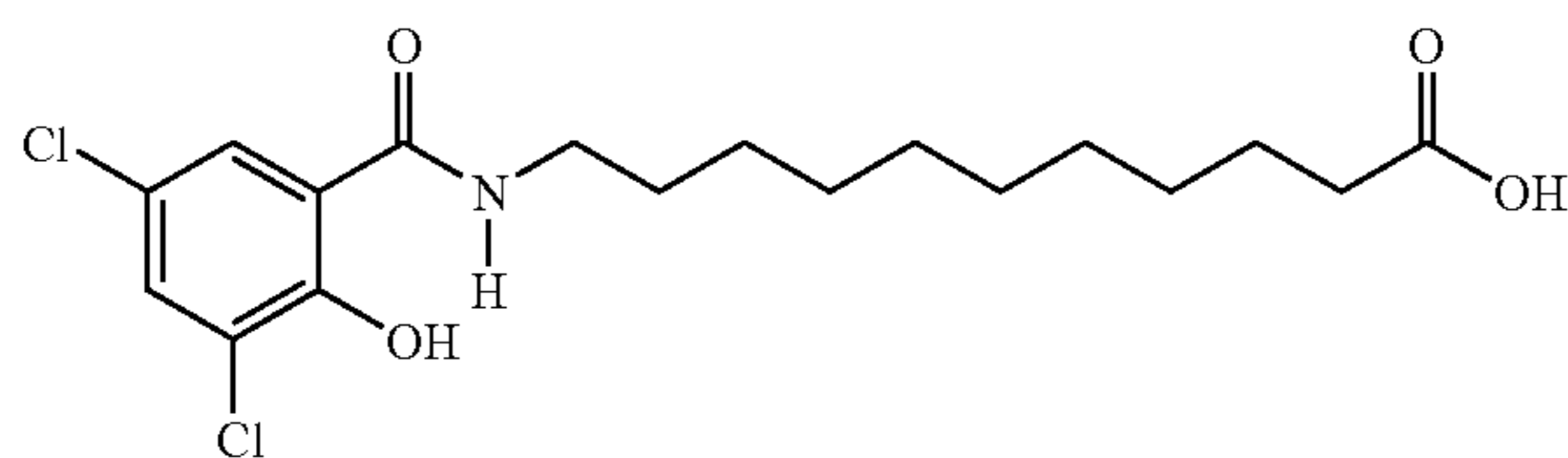
11-N-(3,5-dichloro-2-hydroxybenzoyl)aminoundecanoic acid
