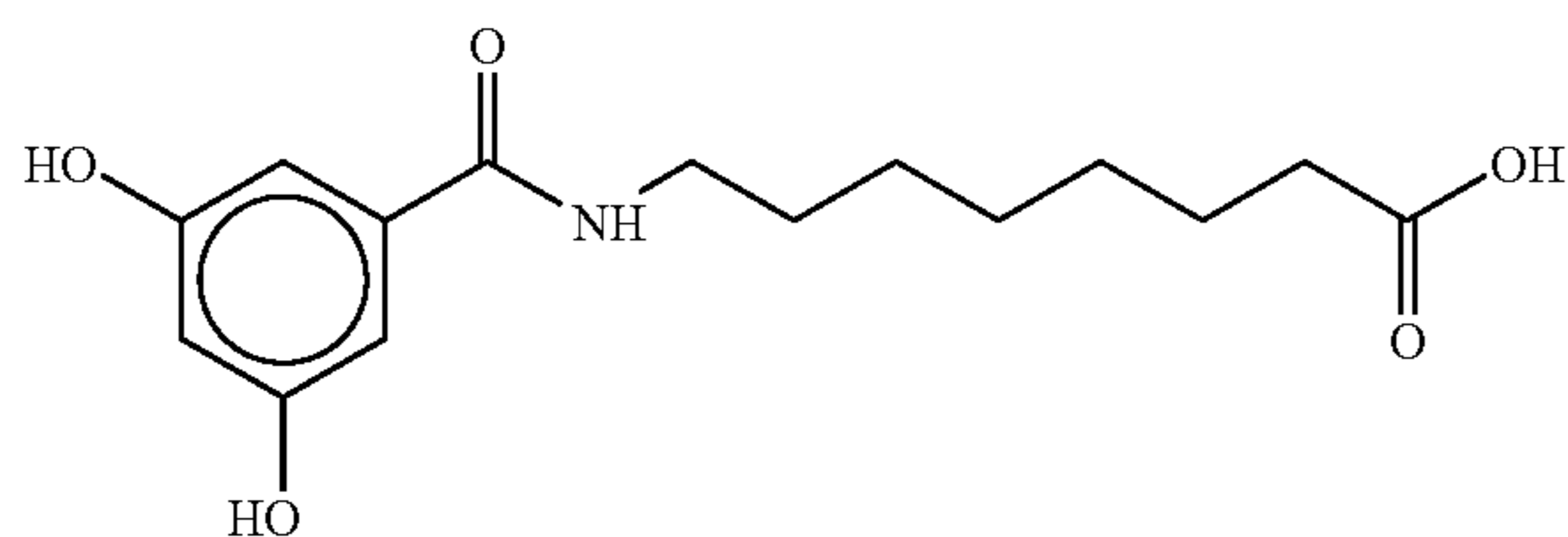
8-(N-3,5-Dihydroxybenzoyl)aminocaprylic acid
