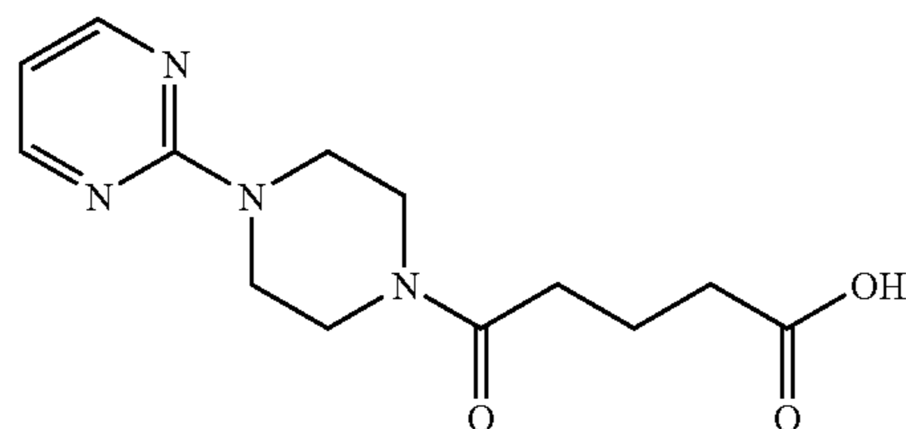
4-(1-(2-pyrimidyl)piperazinoyl)butyric acid
