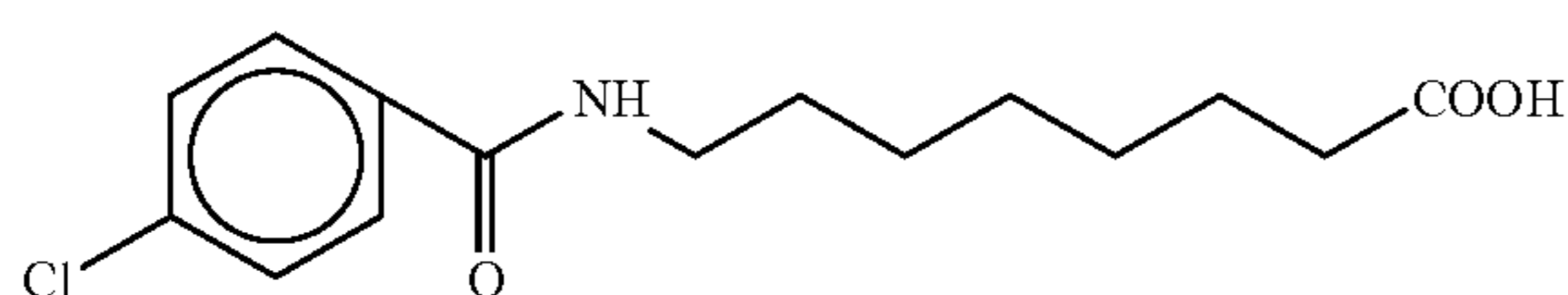
8-[N-(4-chlorobenzoyl)]aminocaprylic acid
