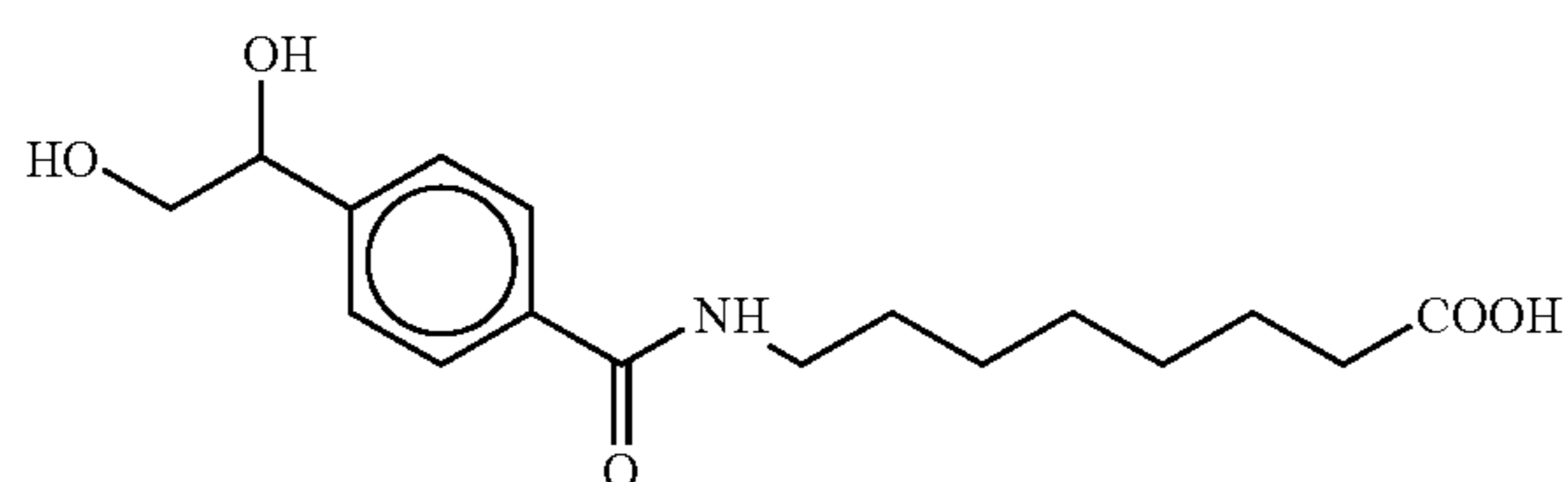
8-(4-(1,2-dihydroxyethyl)benzoyl)aminocaprylic acid
