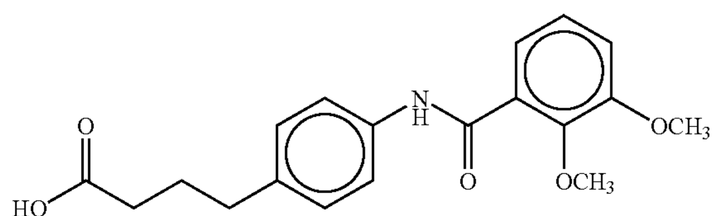
4-(4-(2,3-dimethoxybenzoyl)aminophenyl)butyric acid
