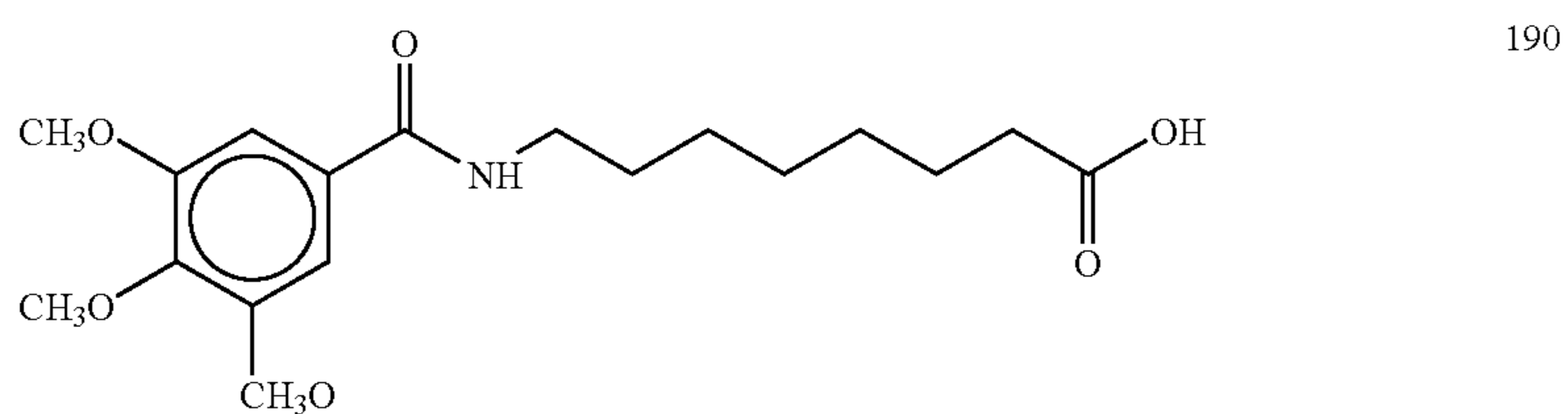
8-(3,4,5-Trimethoxybenzoyl)aminocaprylic acid
