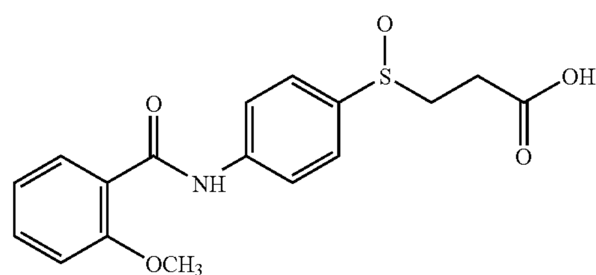
4-(2-methoxybenzoyl)amino 3-carboxysulfoxide
