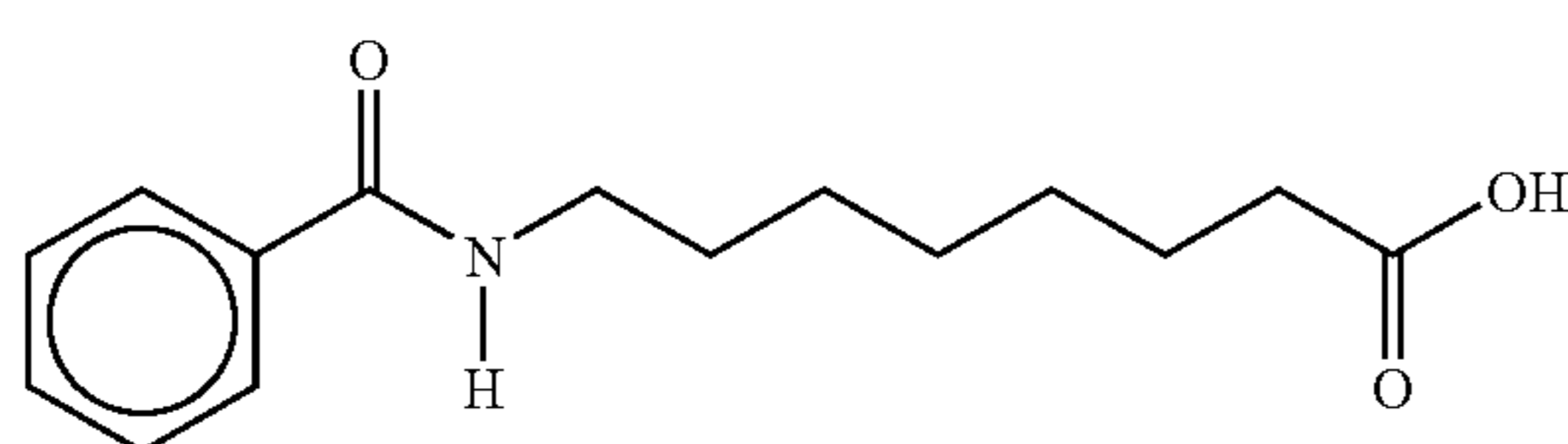
8-(N-benzoyl)aminocaprylic acid
