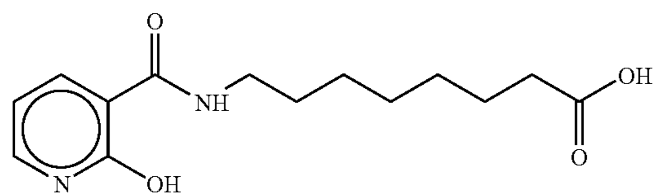
8-(2-Hydroxynicotinoyl)aminocaprylic acid
