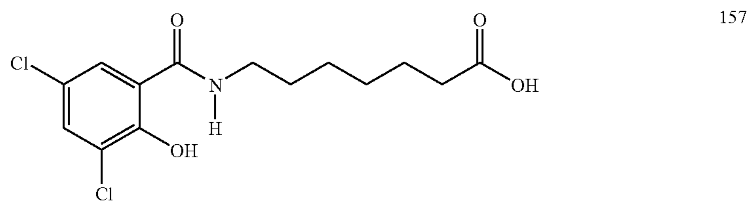
7-N-(3,5-dichloro-2-hydroxybenzoyl)aminoheptanoic acid
