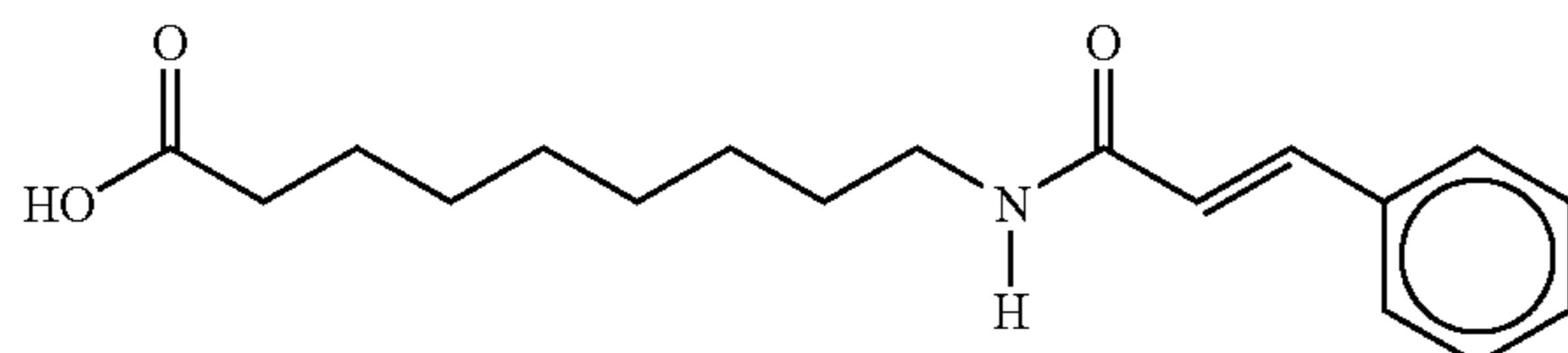
9-(cinnamoylamino)nonanoic acid
