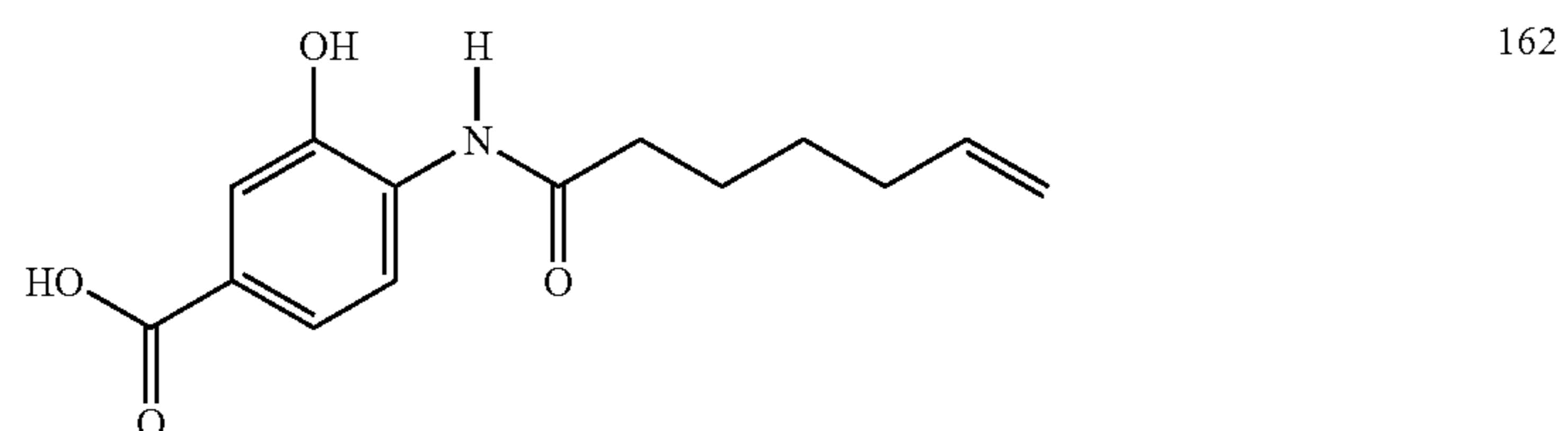
N-(2-hydroxy-4-carboxy)-6-heptenamide
