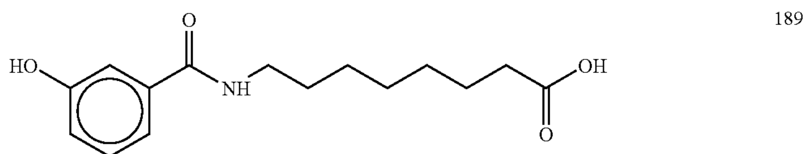
8-(3-Hydroxybenzoyl)aminocaprylic acid
