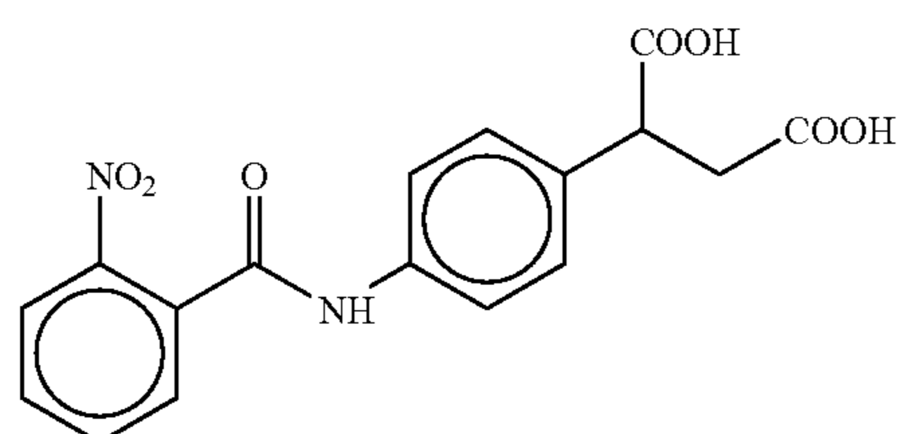
4-(2-Nitrobenzoyl)aminophenylsuccinic acid
