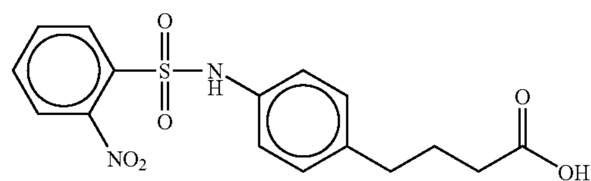
4-(4-(2-nitrobenzenesulfonyl)aminophenyl)butyric acid
