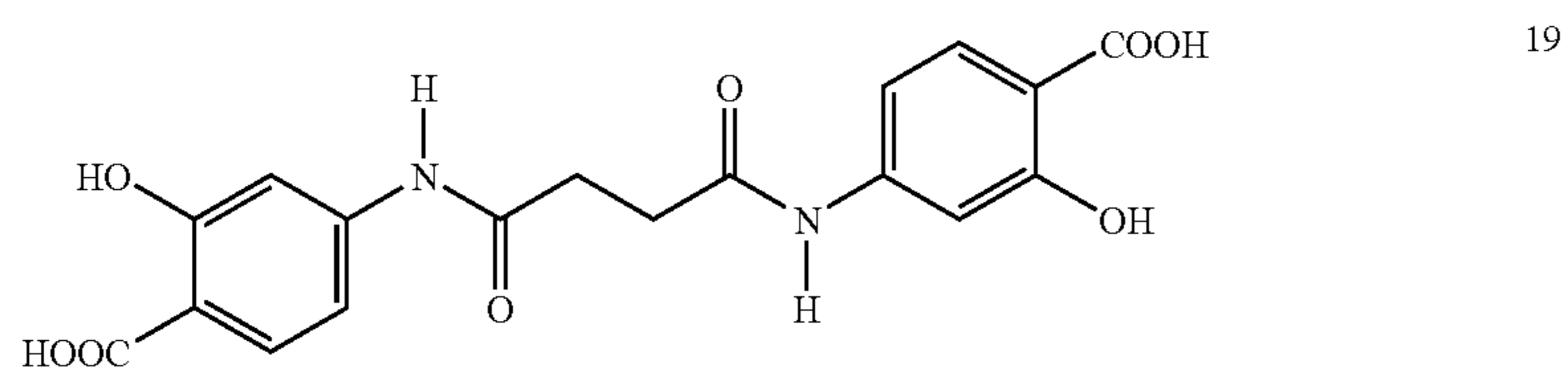
Succinyl-4-aminosalicylic acid
