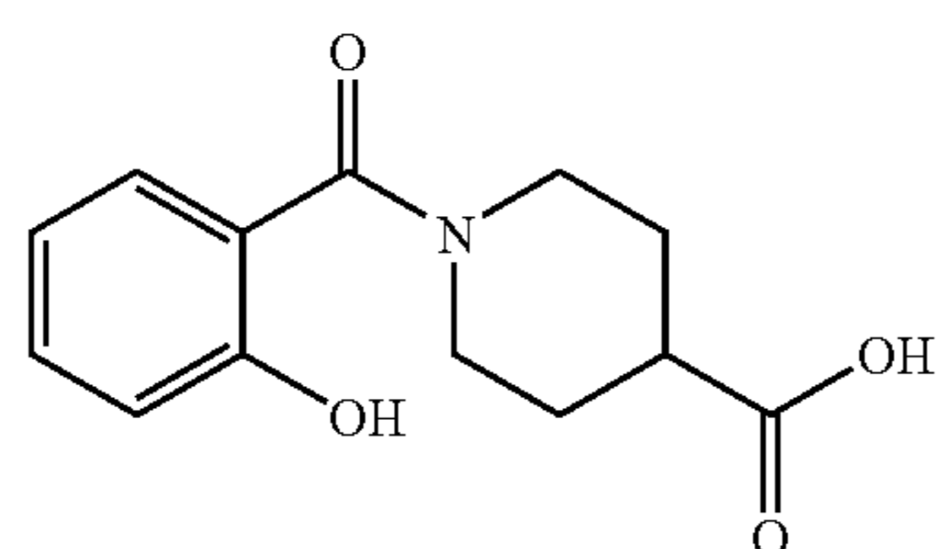
N-(2-hydroxybenzoyl)isonipecotic acid
