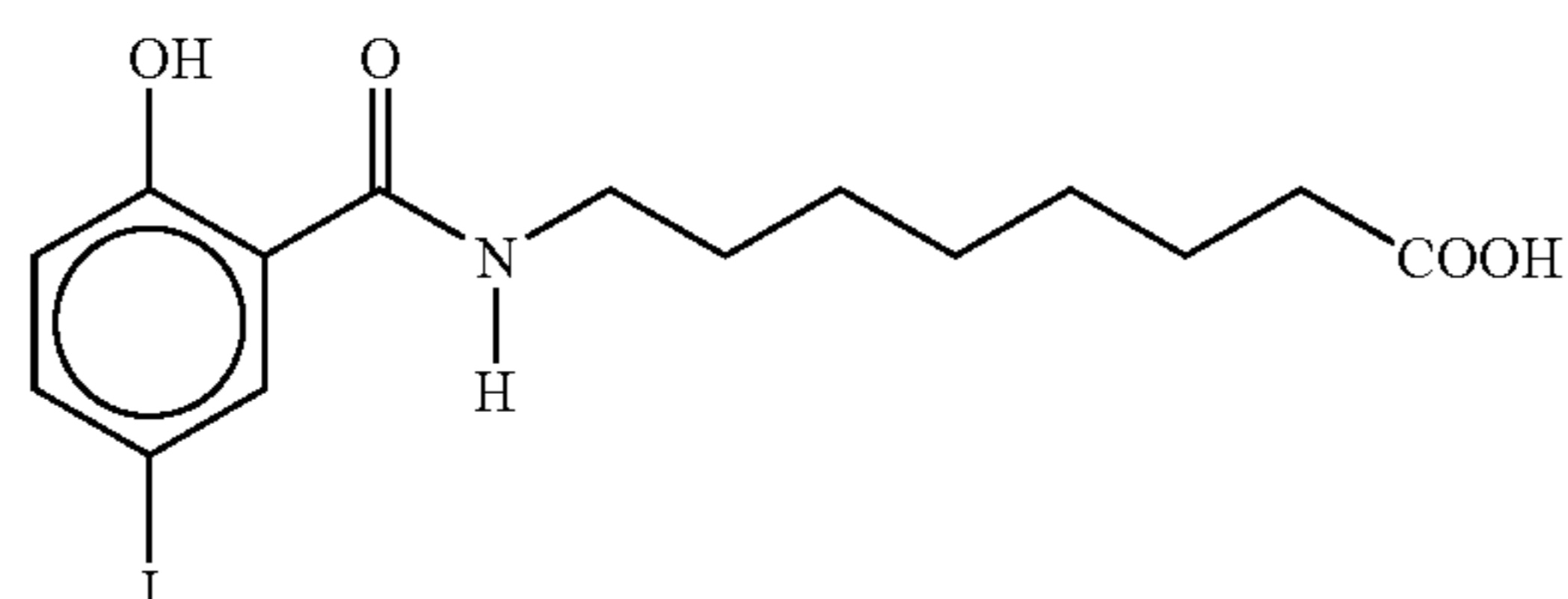
8-(N-2-hydroxy-5-iodobenzoyl)aminocaprylic acid
