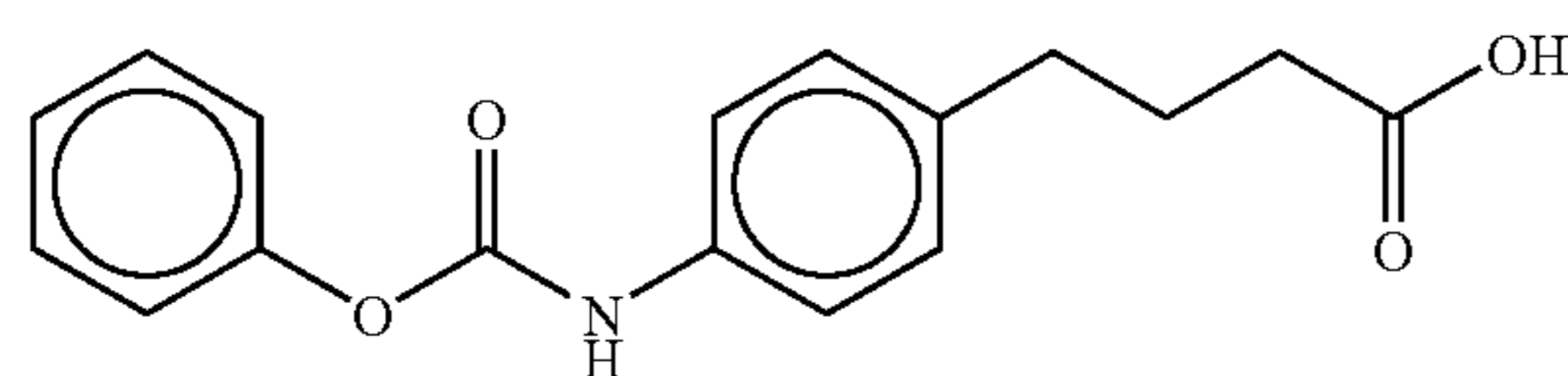
4-(4-phenyloxycarbonylaminophenyl)butyric acid
