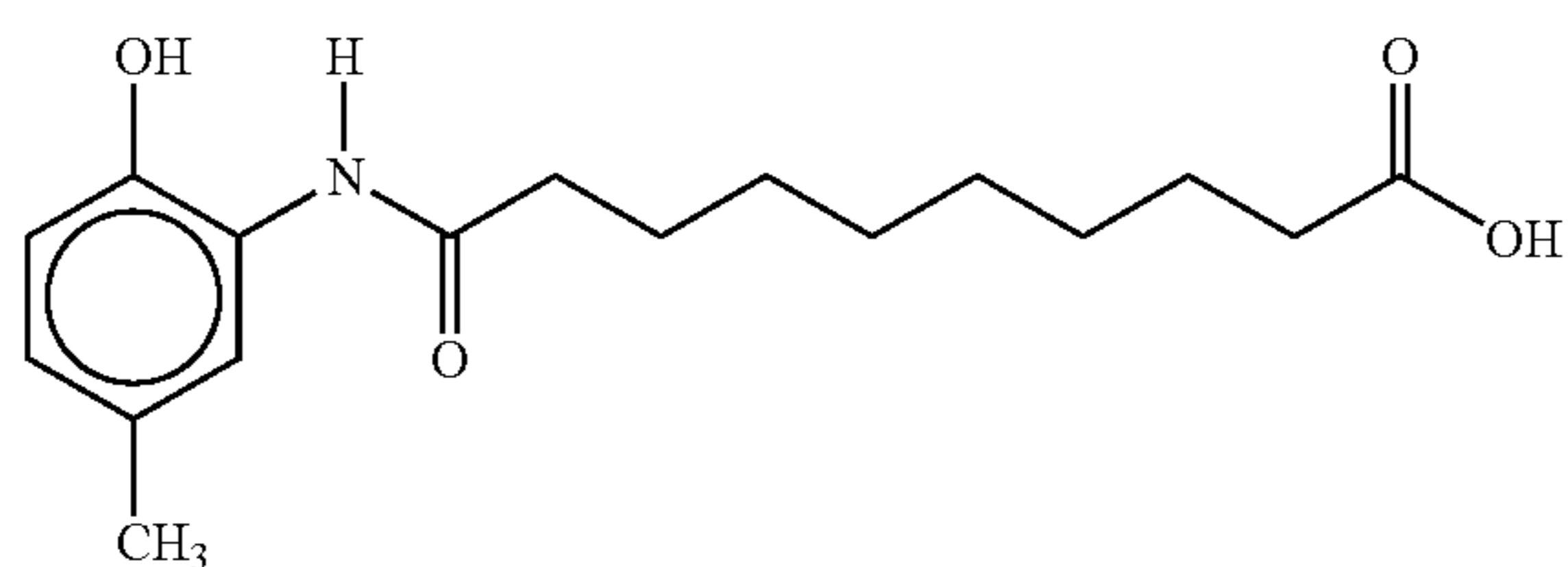
9-(2-hydroxy-5-methylanilino)nonanoic acid
