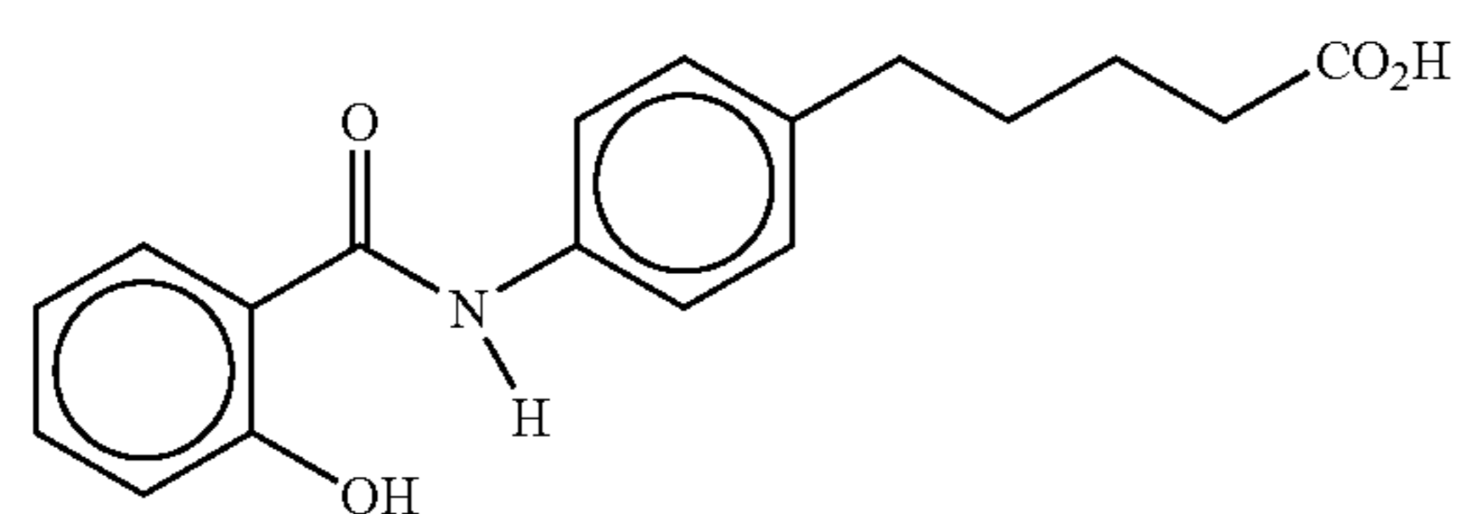
N-salicyloyl-5-(4-aminophenyl)valeric acid
