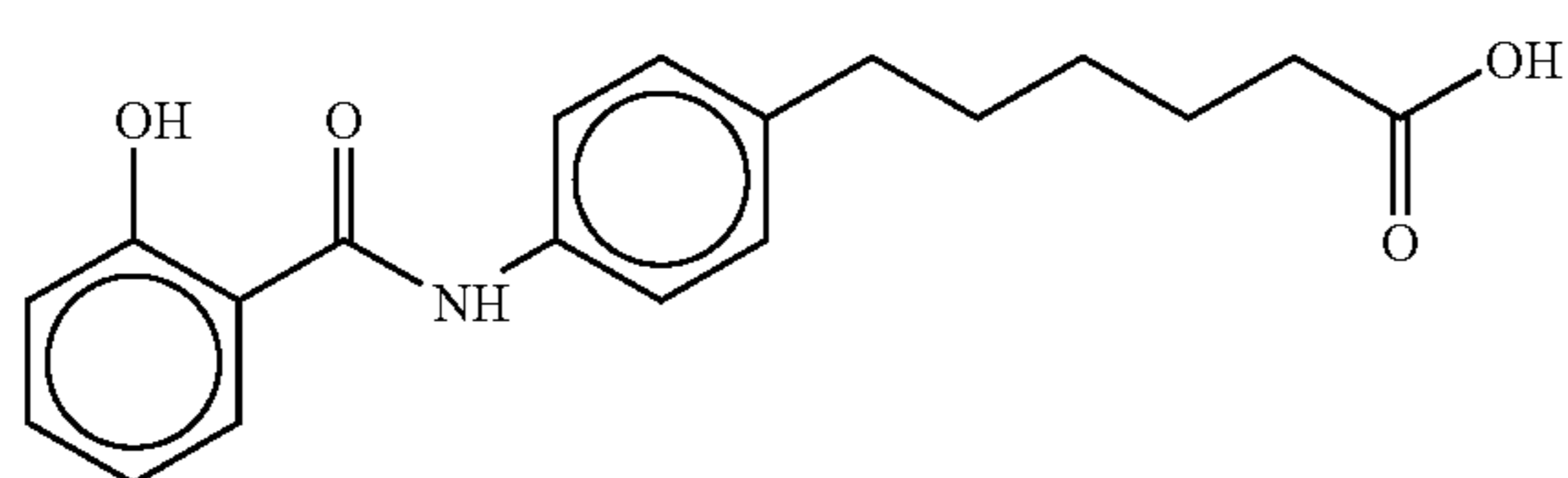
6-(4-(salicyloyl)amino)phenyl)hexanoic acid
