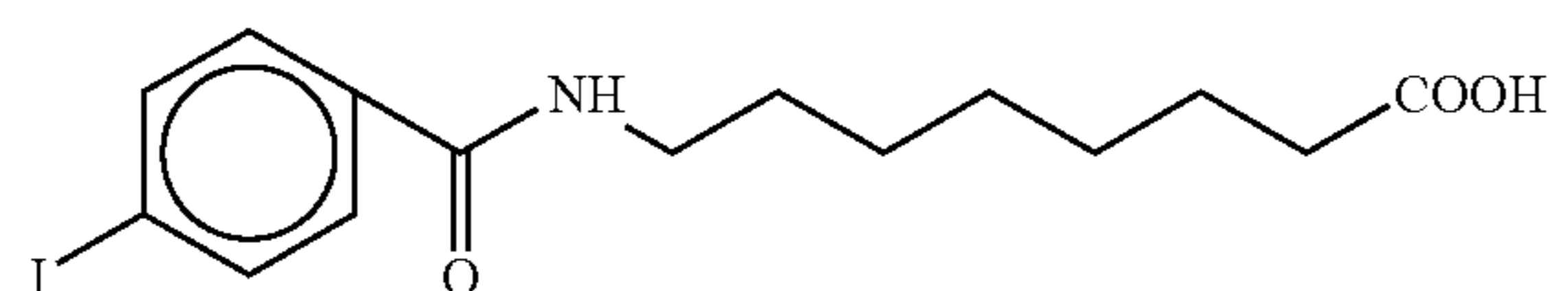
8-[N-(4-iodobenzoyl)]aminocaprylic acid
