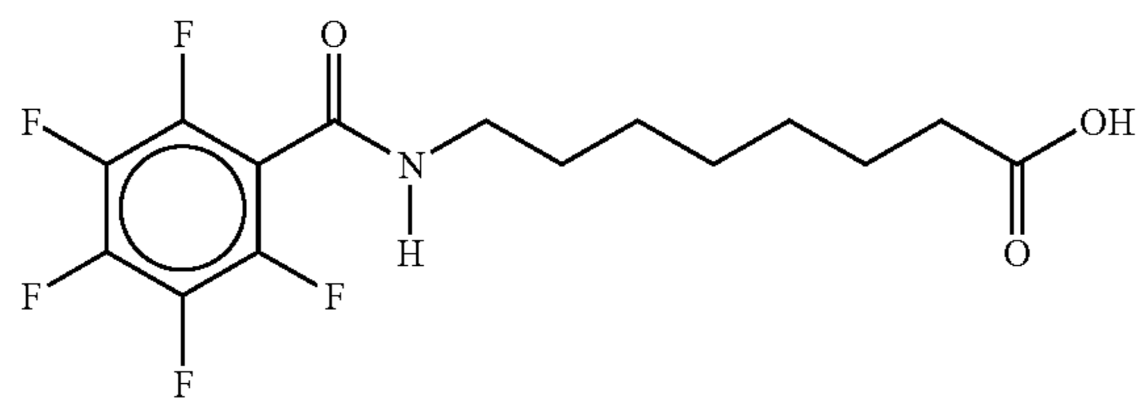
8-(pentafluorobenzoyl)aminocaprylic acid
