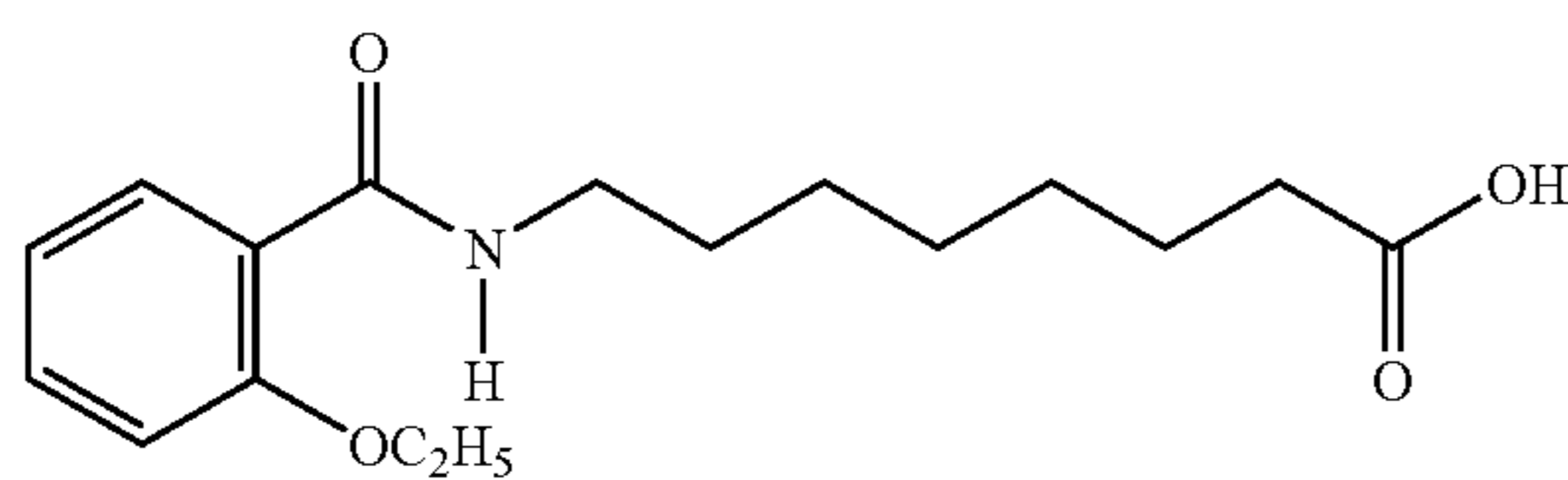
8-(2-ethoxybenzoyl)aminocaprylic acid
