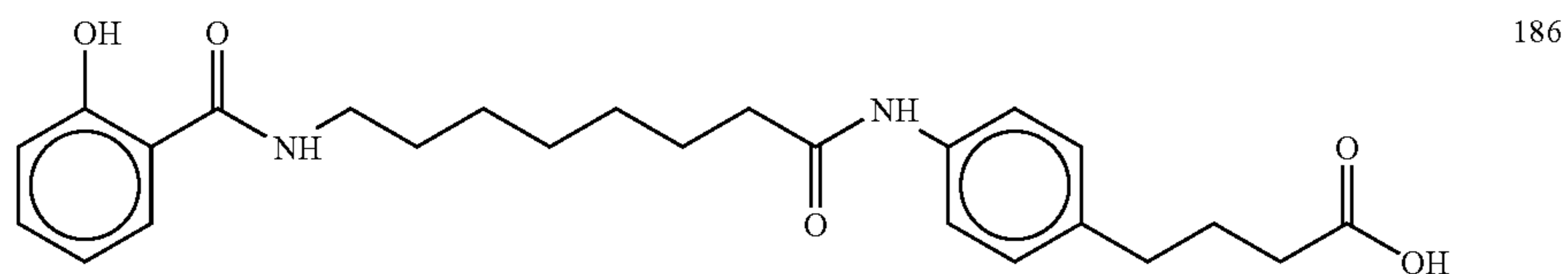
4-(4-(N-8(N-Salicyloyl)aminocaprylic)aminophenyl)butyric acid
