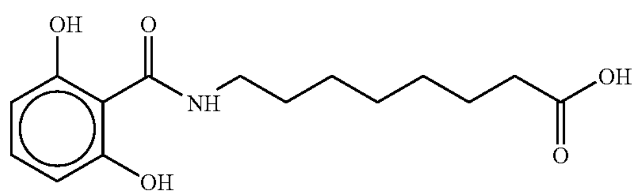
8-(N-2,6-Dihydroxybenzoyl)aminocaprylic acid
