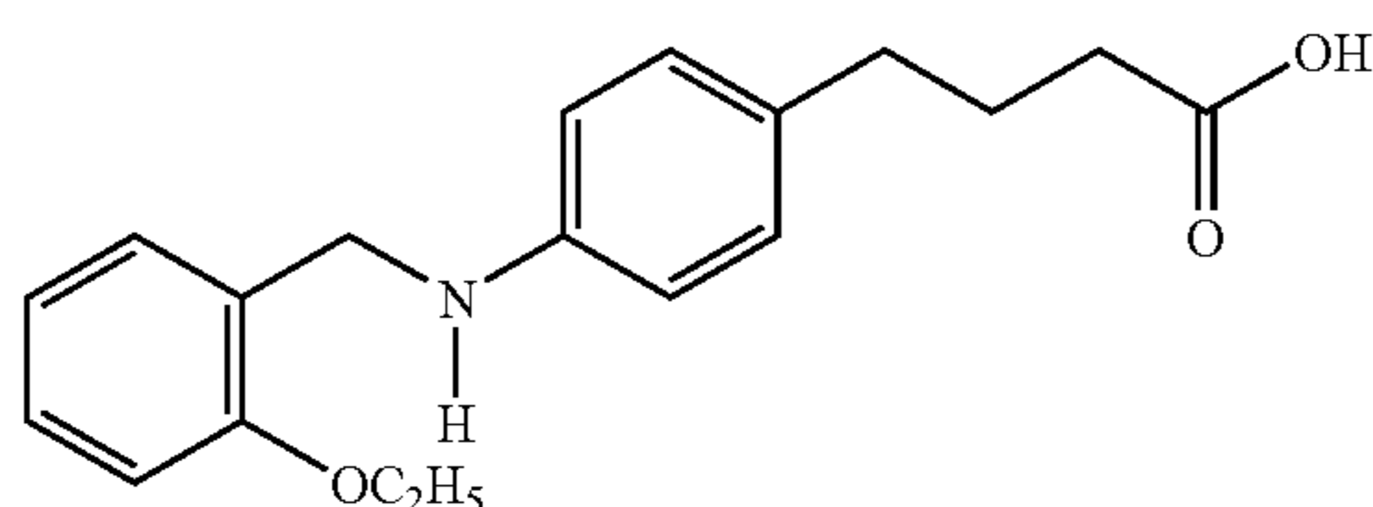
4-(4-(2-ethoxybenzoyl)aminophenyl)butyric acid
