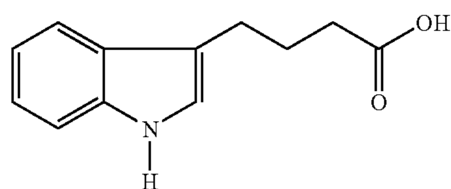
3-indolebutyric acid
