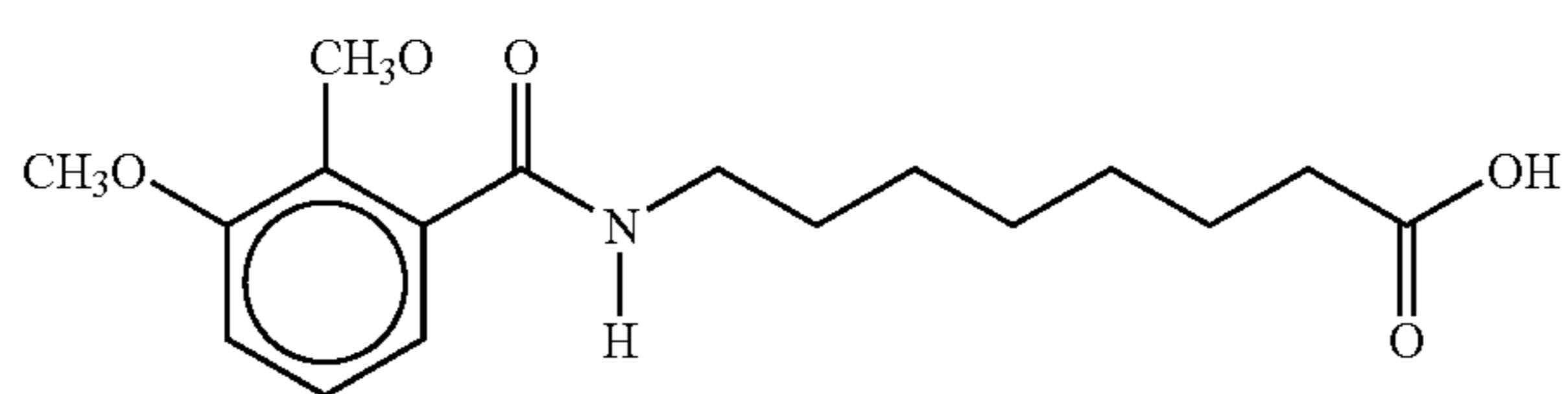
8-(N-2,3-Dimethoxybenzoyl)aminocaprylic acid
