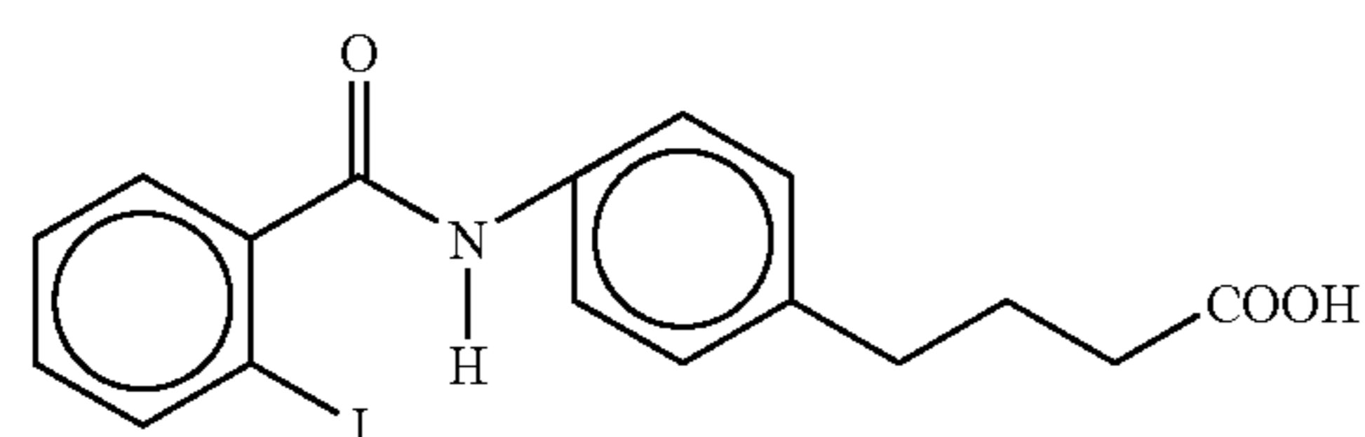
4-{4-[N-(2-iodobenzoyl)aminophenyl]}butyric acid
