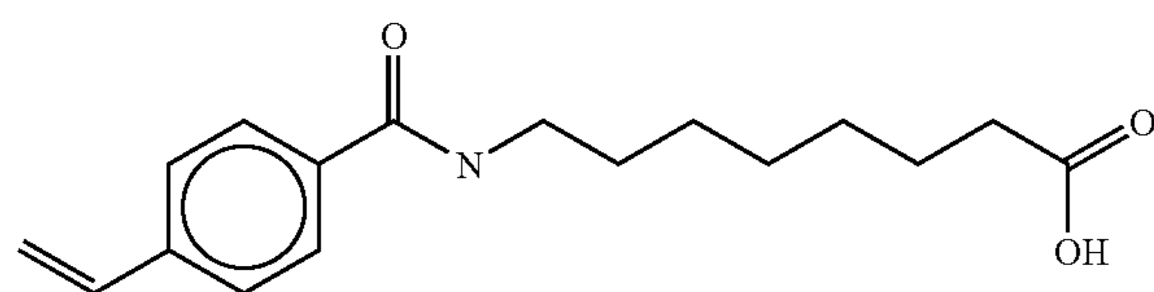
8-(vinylbenzoyl)aminocaprylic acid
