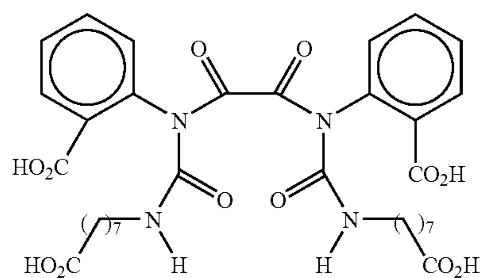
Bis(N-2-carboxylphenyl-N-(N'-8-octanoic acid)urea)oxalyl diamide
