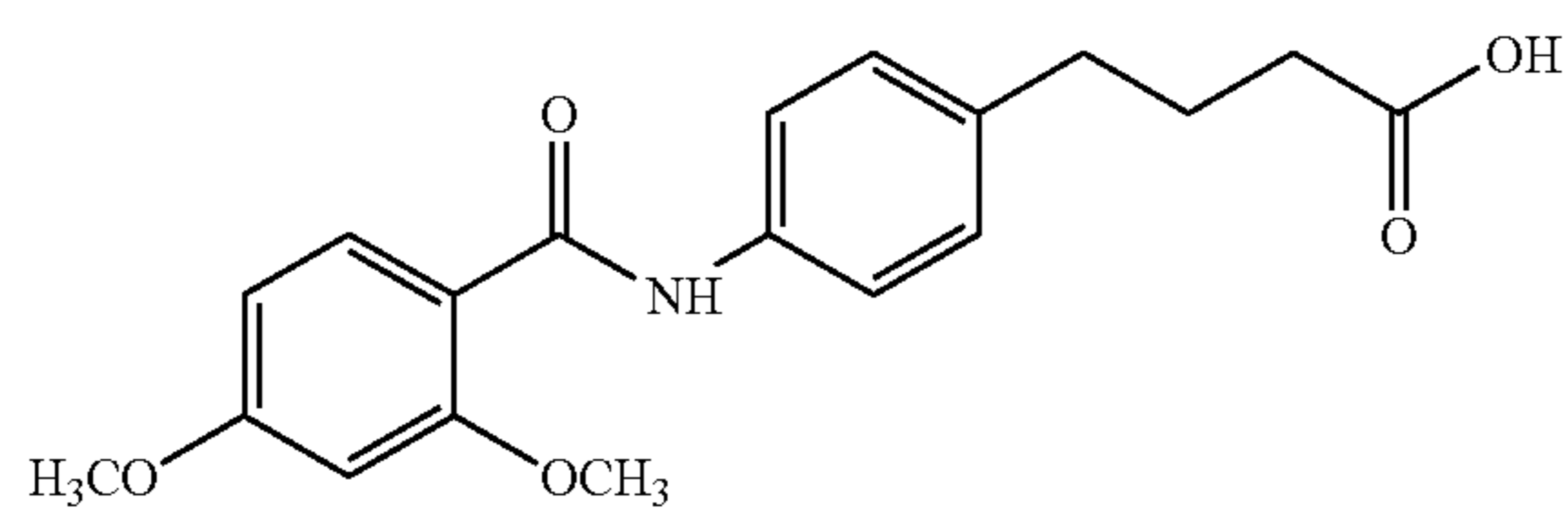
4-(4-(2,4-dimethoxybenzoyl)aminophenyl)butyric acid
