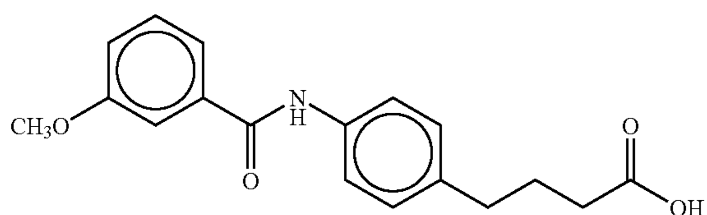
4-(4-(3-anisoyl)aminophenyl)butyric acid
