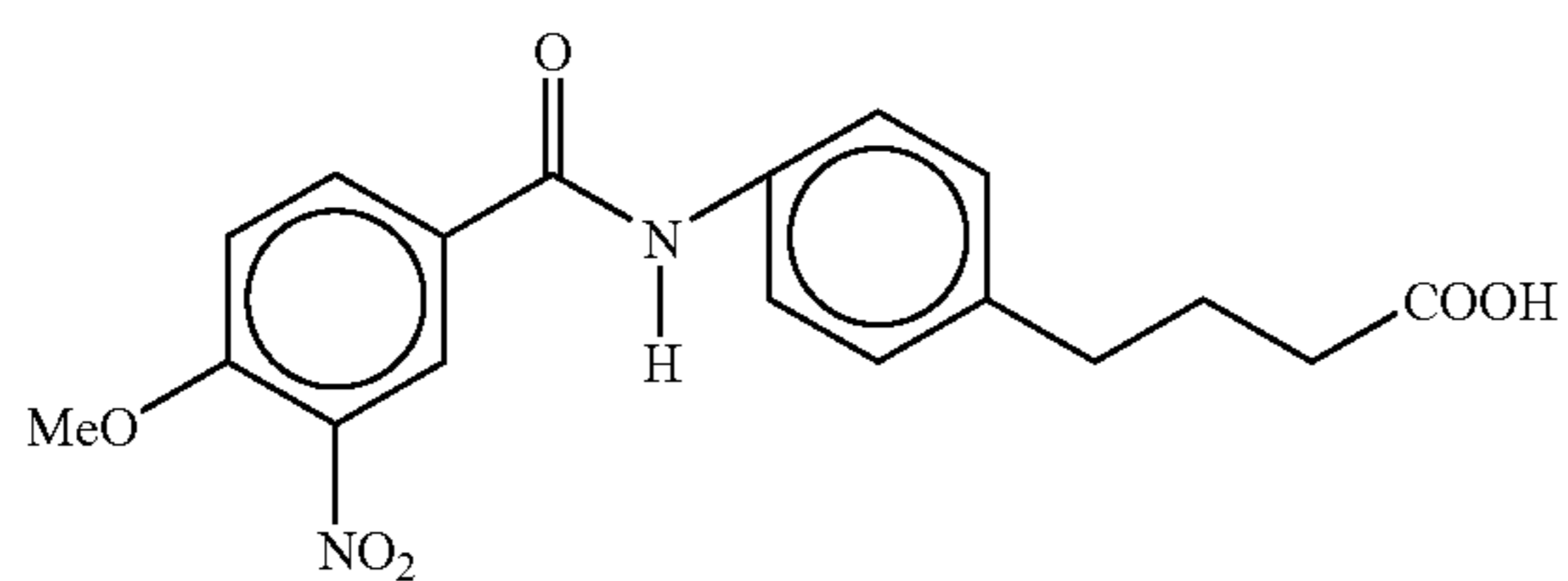
4-[4-N-(4-methoxy-3-nitrobenzoyl)aminophenyl]butyric acid
