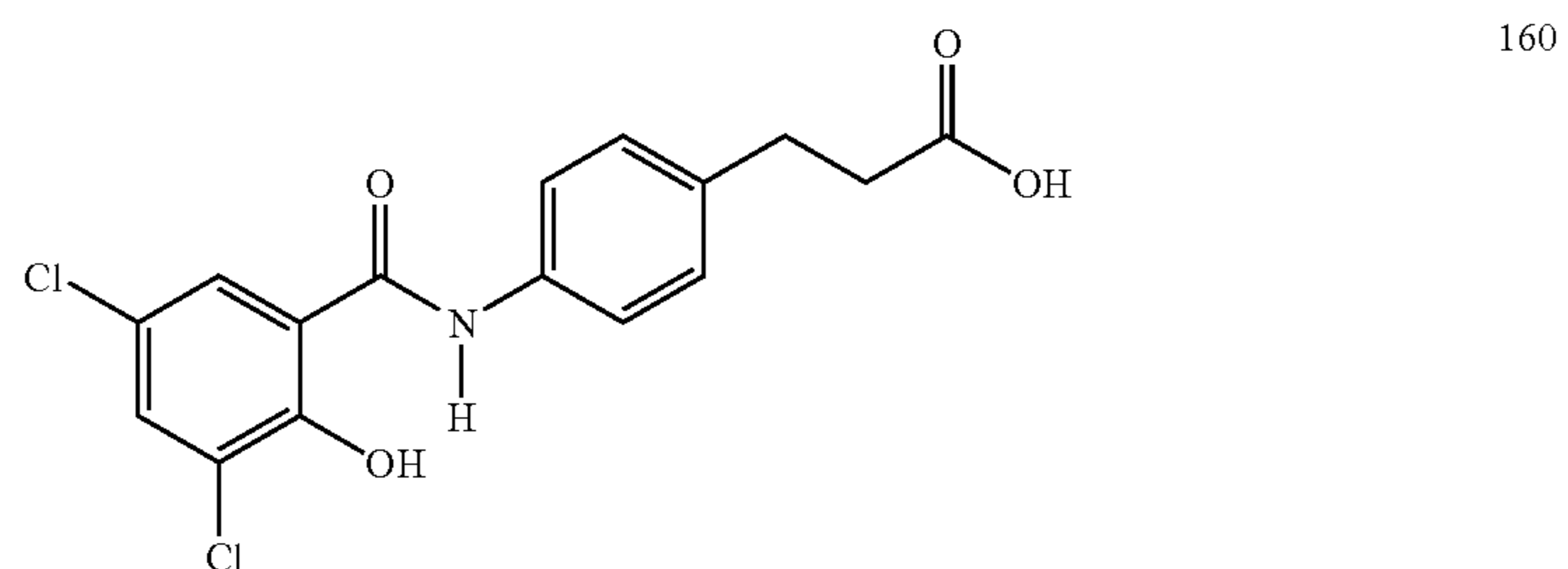
N-[3,5-dichloro-2-hydroxybenzoyl-3-(4-aminophenyl)]propionic acid
