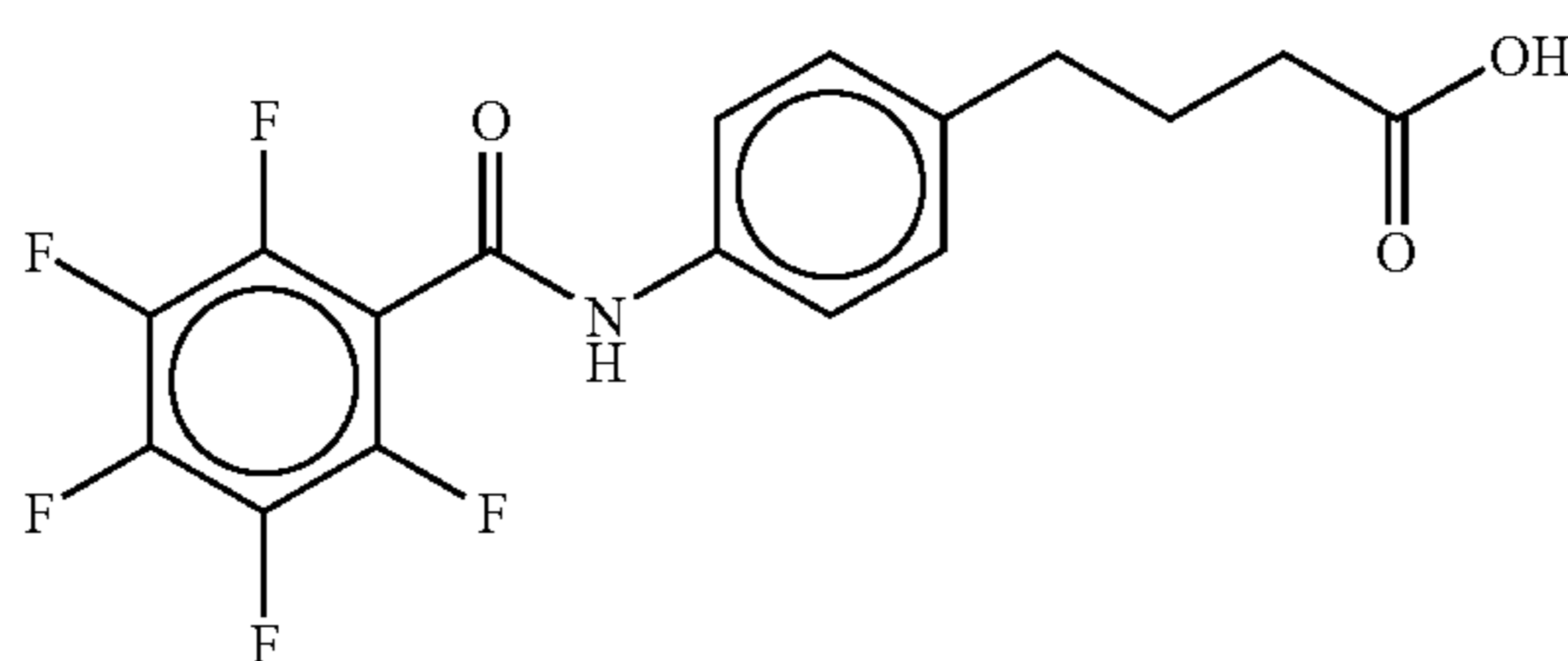
4-(4-(pentafluorobenzoyl)aminophenyl)butyric acid
