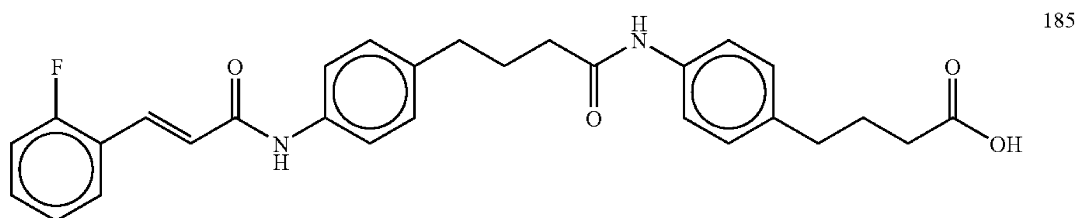
4-(4-(N-(2-Fluorocinnamoyl))aminophenyl) butyric
