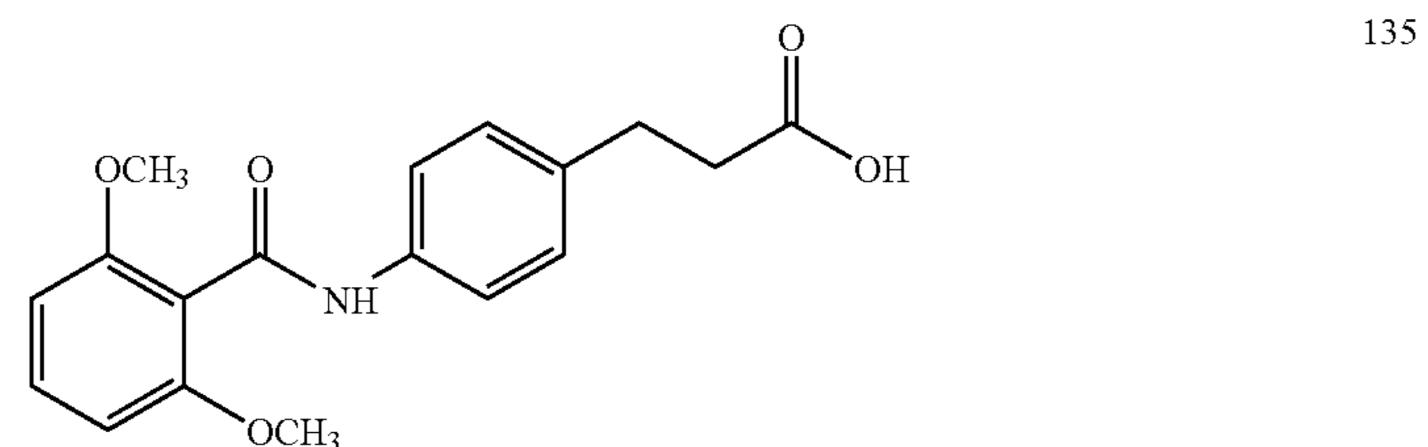
3-(4-(2,6-dimethoxybenzoyl)aminophenyl)propanoic acid
