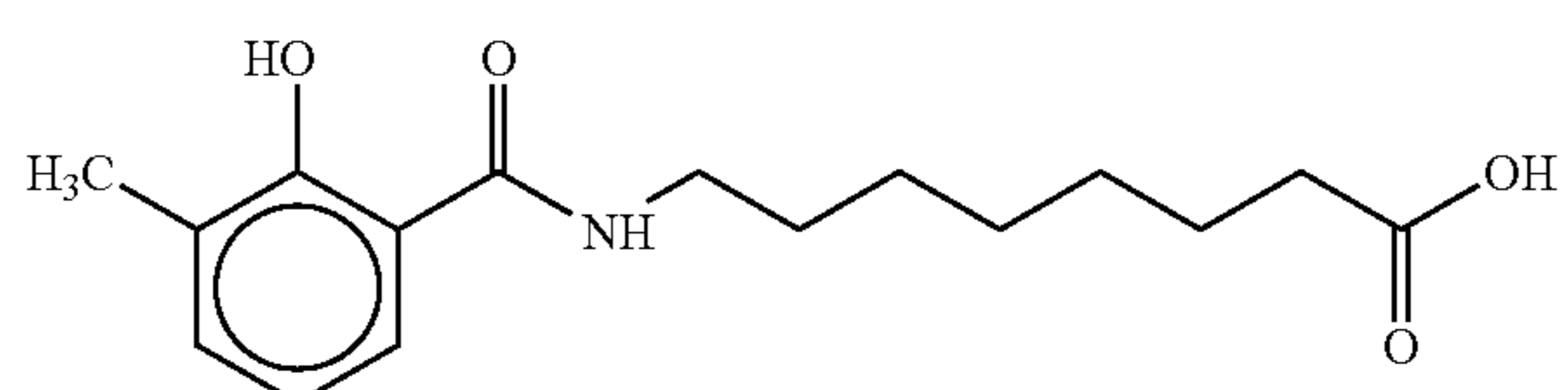
8-(N-3-methylsalicyloyl)aminocaprylic acid
