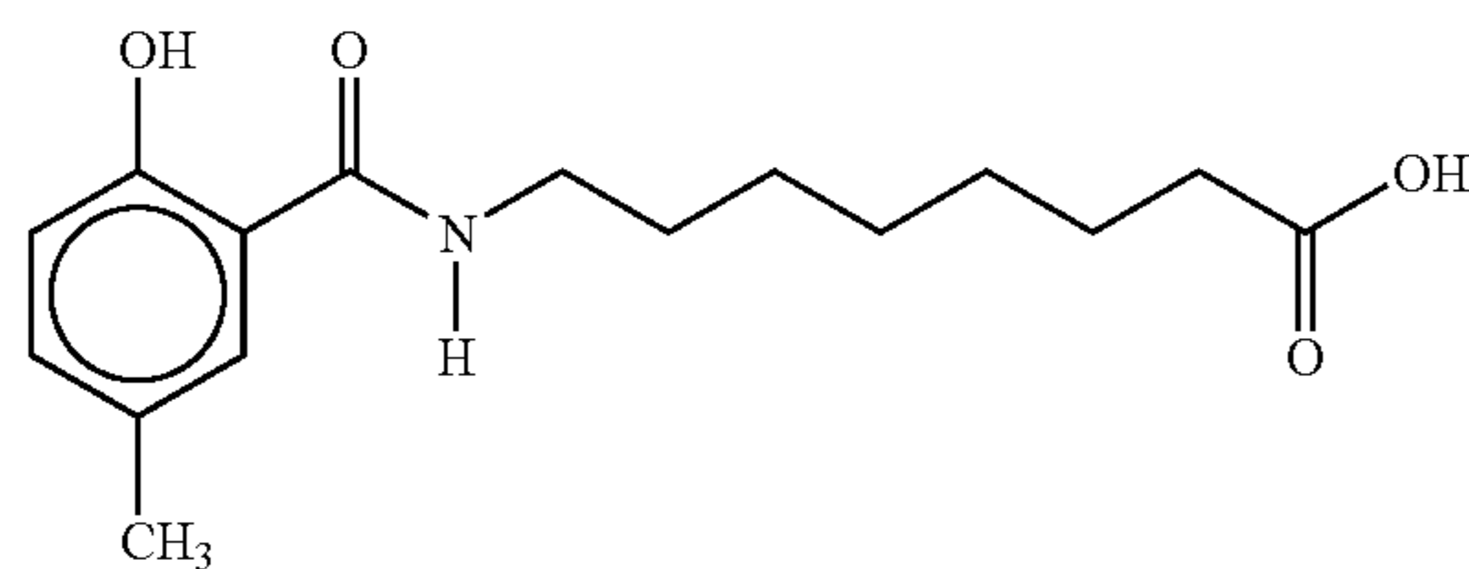
8-(N-5-methylsalicyloyl)aminocaprylic acid
