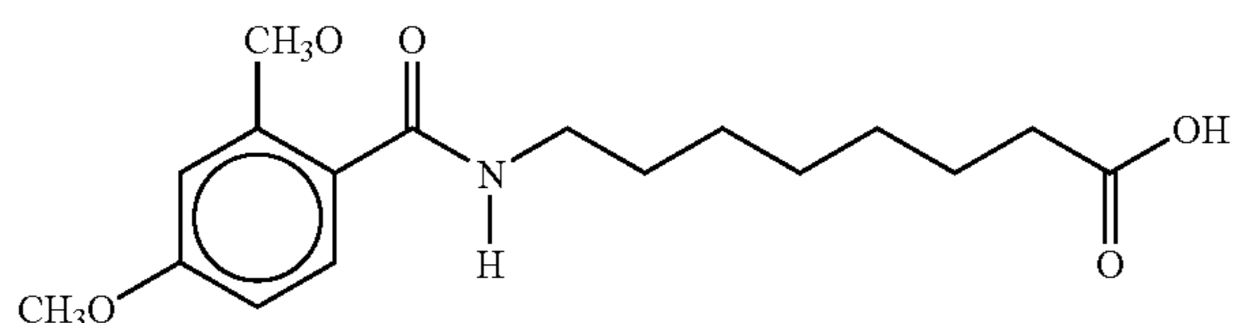
8-(N-2,3-Dimethoxybenzoyl)aminocaprylic acid
