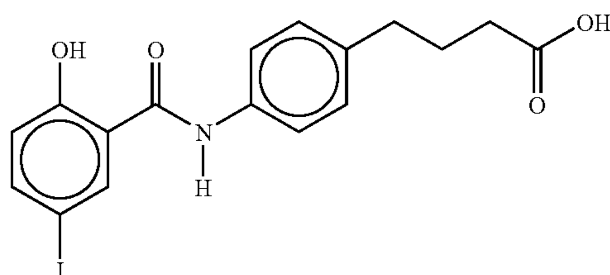
4-{-[N-(2-hydroxy-5-iodobenzoyl)]aminophenyl}butyric acid
