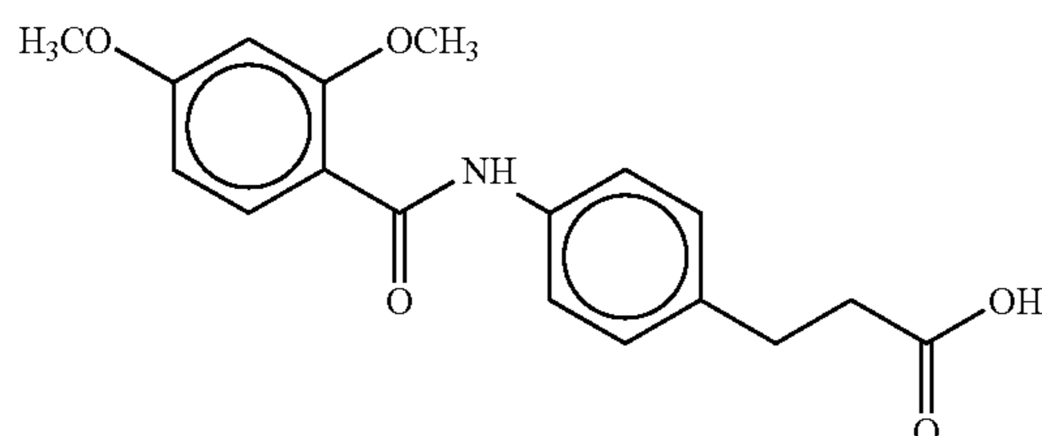
3-[4-(2,4-dimethoxybenzoyl)aminophenyl]propionic acid
