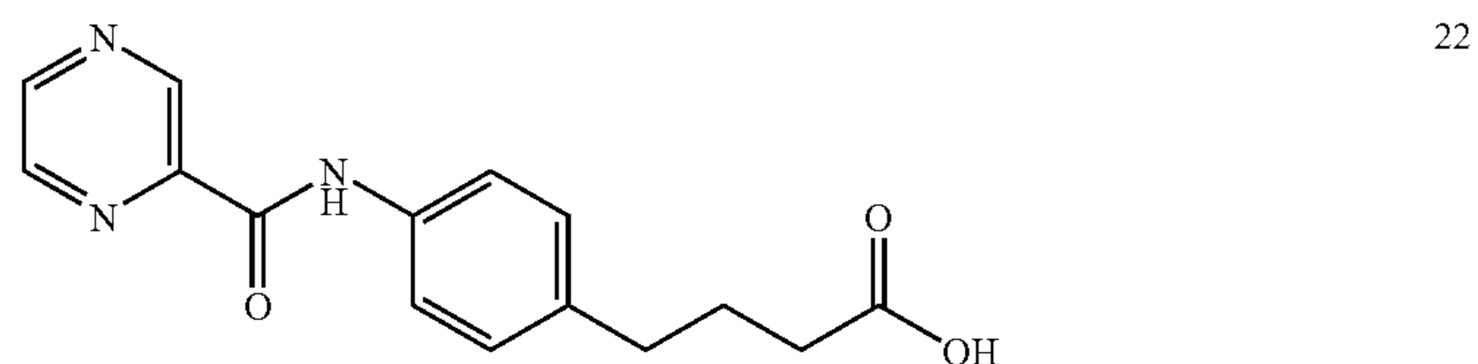
4-(4-(2-pyrazinecarbonyl)aminophenyl)butyric acid
