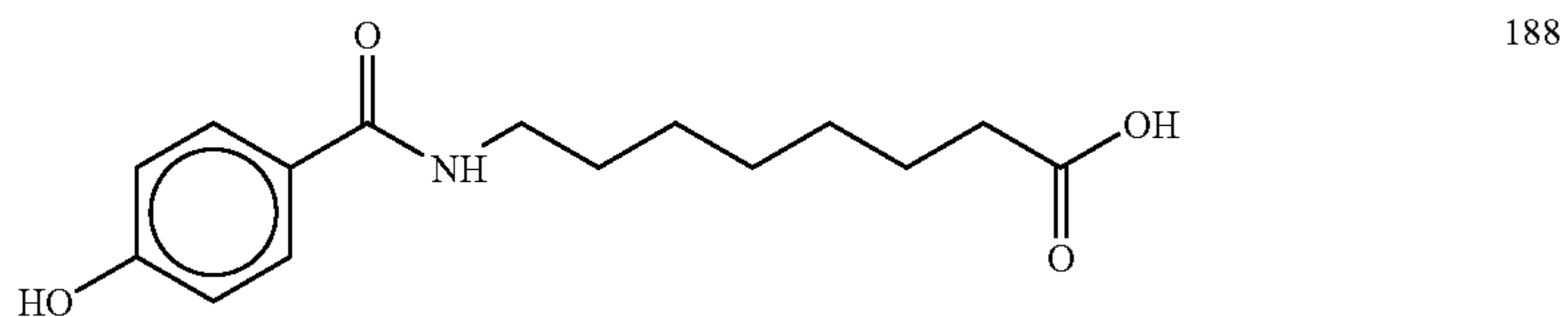
8-(4-Hydroxybenzoyl)aminocaprylic acid
