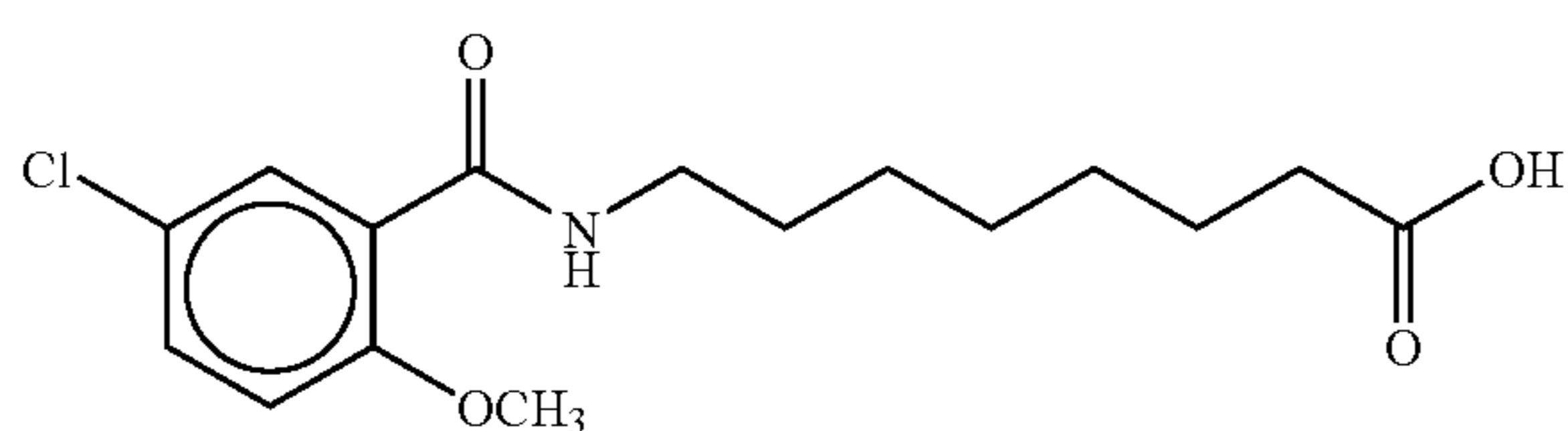
8-(5-chloro-o-anisoyl)aminocaprylic acid
