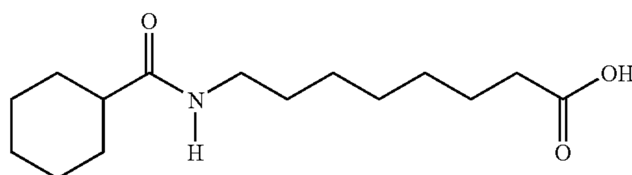
8-N-cyclohexanoylaminovaleric acid
