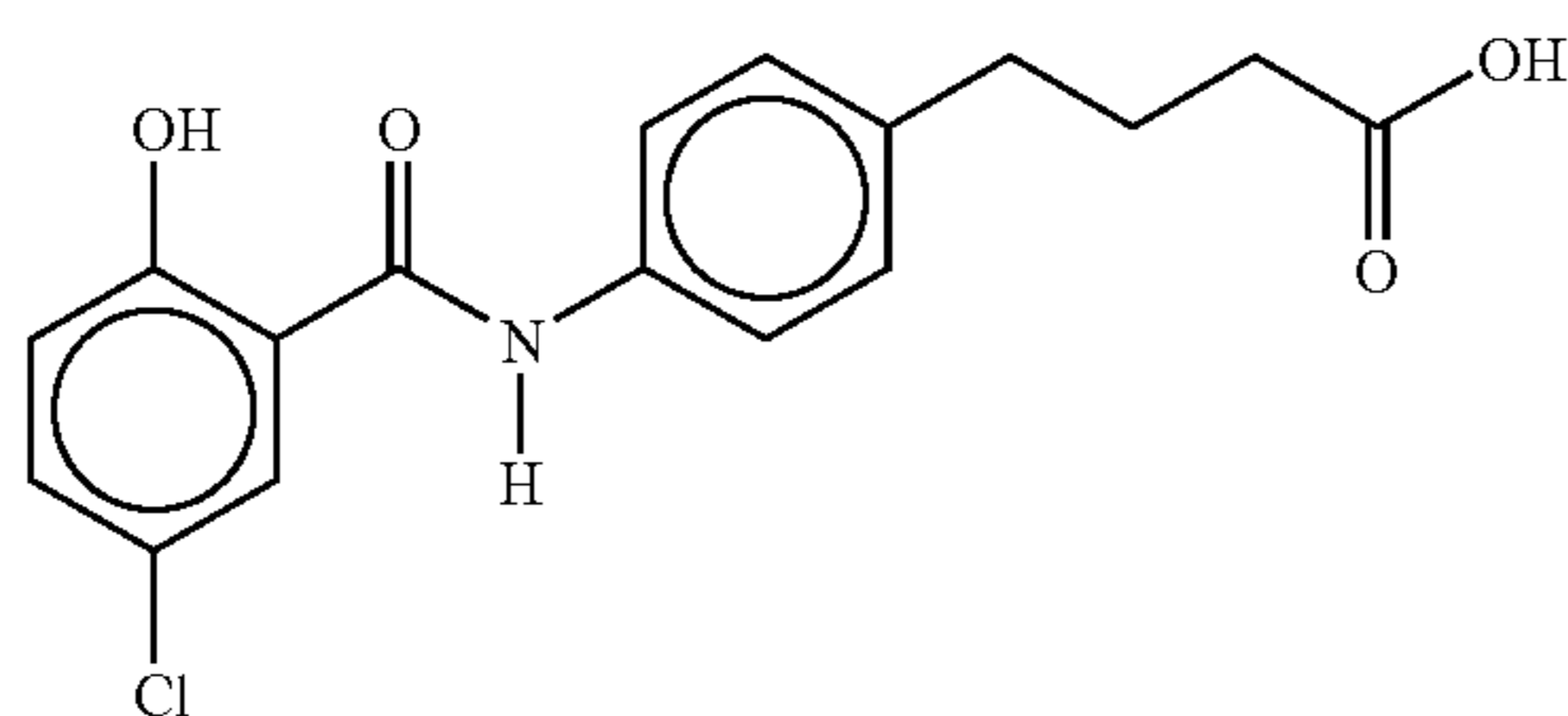
8-N-(2-chloro-6-fluorobenzoyl)aminocaprylic acid
