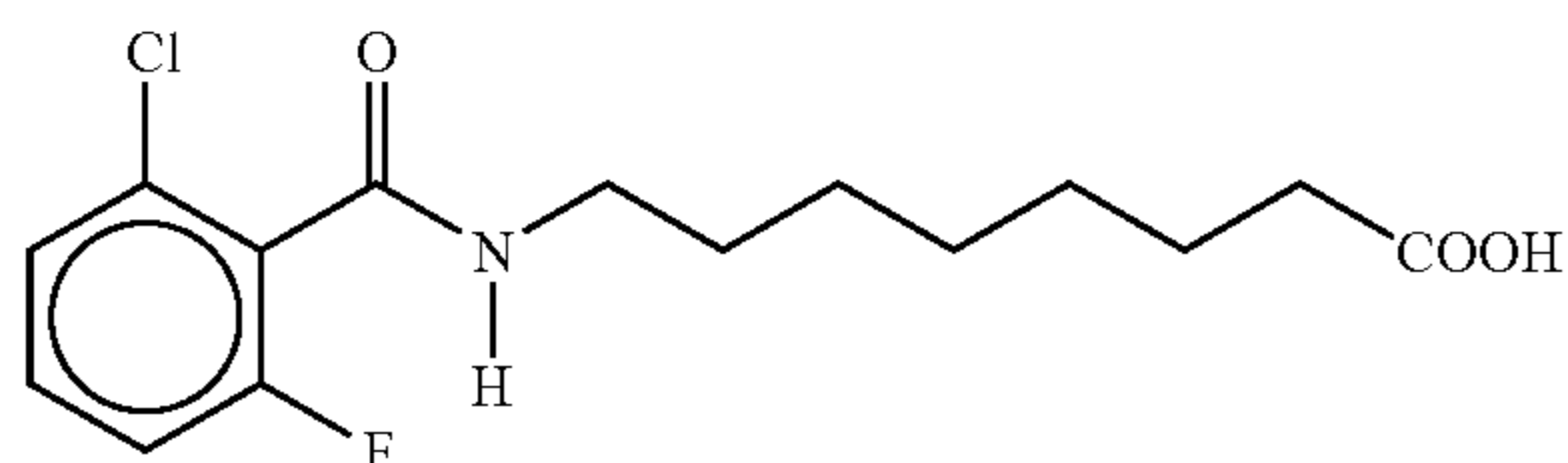
8-N-(2-chloro-6-fluorobenzoyl)aminocaprylic acid
