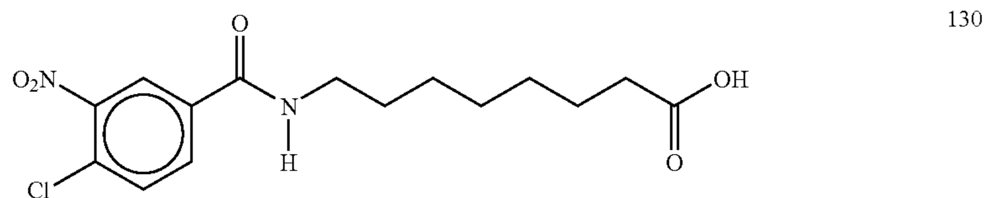
8-(4-chloro-3-nitrobenzoyl)aminocaprylic acid
