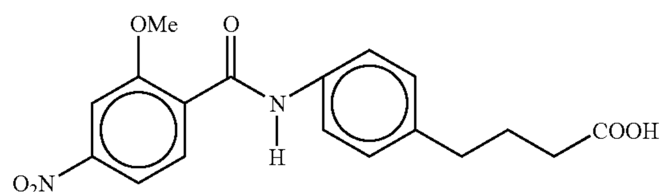
4-{N-[4-(2-methoxy-4-nitrobenzoyl)aminophenyl]}butyric acid
