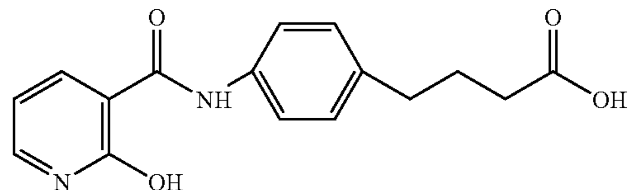
4-(4-(2-hydroxynicotinoyl)aminophenyl)butyric acid
