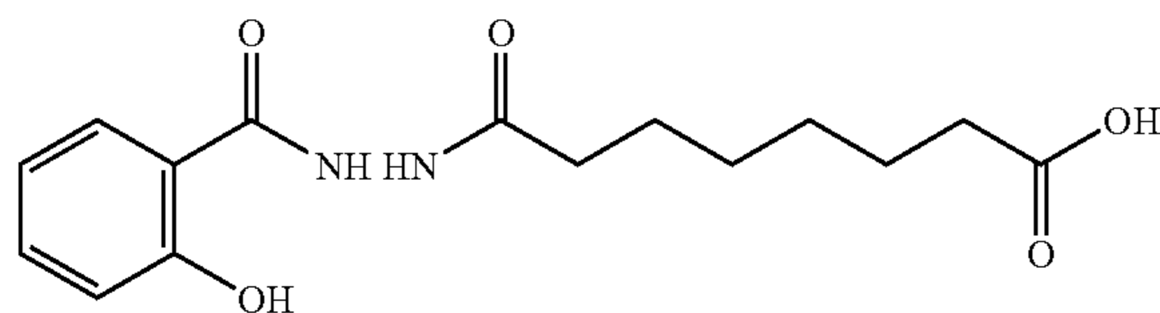
1-salicyloyl-2-suberyl hydrazide
