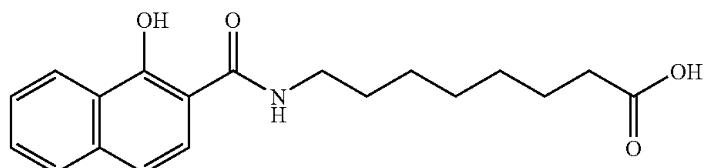
8-(N-(1-hydroxy-2-naphthoyl)aminocaprylic acid
