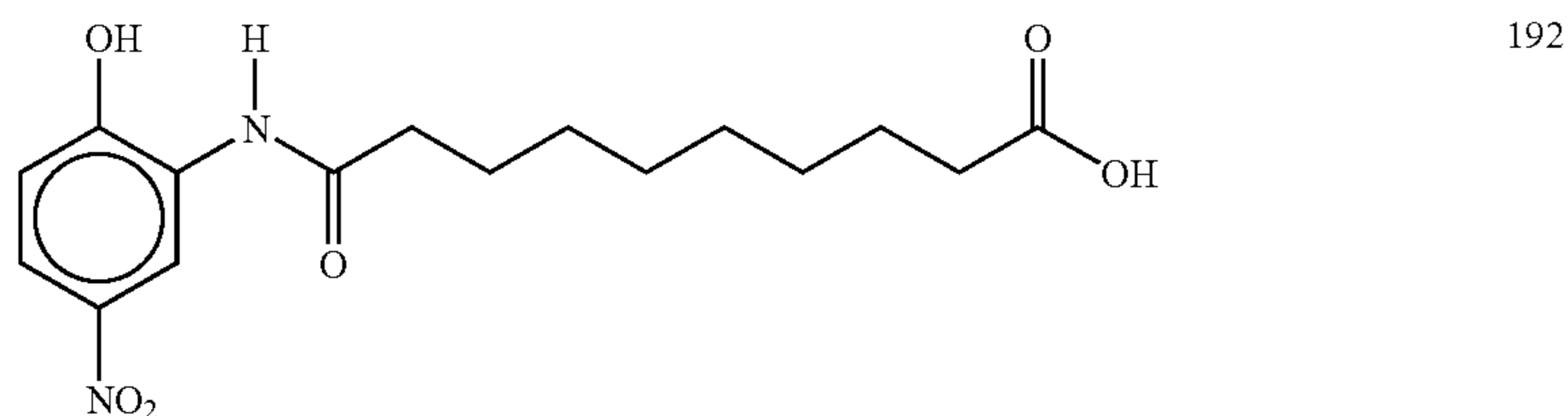
N-10-(2-hydroxy-5-nitroanilino)decanoic acid
