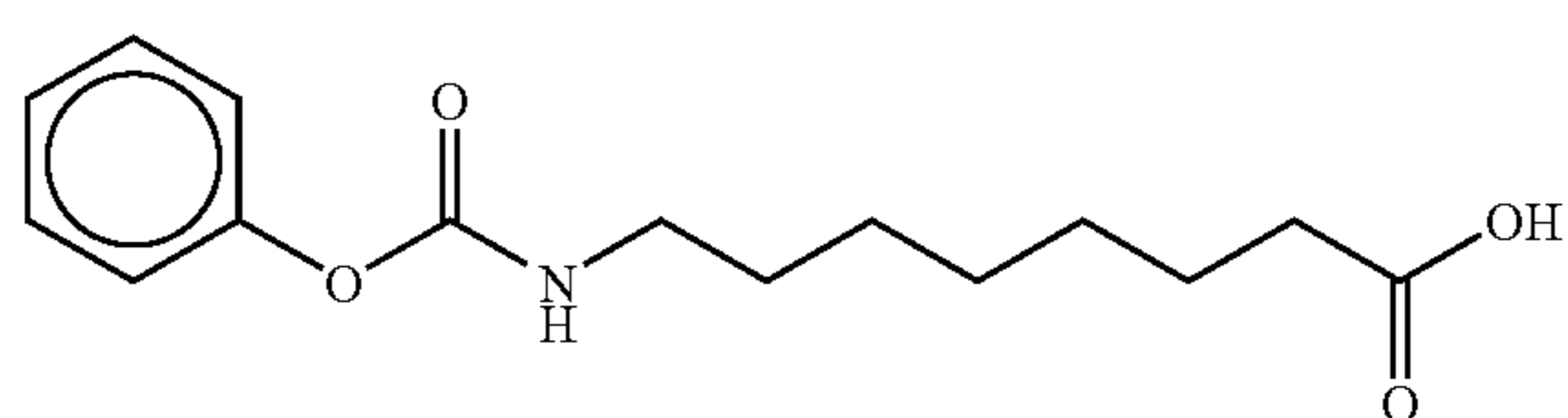
8-(phenylcarbonylamino)caprylic acid
